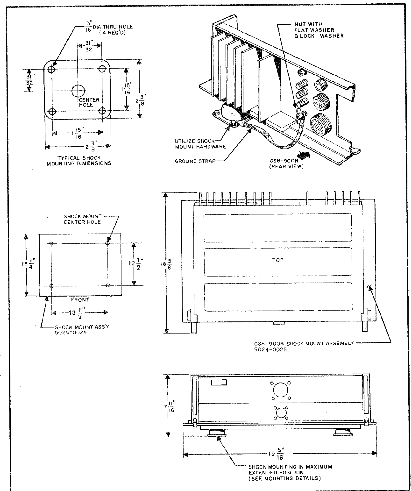
Figure 2.3 Shock Mount Assembly and Details
