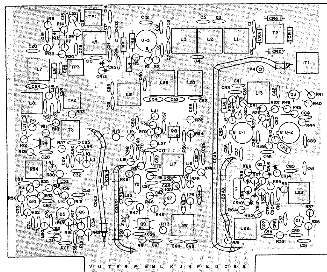
Translator (1A4A3)
