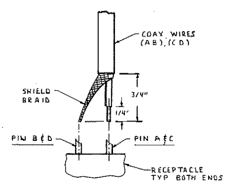
CABLE CONNECTION PROCEDURE DETAIL I
