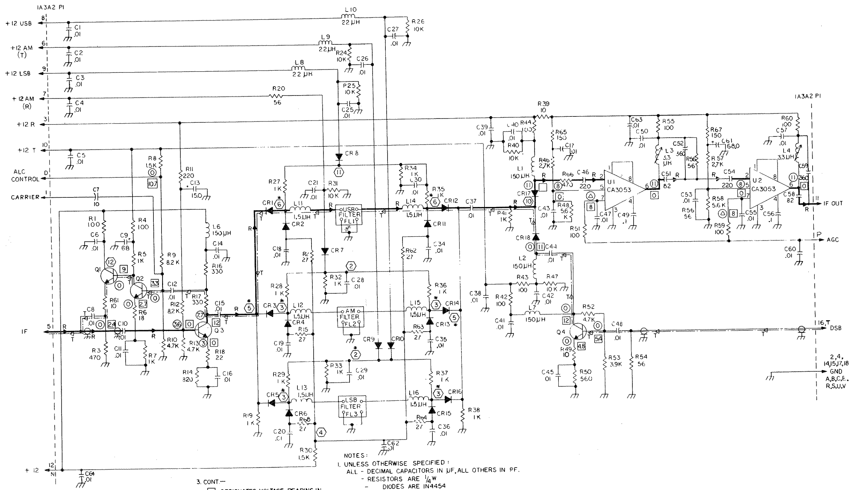
Figure 5.19 IF/Filter (1A3A2) Schematic
