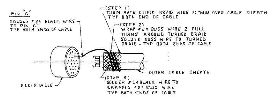
PIN "G" GROUNDING PROCEDURE DETAIL II
