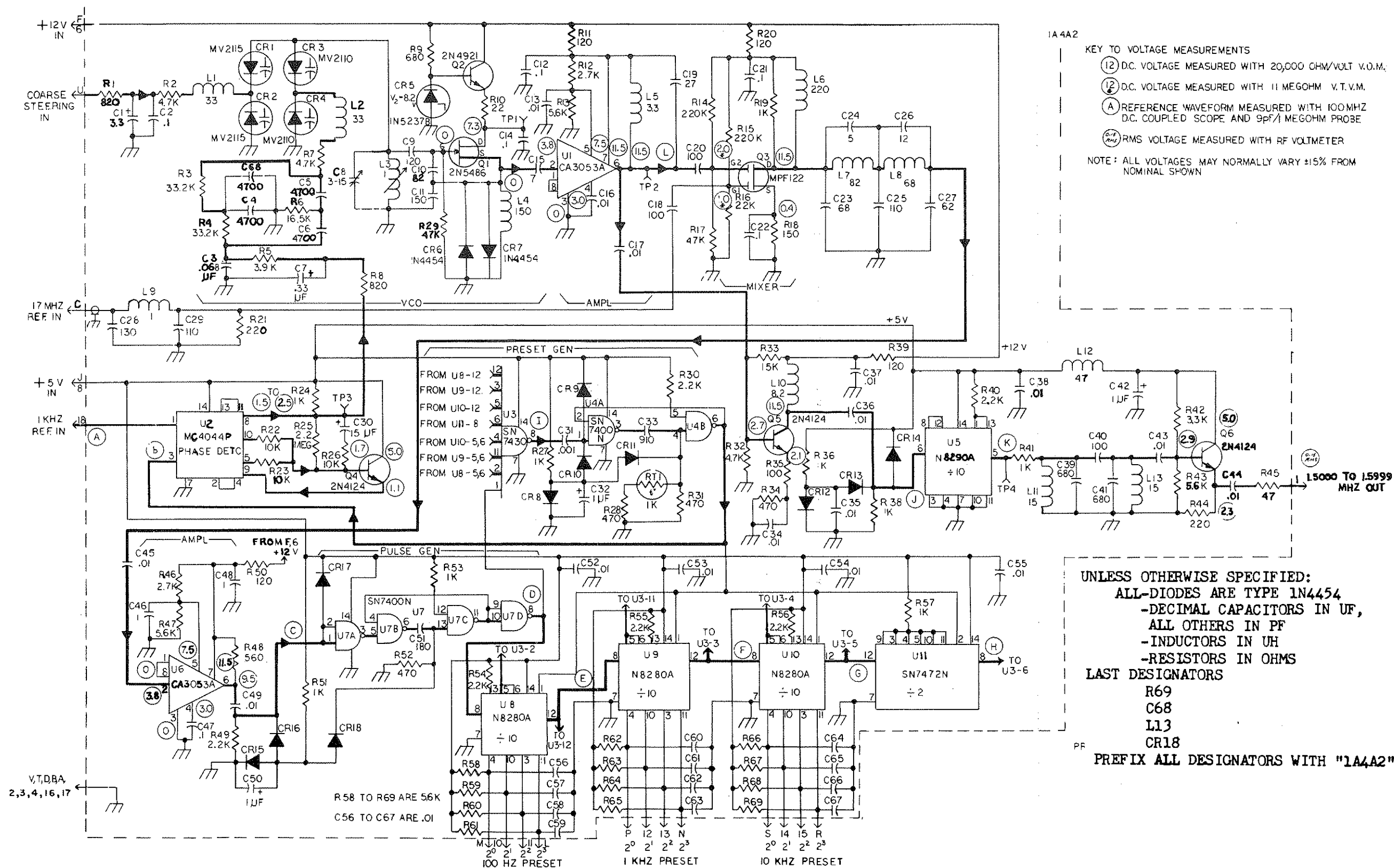
Figure 5.13 Low Digit Generator (1A4A2) Schematic
