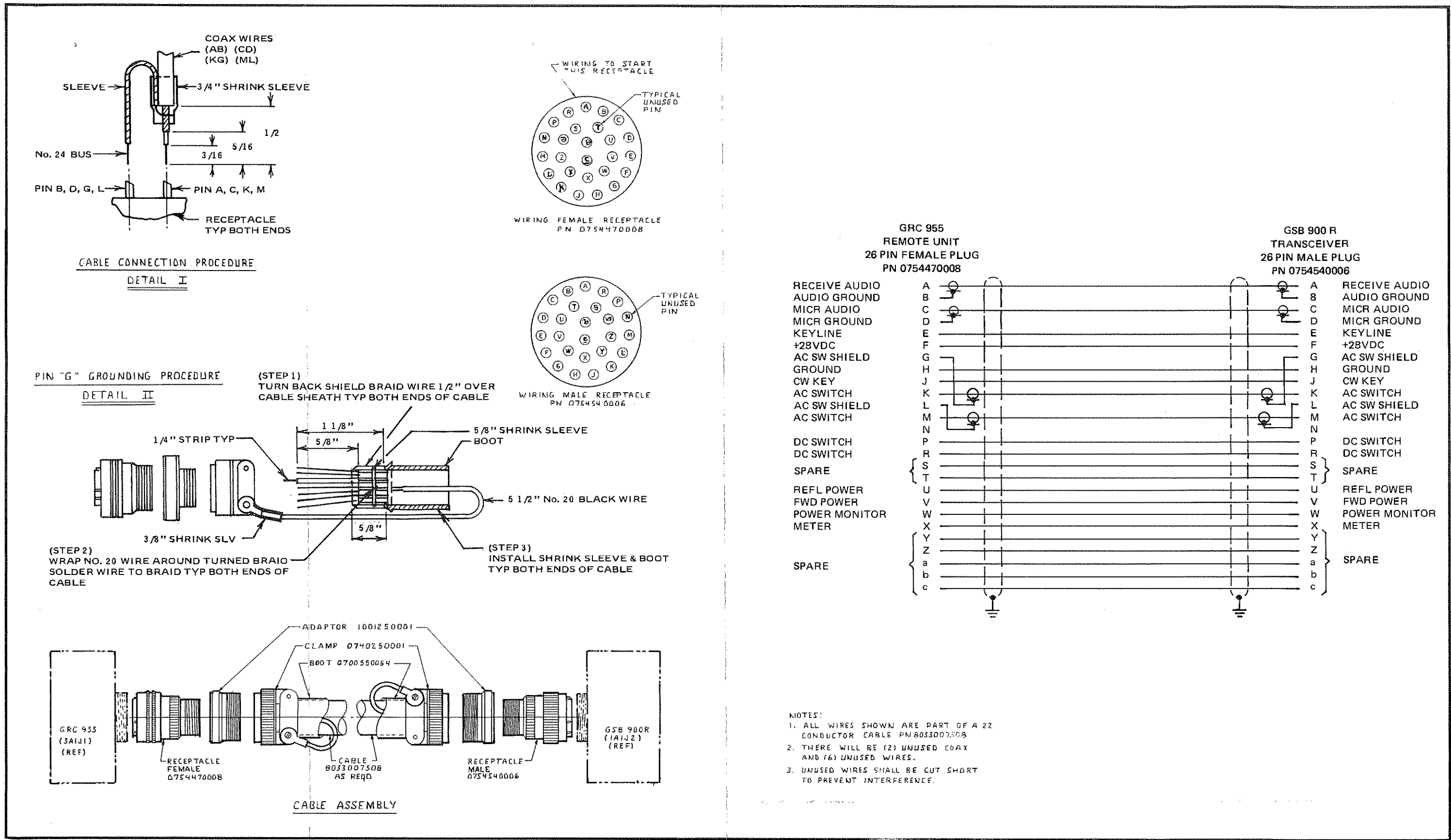
Figure 2.6B Interconnecting Cable Diagram and Ass'y (22 Wire) Change Date 19 Feb 1981
