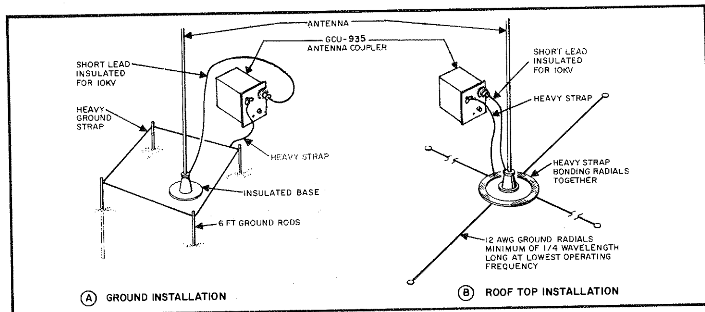
Figure 2.7 Whip Antenna
