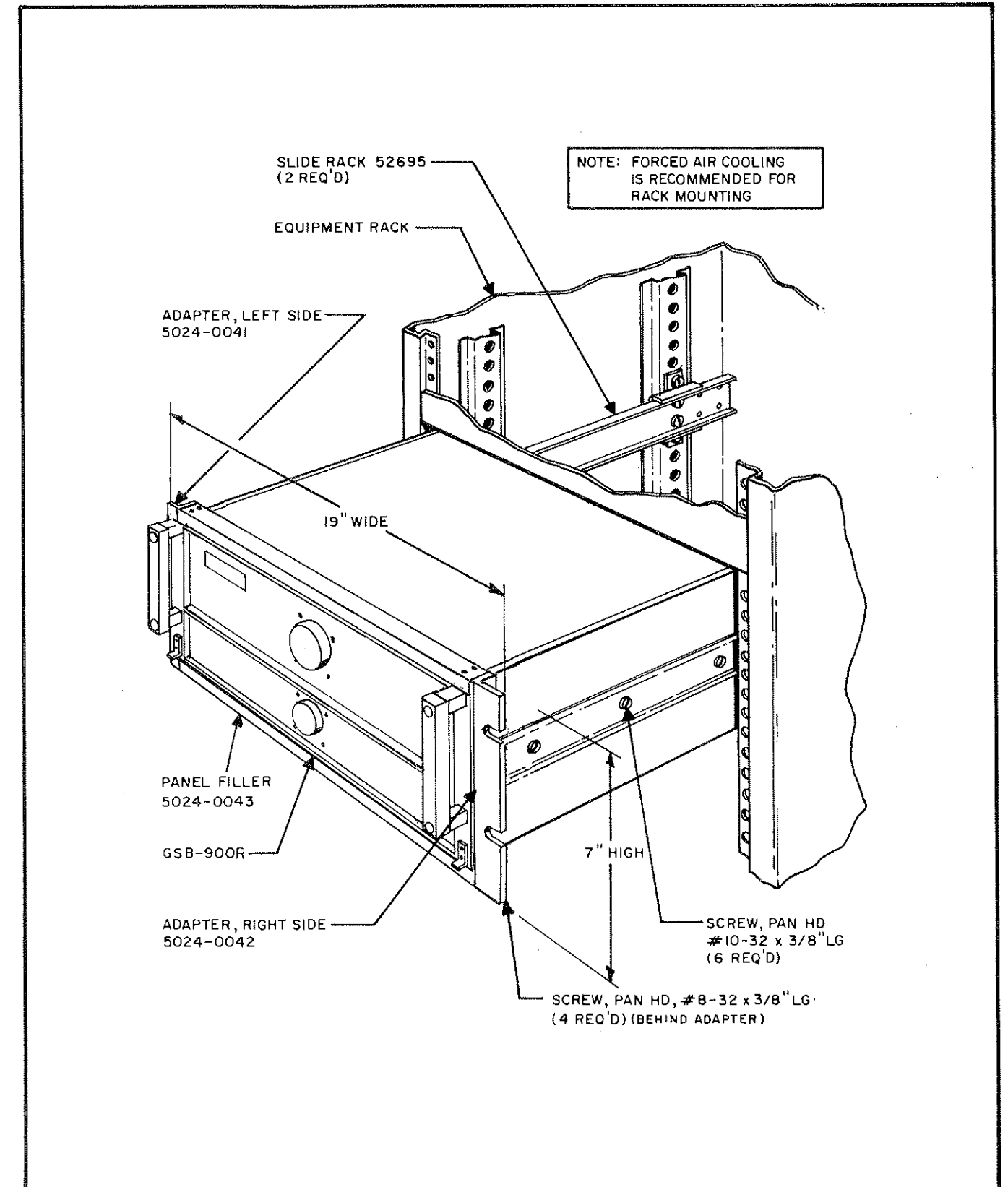
Figure 2.5 Rack Mounted Installation
