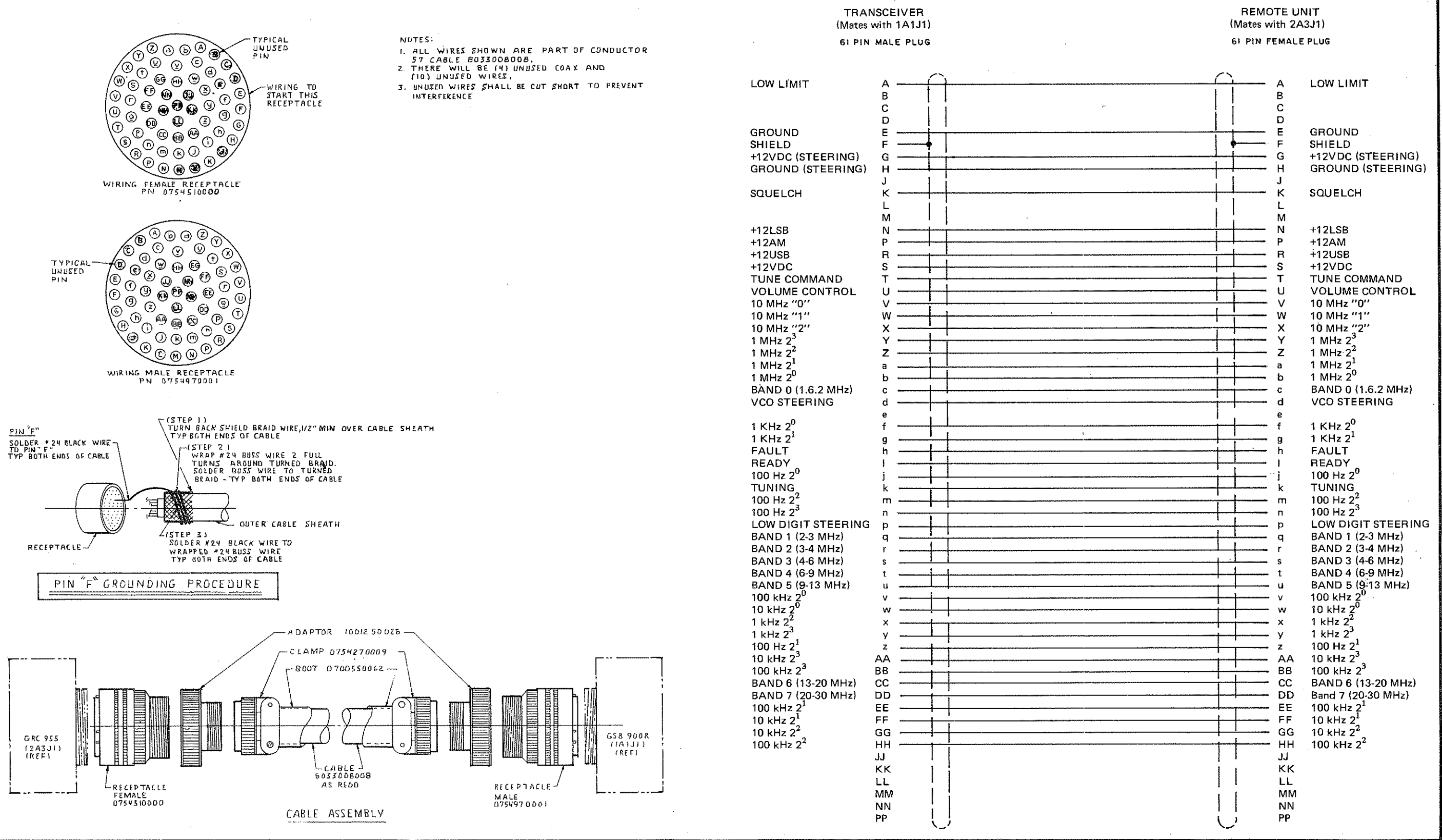
Figure 2.6A Interconnecting Cable Diagram and Ass'y (57 Wire)
