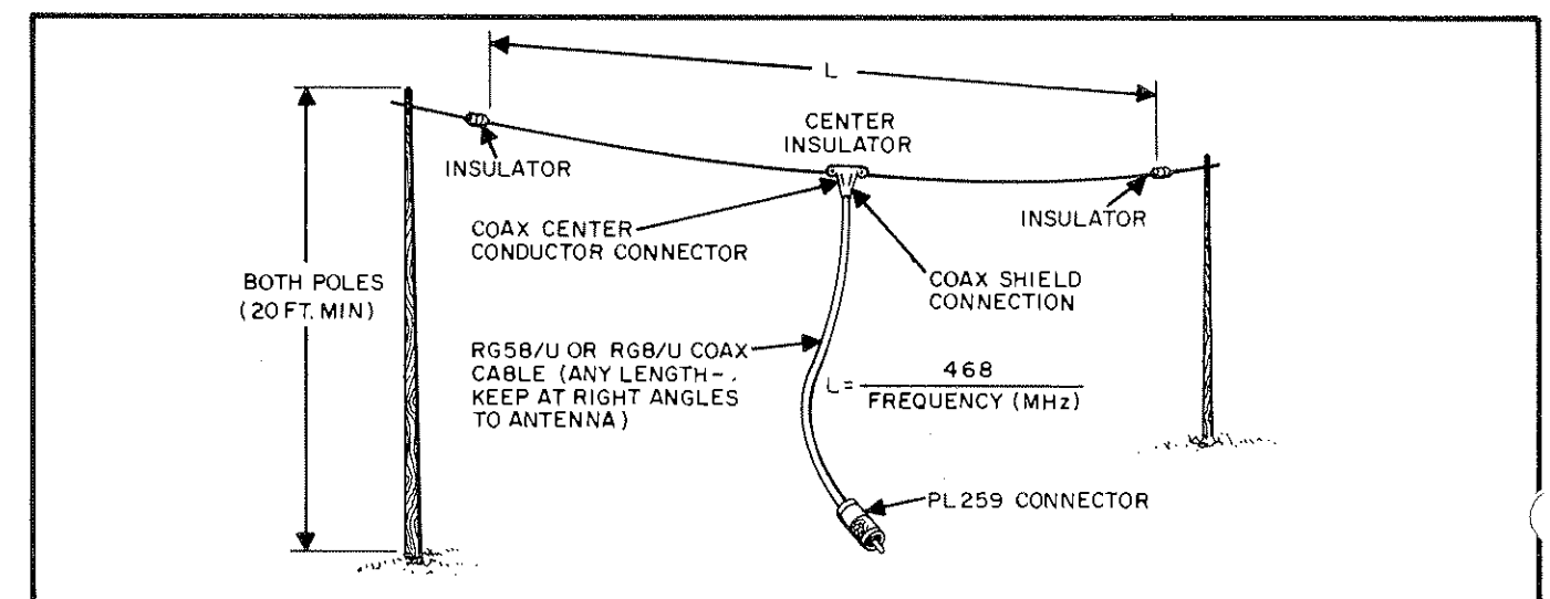
Figure 2.8 Doublet Antenna
