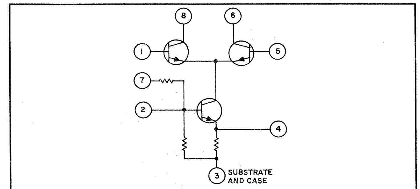
Figure 4.3 CA3053 Schematic of U1 and U2
