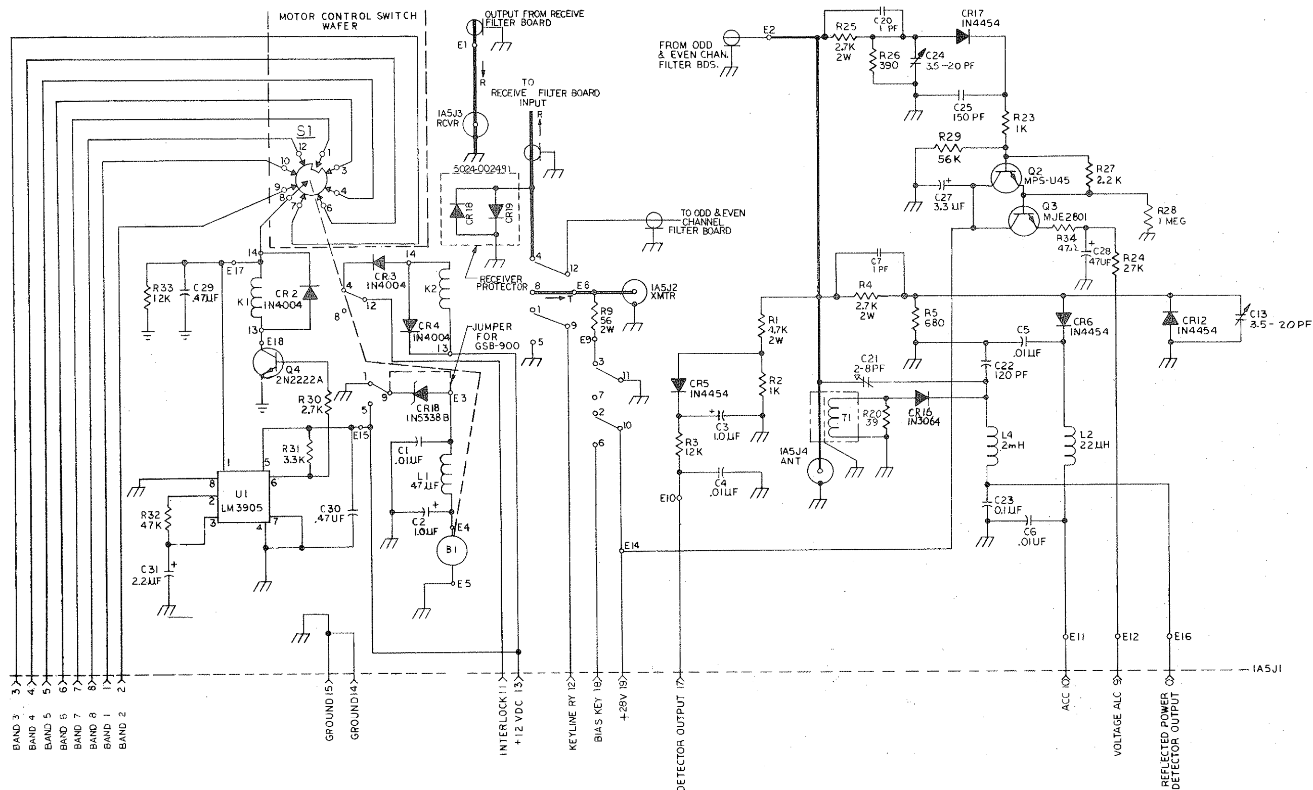
Figure 5.28 Motor Control Board (1A5A4) Schematic
