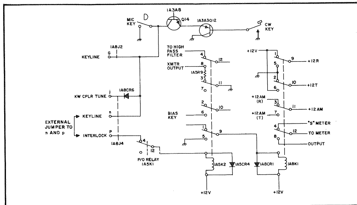
Figure 4.8 Keying Circuit
