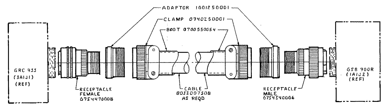
CABLE ASSEMBLY
