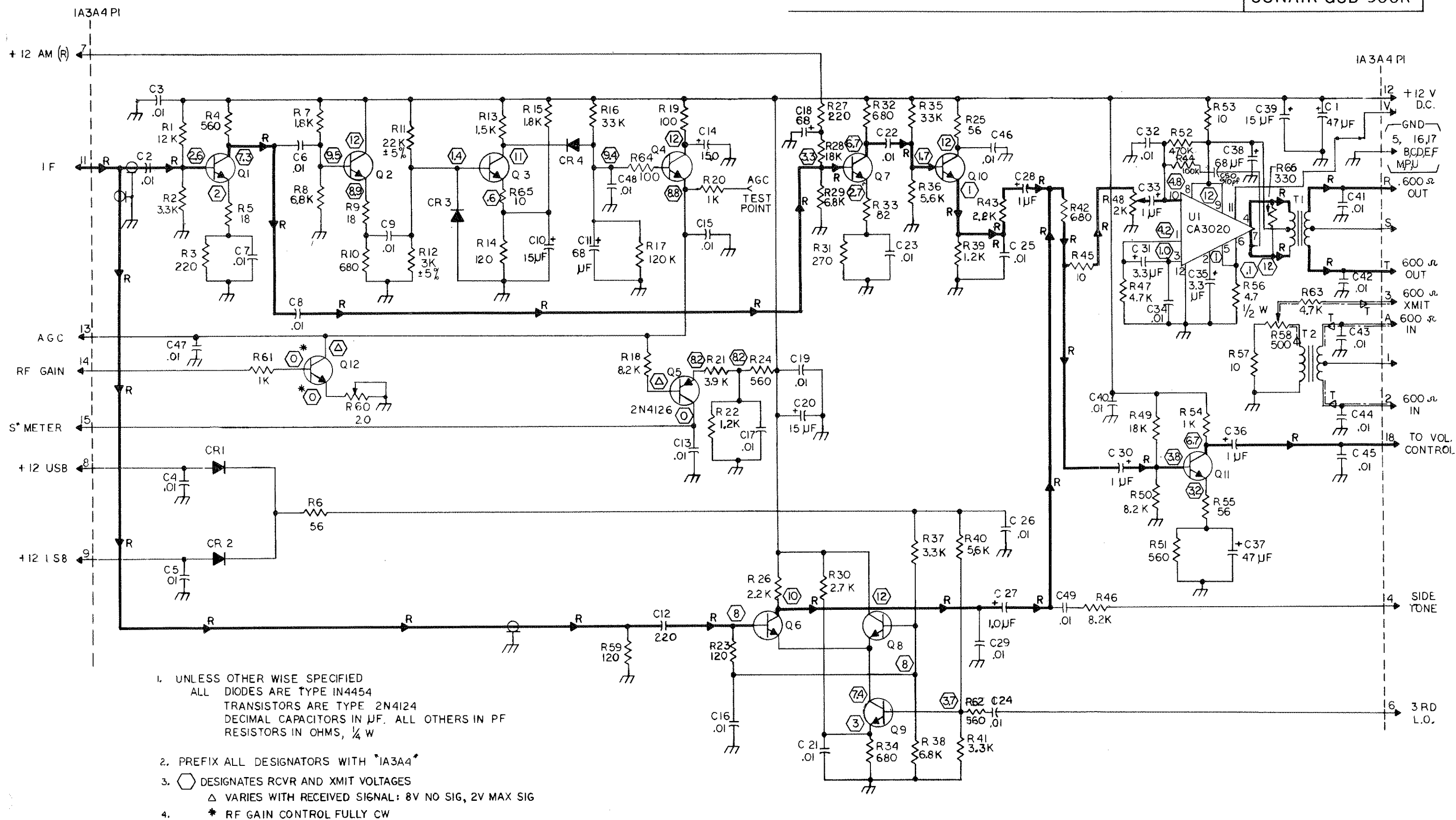
Figure 5.20 Audio Board (1A3A4) Schematic
