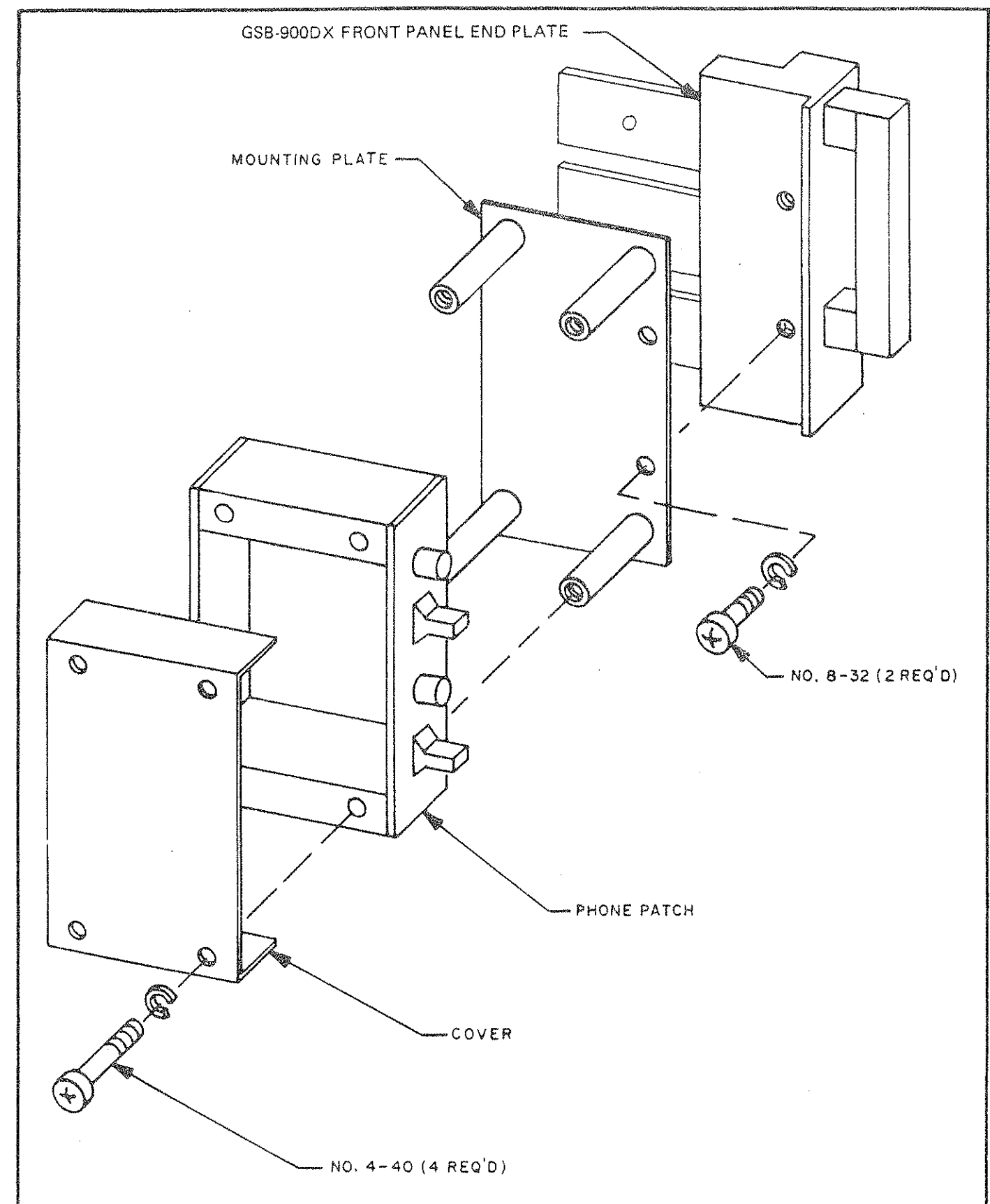
Figure 6.1 GSB-900DX Phone Patch Mounting Instructions
