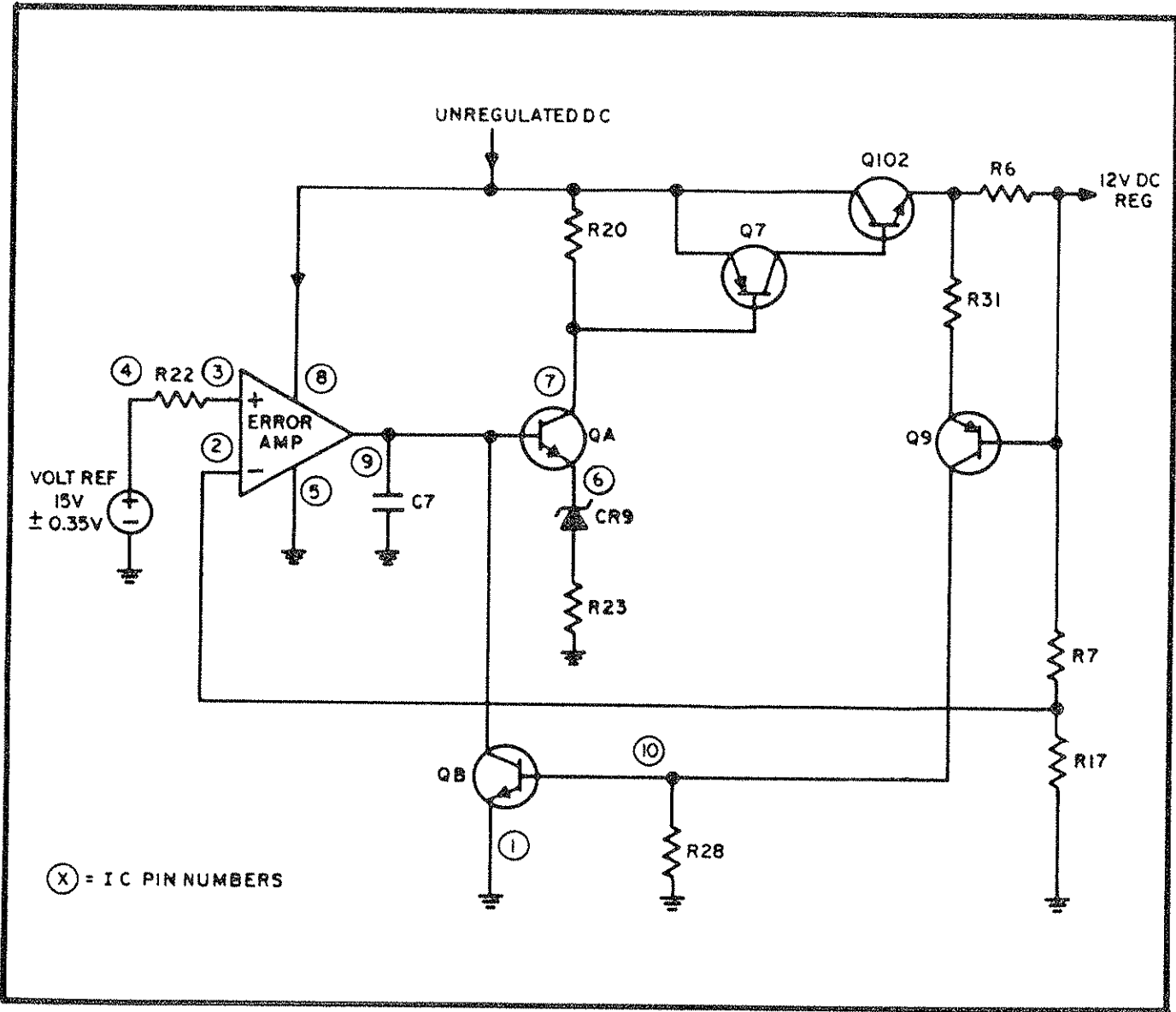
Figure 4.7 723IC Regulator
