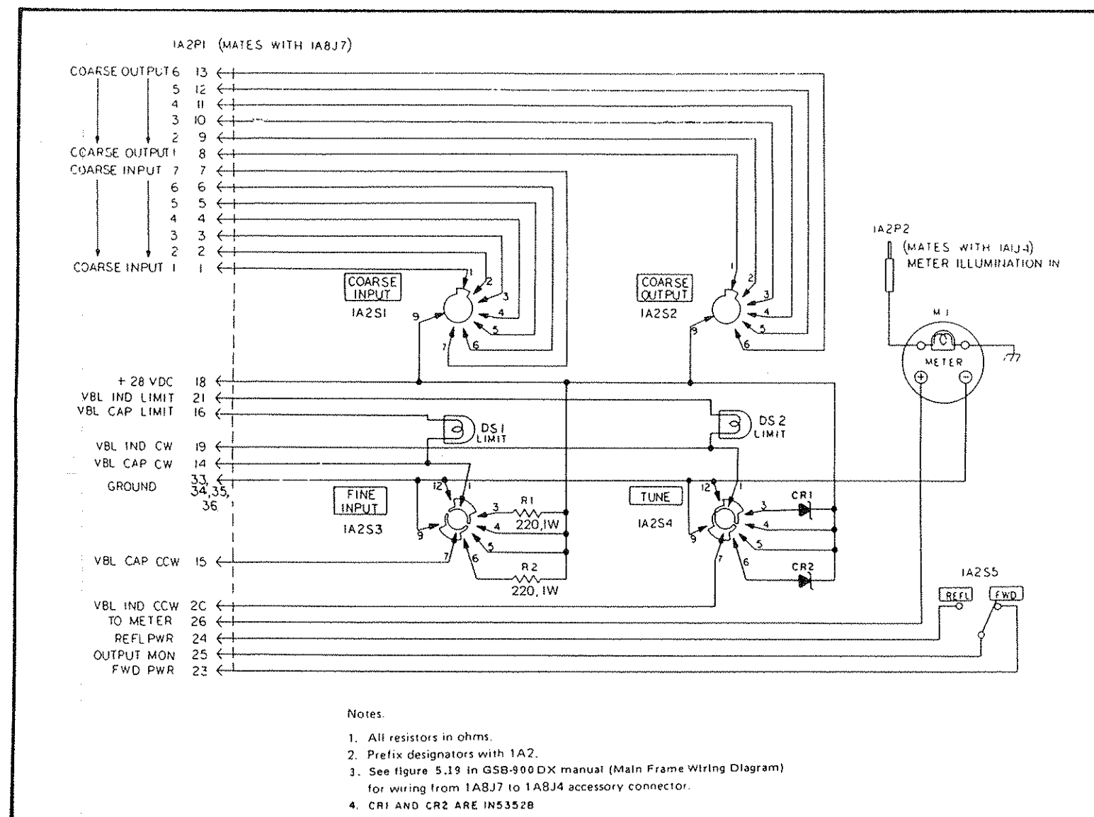
Figure 5.22 Schematic Diagram GCU-910A Antenna Tuning Control Unit
