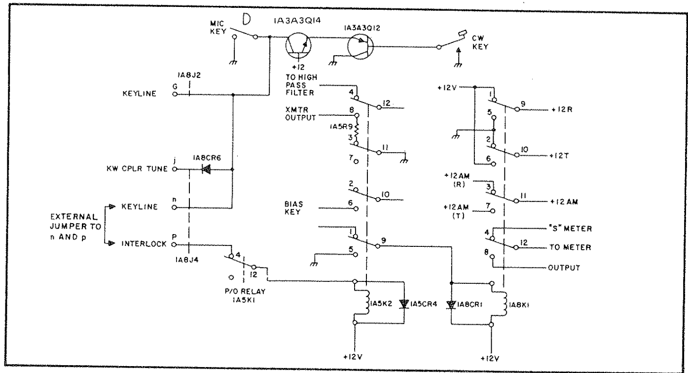
Figure 4.10 Keying Circuit
