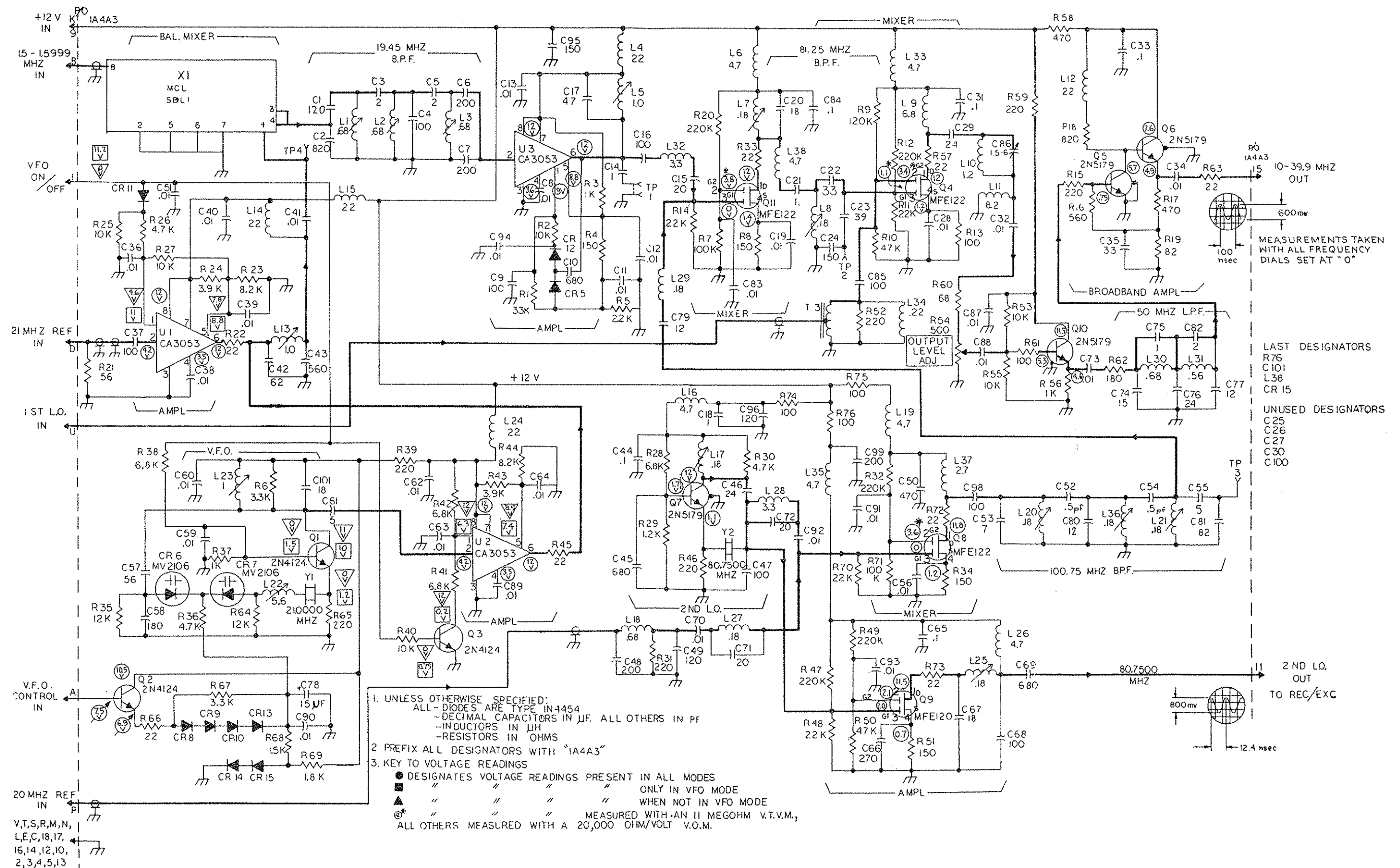
Figure 5.26 Translator Schematic (1A4A3)
