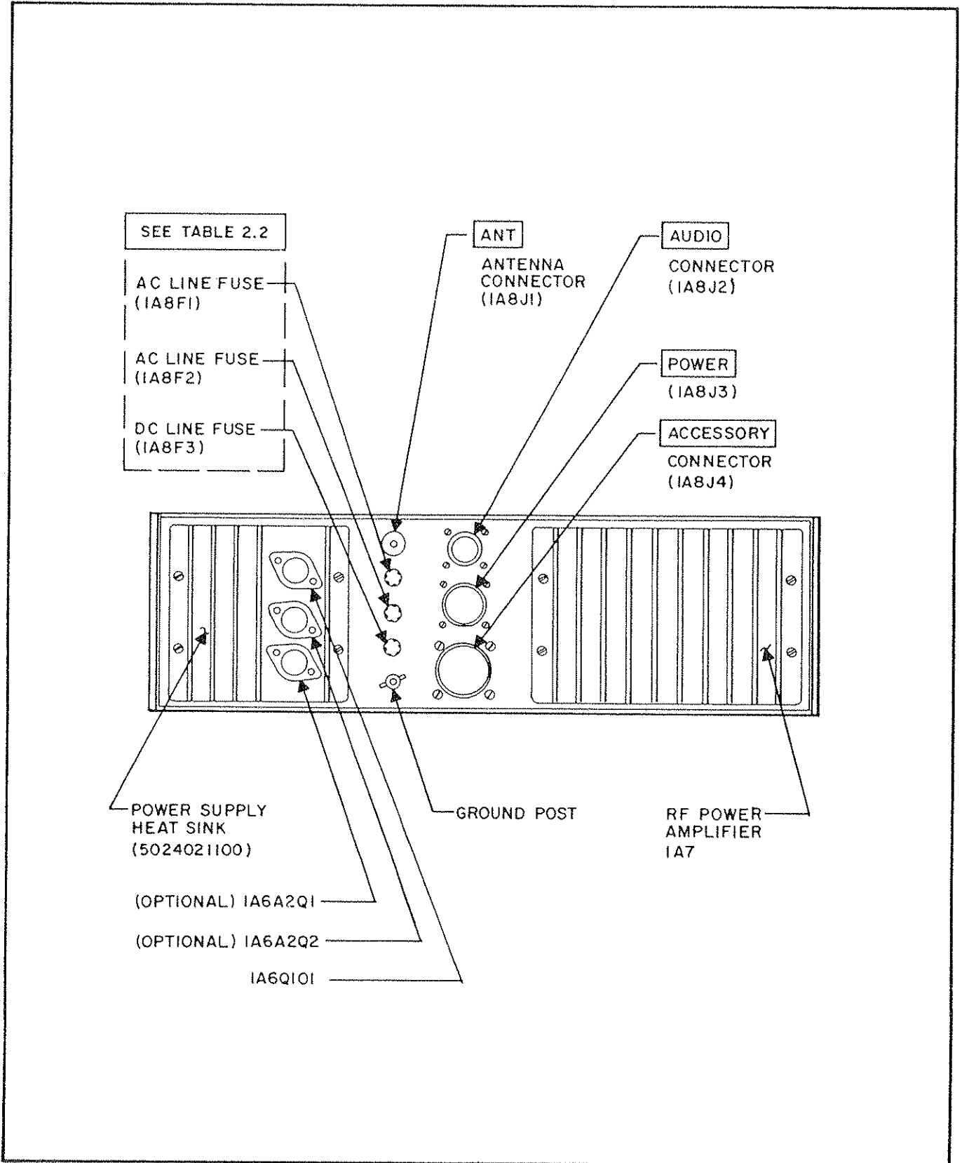
Figure 3.2 GSB-900DX Rear Aprons Components and Connectors
