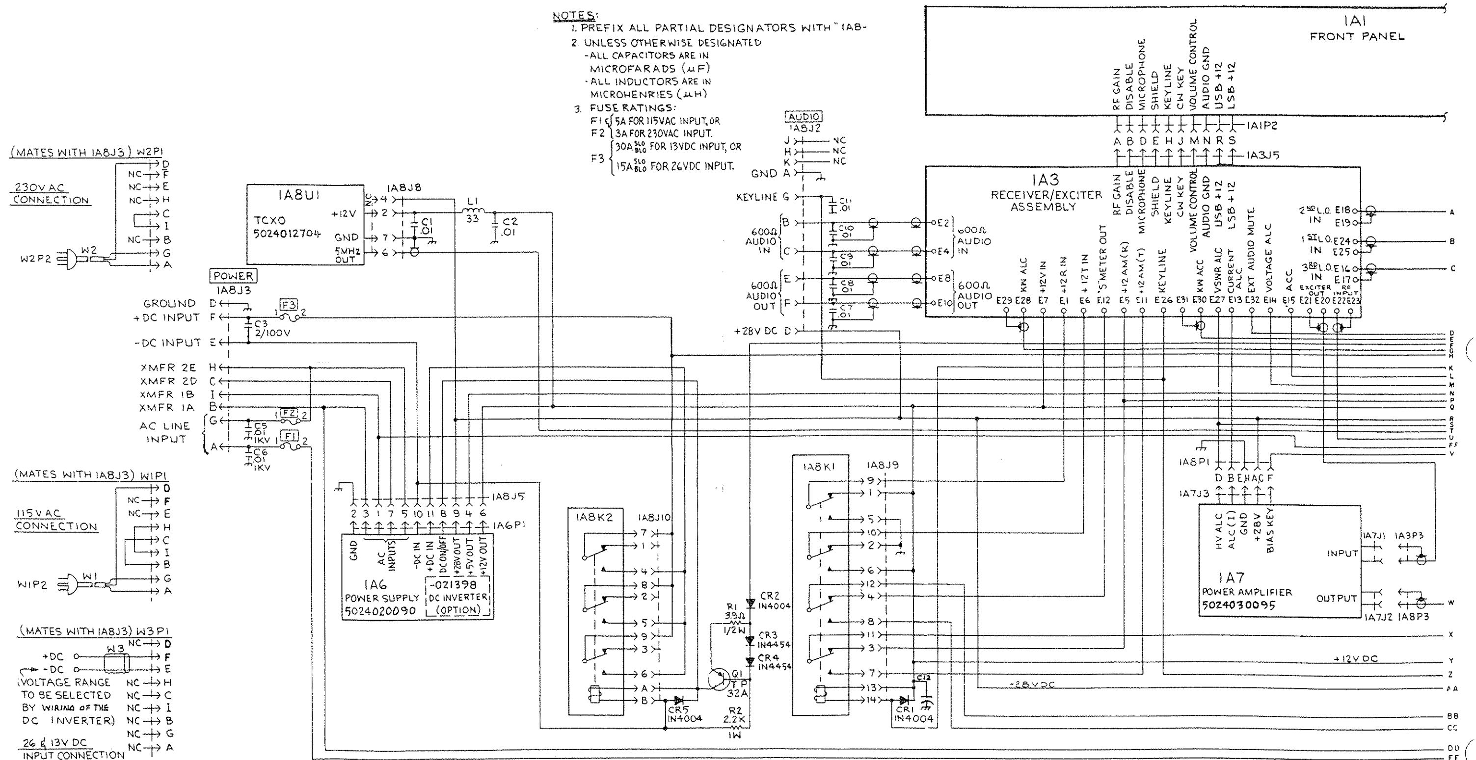
Figure 5.19 Main Frame Wiring
