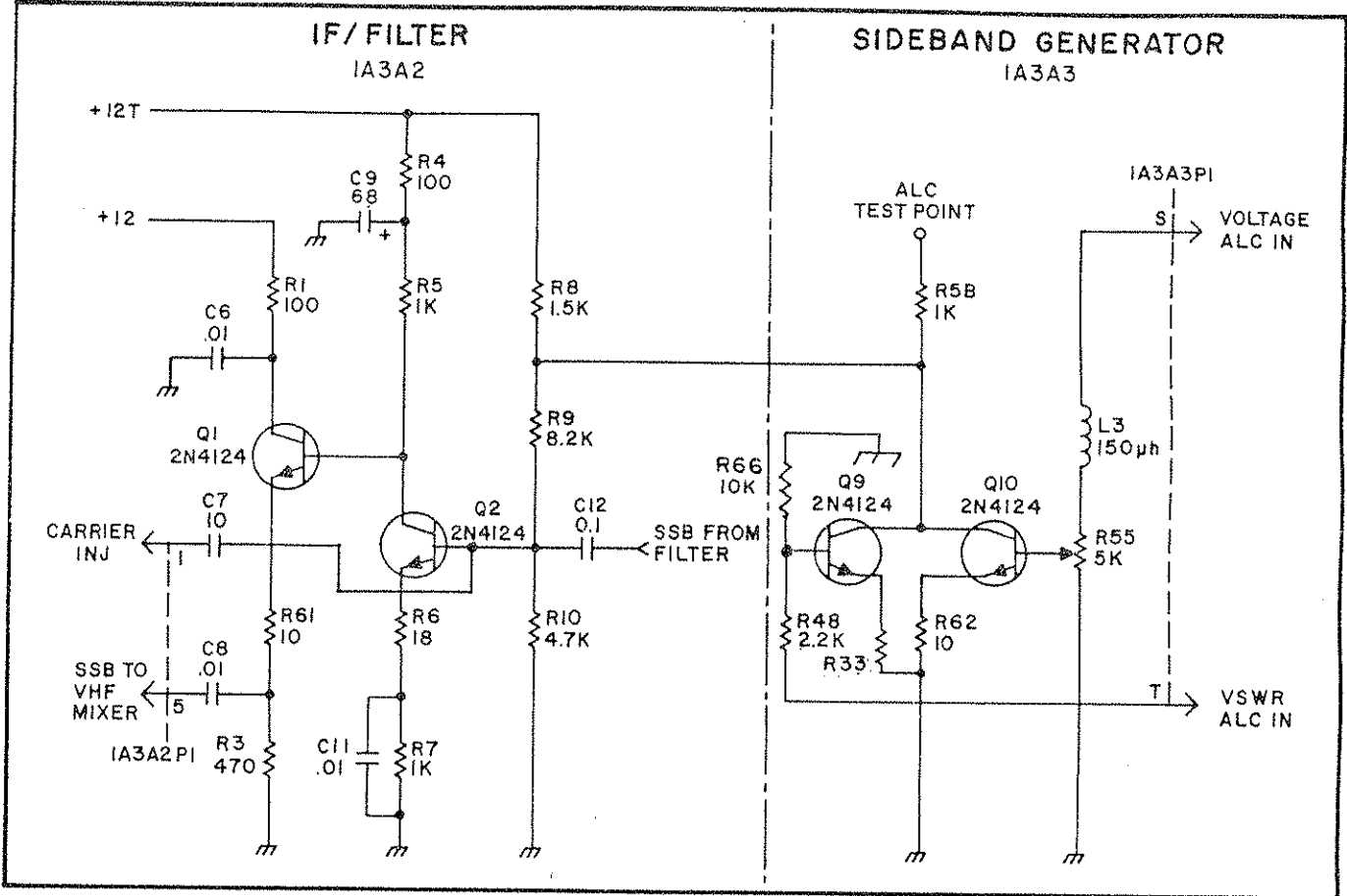
Figure 4.5 Voltage &amp; VSWR ALC Control Schematic
