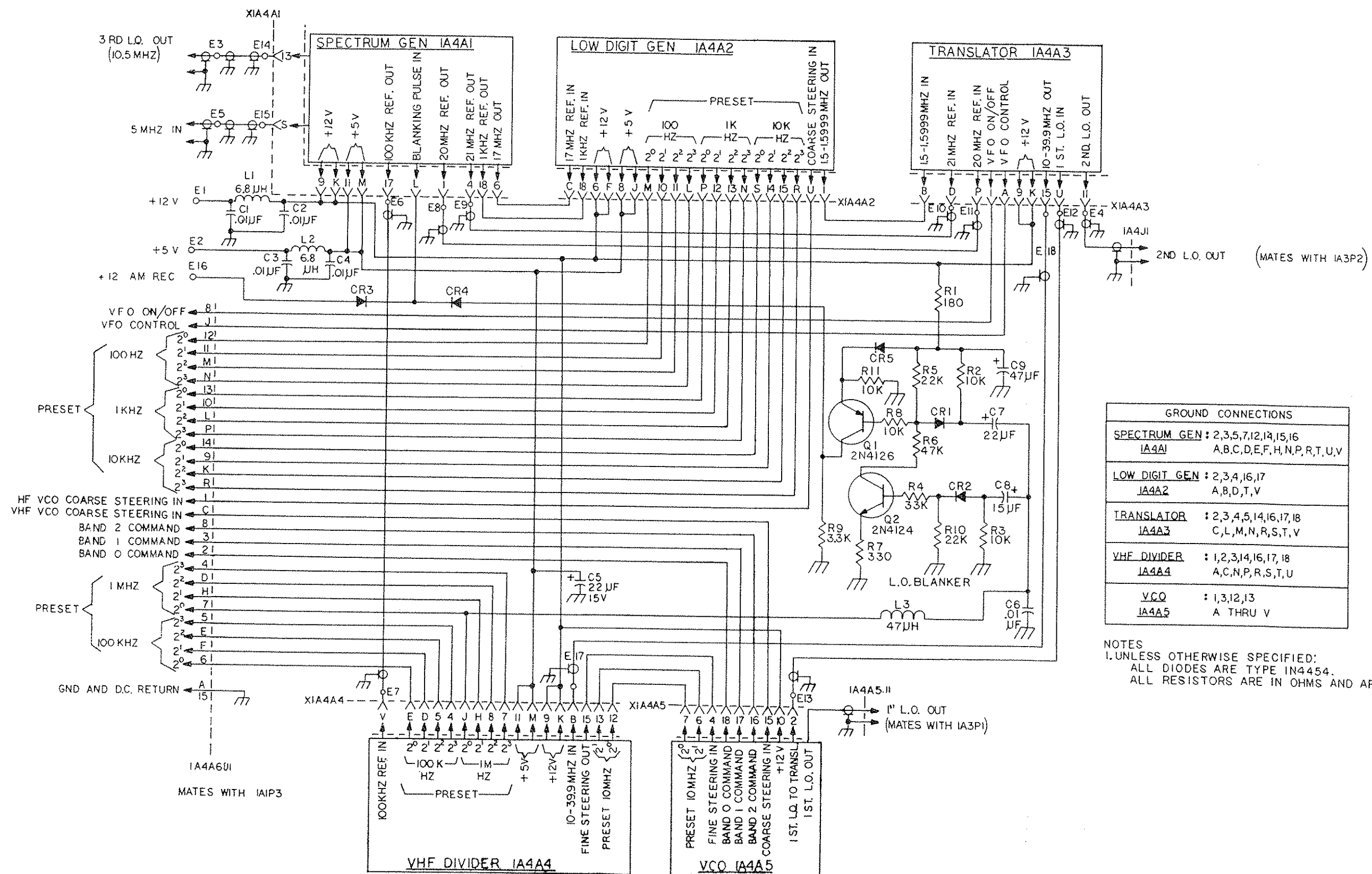
Figure 5.29 Synthesizer Mother Board (1A4A6) Schematic
