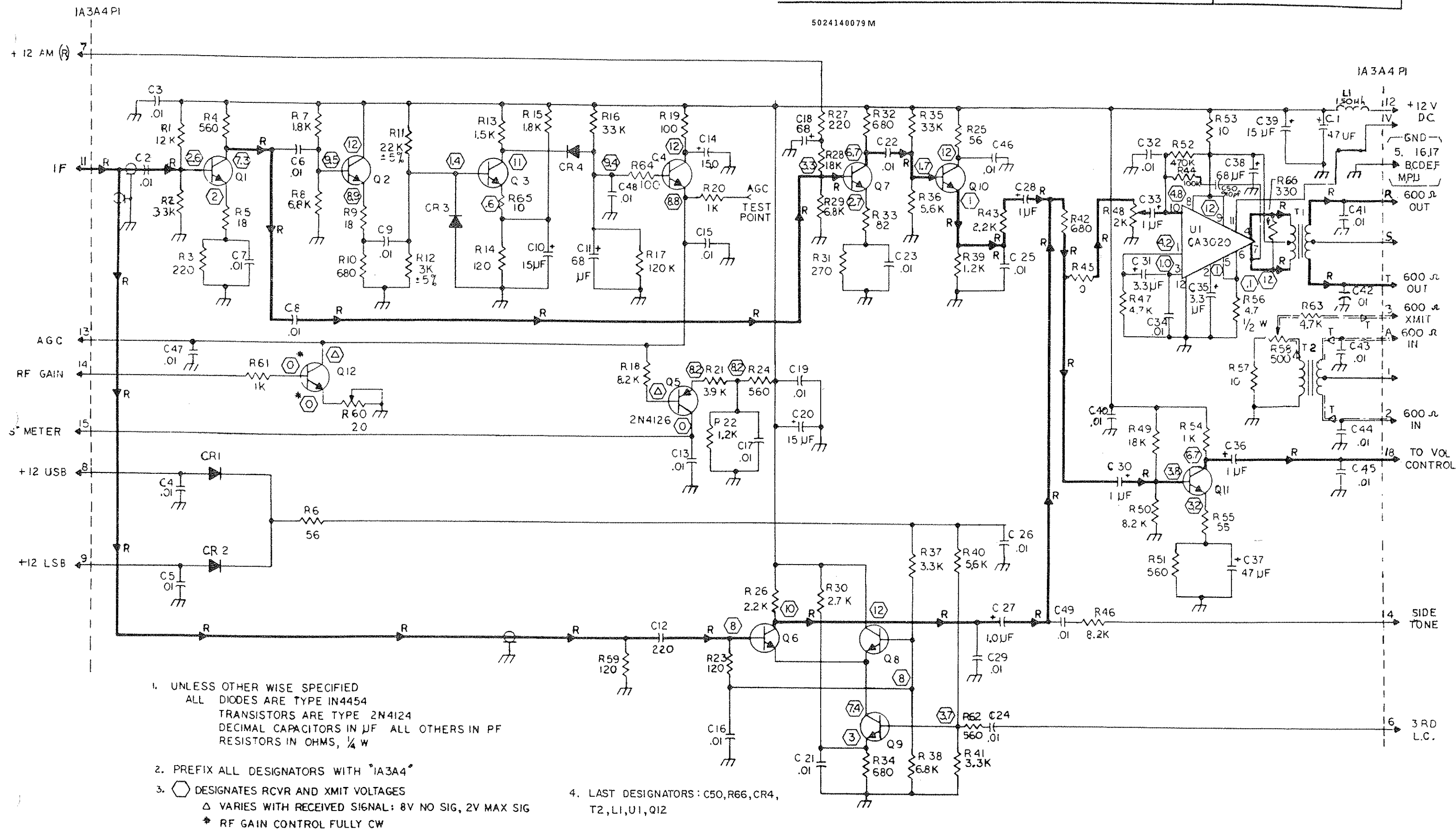
Figure 5.32 Audio Board Schematic (1A3A4)
