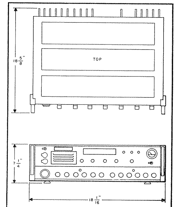
Figure 2.1 Outline Configuration
