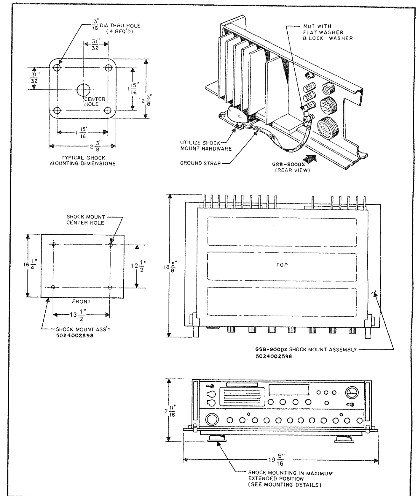
Figure 2.4 Shock Mount Assembly and Details
