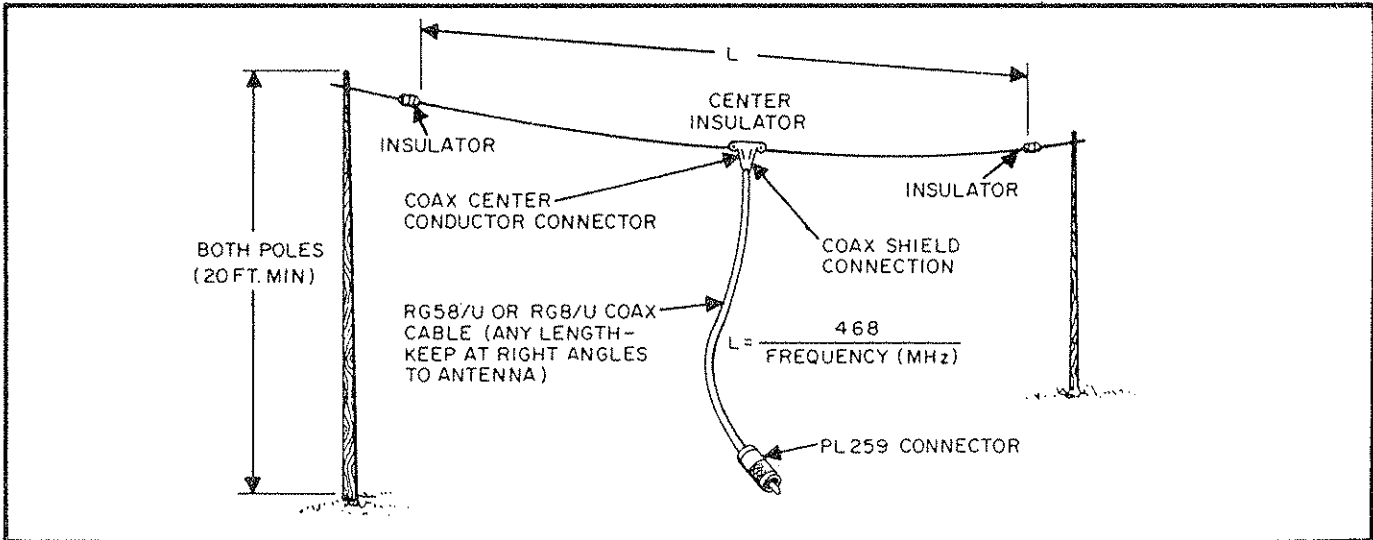
Figure 2.8 Doublet Antenna
