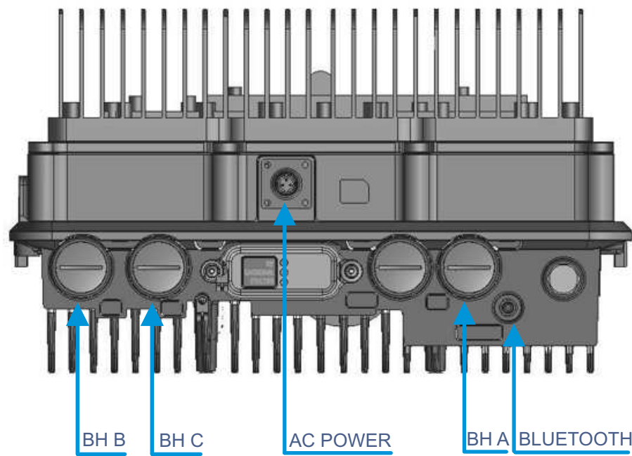
Figure 37 Flexi Zone Micro BTS (FWGR) interfaces - bottom view
