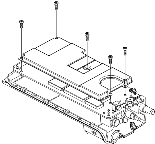
Figure 33. Removing the Main Board from the Chassis
