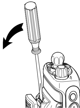
Figure 23. Removing the Belt Clip
