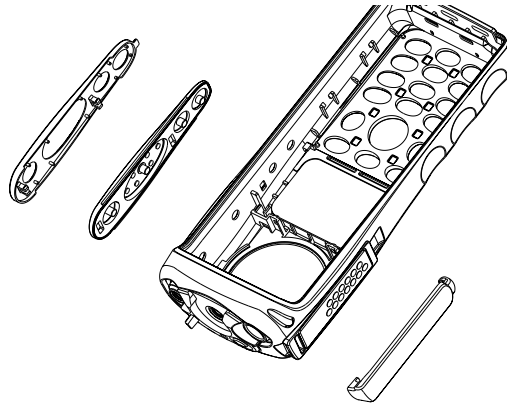
Figure 39. PTT Removal
