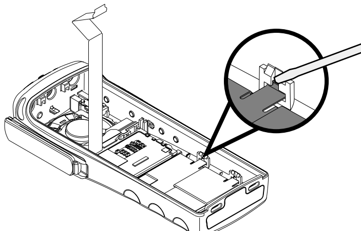
Figure 35. Retainer Removal
