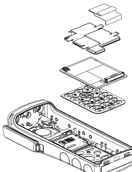
Figure 36. Keypad Retainer and Boards Removal
