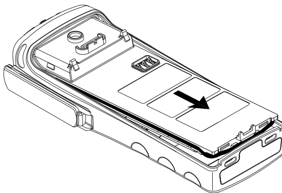
Figure 31. Chassis Separation
