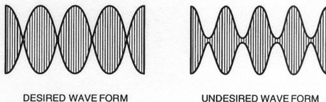
Figure 4. AME Waveforms
