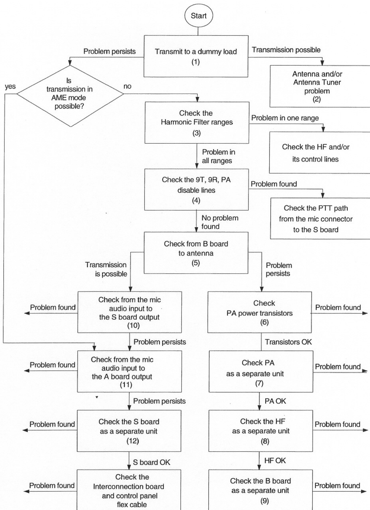
Figure 8. Transmitter Troubleshooting Chart
