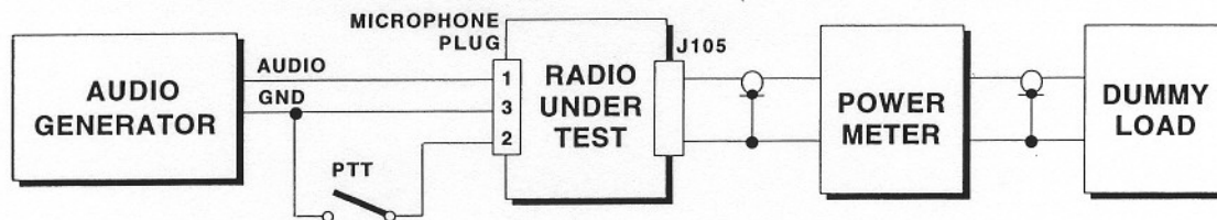
a. Transmitter Test Setup with Serial Power Meter
