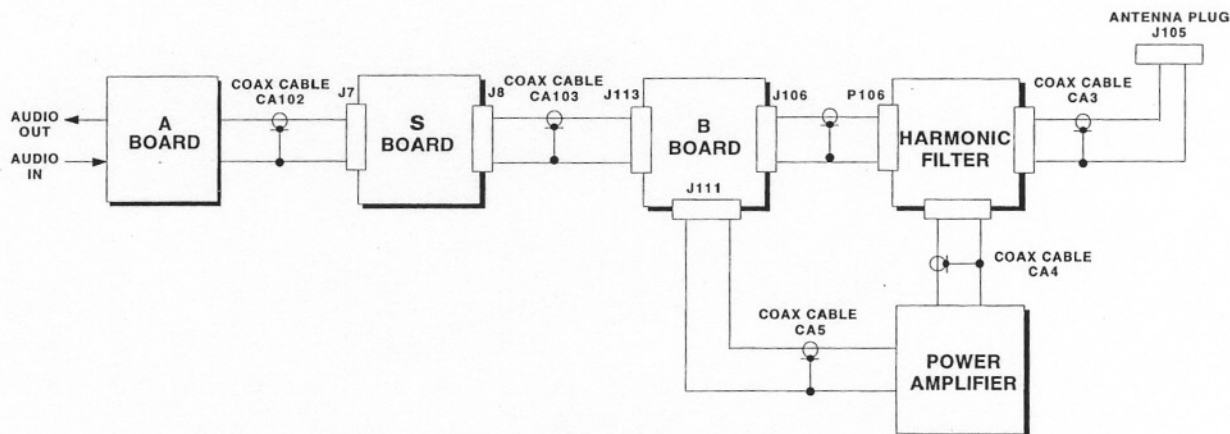
Figure 7. RF Connections between the Radio's Units
