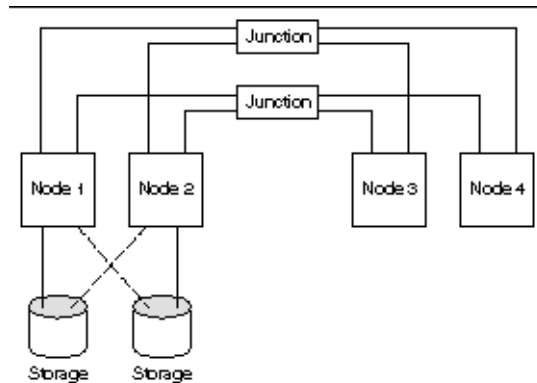
FIGURE 2-4 Pair+N Topology
