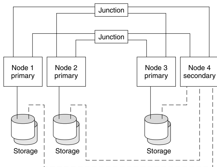
FIGURE 2-5 N+1 Topology
