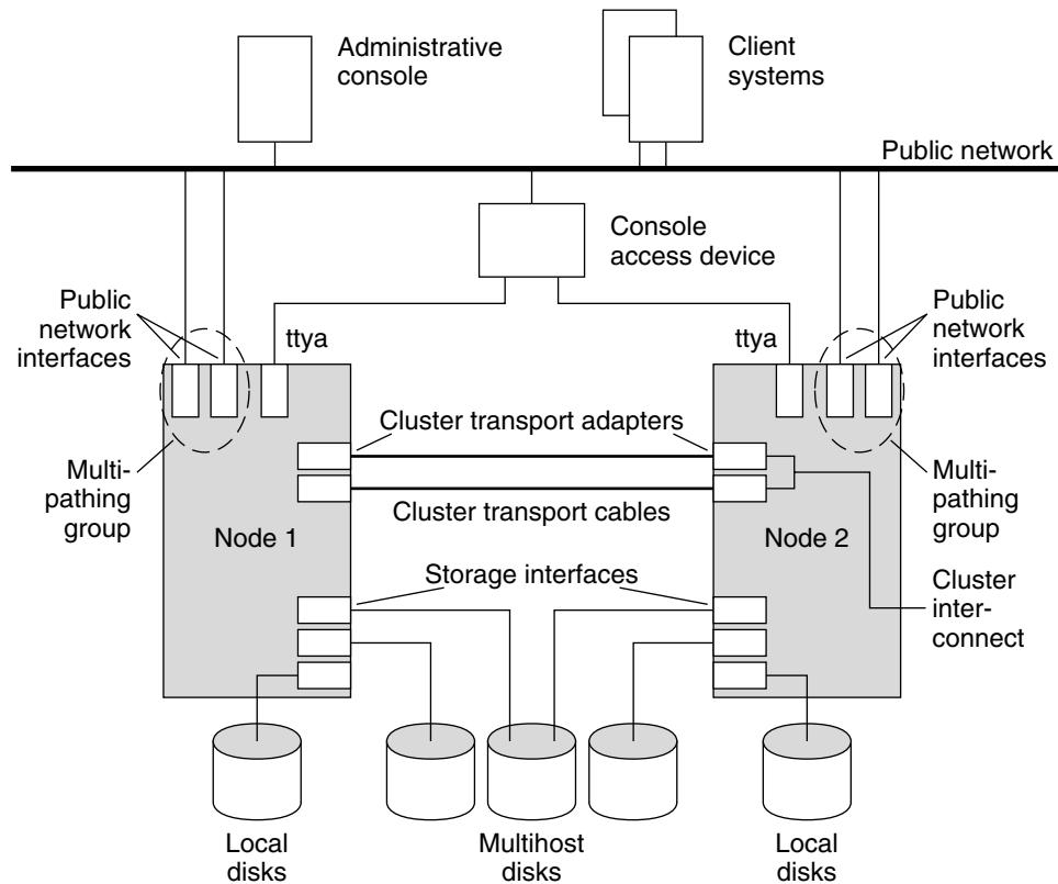
FIGURE 2-1 Sample Two-Node Cluster Configuration
