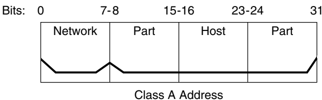
FIGURE 5-4 Byte Assignment in a Class A Address
