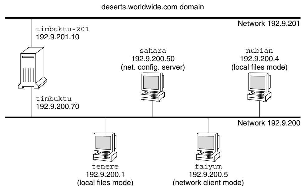
FIGURE 4-1 Hosts in a Sample Network
