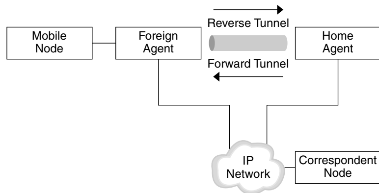
FIGURE 23-4 Mobile IP With a Reverse Tunnel
