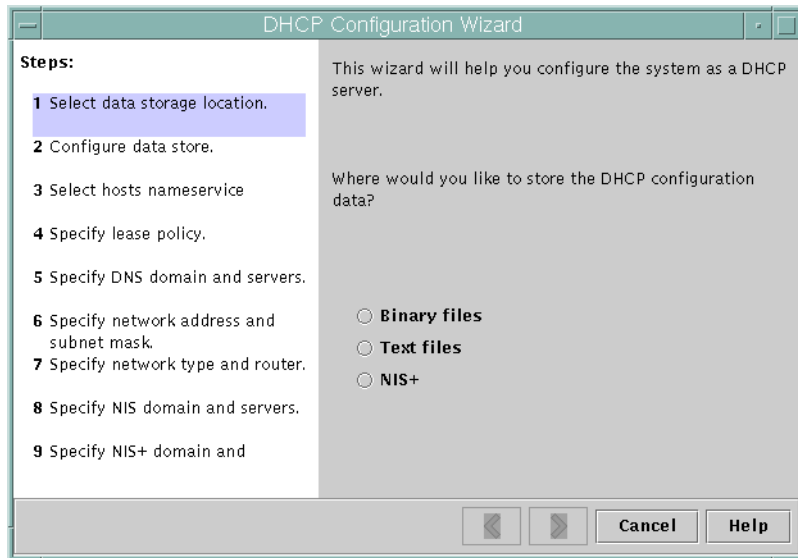
FIGURE 9-2 DHCP Configuration Wizard's Initial Screen
