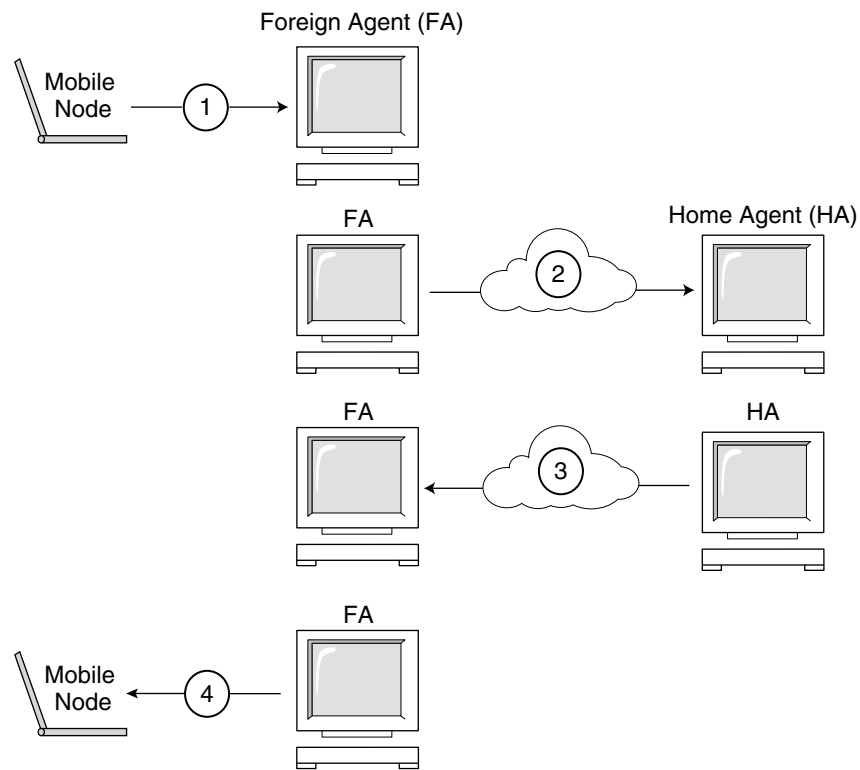
FIGURE 23-7 Mobile IP Registration Process
