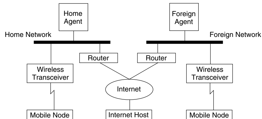
FIGURE 23-1 Mobile IP Topology
