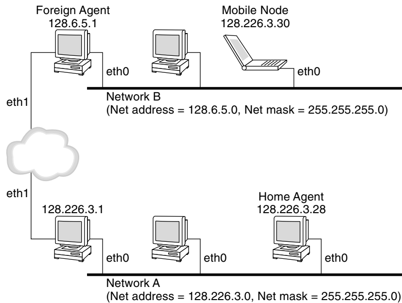
FIGURE 23-3 Mobile Node Moving to a Foreign Network
