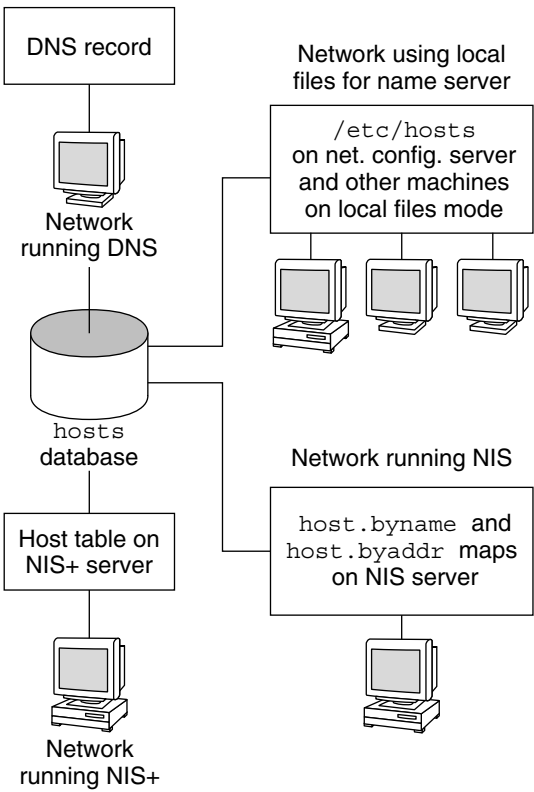
FIGURE 5-2 Forms of the hosts Database Used by Name Services
