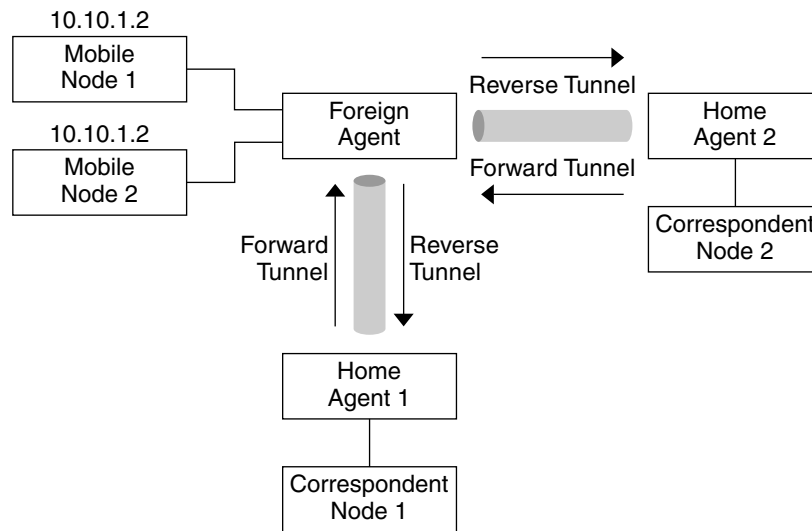
FIGURE 23-6 Privately Addressed Mobile Nodes Residing on Different Foreign Networks
