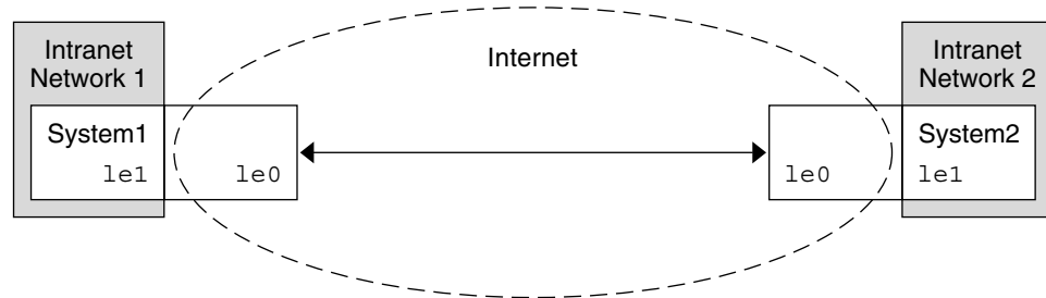
FIGURE 19-3 Virtual Private Network
