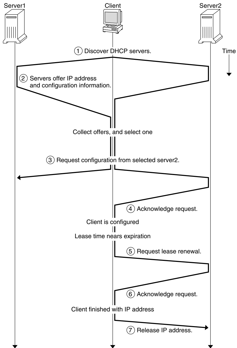
FIGURE 7-1 Sequence of Events for DHCP Service
