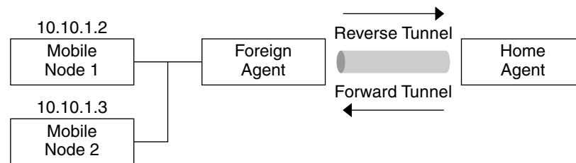
FIGURE 23–5 Privately Addressed Mobile Nodes Residing on the Same Foreign Network
