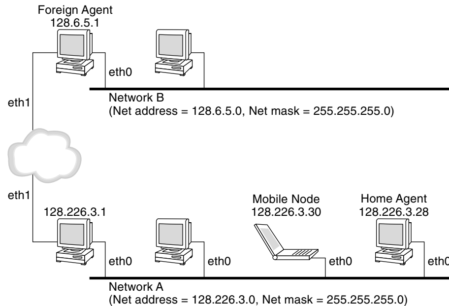
FIGURE 23-2 Mobile Node Residing on Home Network
