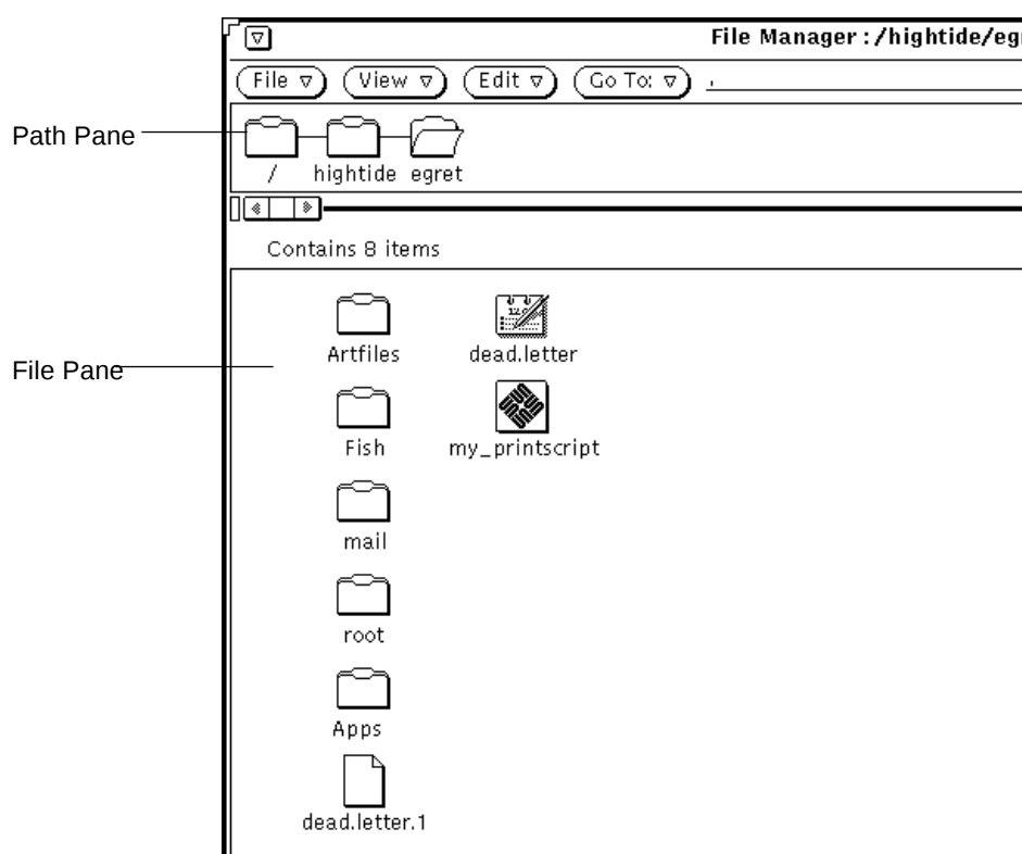
Figure 2-14 Icons in the File Pane
