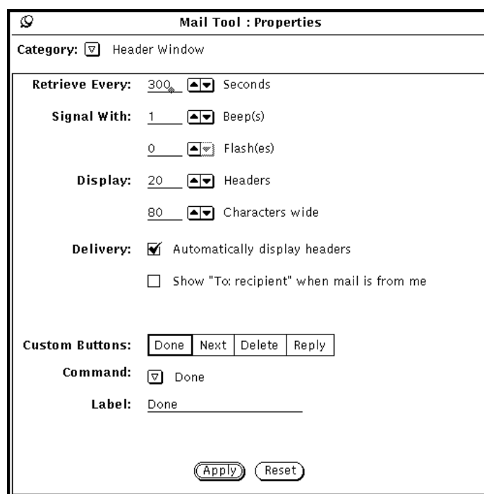
Figure 4-31 Header Window Properties
