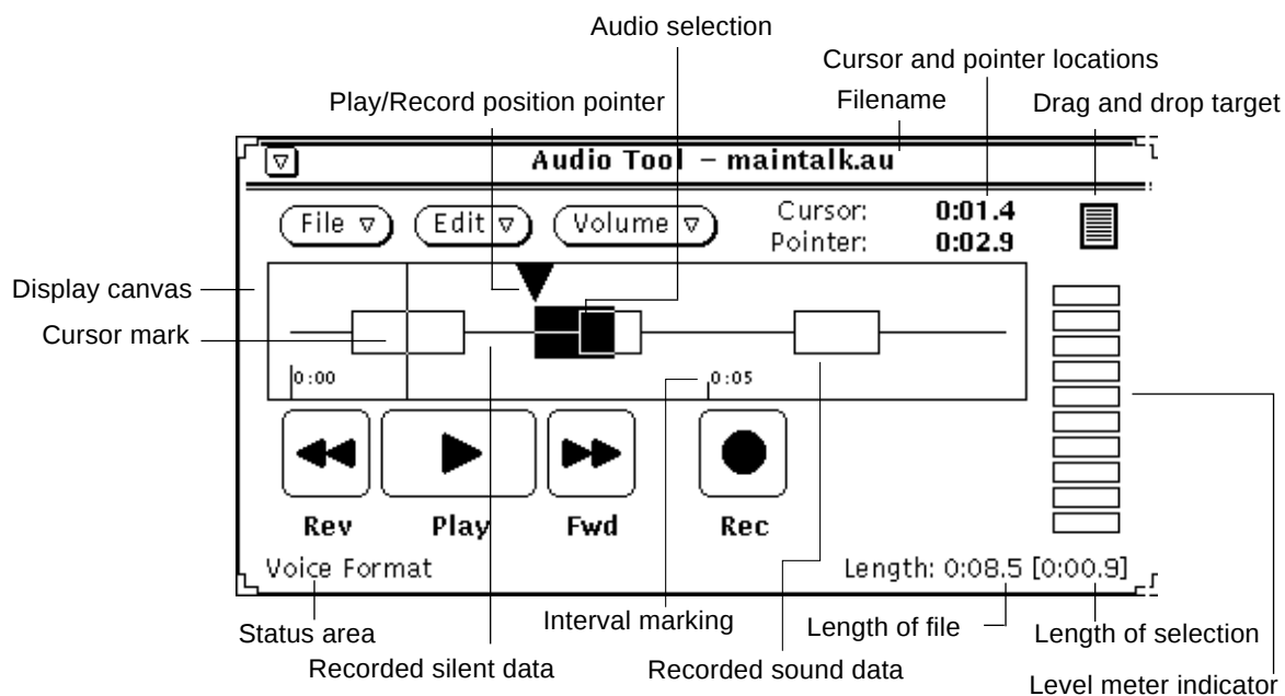
Figure 11-11 Audio Tool Base Window
