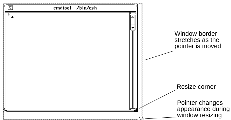
Figure 1-27 Stretching a Window by its Resize Corner
