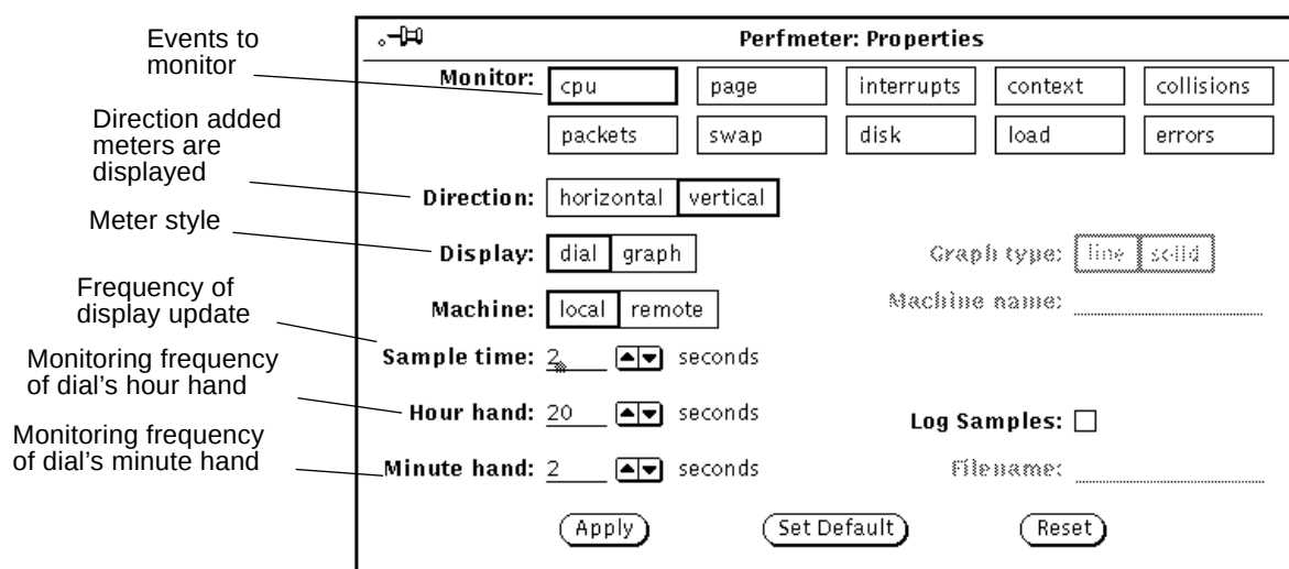
Figure 9-6 The Performance Meter Properties Window
