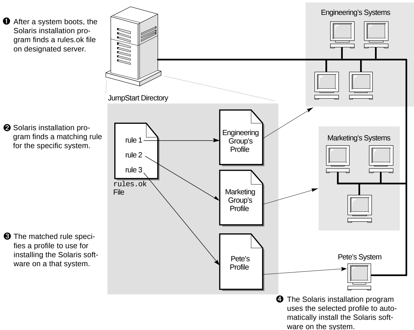
Figure 4-3 How a Custom JumpStart Installation Works: Networked Example
