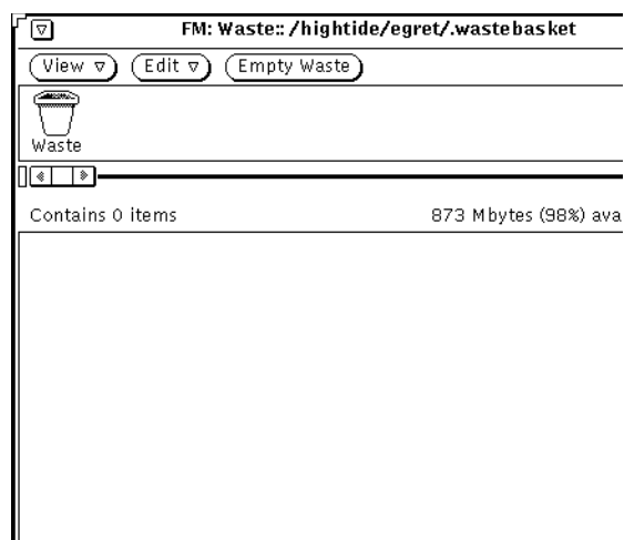
Figure 2-28 Wastebasket Window
