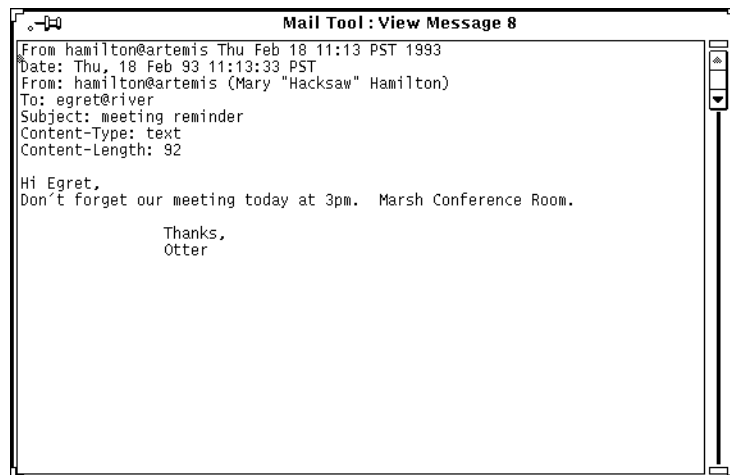
Figure 4-8 Header window
