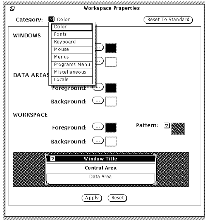
Figure 17-2 Category Menu
