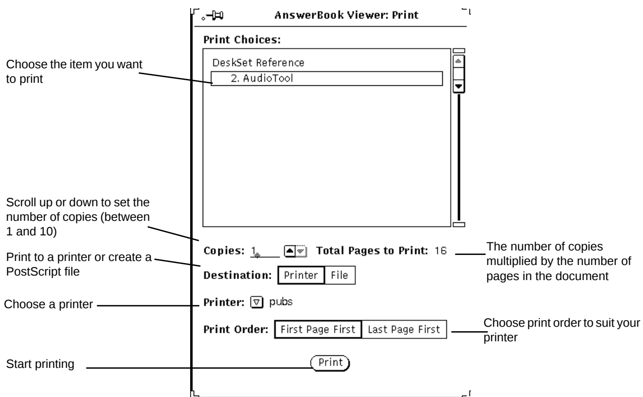
Figure 19-22 Print Window
