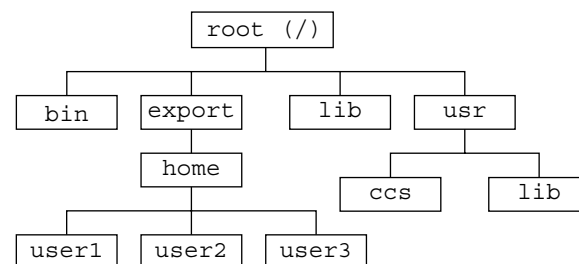
FIGURE 3–1 File System Hierarchy
