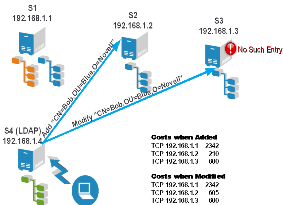
Figure 19-4 ARC Deployment Considerations
