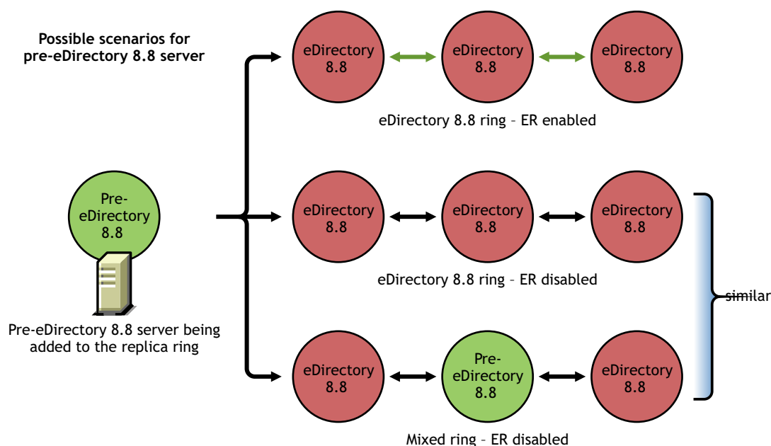
Figure 11-5 Possible Scenarios for Pre-eDirectory 8.8 Server
