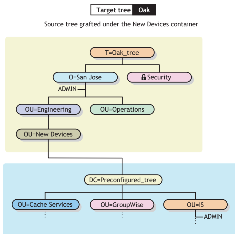
Figure 10-4 Grafted eDirectory Tree
