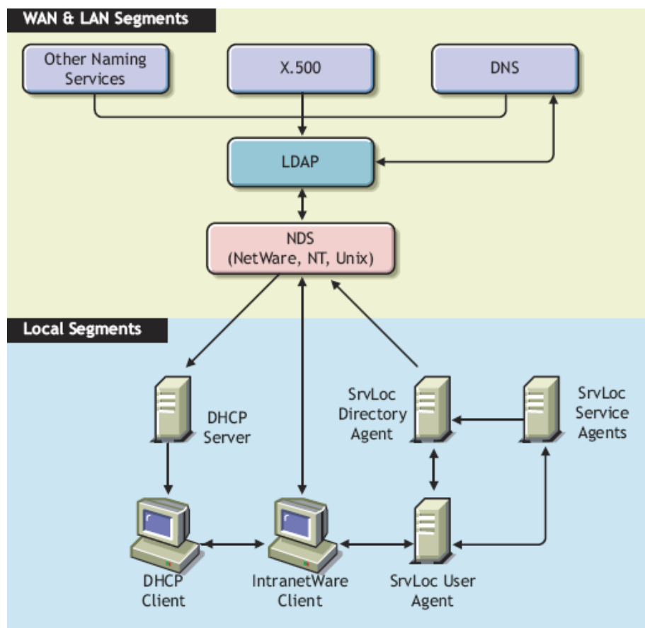
Figure 16-3 Integrated Network Services Discovery
