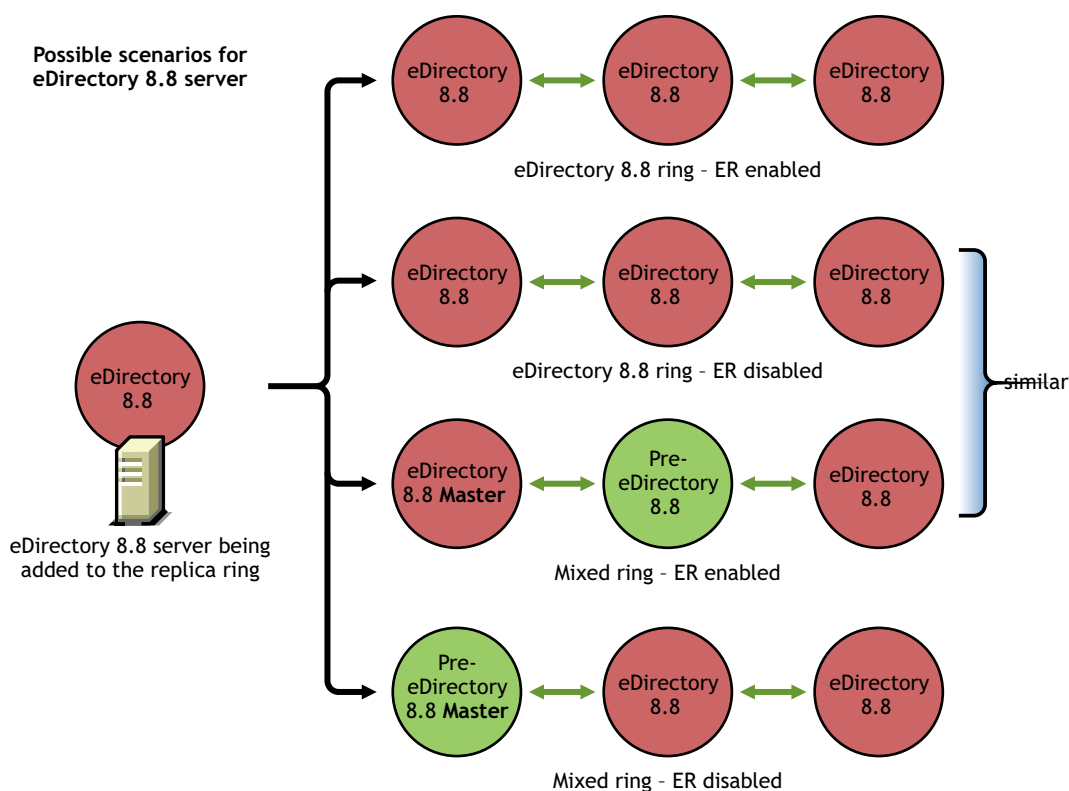
Figure 11-8 Possible Scenarios for eDirectory 8.8 Server
