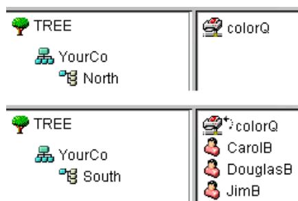
Figure 1-7 Alias Object in eDirectory Container
