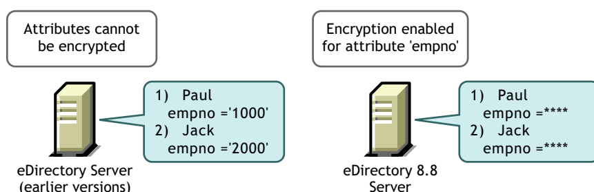
Figure 11-1 Encrypted Attributes
