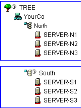
Figure 1-17 Sample Partitions
