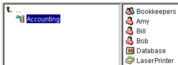
Figure 1-3 Container Object
