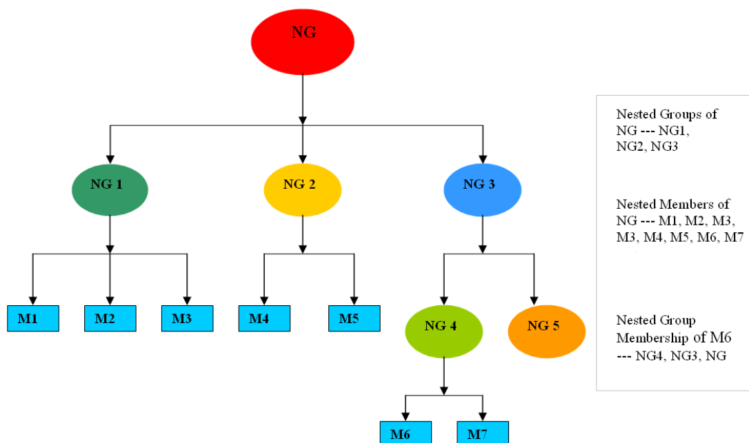
Figure 1-5 Nested Groups
