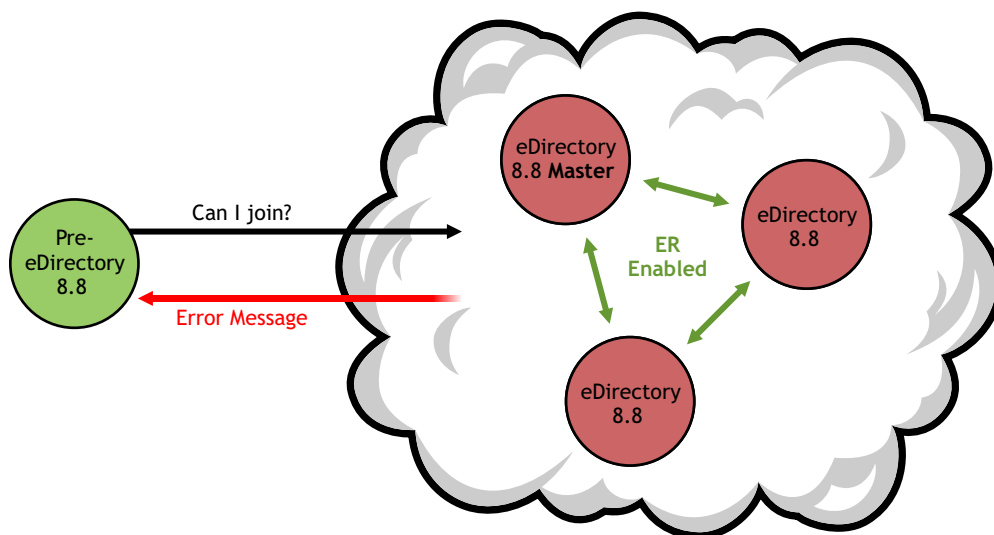
Figure 11-6 Adding Pre-eDirectory 8.8 Server to eDirectory 8.8 Replica Ring with Encrypted Replication Enabled.
