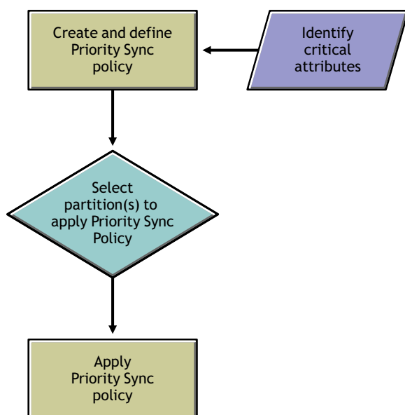
Figure 3-5 Priority Sync process
