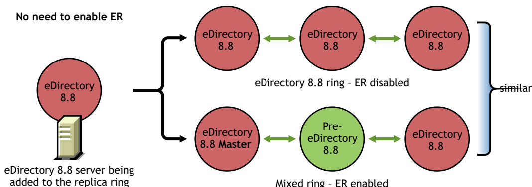
Figure 11-10 Adding eDirectory 8.8 Server to Replica Rings where Encrypted Replication is Disabled.
