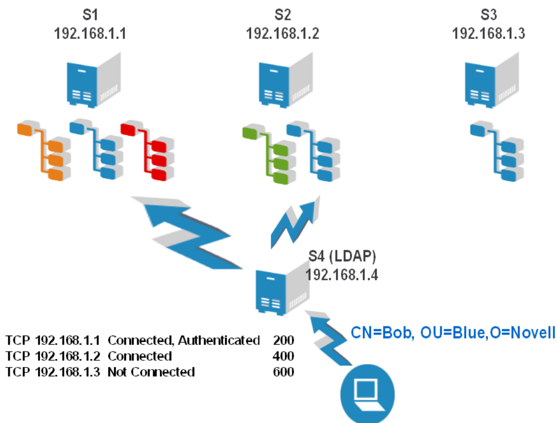
Figure 19-2 One Stop Server Effect
