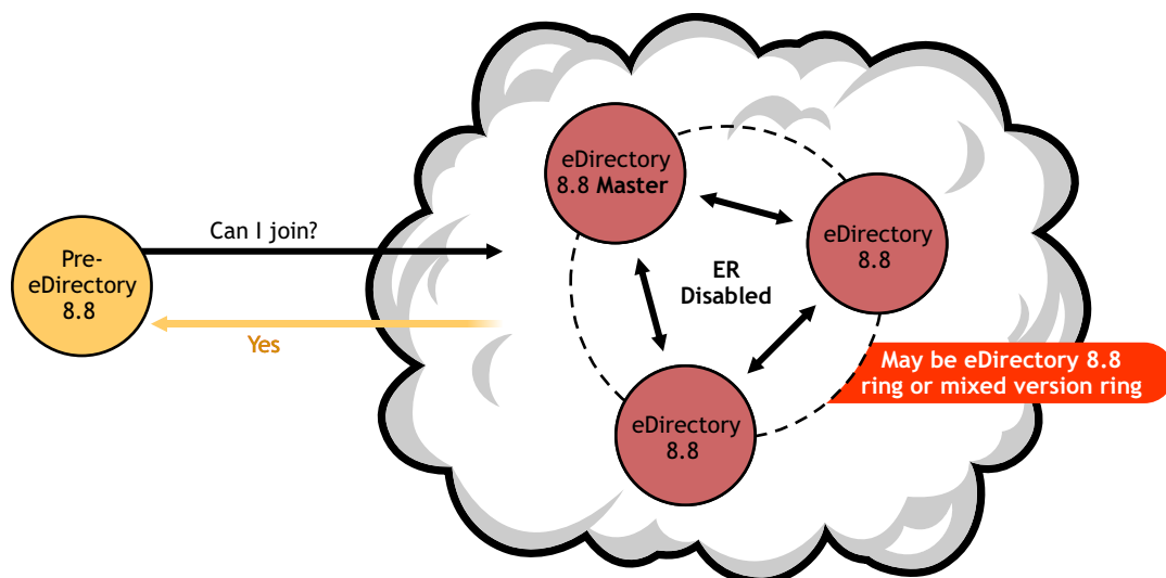
Figure 11-7 Adding Pre-eDirectory 8.8 Server to Replica Ring with Encrypted Replication Disabled
