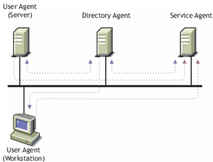
Figure 16-2 SLP Directory Agent Interaction
