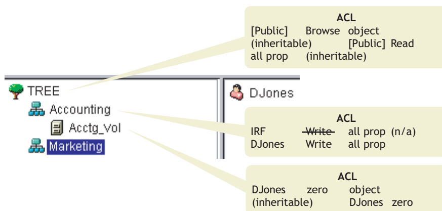
Figure 1-21 Sample Trustee Rights
