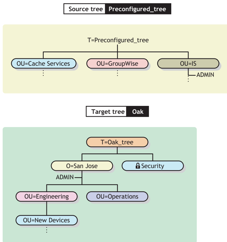
Figure 10-3 eDirectory Trees before a Graft
