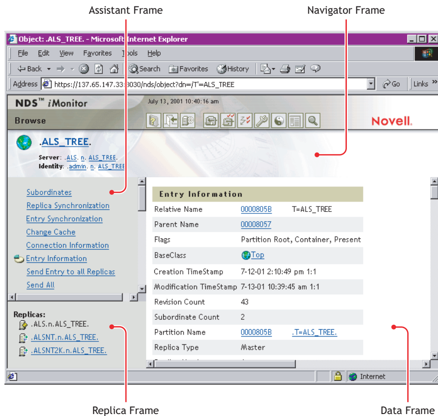
Figure 8-1 iMonitor Frames
