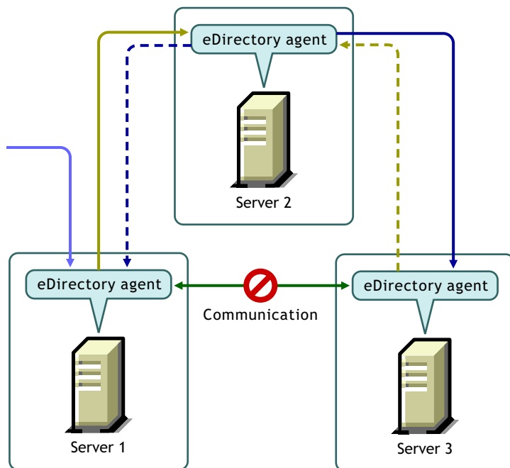
Figure 3-3 Transitive Synchronization
