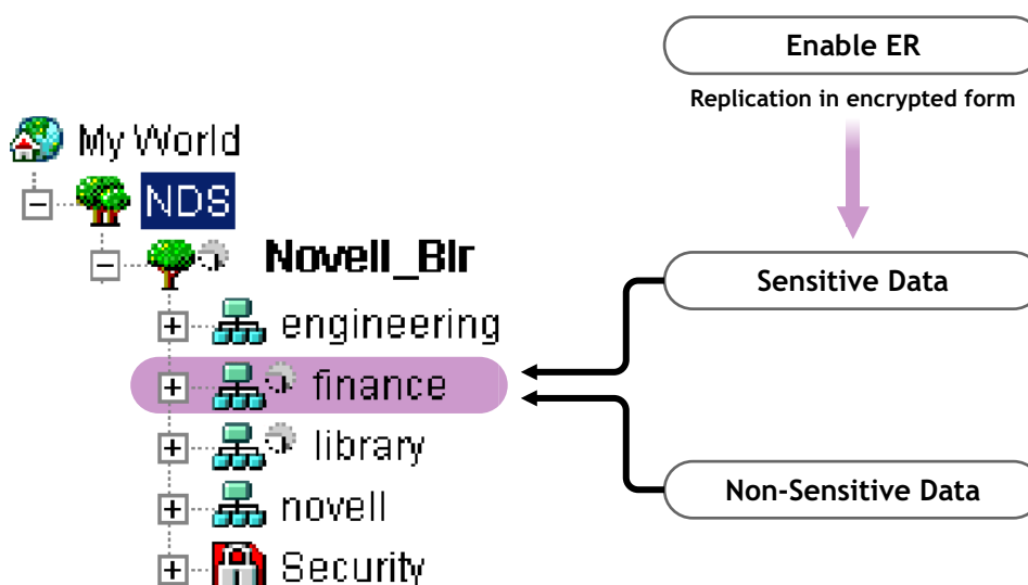
Figure 11-3 Encrypted Replication
