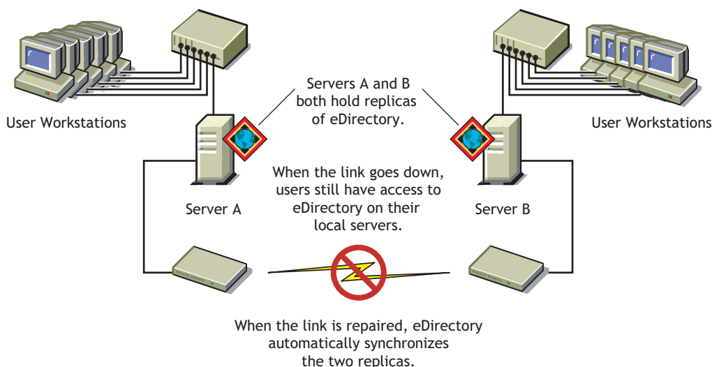
Figure 1-19 eDirectory Replicas
