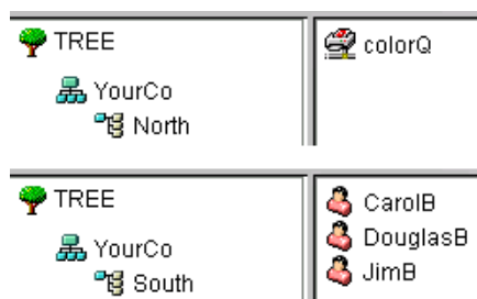
Figure 1-6 Sample Containers
