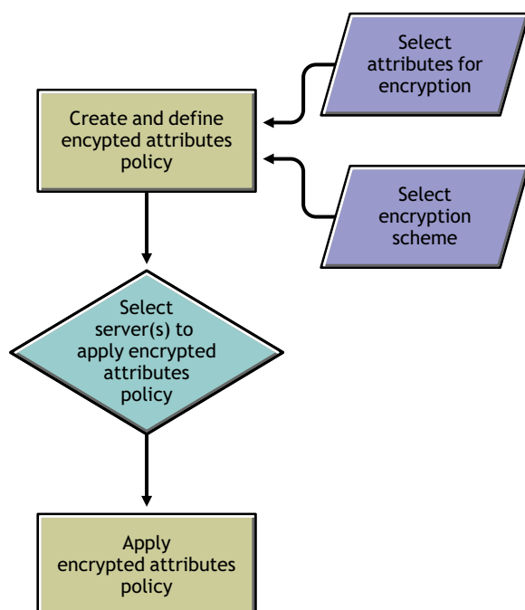
Figure 11-2 Encrypting Attributes
