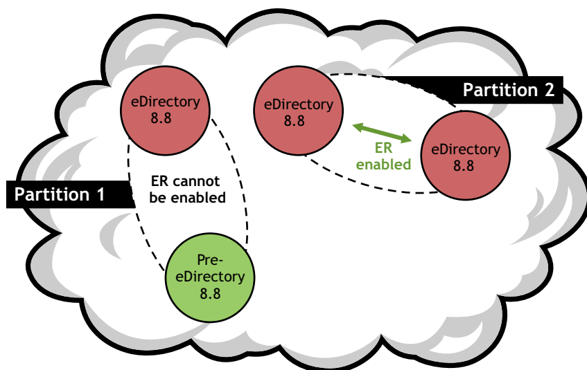
Figure 11-4 Encrypted Replication at Partition Level
