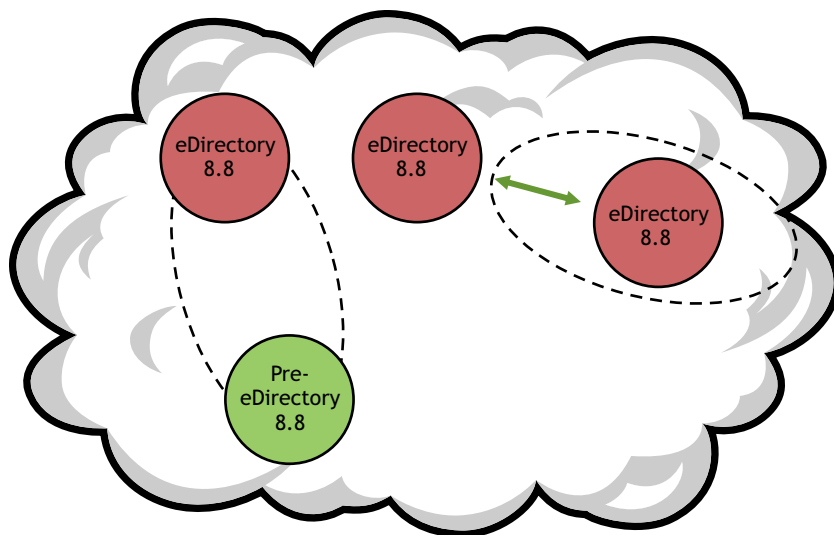
Figure 11-9 Adding eDirectory 8.8 Server to eDirectory Replica Ring with Encrypted Replication Enabled
