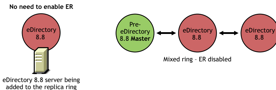
Figure 11-11 Adding eDirectory 8.8 server to a Replica Ring where Master Replica is a Pre-eDirectory 8.8 Server
