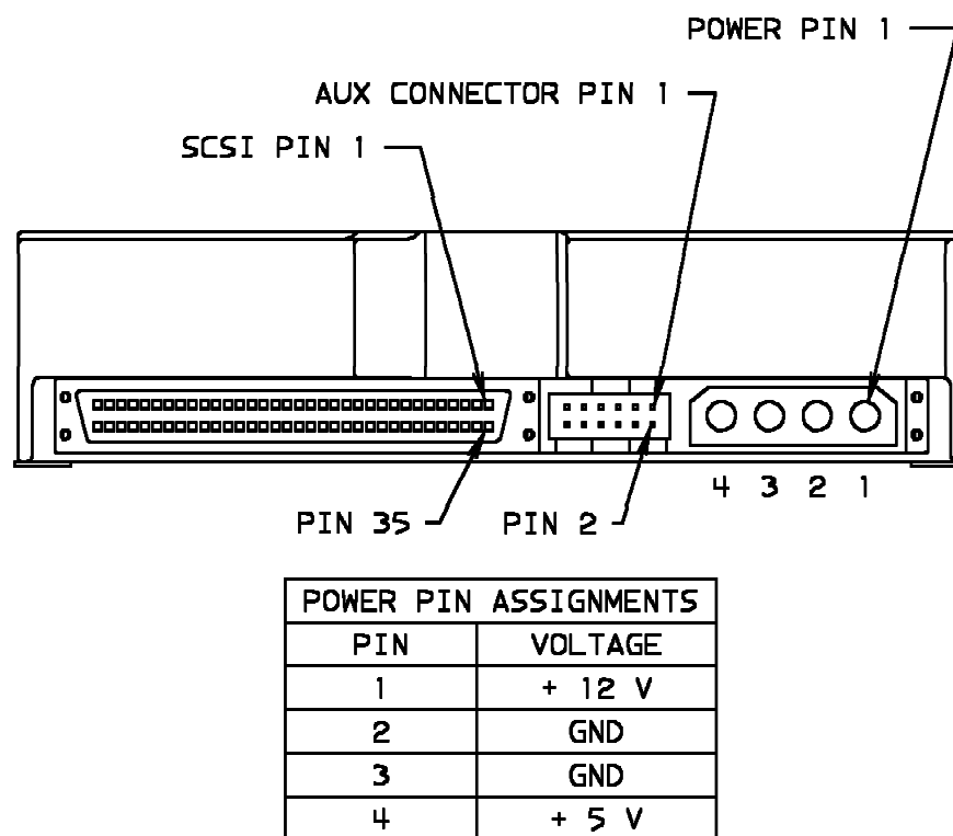
Figure 27. Electrical connectors (rear view) -- 68 pin models.
