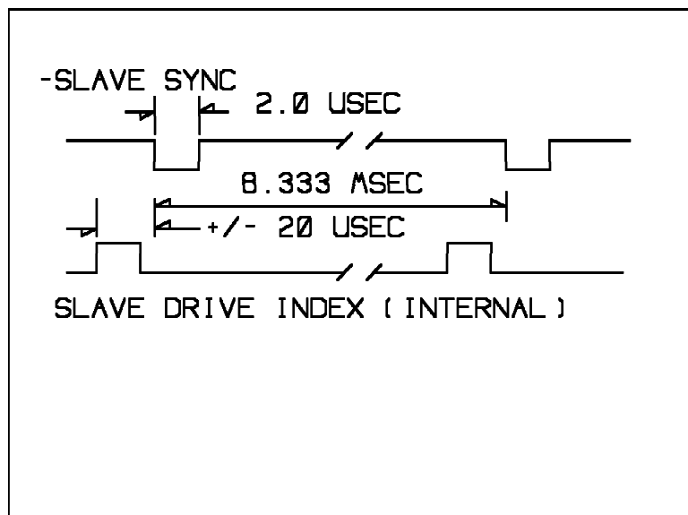
Figure 37. Slave-Sync to Slave-Index Timing
