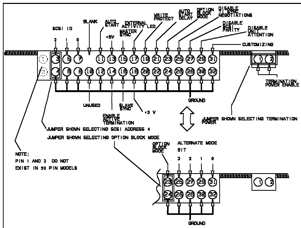
Figure 30. 50 pin Single Ended Front Option Jumper Block (& TermPower Block)
