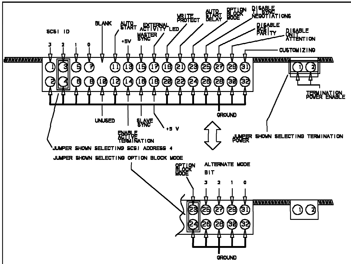
Figure 31. 68 pin Single Ended Front Option Jumper Block (& TermPower Block)
