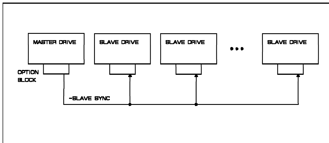
Figure 38. Daisy-Chain Connection of Synchronization Bus
