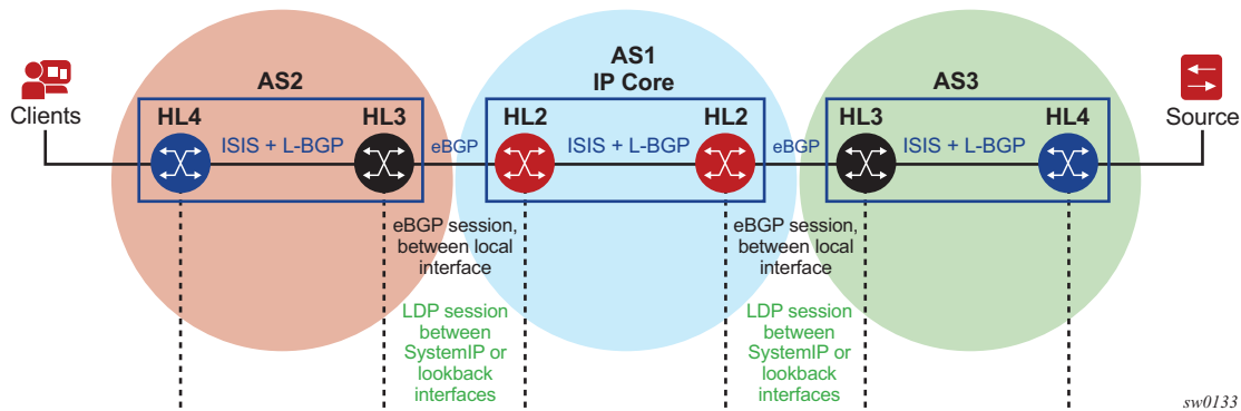
Figure 81 ASBR and eBGP
