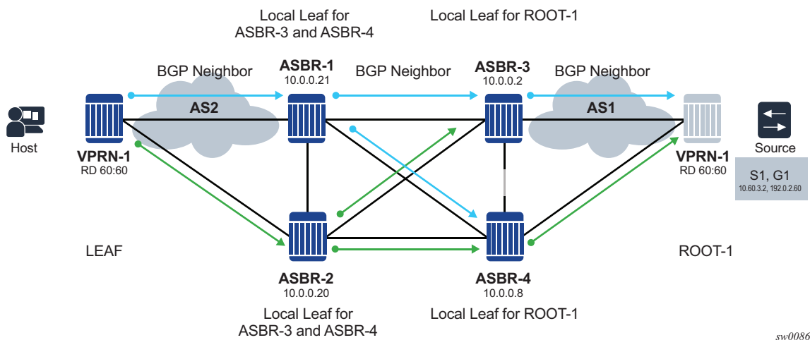
Figure 89 ASBR Node Acting as Local Leaf
