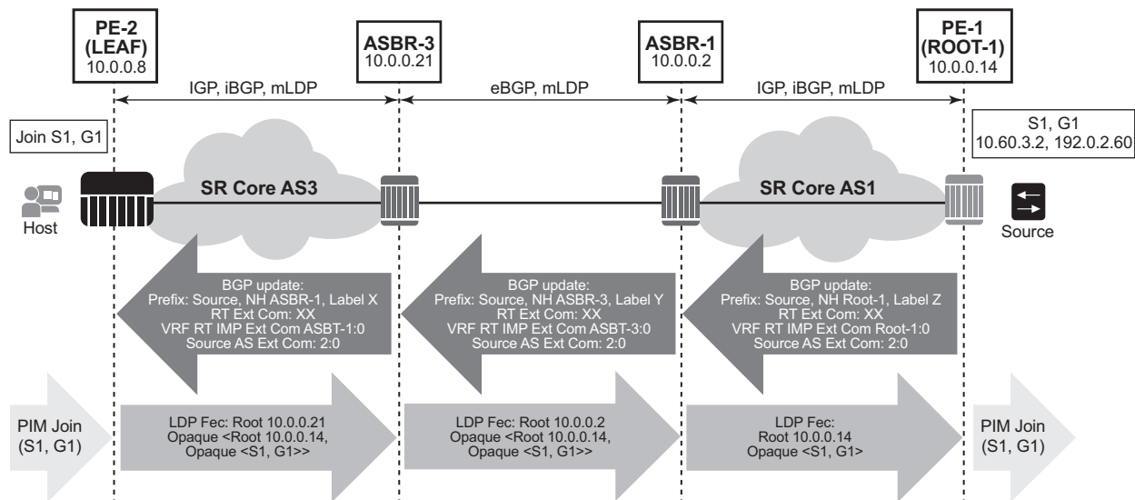
Figure 77 Non-VPN mLDP with Recursive Opaque for Inter-AS
