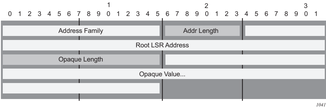
Figure 83 ECHO Request Target FEC Stack TLV
