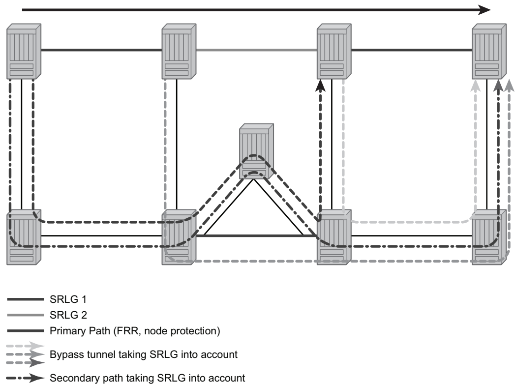
Figure 30 Shared Risk Link Groups
