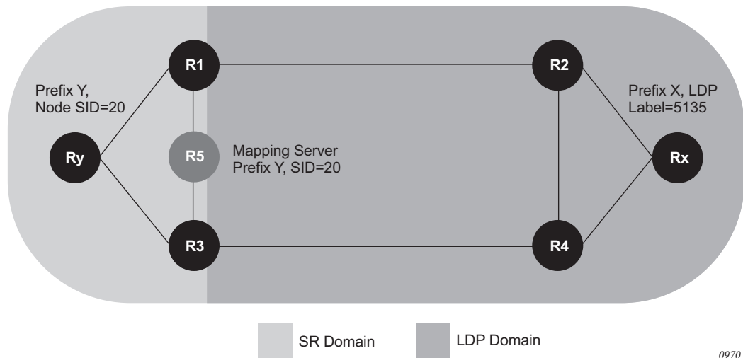
Figure 72 Stitching in the LDP-to-SR Direction
