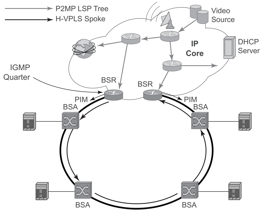
Figure 35 Application of P2MP LSP in Video Broadcast
