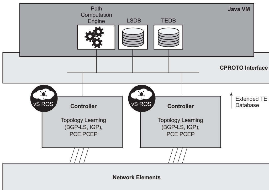
Figure 57 Packet Network Resource Controller (NRC-P) Architecture
