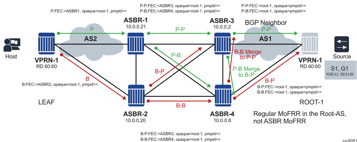
Figure 99 Resolution via ASBR-3
