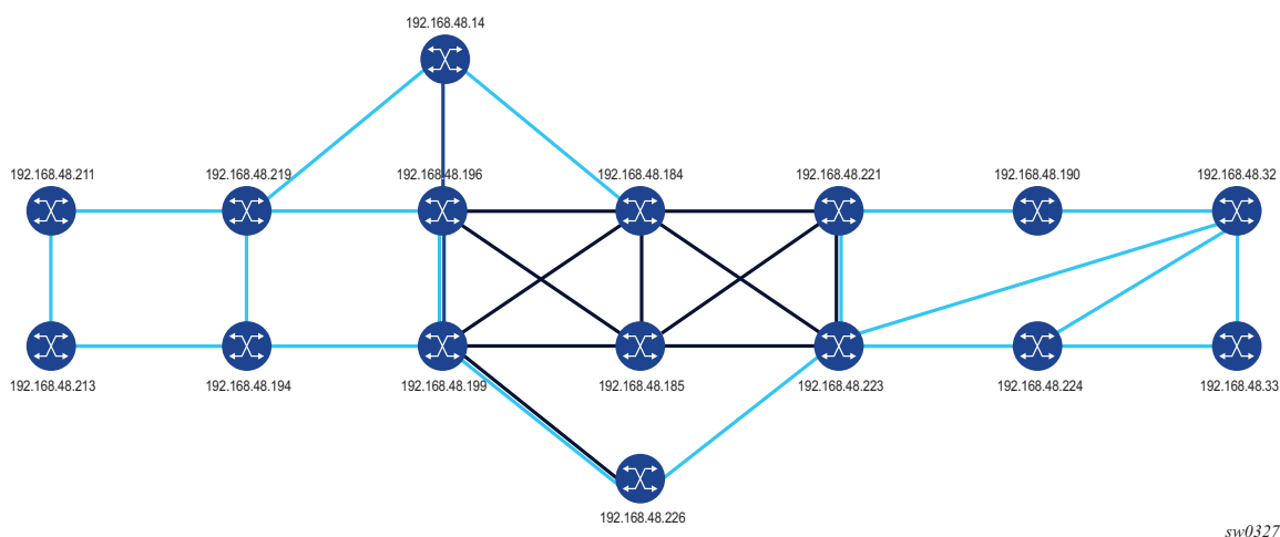
Figure 60 Multi-level IS-IS Topology in the NSP GUI
