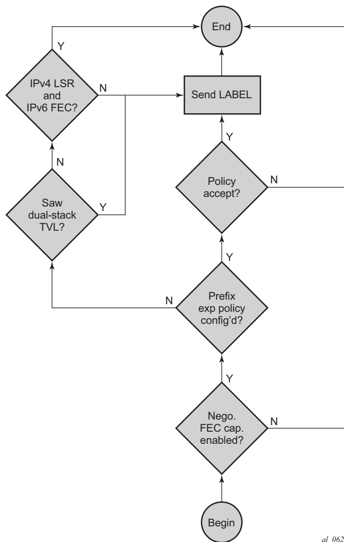
Figure 104 LDP IPv6 Address and FEC Distribution Procedure
