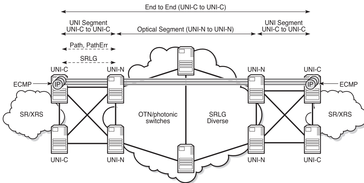
Figure 45 End-to-End ECMP with gLSP Diversity Across Single UNI-C
