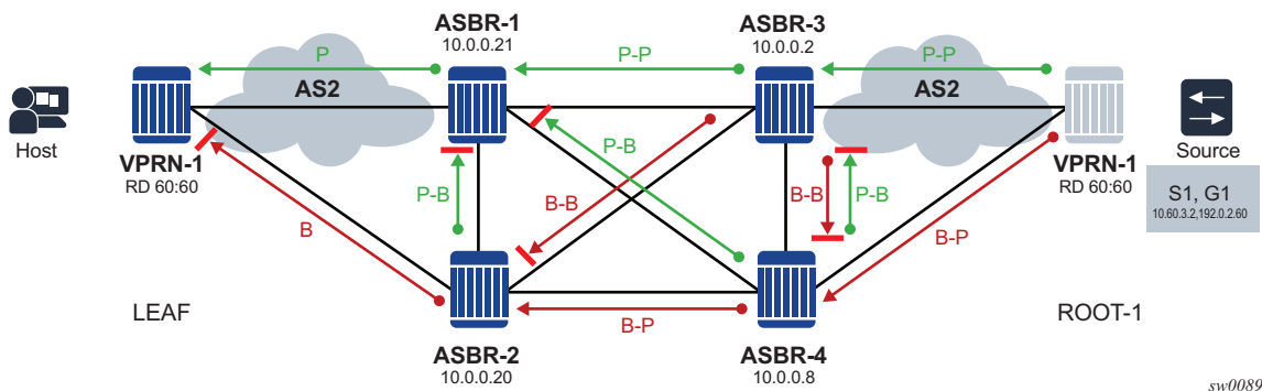
Figure 96 Traffic Flow
