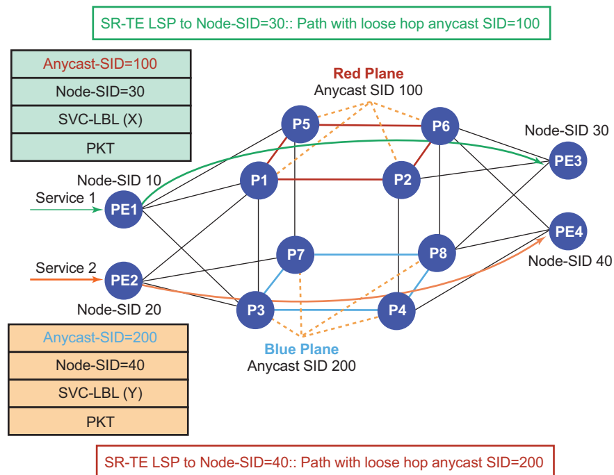
Figure 36 Multi-plane TE with Node Protection
