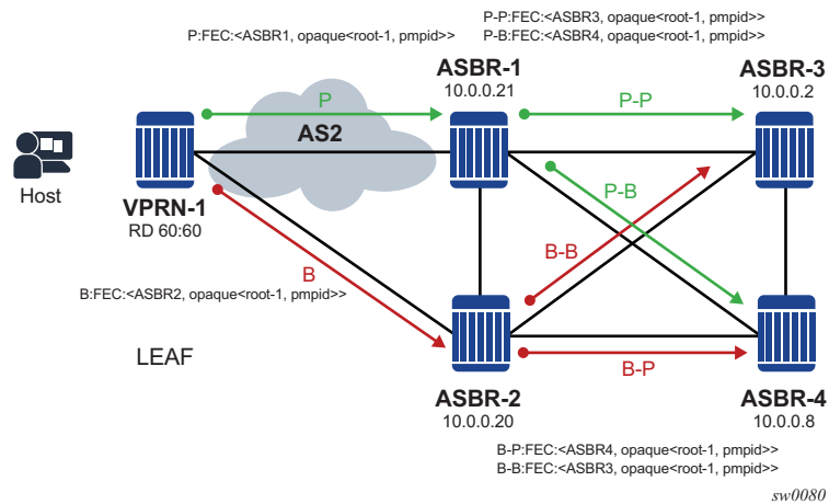
Figure 94 ASBR MoFRR ASBR Behavior
