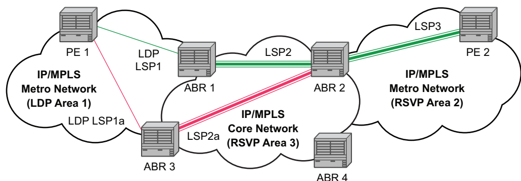
Figure 67 LDP over RSVP Application Variant
