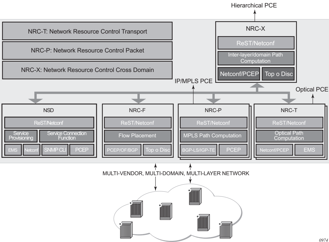
Figure 56 NSP Functional Modules
