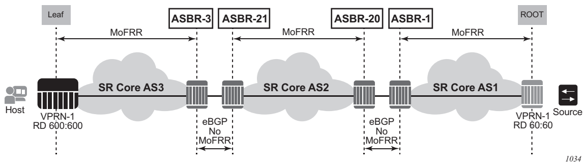
Figure 82 ASBRs Using eBGP Without IGP
