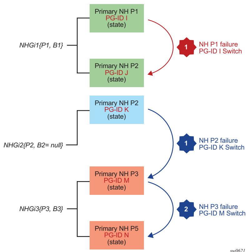
Figure 53 NHG Failover Based on PG-ID Switch
