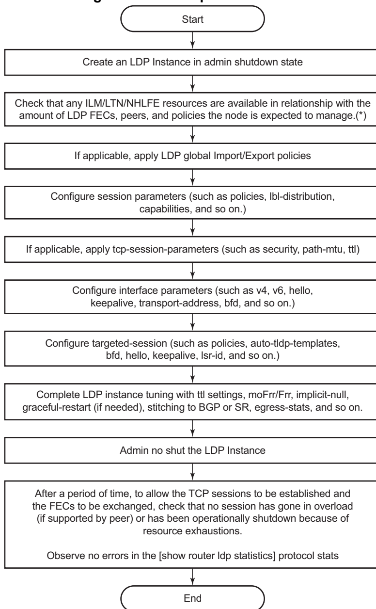
Figure 108 LDP Configuration and Implementation
