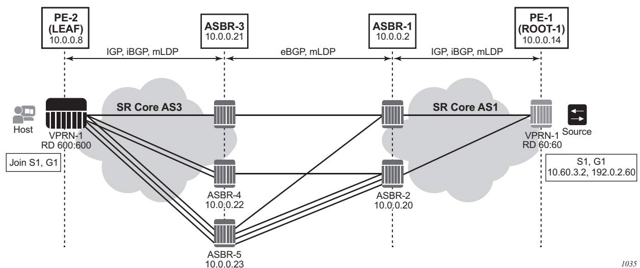
Figure 85 ECMP Support
