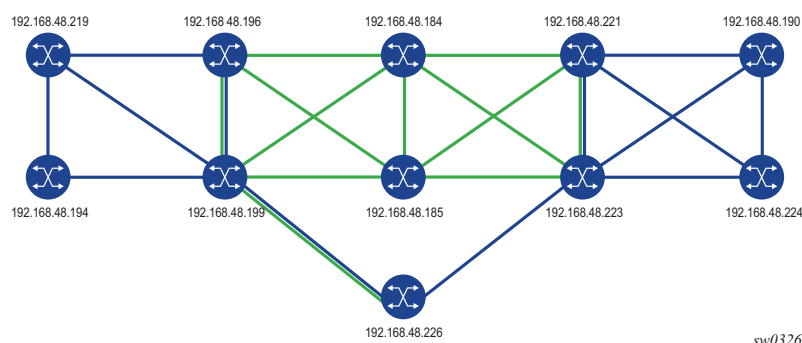
Figure 39 Multi-level IS-IS Topology in the NSP GUI
