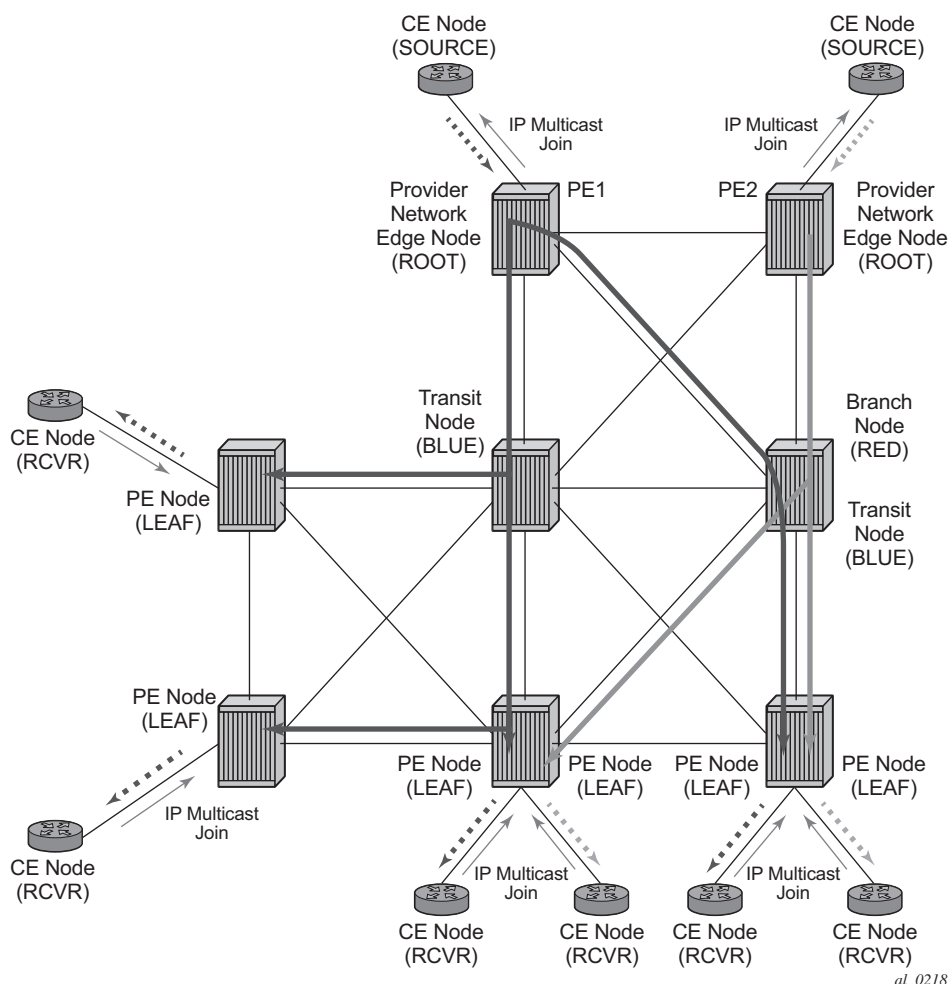
Figure 73 Video Distribution using P2MP LDP
