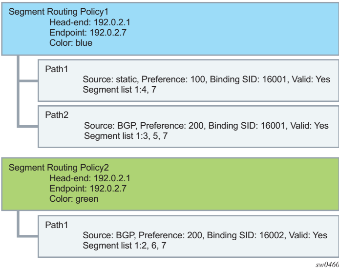
Figure 63 Relationship Between Segment Routing Policies and Paths
