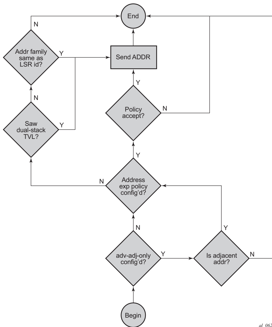
Figure 105 LDP IPv6 Address and FEC Distribution Procedure
