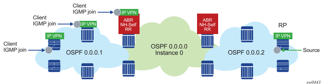
Figure 87 Intra-AS Non-segmented Topology
