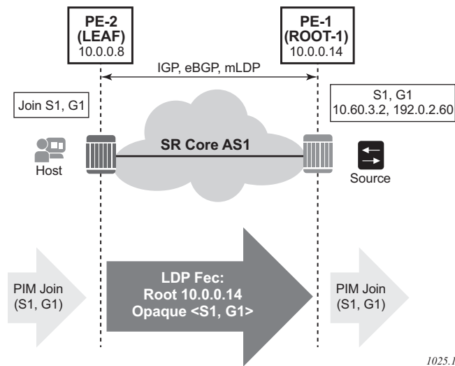
Figure 75 mLDP FEC for Single AS with Transit IPv4 Opaque
