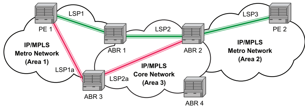
Figure 66 LDP over RSVP Application
