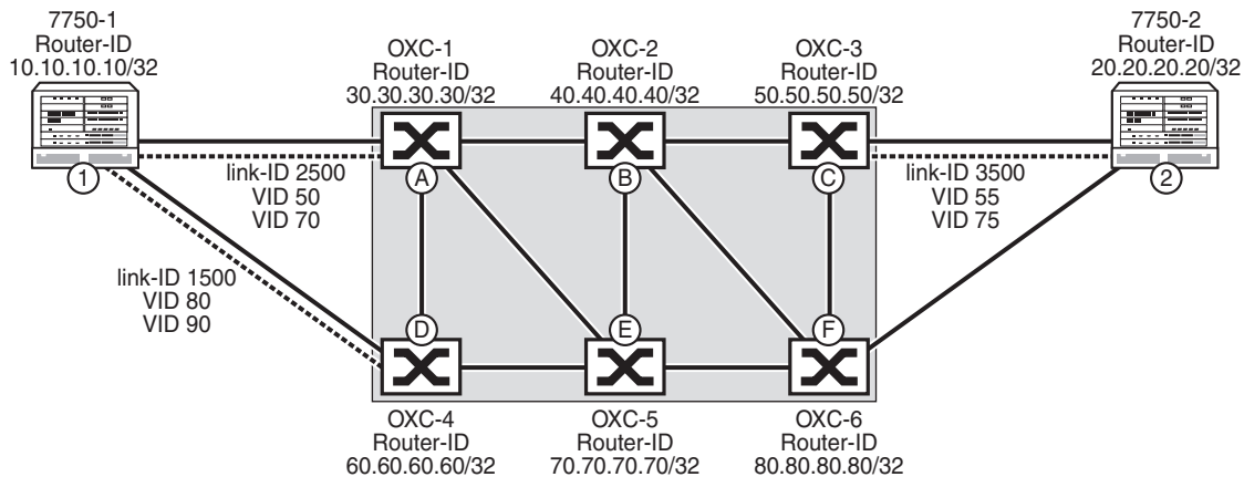
Figure 52 SRLG Example
