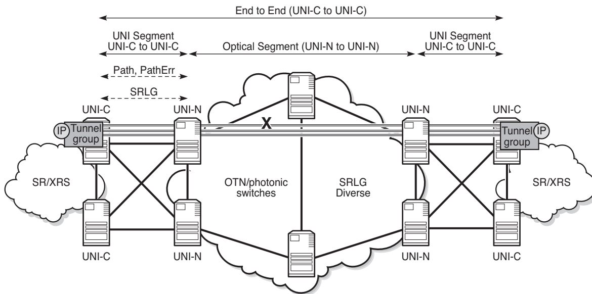
Figure 47 gLSP Re-Establishment (PATH Refresh)
