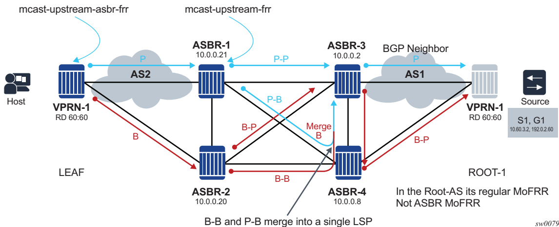
Figure 92 ASBR MoFRR and IGP MoFRR
