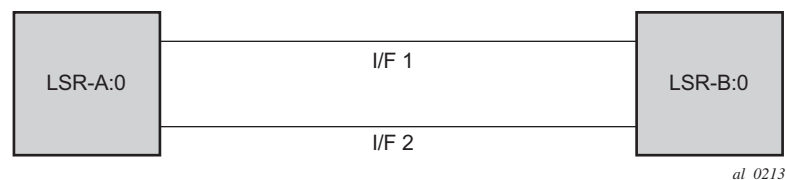
Figure 65 LDP Adjacency and Session over Unnumbered Interface
