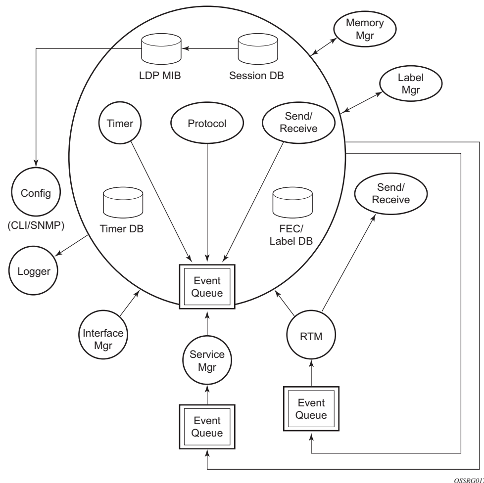
Figure 64 Subsystem Interrelationships
