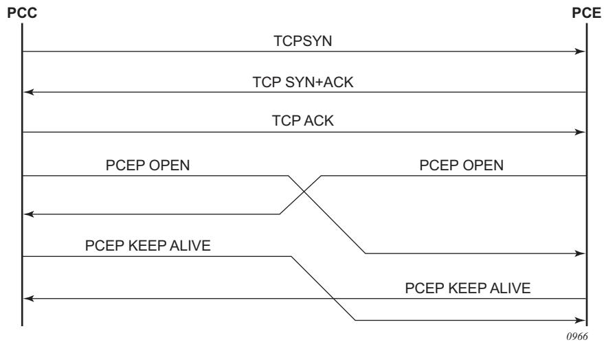
Figure 58 PCEP Session Initialization
