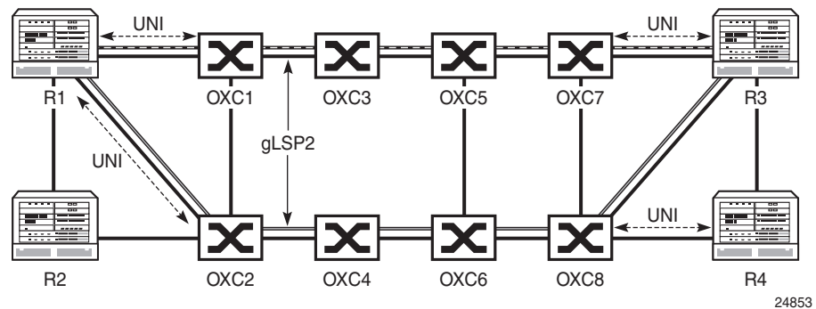
Figure 41 Multi-Layer Resiliency
