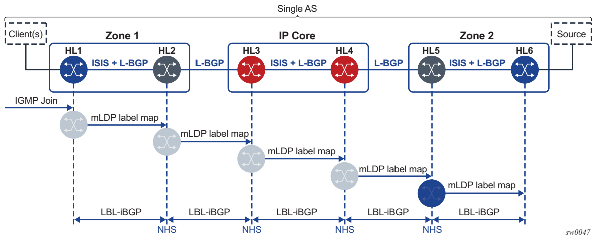
Figure 79 Example AS
