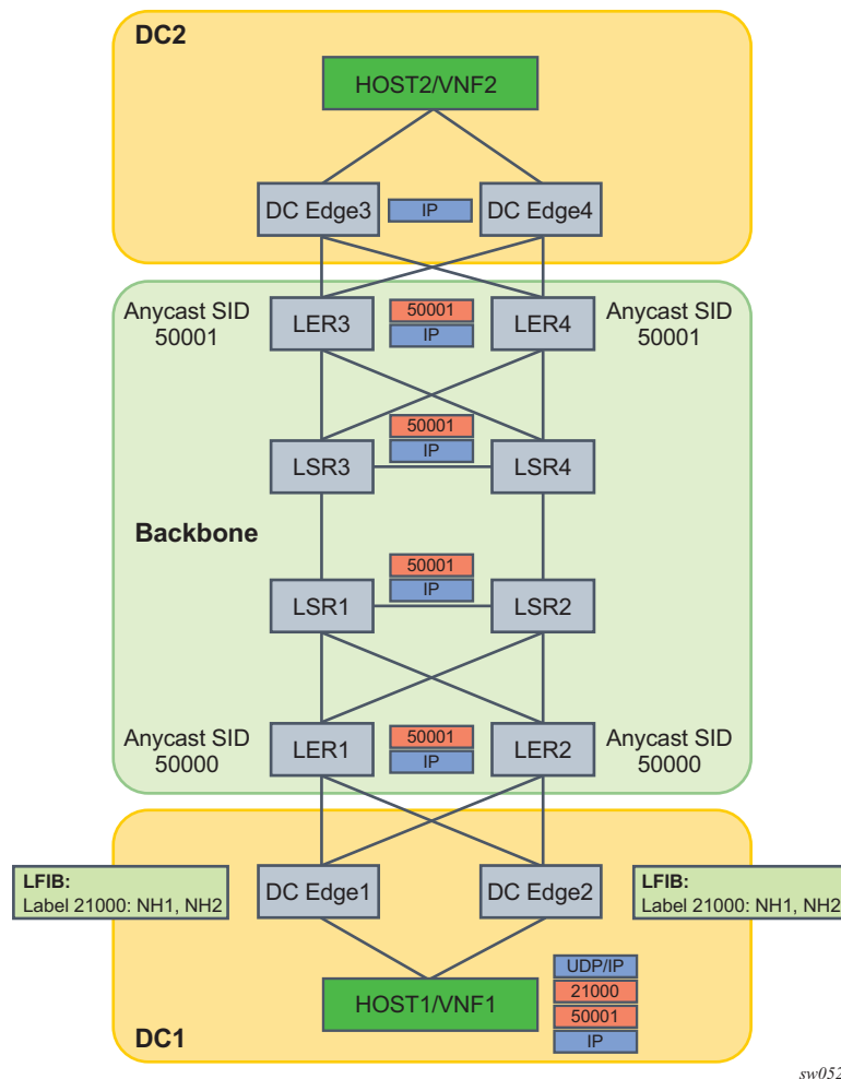
Figure 54 Traffic Steering to an Indirect Next-hop using a Static Label Route
