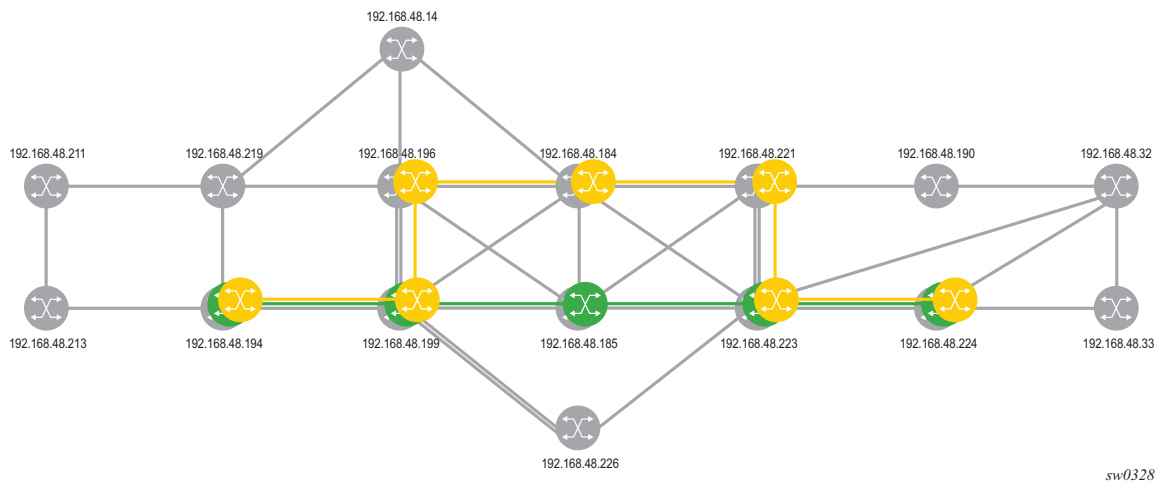
Figure 61 Primary and Secondary RSVP-TE LSP Paths in the NSP GUI
