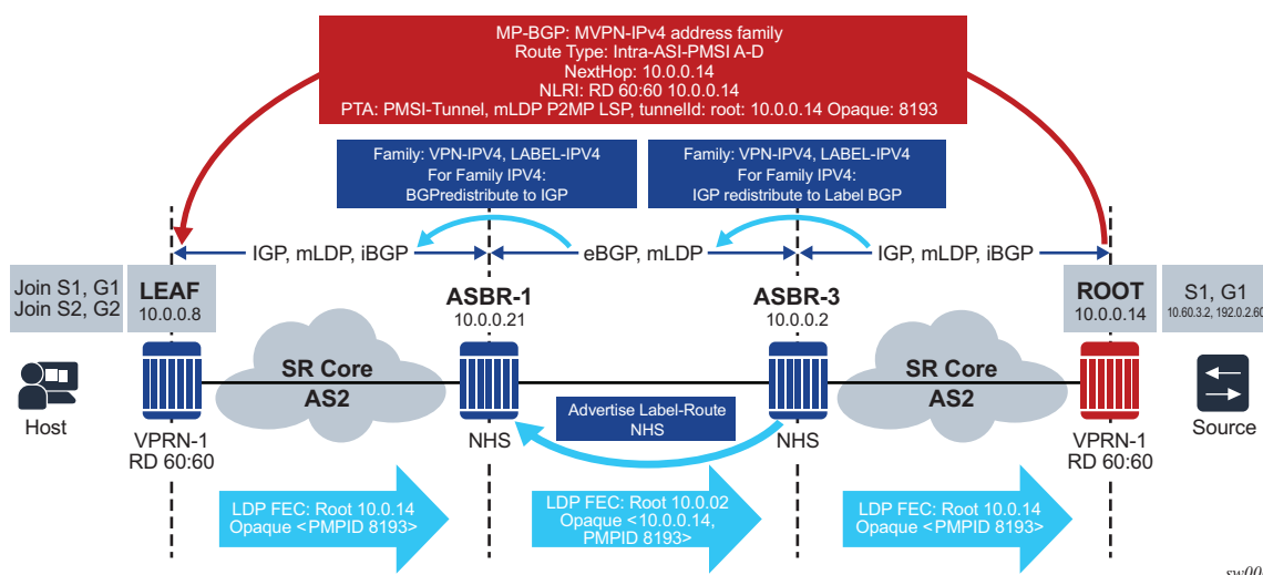
Figure 78 Optimized Option C — Leaf Router Not Responsible for Recursive FEC
