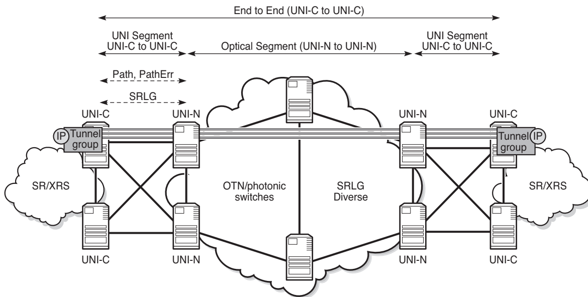
Figure 46 End-to-End Load Sharing GMPLS Tunnel Group with gLSP Path Diversity
