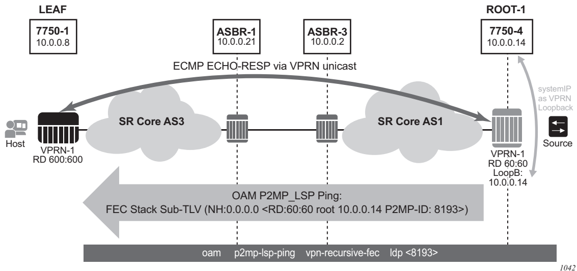
Figure 84 MVPN Inter-AS Option B OAM
