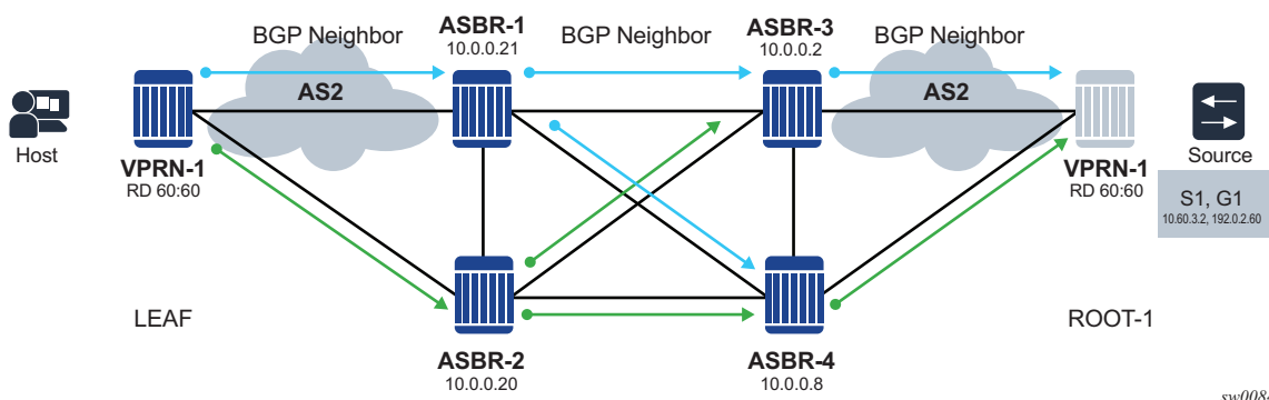
Figure 88 BGP Neighboring for MoFRR
