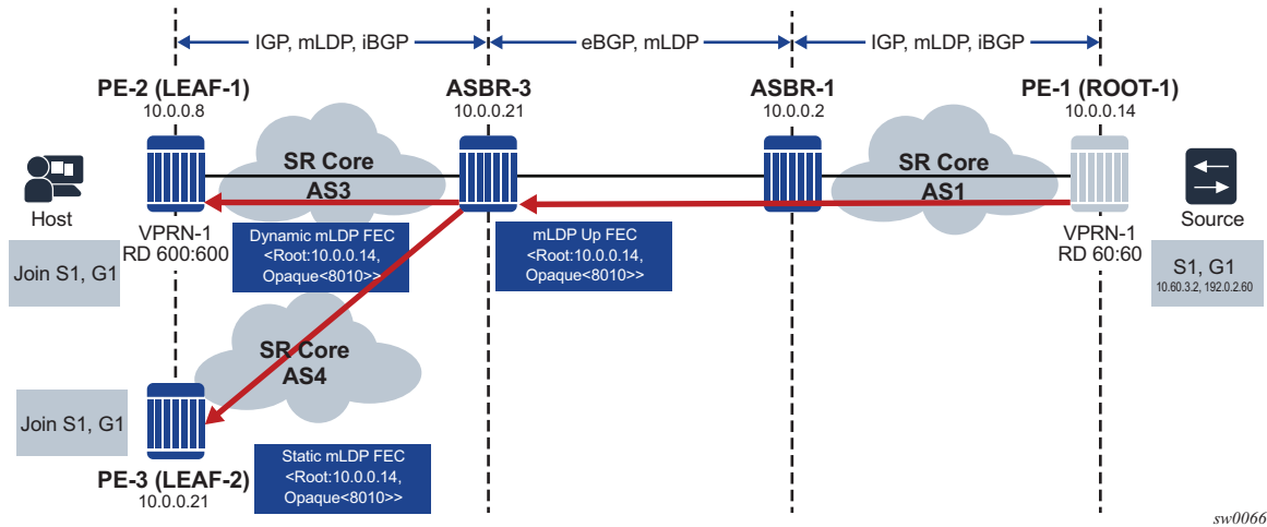
Figure 86 Static and Dynamic mLDP Interaction
