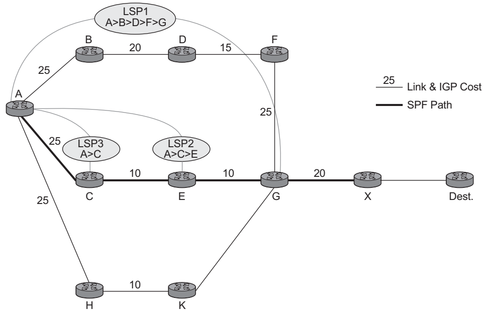
Figure 68 LDP over RSVP Without ABR Stitching Point
