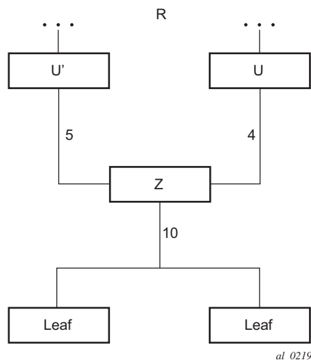
Figure 101 mLDP LSP with Backup Upstream LSR Nodes
