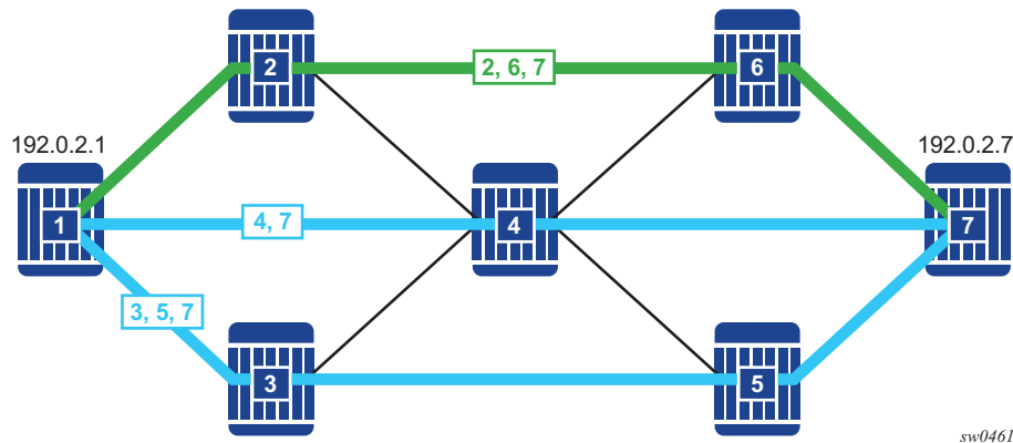
Figure 62 Network Example with 2 Segment Routing Policies
