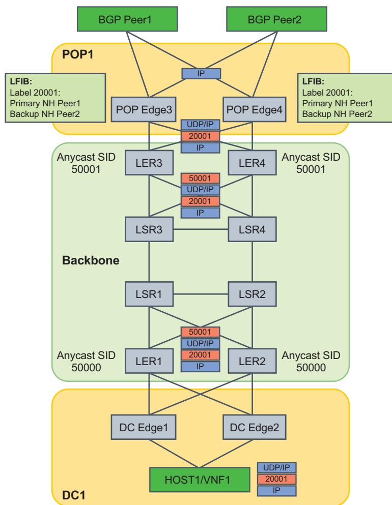
Figure 55 Traffic Steering to a Direct Next-hop using a Static Label Route
