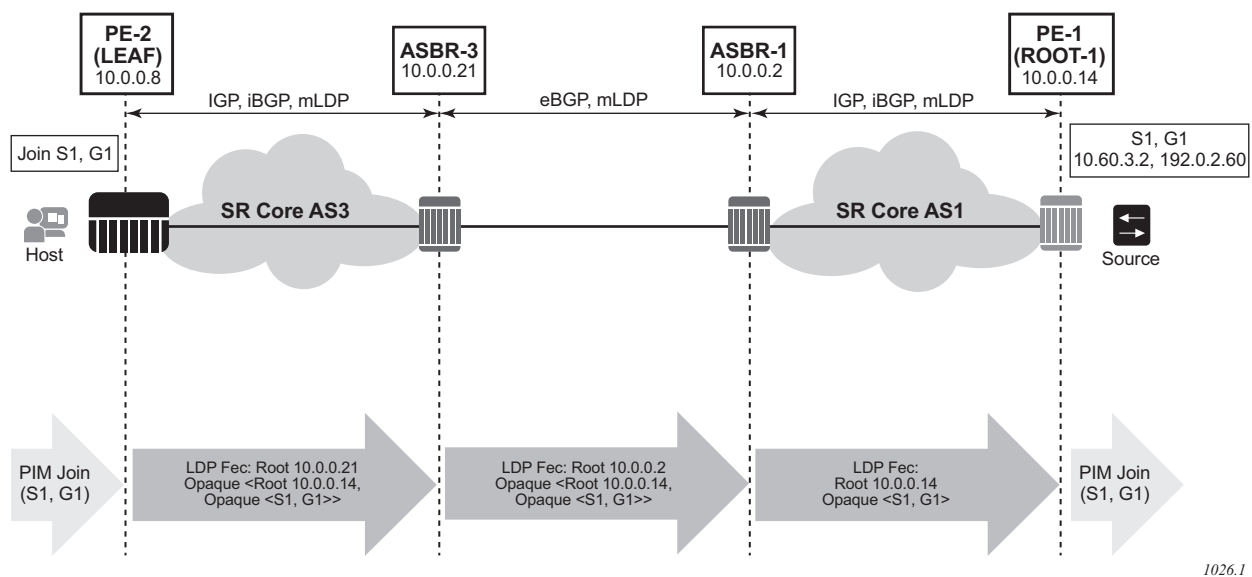
Figure 76 mLDP FEC for Inter-AS with Recursive Opaque Value
