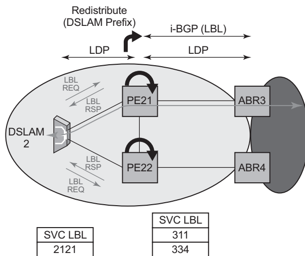
Figure 71 Application of LDP to BGP FEC Stitching
