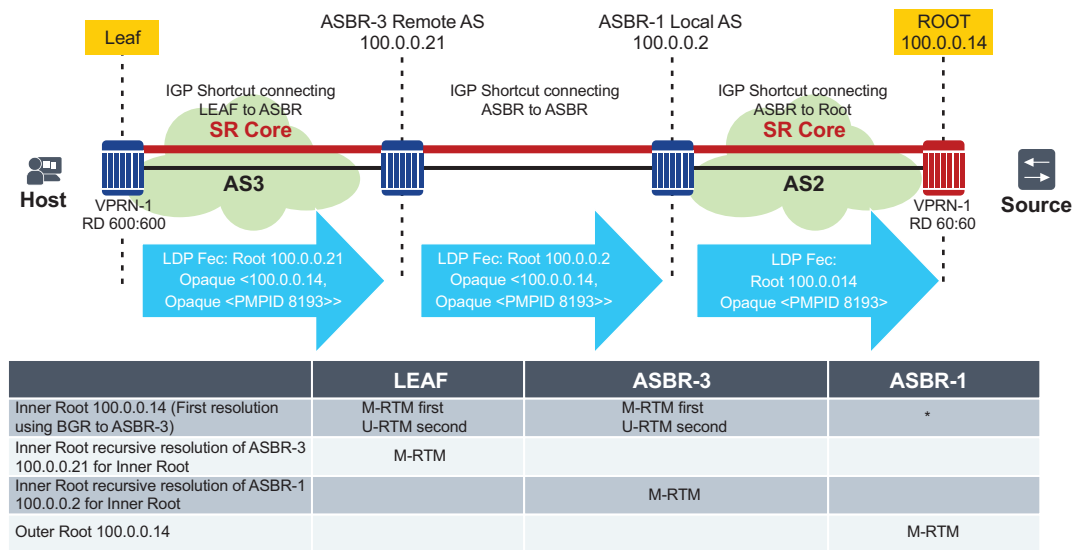
Figure 102 Recursive FEC Behavior
