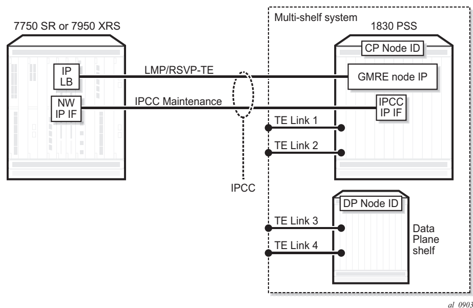
Figure 43 Identifier Architecture
