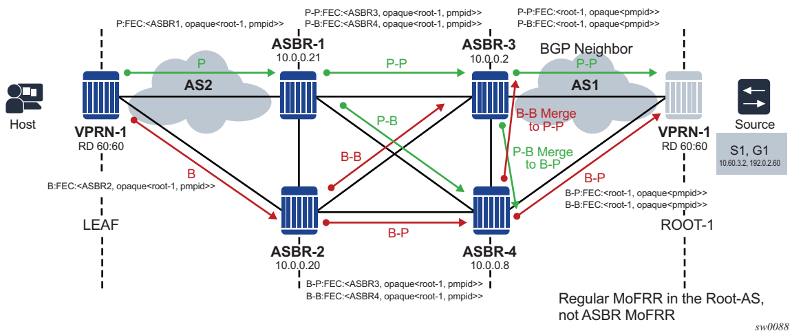
Figure 95 MoFRR Root AS Behavior
