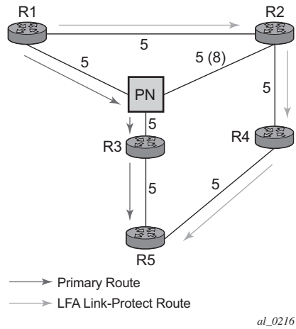
Figure 70 Example Topology with Broadcast Interfaces
