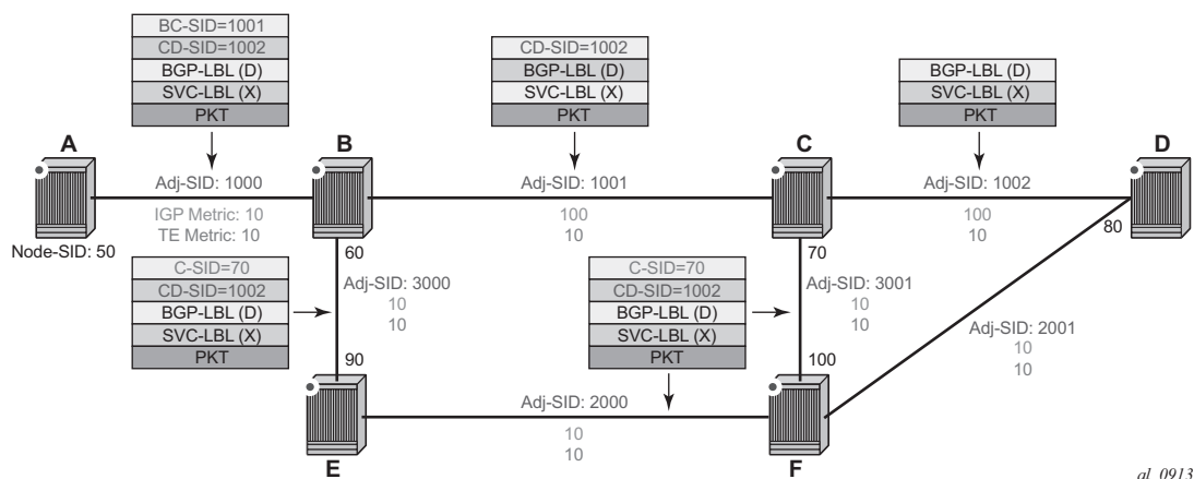
Figure 37 SR-TE LSP Label Stack Programming
