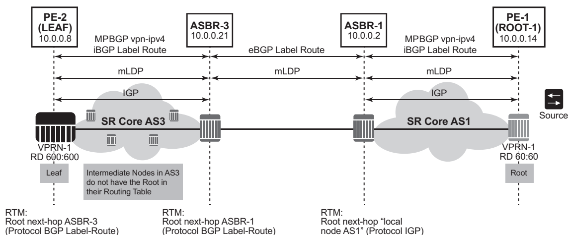
Figure 74 Inter-AS Option C
