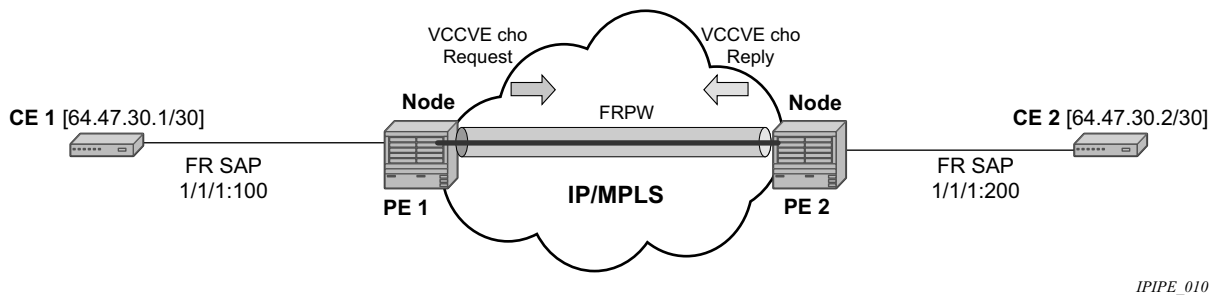
Figure 25 VCCV-Ping Application
