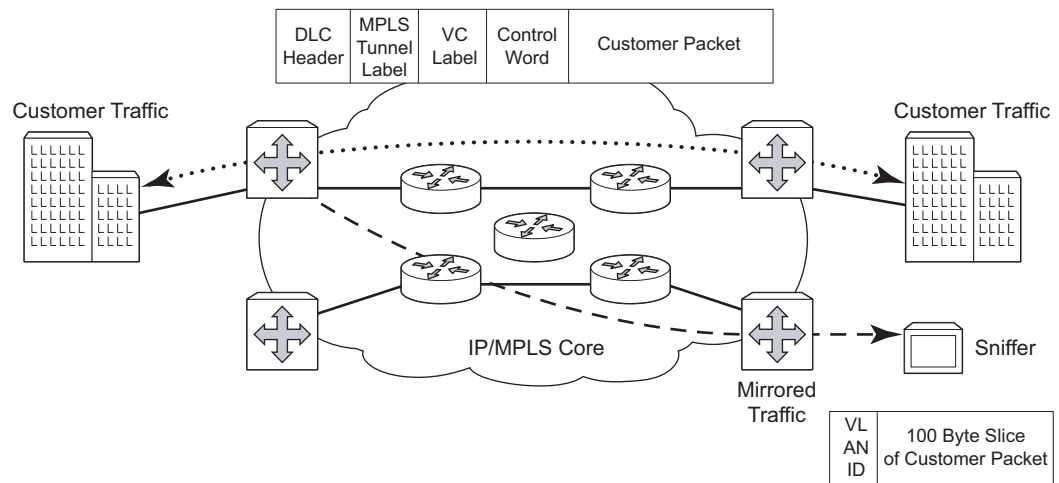
Figure 1 Service Mirroring
