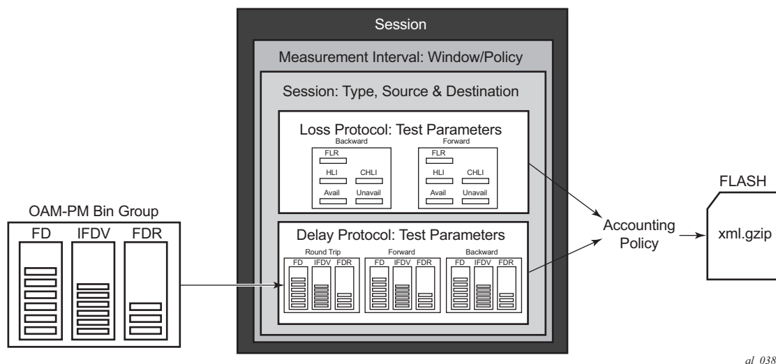
Figure 41 OAM-PM Architecture Hierarchy
