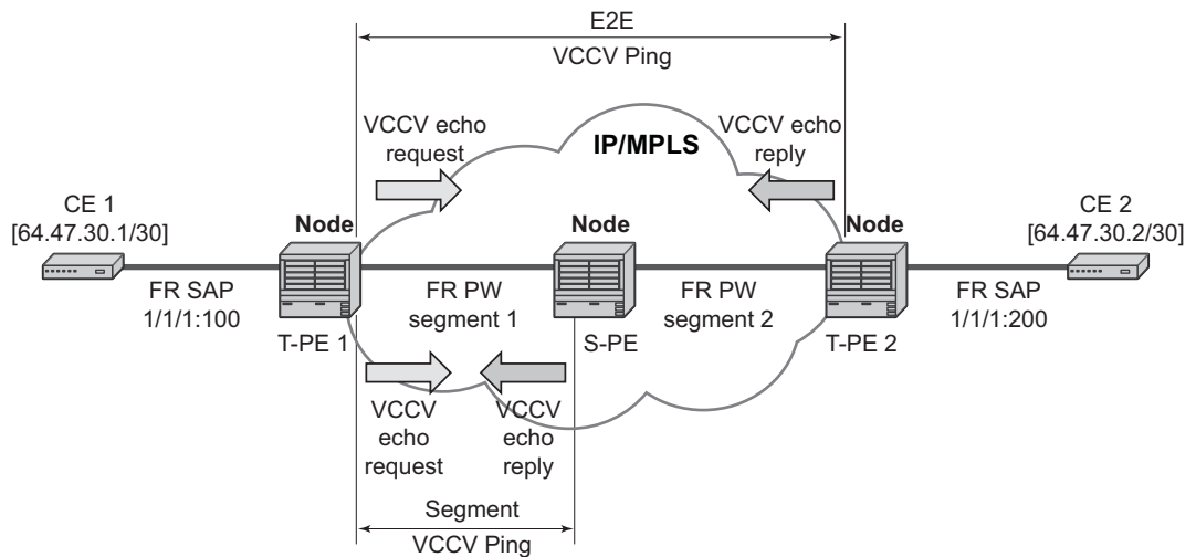
Figure 26 VCCV Ping over a Multi-Segment Pseudowire
