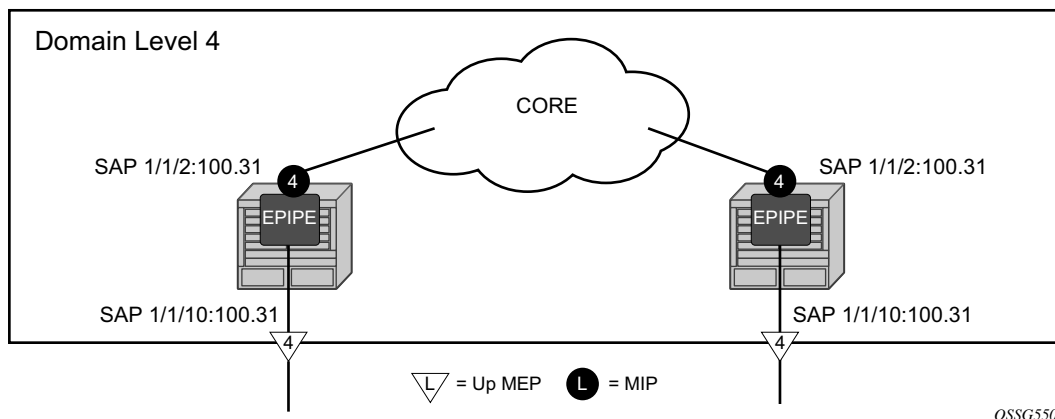
Figure 30 MIP Creation Default
