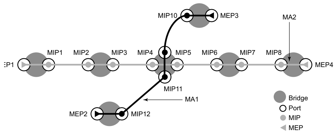
Figure 27 MEP and MIP
