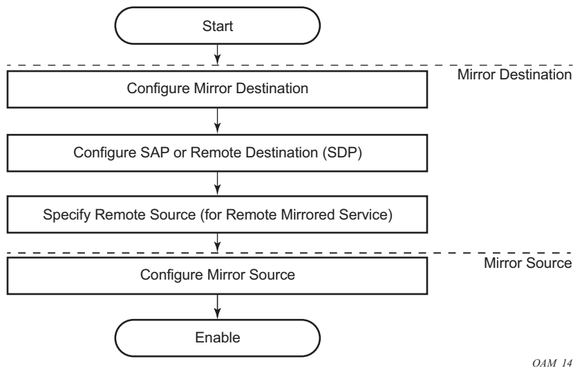
Figure 14 Mirror Configuration and Implementation Flow
