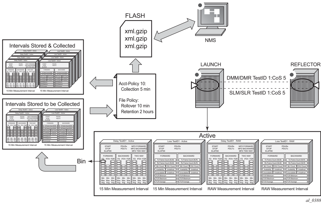
Figure 43 Relating OAM-PM Components
