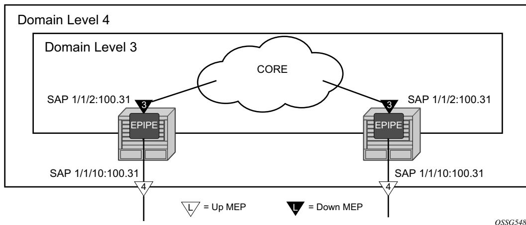
Figure 28 MEP Creation
