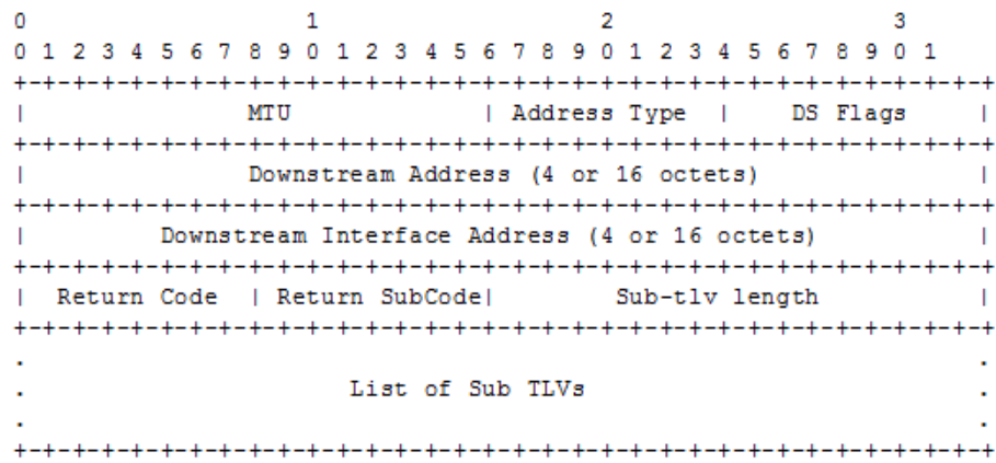
Figure 22 DDMAP TLV
