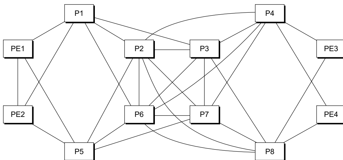
Figure 24 Network Resilience Using LDP ECMP
