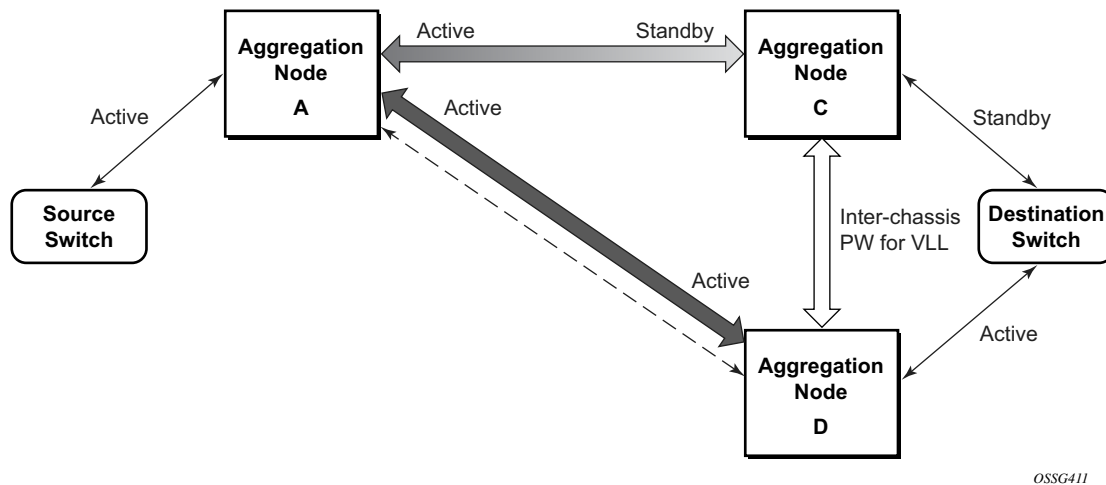
Figure 12 State Engine for a Non-Redundant Service to a Redundant Mirror Service
