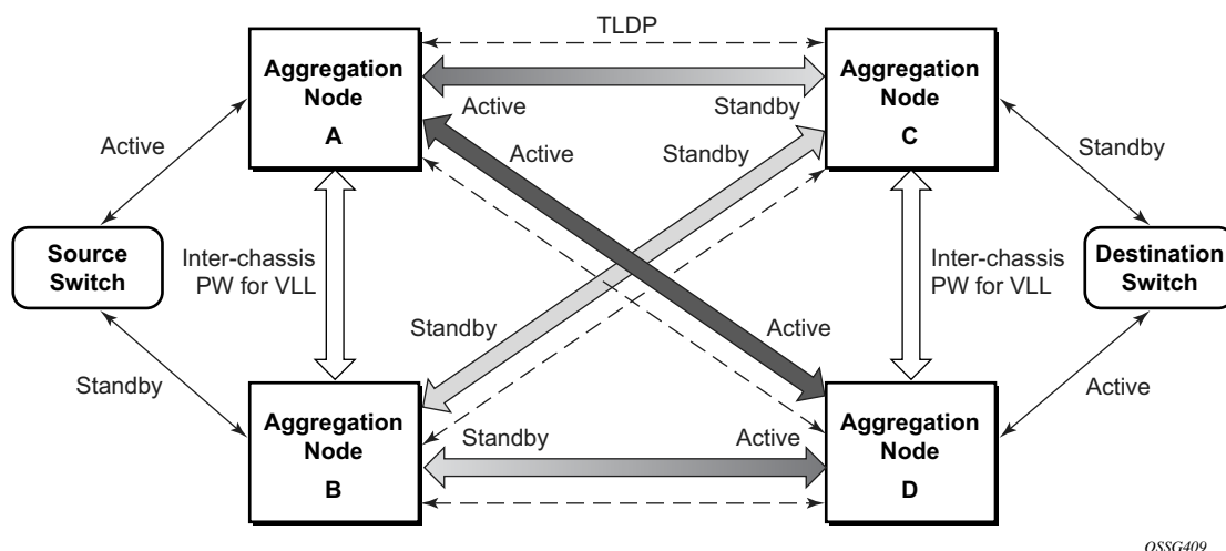
Figure 20 State Engine for Redundant Service to a Redundant Mirror Service
