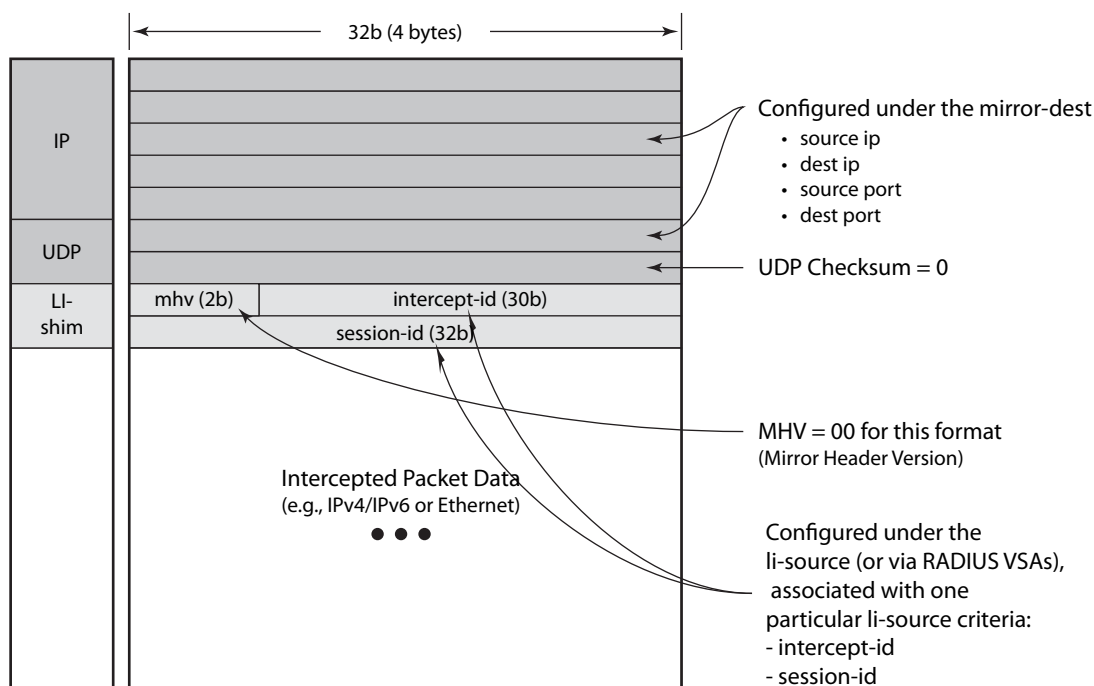
Figure 8 Routable Encapsulation Format
