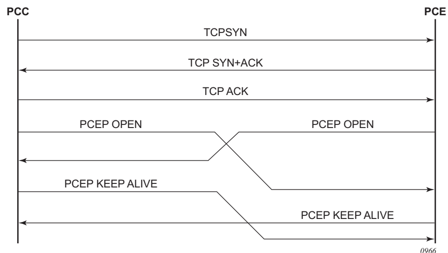
Figure 55 PCEP Session Initialization
