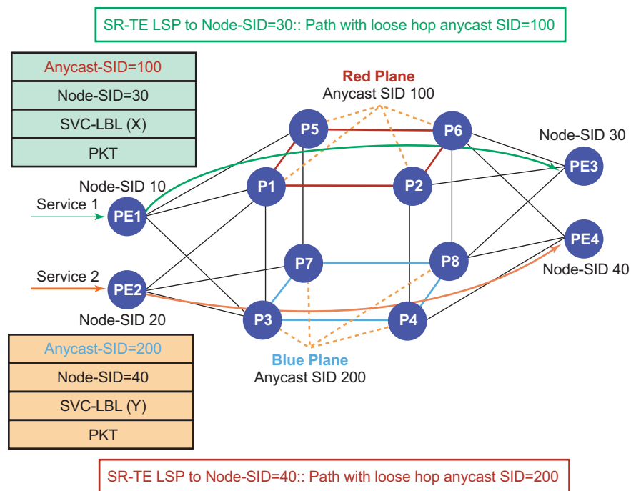
Figure 37 Multi-plane Traffic Engineering with Node Protection
