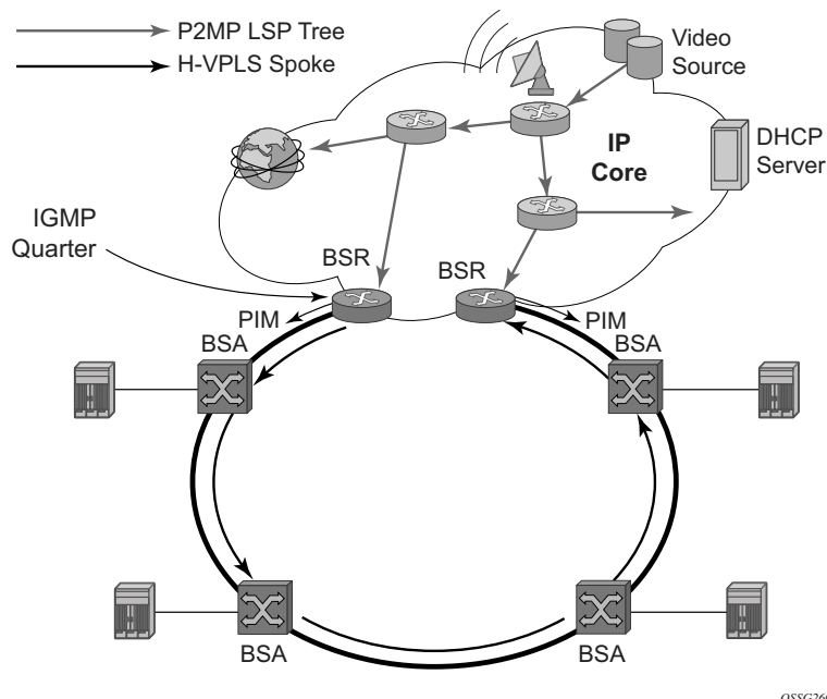
Figure 36 Application of P2MP LSP in Video Broadcast
