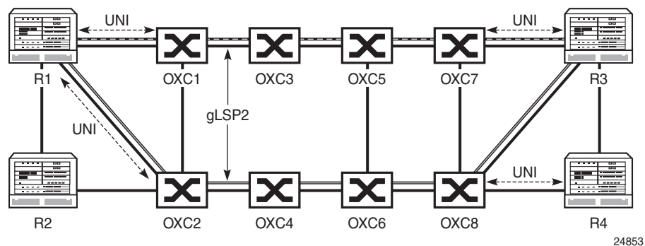
Figure 41 Multi-Layer Resiliency
