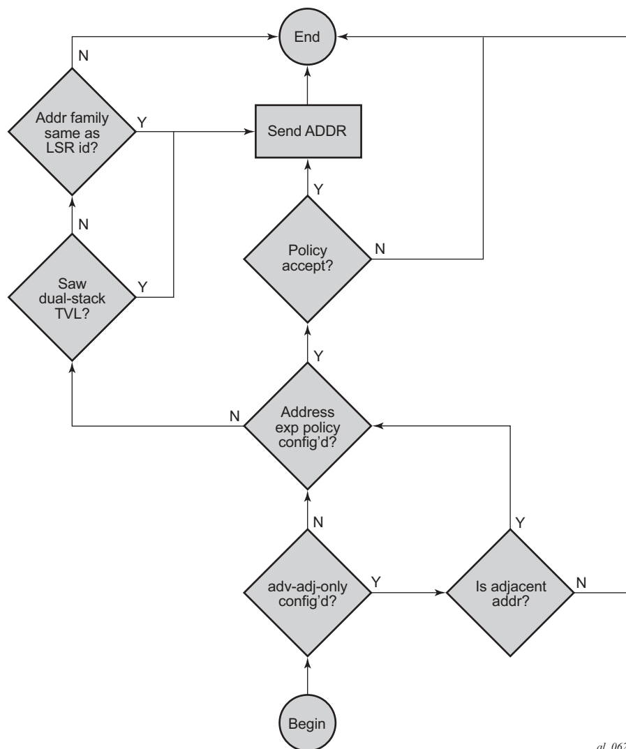
Figure 77 LDP IPv6 Address and FEC Distribution Procedure
