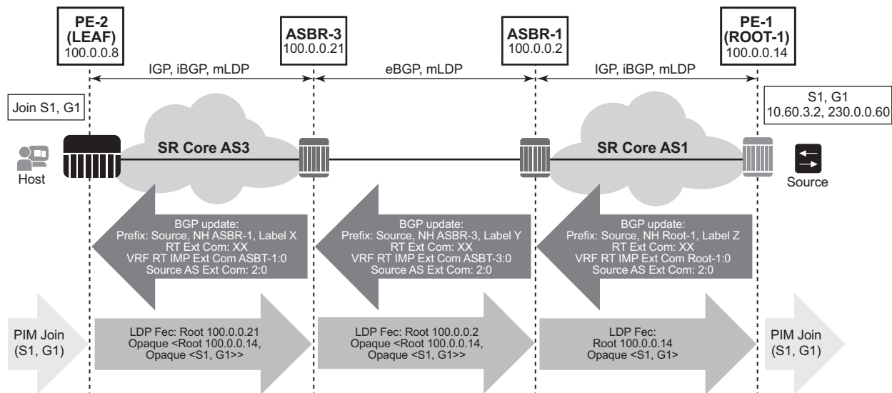
Figure 69 Non-VPN mLDP with Recursive Opaque for Inter-AS
