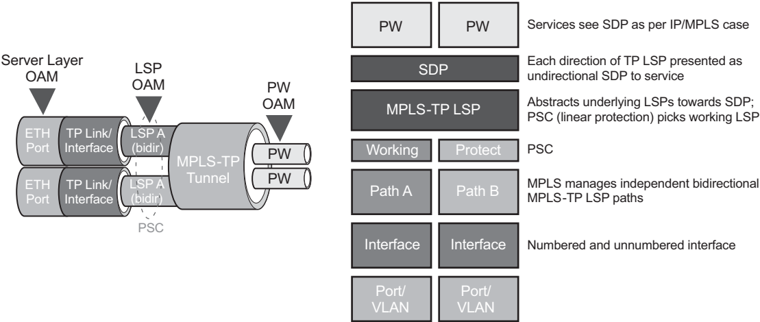
Figure 7 MPLS-TP Model
