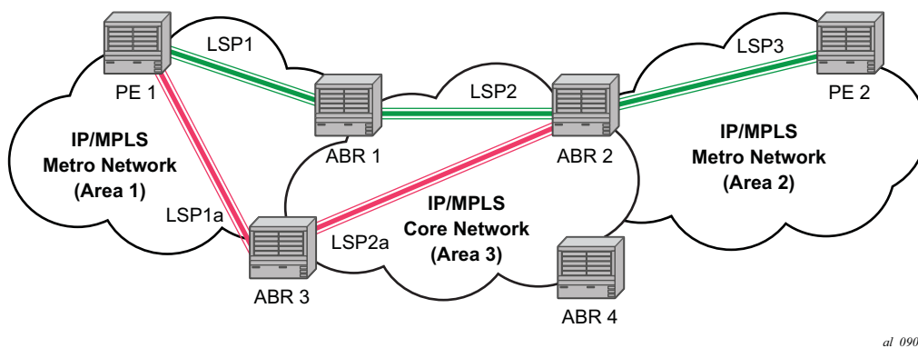
Figure 58 LDP over RSVP Application
