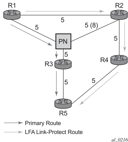
Figure 62 Example Topology with Broadcast Interfaces
