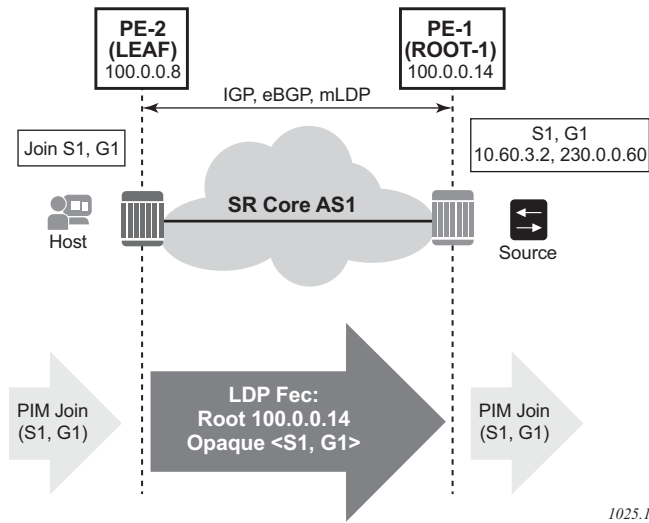
Figure 67 mLDP FEC for Single AS with Transit IPv4 Opaque
