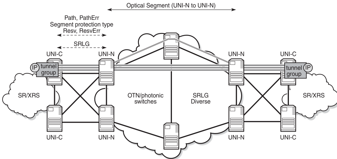
Figure 51 Optical Segment Protection Domain
