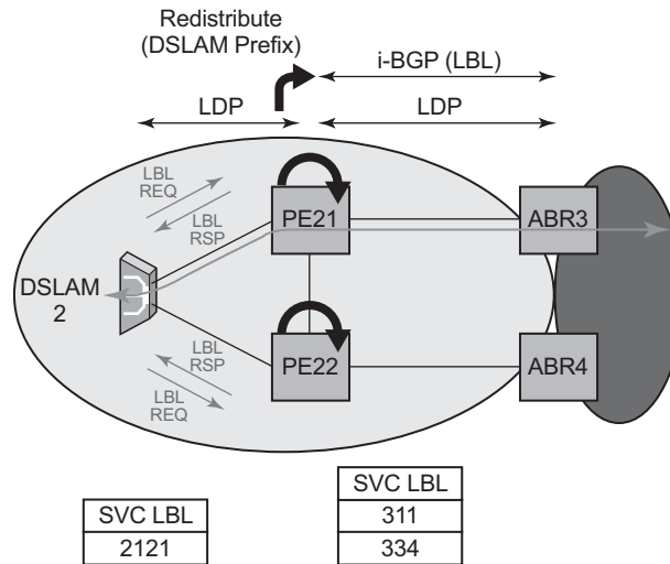
Figure 63 Application of LDP to BGP FEC Stitching
