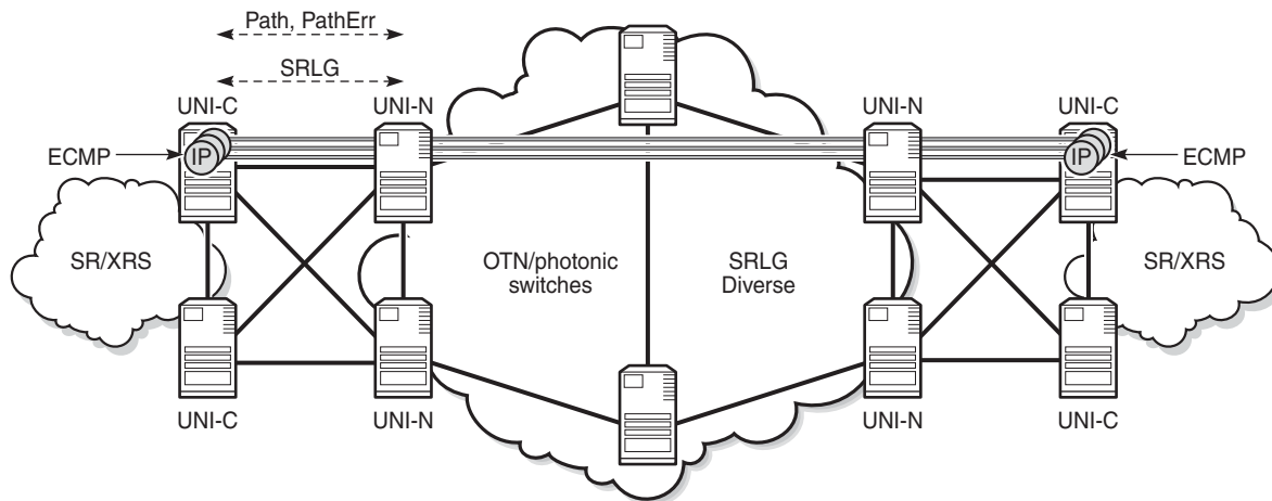
Figure 45 End-to-End ECMP with gLSP Diversity Across Single UNI-C
