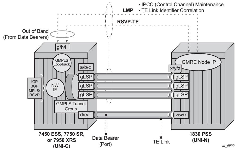
Figure 42 GMPLS UNI Architecture
