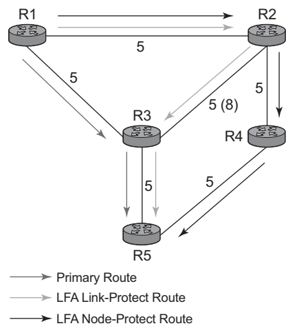
Figure 61 Topology with Primary and LFA Routes
