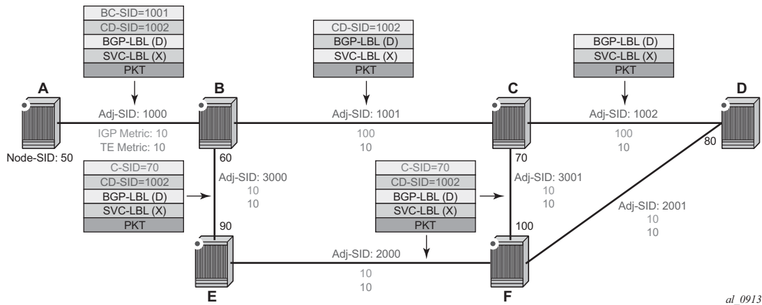
Figure 38 SR-TE LSP Label Stack Programming
