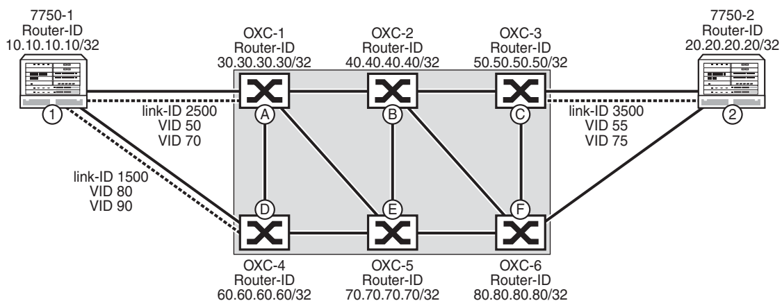
Figure 52 SRLG Example
