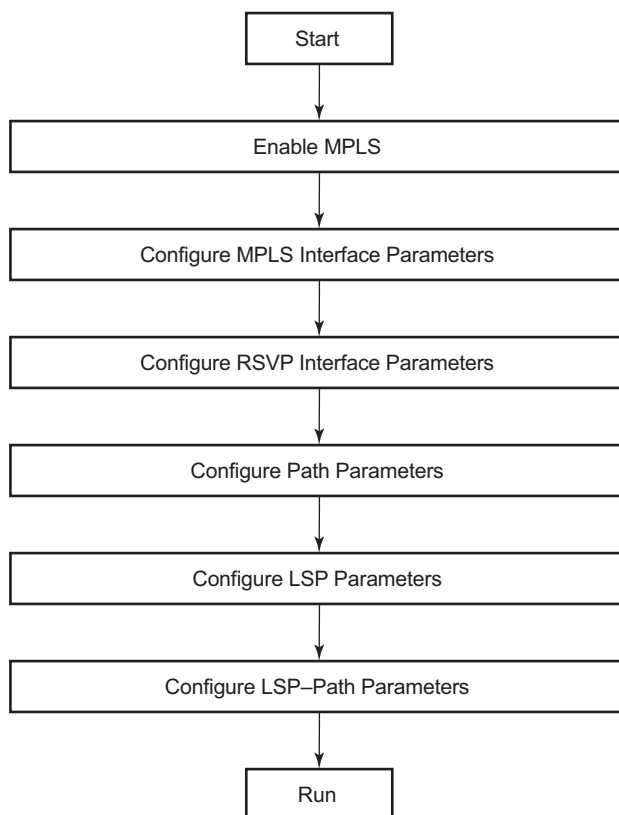
Figure 39 MPLS and RSVP Configuration and Implementation Flow
