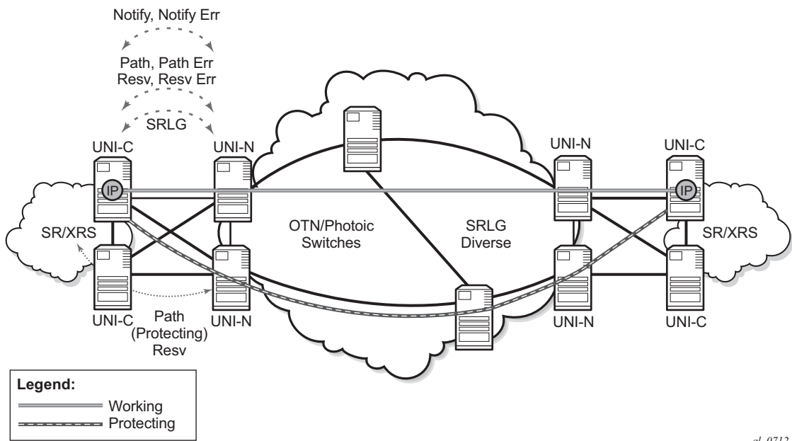
Figure 49 1:N Protection, with N=1 (RFC4872)
