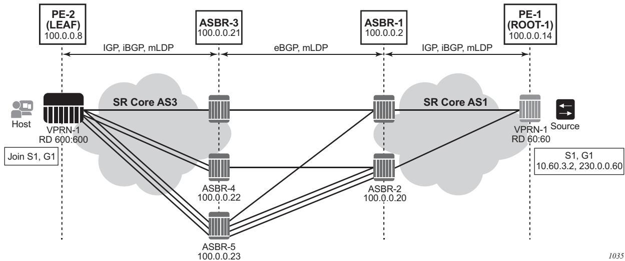
Figure 73 ECMP Support
