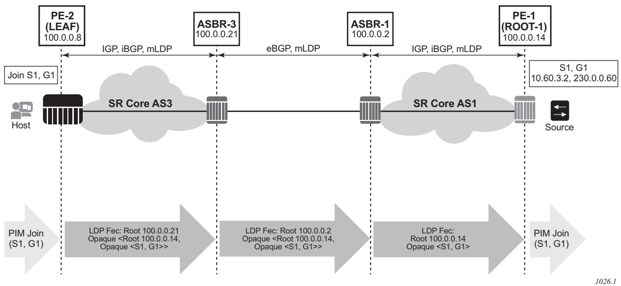
Figure 68 mLDP FEC for Inter-AS with Recursive Opaque Value
