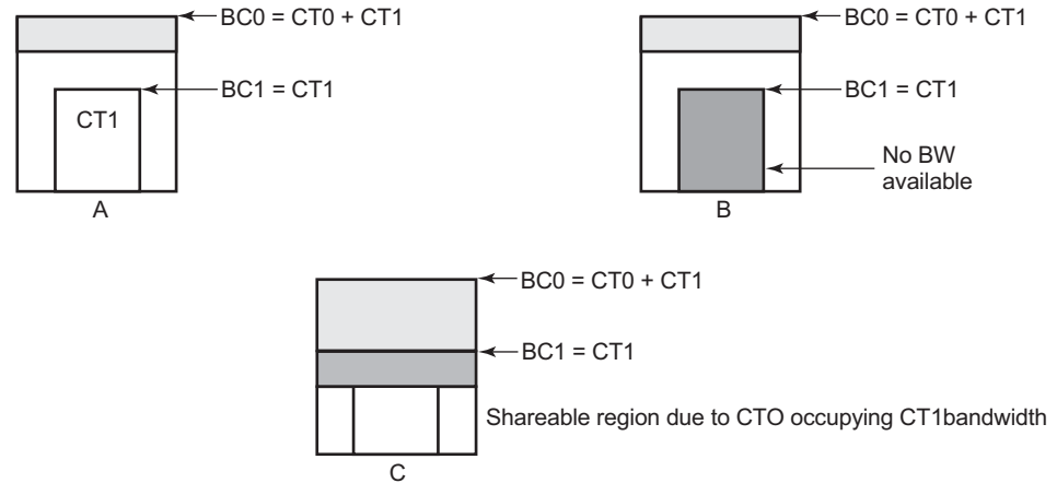
Figure 30 Sharing Bandwidth When an LSP Primary Path is Upgraded to Main CT
