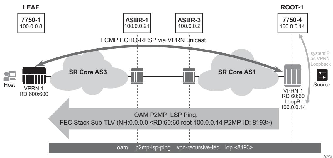
Figure 72 MVPN Inter-AS Option B OAM
