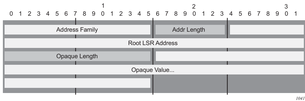
Figure 71 ECHO Request Target FEC Stack TLV
