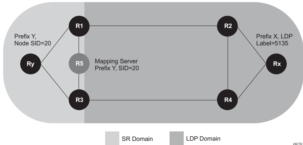
Figure 64 Stitching in the LDP-to-SR Direction
