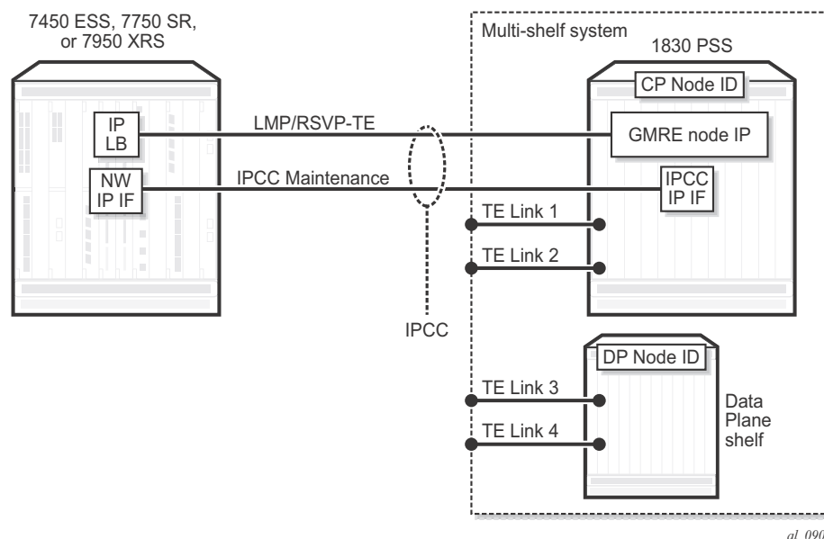
Figure 43 Identifier Architecture
