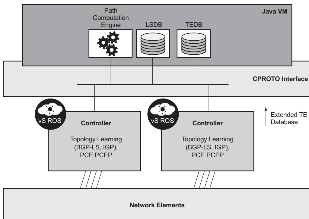
Figure 54 Packet Network Resource Controller (NRC-P) Architecture
