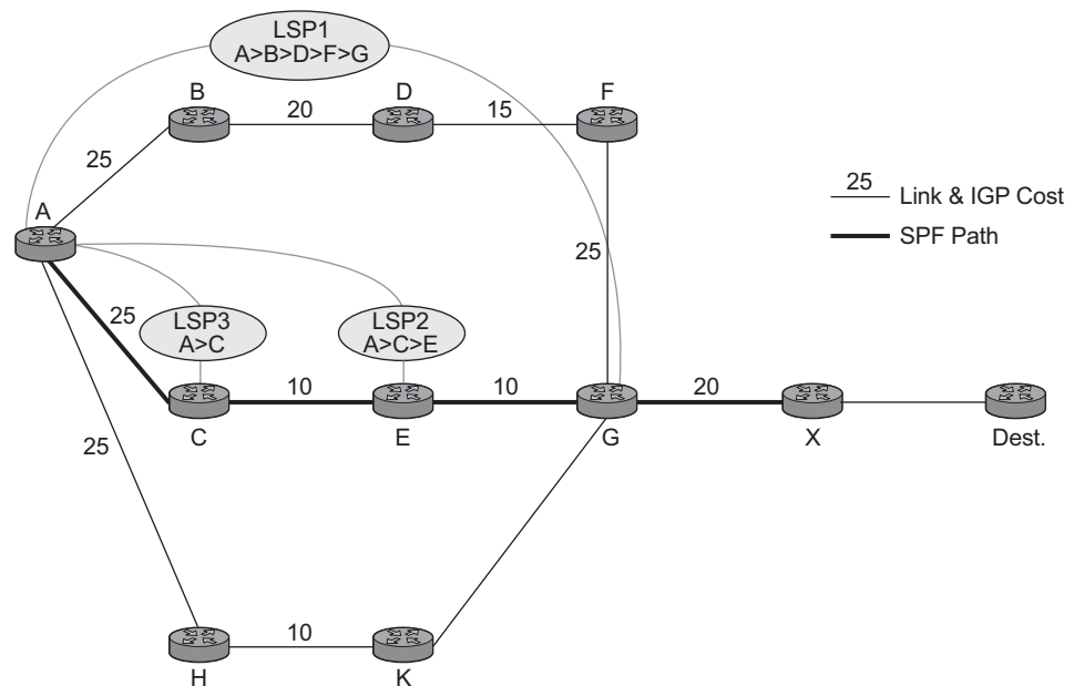
Figure 60 LDP over RSVP Without ABR Stitching Point
