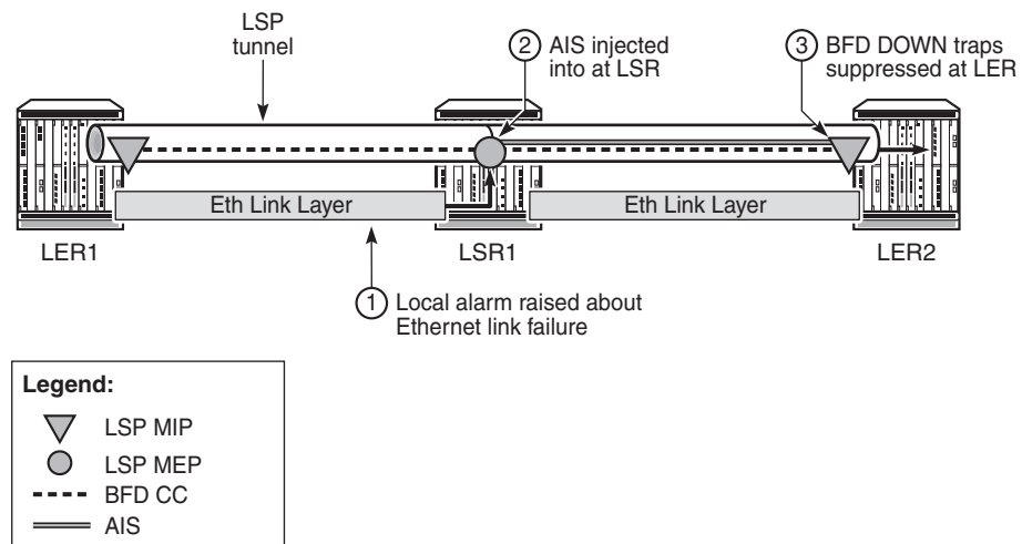
Figure 24 Example of AIS in MPLS-TP
