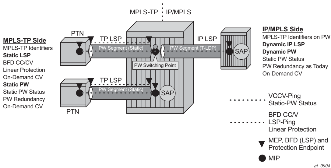
Figure 23 Static - Dynamic PW Switching with MPLS-TP
