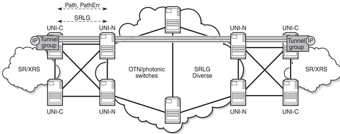
Figure 46 End-to-End Load Sharing GMPLS Tunnel Group with gLSP Path Diversity
