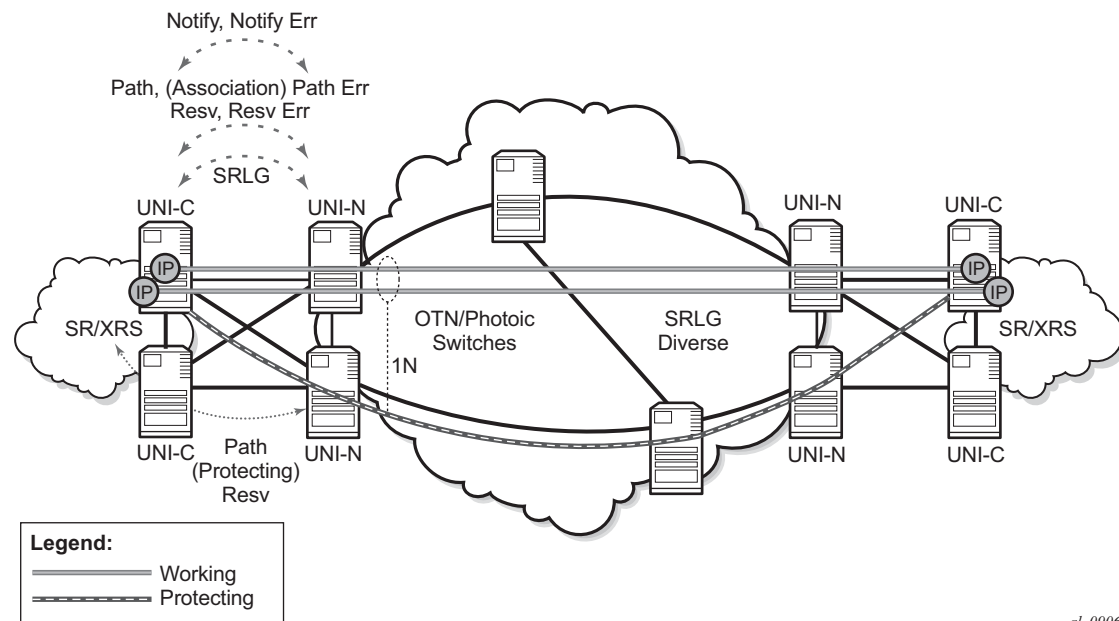
Figure 50 N>1 Protection
