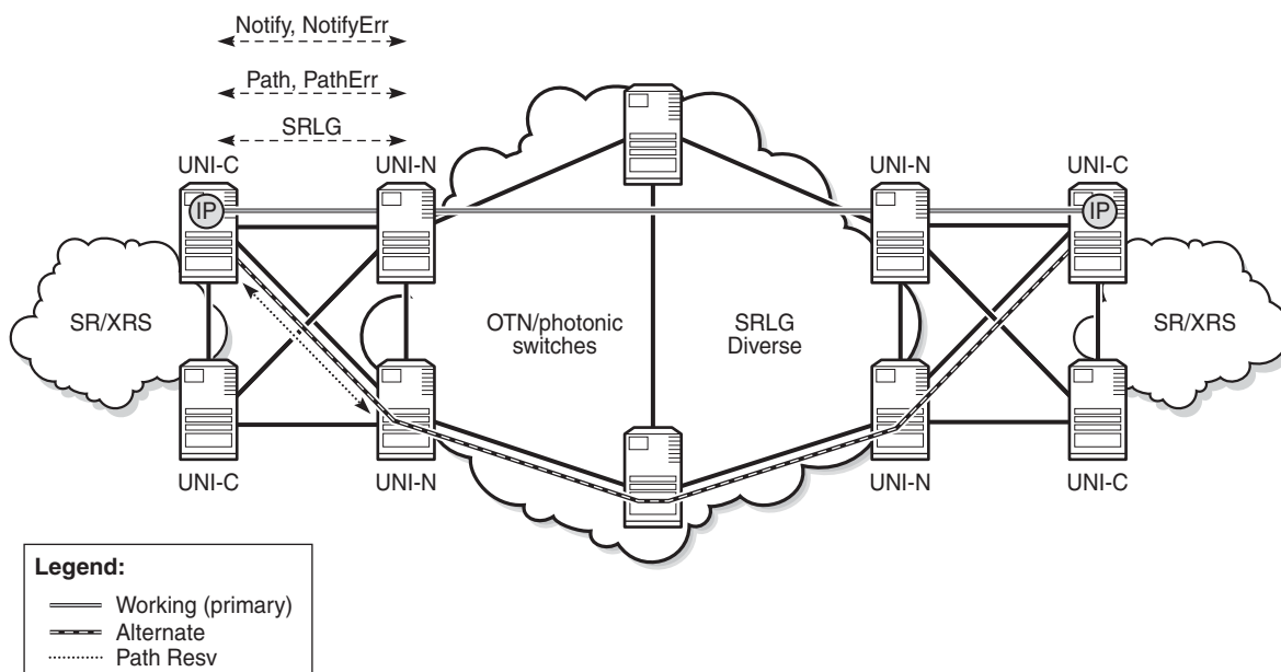
Figure 48 Full LSP Rerouting
