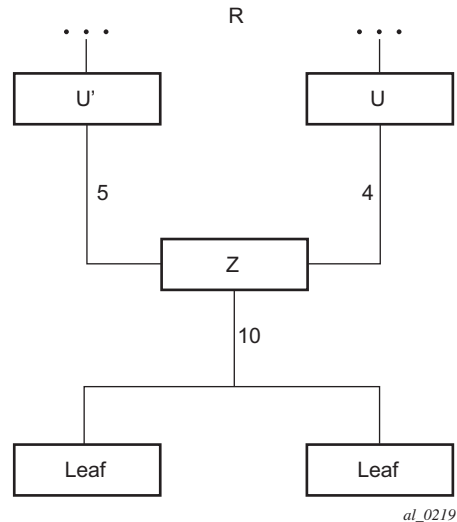
Figure 74 mLDP LSP with Backup Upstream LSR Nodes
