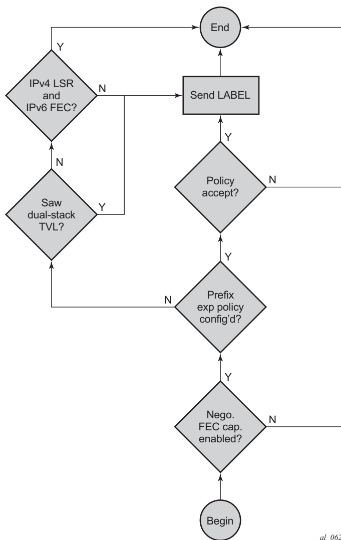
Figure 76 LDP IPv6 Address and FEC Distribution Procedure
