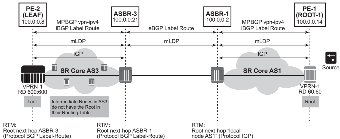
Figure 66 Inter-AS Option C
