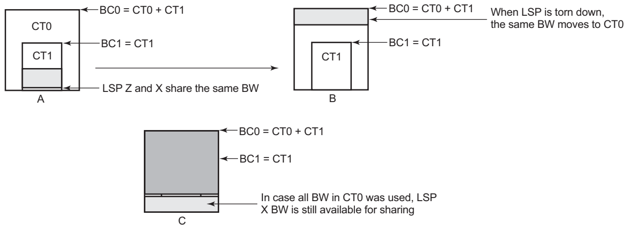
Figure 29 Sharing bandwidth when an LSP primary path is downgraded to backup CT
