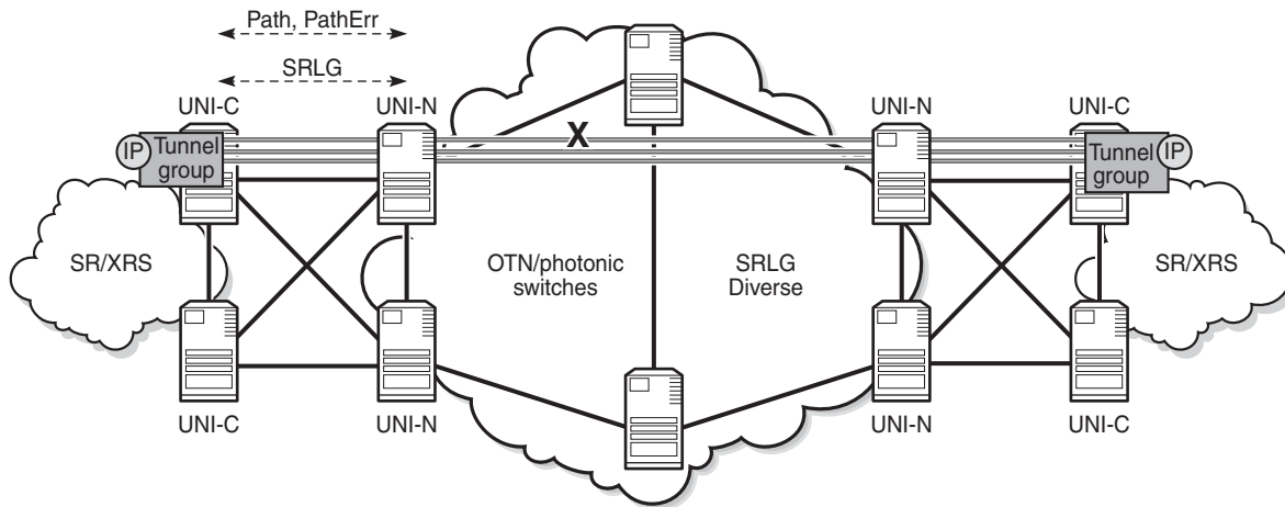
Figure 47 gLSP Re-Establishment (PATH Refresh)
