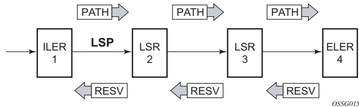
Figure 5 Establishing LSPs
