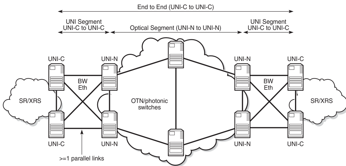
Figure 44 General GMPLS UNI Interconnection Architecture
