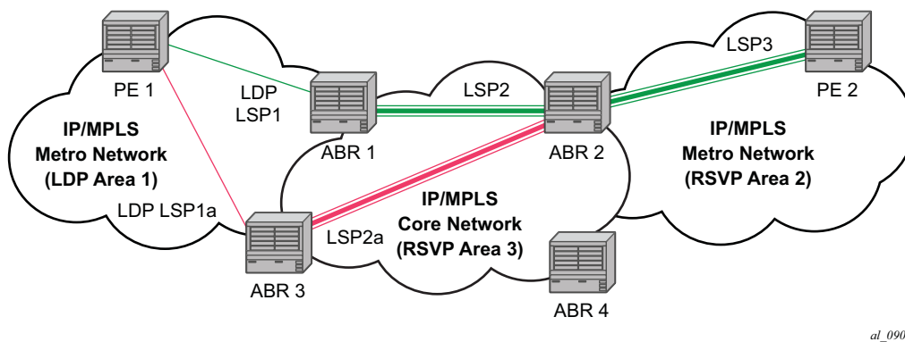
Figure 59 LDP over RSVP Application Variant
