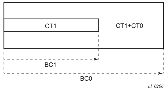
Figure 25 RDM with Two Class Types
