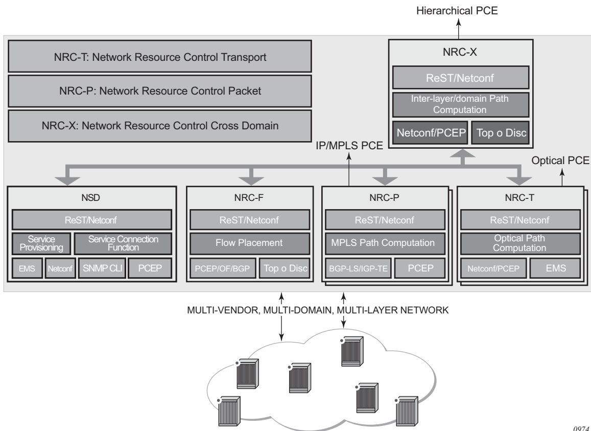
Figure 53 NSP Functional Modules
