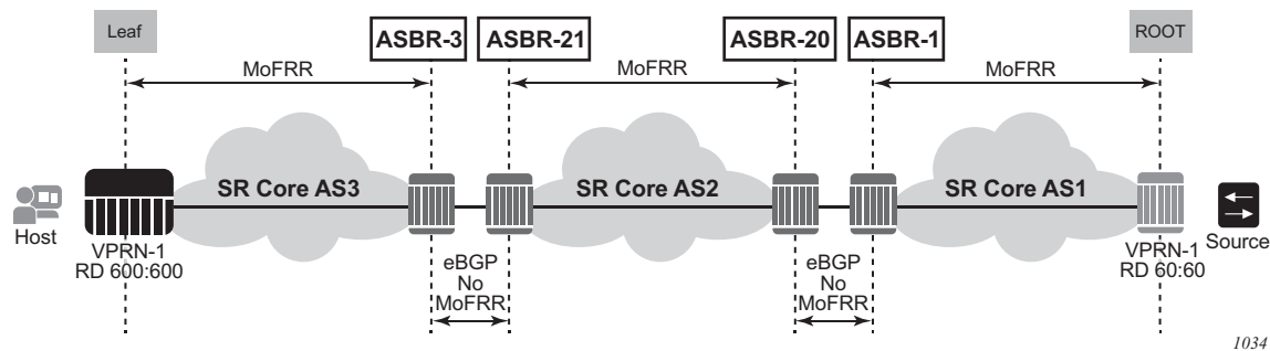
Figure 70 ASBRs Using eBGP Without IGP
