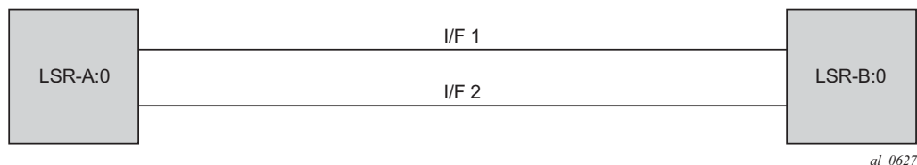
Figure 75 LDP Adjacency and Session over an IPv6 Interface
