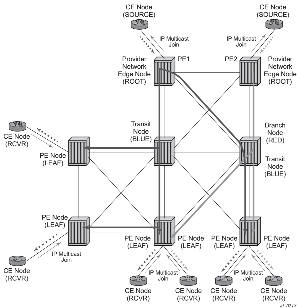
Figure 65 Video Distribution using P2MP LDP
