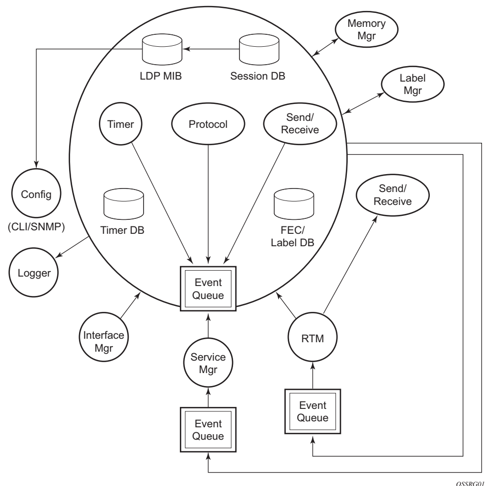
Figure 56 Subsystem Interrelationships
