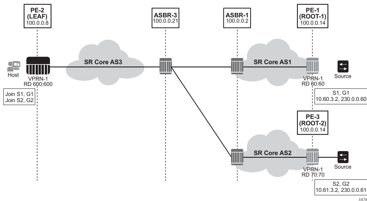
Figure 42 Identical System IP on Multiple PEs (Option B)
