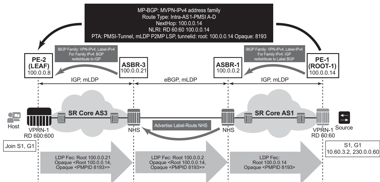
Figure 45 Non-segmented mLDP PMSI Establishment (Option C)
