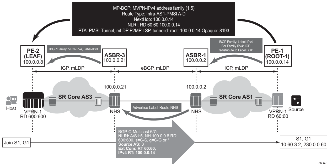
Figure 46 Non-segmented mLDP C-multicast Exchange (Option C)
