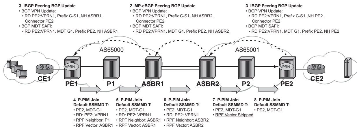
Figure 38 Inter-AS Option B Default MDT Setup
