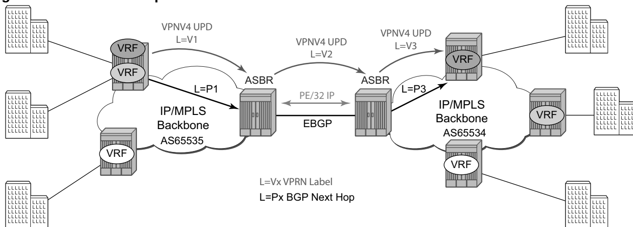
Figure 21 Inter-AS Option-B
