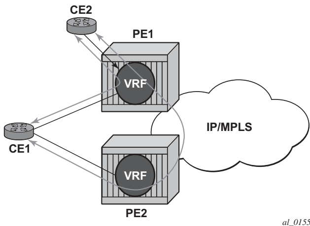
Figure 11 Basic eiBGP Topology
