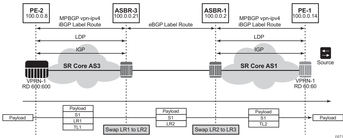
Figure 41 Unicast VPN Option C with Segmented MPLS
