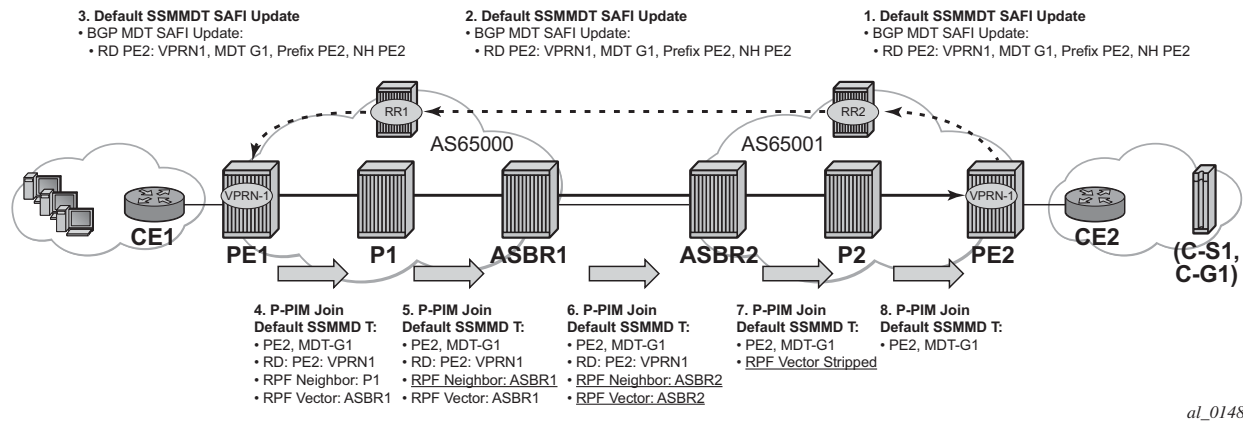
Figure 39 Inter-AS Option C Default MDT Setup
