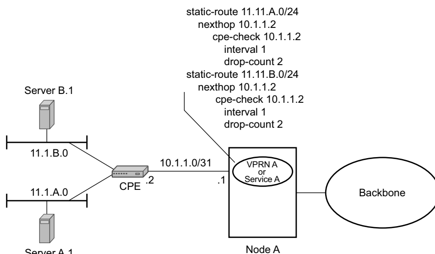
Figure 13 Directly Connected IP Target
