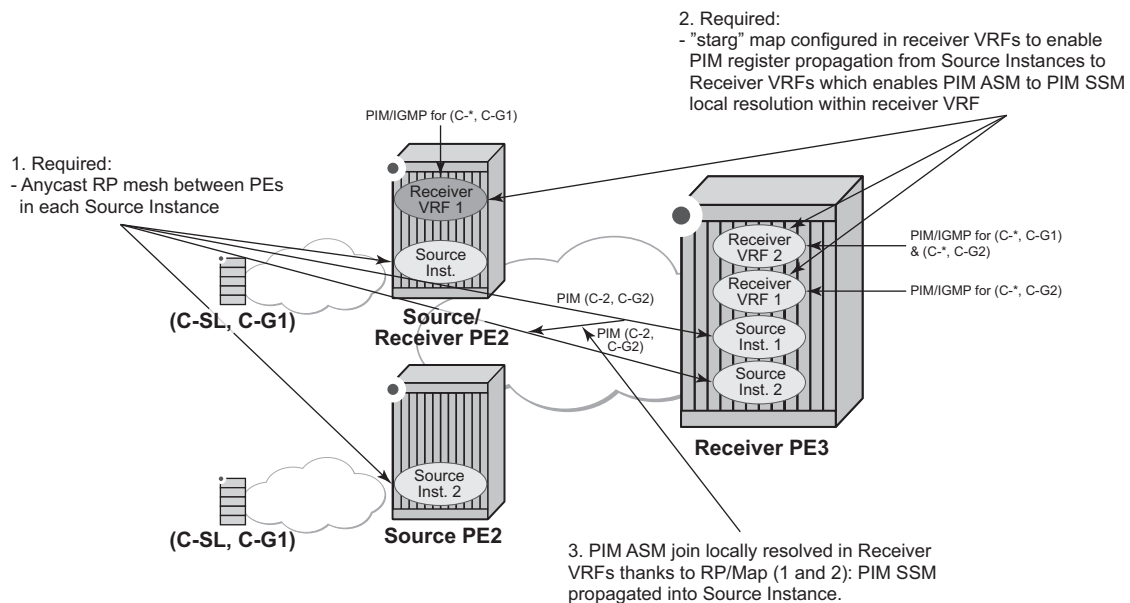
Figure 32 Multicast Extranet with per group PIM ASM mapping
