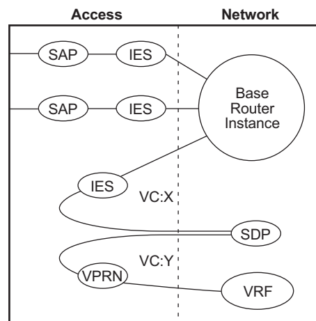
Figure 7 SDP-ID and VC Label Service Identifiers
