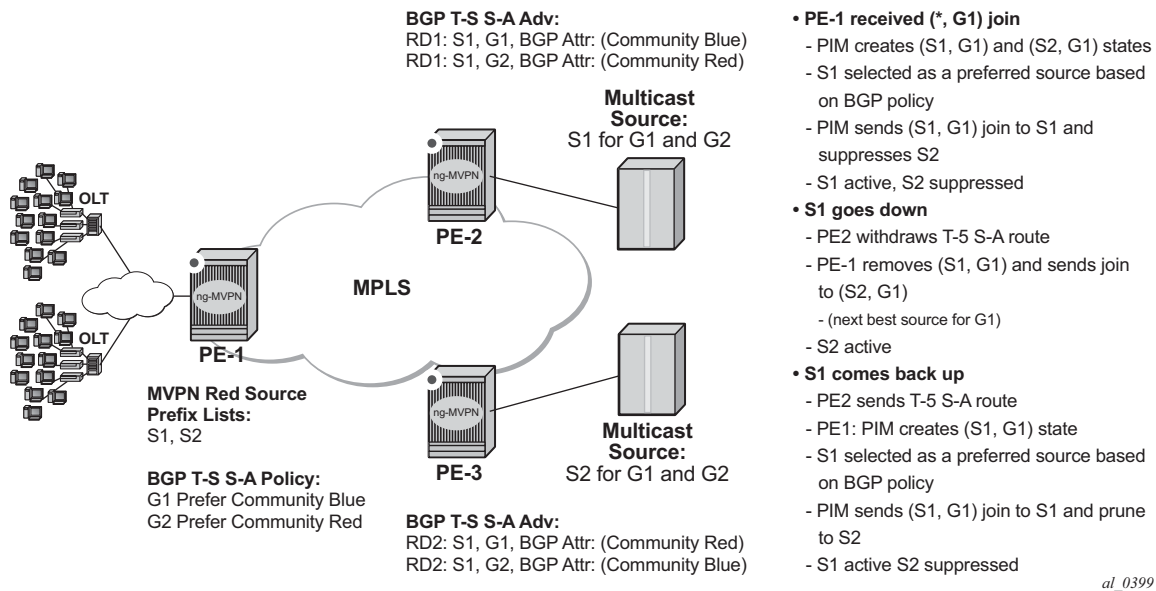
Figure 36 Preferred Source Selection for Multicast Source Geo-Redundancy
