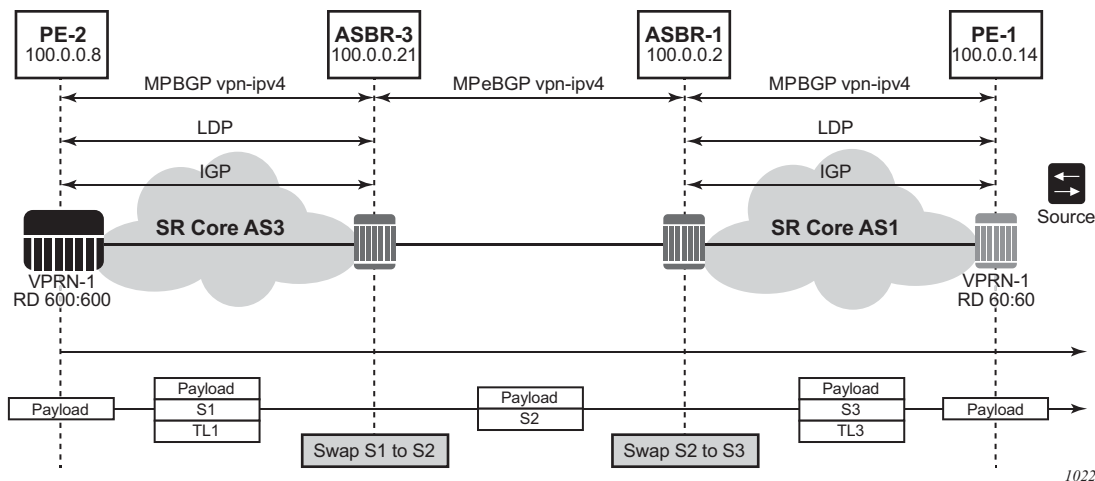
Figure 40 Unicast VPN Option B with Segmented MPLS
