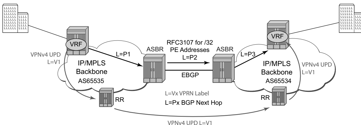
Figure 22 Option C Example
