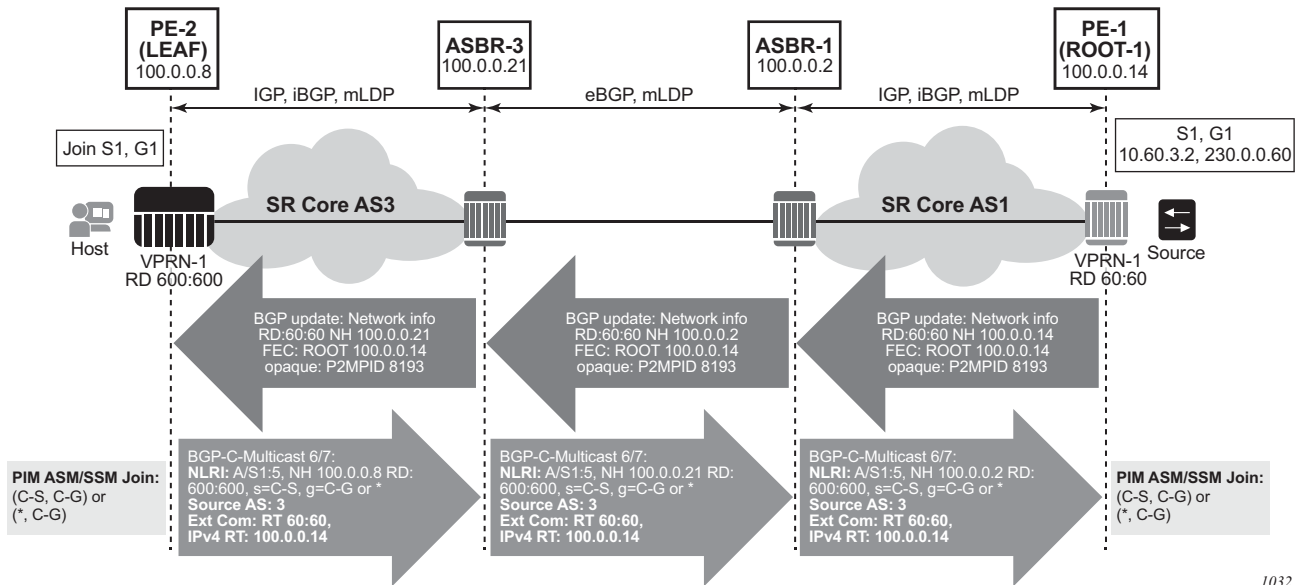
Figure 44 Non-segmented mLDP C-multicast Exchange (Option B)
