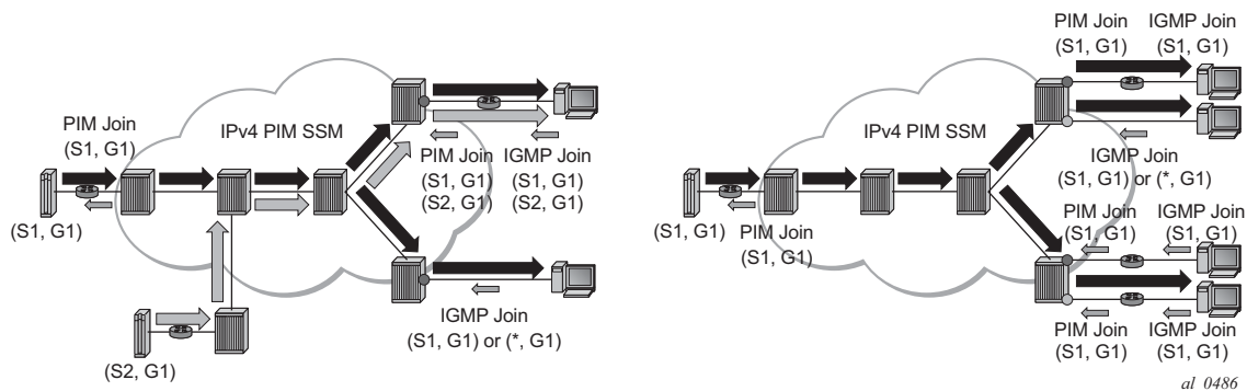
Figure 31 GRT/VRF Extranet
