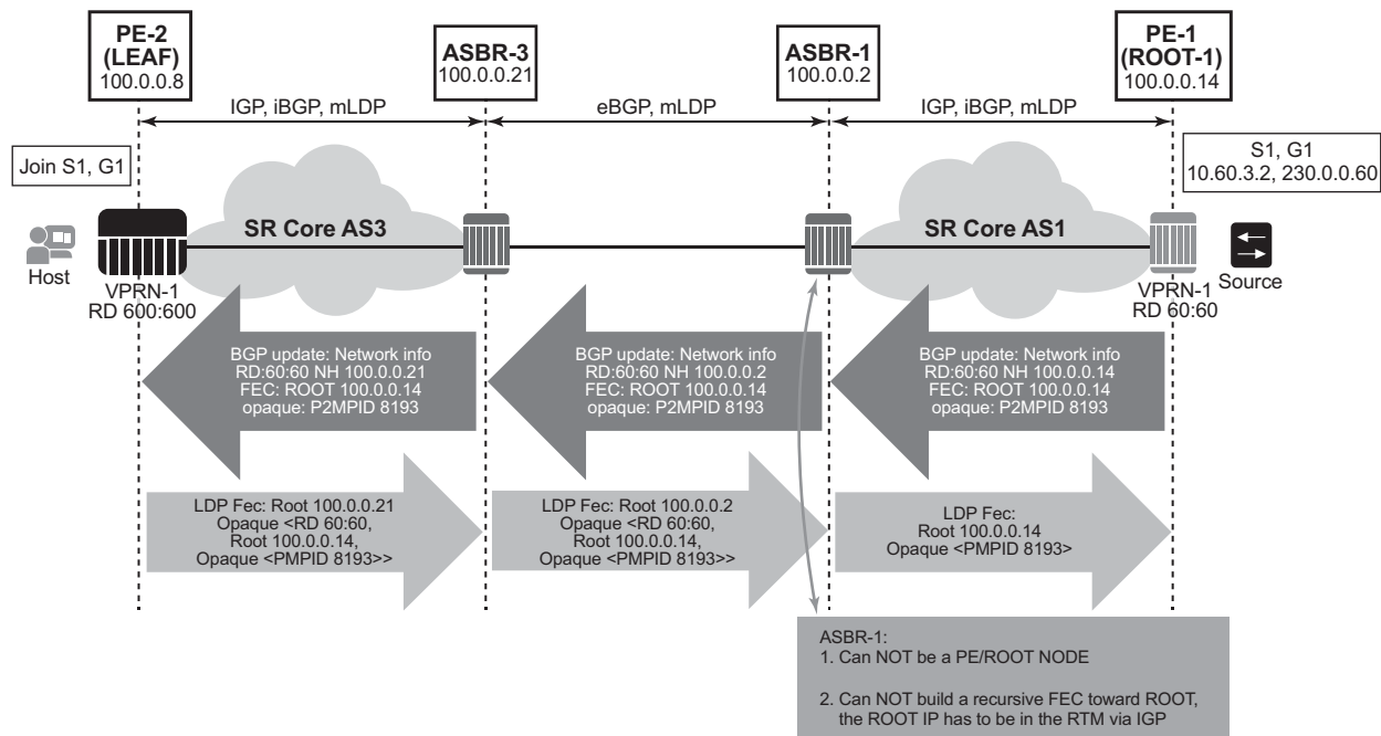
Figure 43 Non-segmented mLDP PMSI Establishment (Option B)
