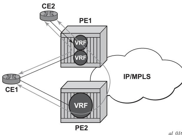
Figure 12 Extranet Load Balancing
