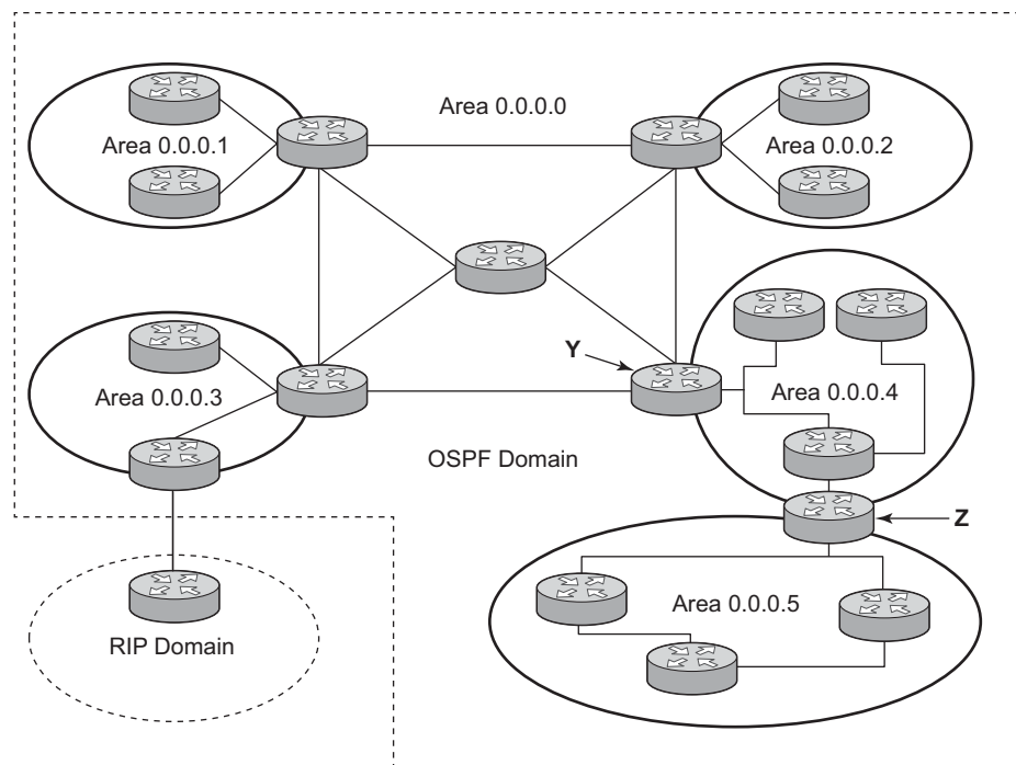
Figure 47 OSPF Areas
