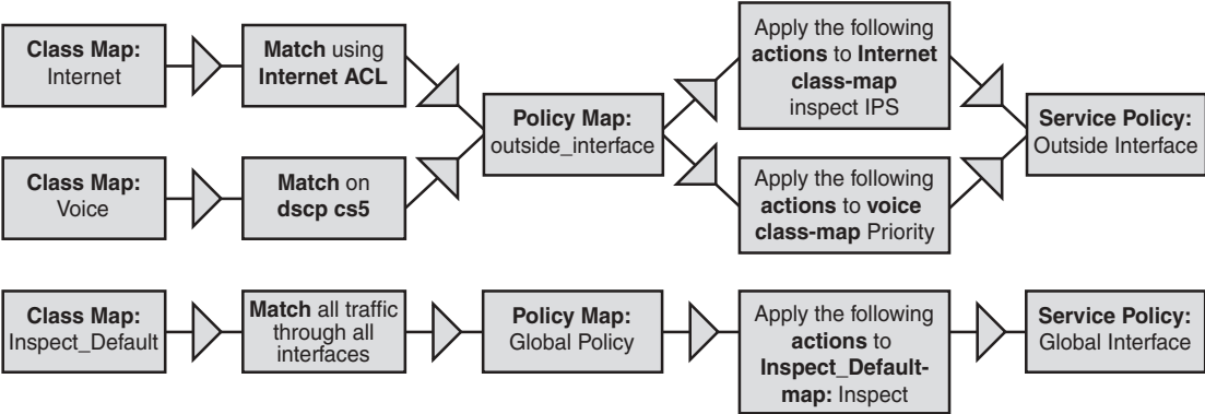
Figure 8-1 Modular Policy Example Flow
