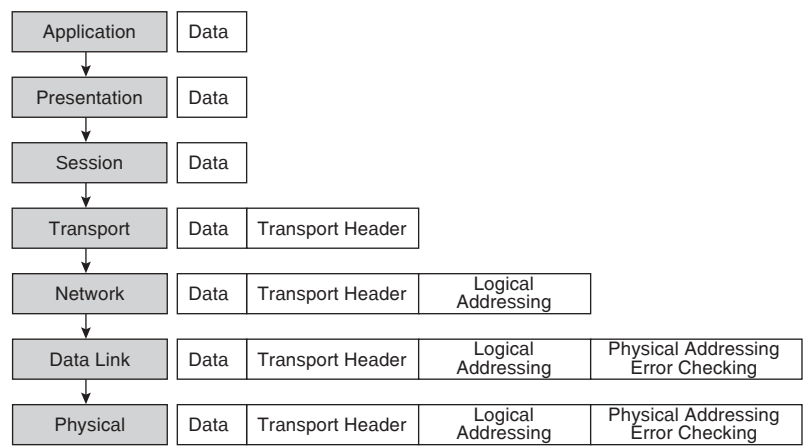
Figure 5-1 Encapsulation of Upper-Layer Data
