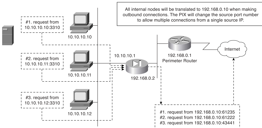
Figure 5-5 PAT
