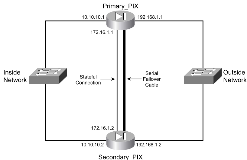
Figure 12-3 Network Diagram of Failover Configuration
