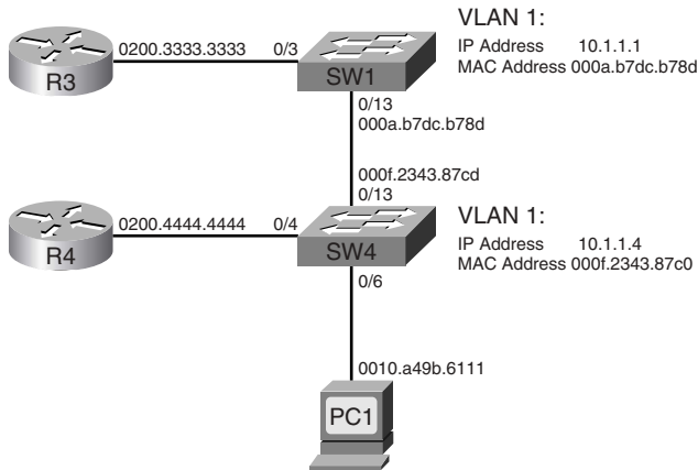
Figure 1-6 Sample Network with MAC Addresses Shown
