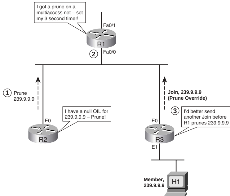
Figure 20-11 Prune Override
