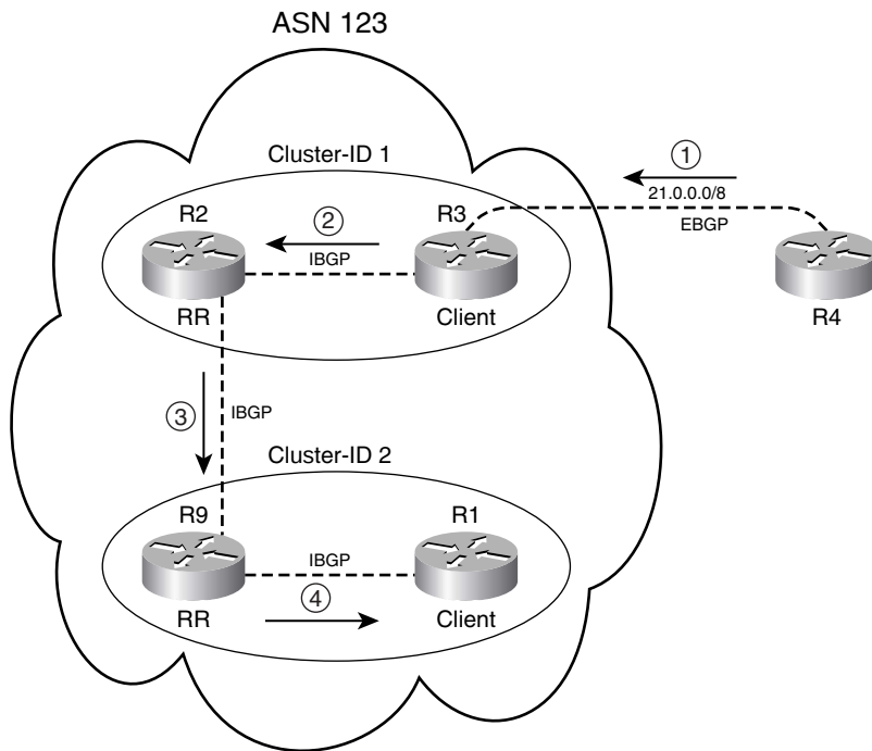
Figure 12-12 Modified AS 123 Used in RR Example 12-15
