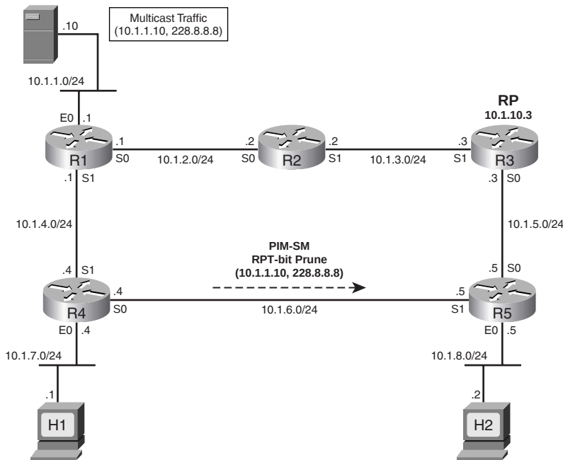
Figure 20-18 R4 Sends PIM-SM Prune with RP Bit Set to R5
