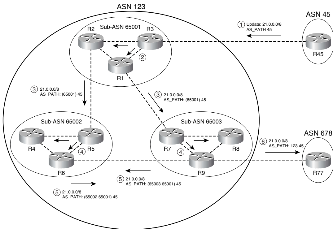
Figure 12-8 AS_PATH Changes in a Confederation
