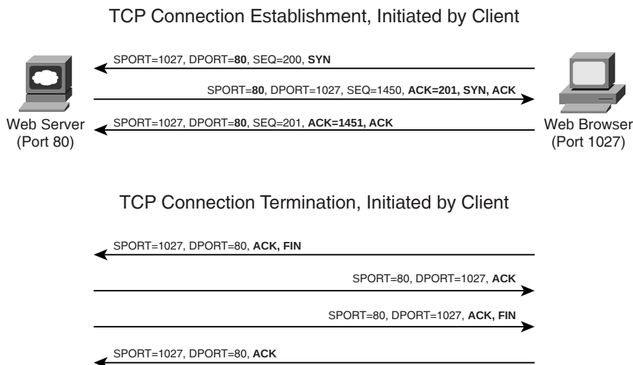
Figure 6-2 TCP Connection Establishment and Termination
