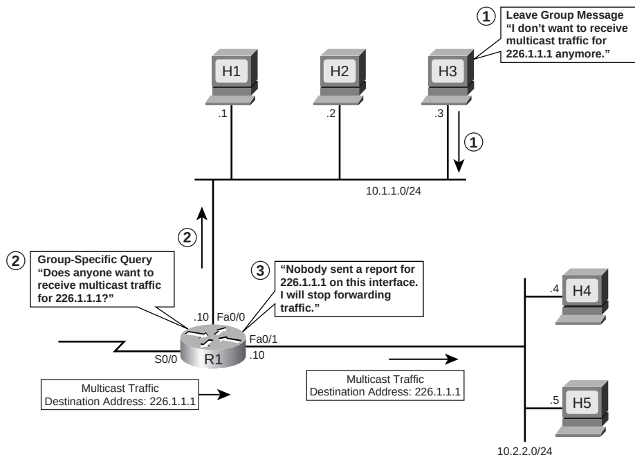
Figure 19-14 IGMPv2 Leave Process—No Response to the Group-Specific Query
