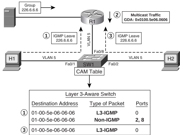
Figure 19-21 Leaving a Group Using IGMP Snooping and CAM Table Entries
