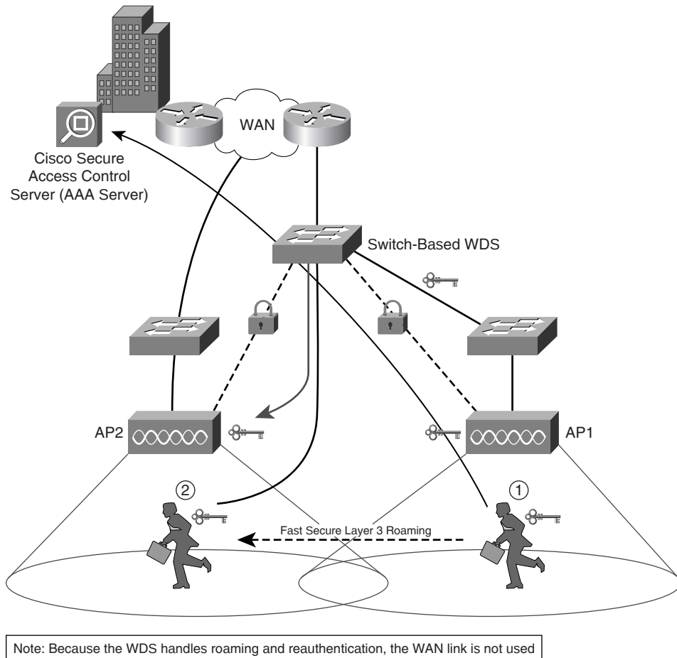
Figure 23-1 Cisco SWAN Fast Secure Roaming
