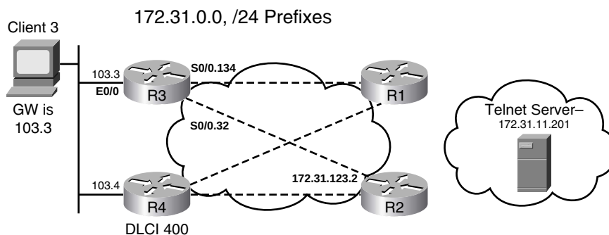
Figure 7-7 Policy Routing Example on Router3
