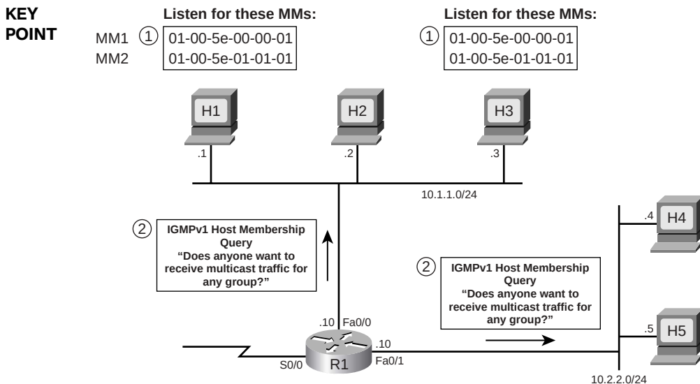
Figure 19-8 IGMPv1 Host Membership Query Process
