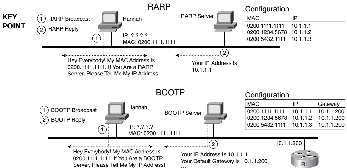
Figure 5-4 RARP and BOOTP—Basic Processes
