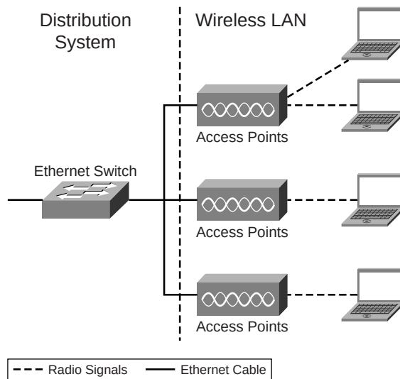
Figure 22-1 Infrastructure Wireless LAN
