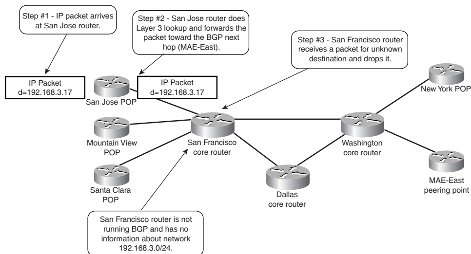
Figure C-17 Connectivity Loss in Network with No BGP on Core Routers
