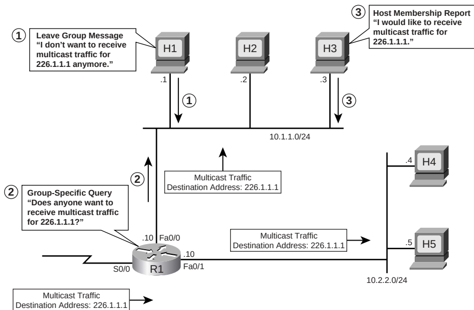
Figure 19-13 How Group-Specific Queries Work with the IGMPv2 Leave Process
