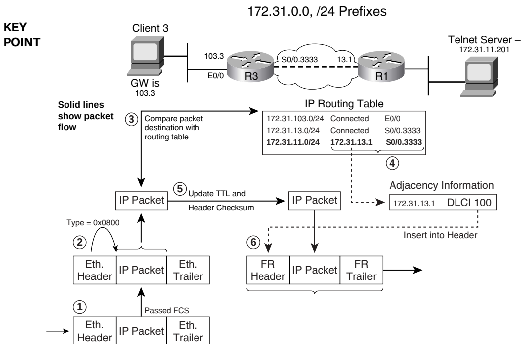
Figure 7-1 Forwarding Process at Router3, Destination Server1
