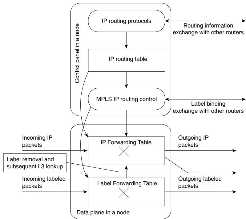
Figure C-4 Architecture of an Edge-LSR
