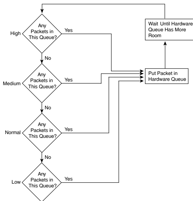
Figure 15-1 PQ Scheduling Logic
