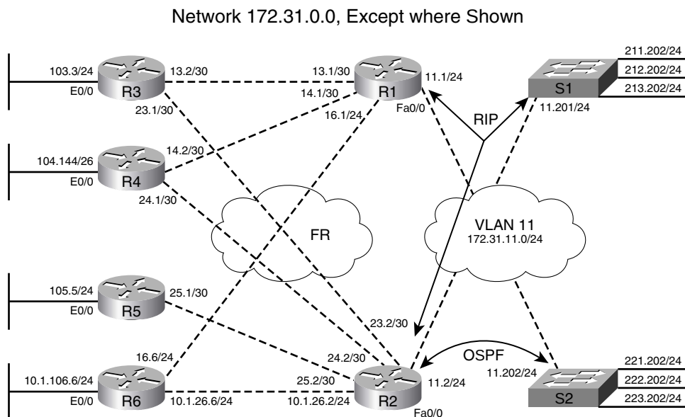
Figure 8-2 Sample Internetwork Used for RIP Configuration Examples
