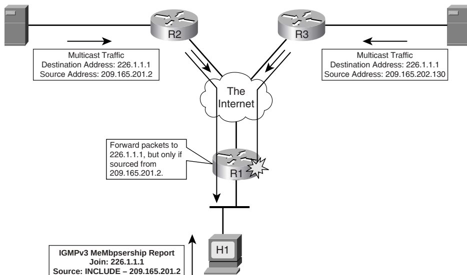
Figure 19-15 IGMPv3 Membership Report
