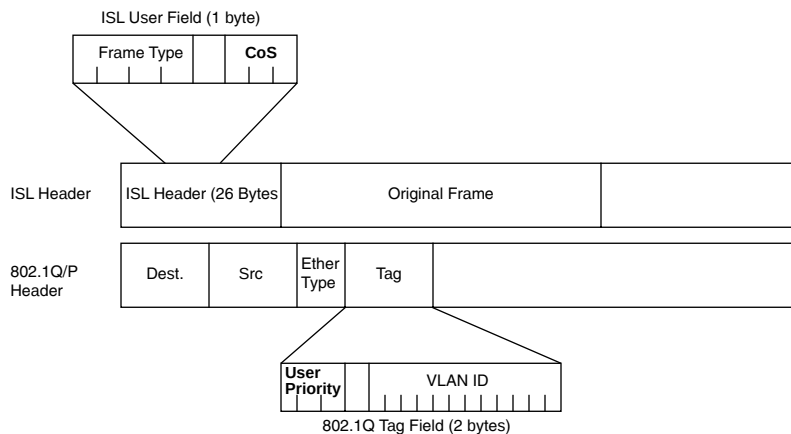
Figure 14-2 LAN CoS Fields
