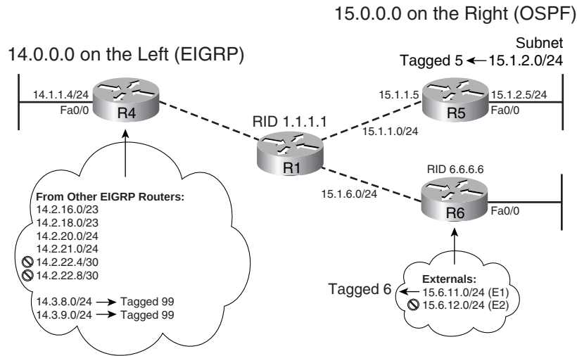
Figure 11-3 OSPF and EIGRP Mutual Redistribution Using Route Maps
