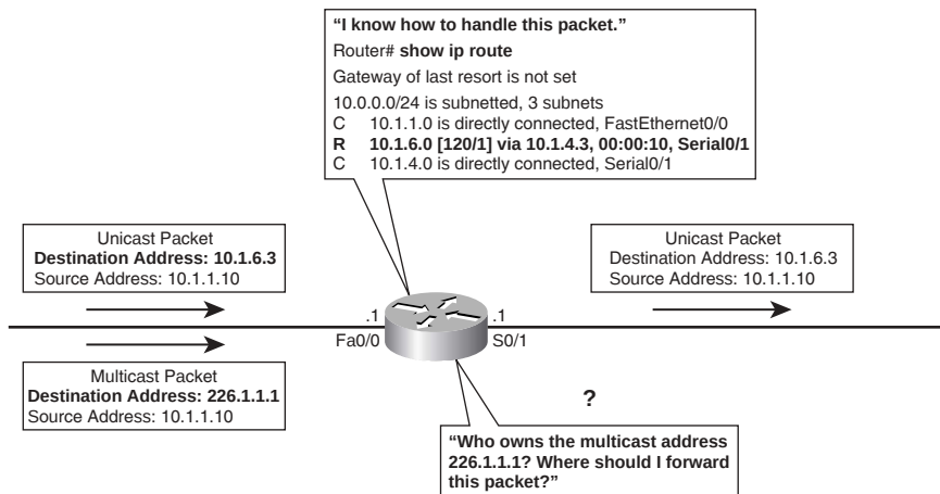
Figure 20-1 Multicast Routing Problem
