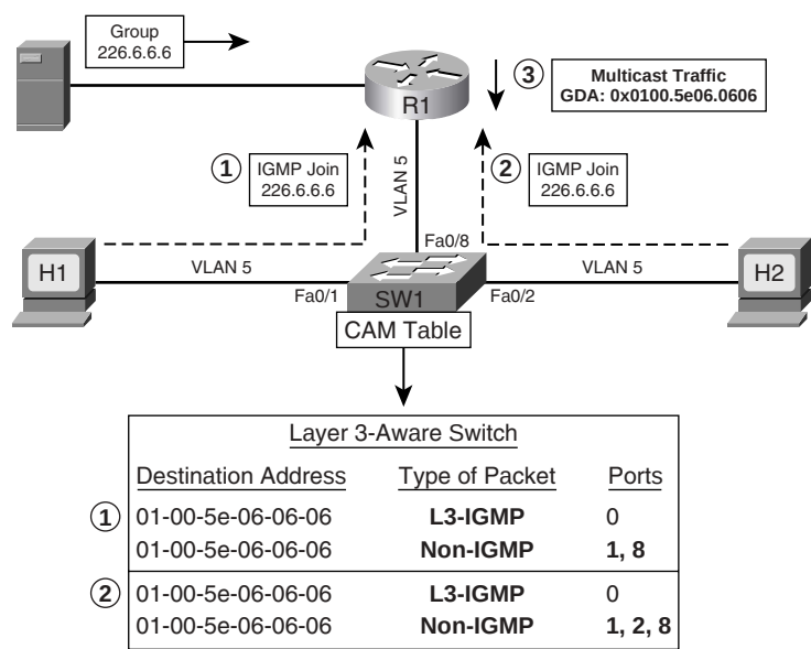
Figure 19-20 Joining a Group Using IGMP Snooping and CAM Table Entries
