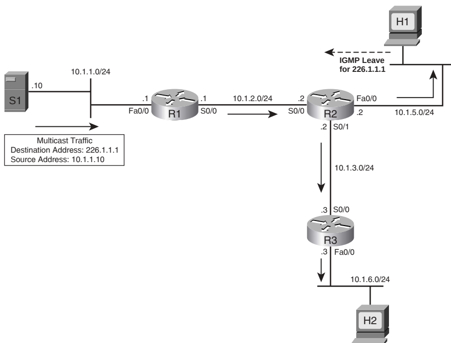
Figure 20-7 Direct Link Between R1 and R3 Is Down and Host H1 Sends an IGMP Leave Message
