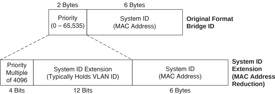
Figure 3-1 IEEE 802.1D STP Bridge ID Formats
