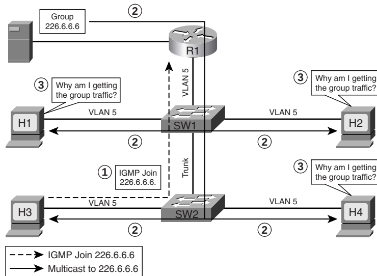
Figure 19-16 Switches Flood Multicast Traffic
