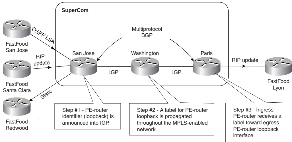
Figure C-26 PN Packet Forwarding—Preparatory Steps
