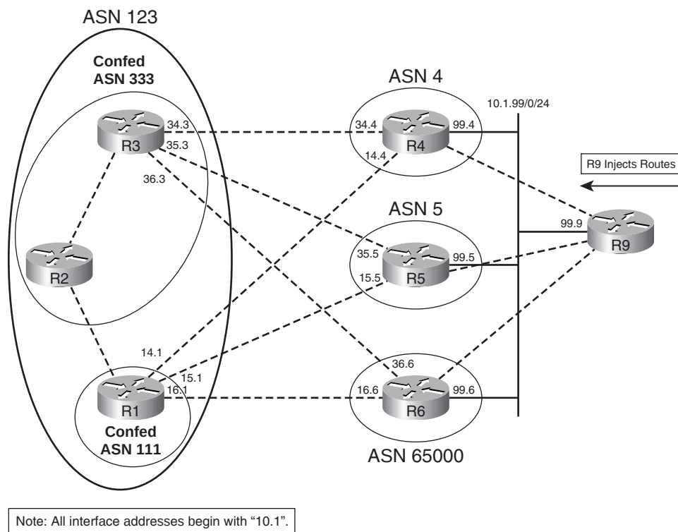
Figure 13-4 Network Used for AS_PATH Filter Examples
