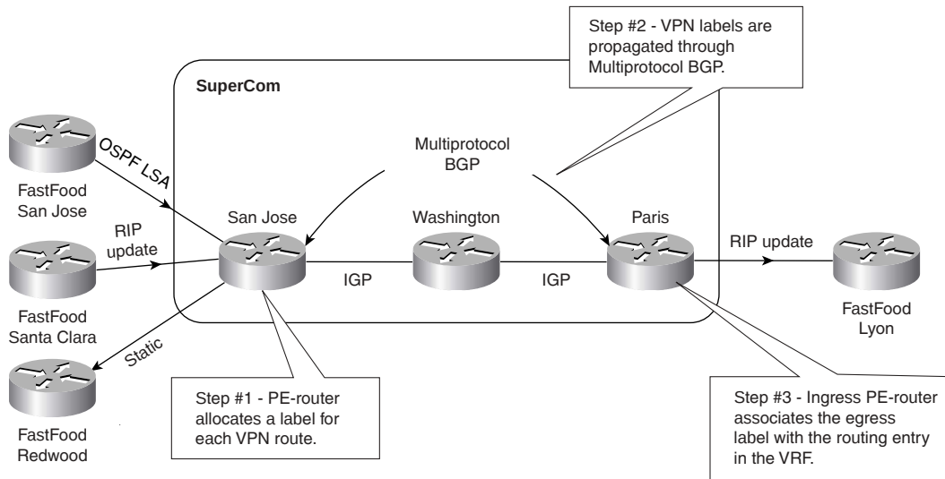
Figure C-27 VPN Label Allocation
