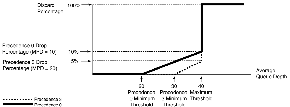
Figure 15-10 Example WRED Profiles for Precedences 0 and 3
