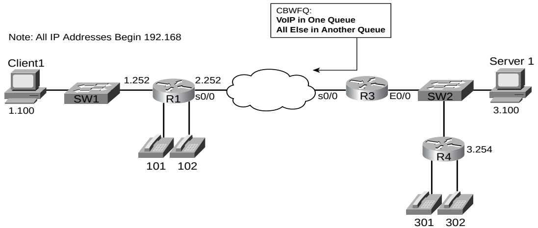
Figure 15-5 Network Used with CBWFQ and LLQ Configuration Examples
