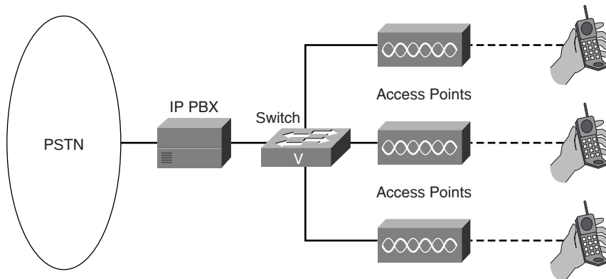
Figure 23-5 Voice over Wireless LAN Configuration
