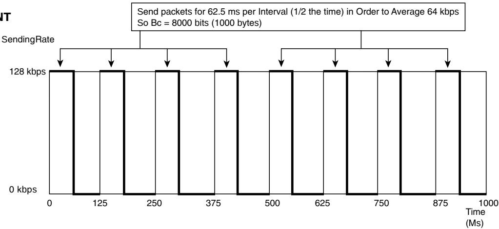
Figure 16-1 Mechanics of Traffic Shaping—128-kbps Access Rate, 64-kbps Shaped Rate
