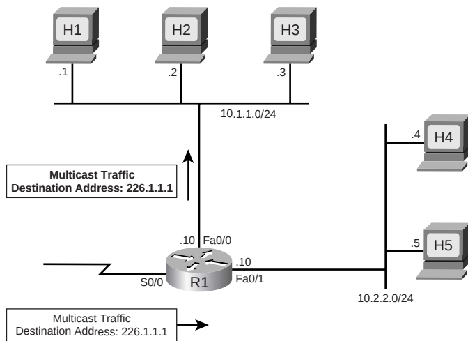
Figure 19-10 R1 Forwarding Traffic for Group 226.1.1.1 on Its Fa0/0 Interface
