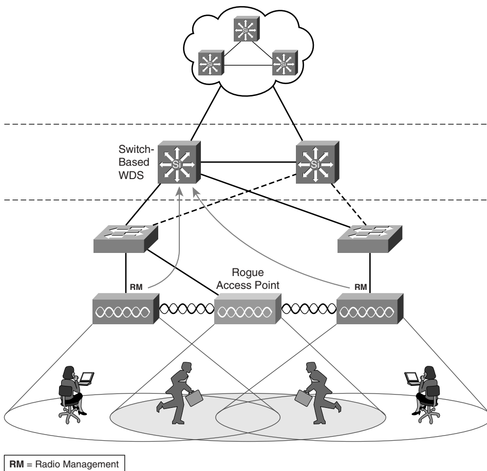
Figure 23-2 Cisco Wireless LAN Threat Defense Solution
