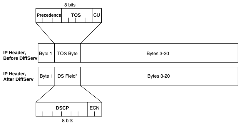
Figure 14-1 IP ToS Byte and DS Field Compared
