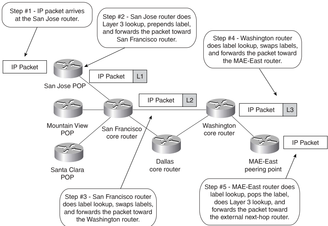
Figure C-5 MPLS Label Imposition and Forwarding
