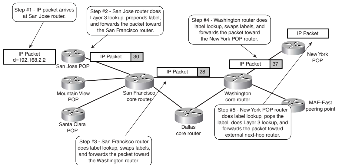
Figure C-15 Double Lookup in New York POP Router
