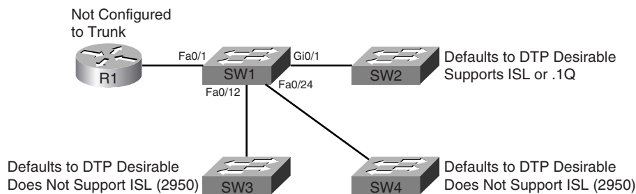
Figure 2-4 Trunking Configuration Reference for Example 2-5
