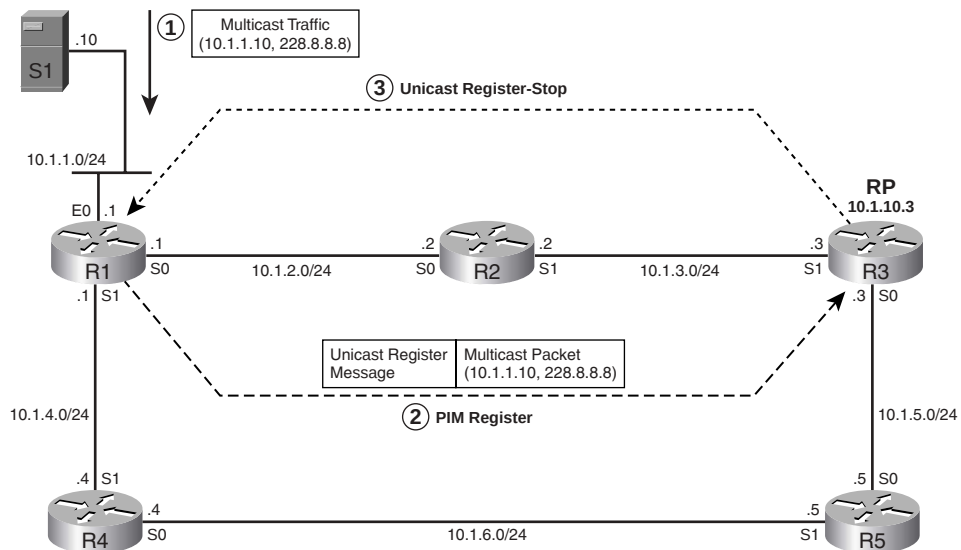
Figure 20-13 Source Registration Process when RP Has Not Received a Request for the Group from Any PIM-SM Router
