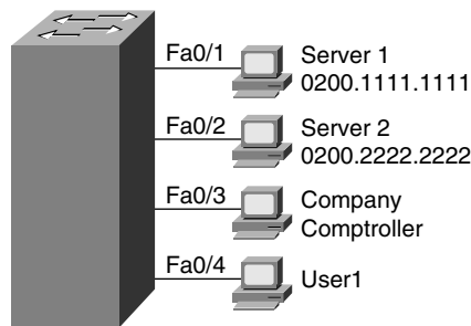
Figure 21-3 Port Security Configuration Example
