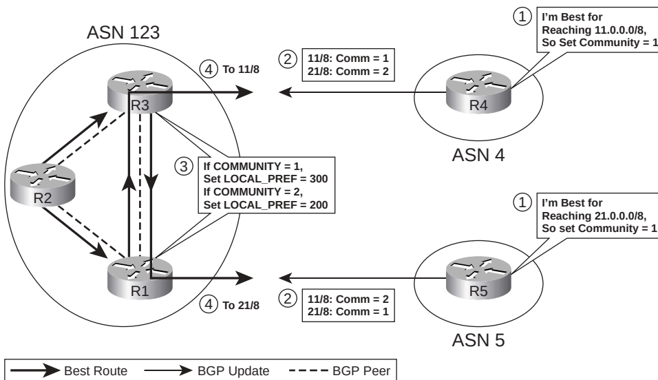
Figure 13-12 Using COMMUNITY to Augment Routing Policies
