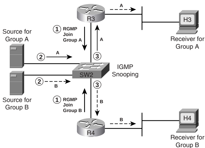
Figure 19-23 More Efficient Forwarding with RGMP Added to IGMP Snooping
