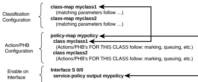
Figure 14-4 MQC Commands and Their Correlation
