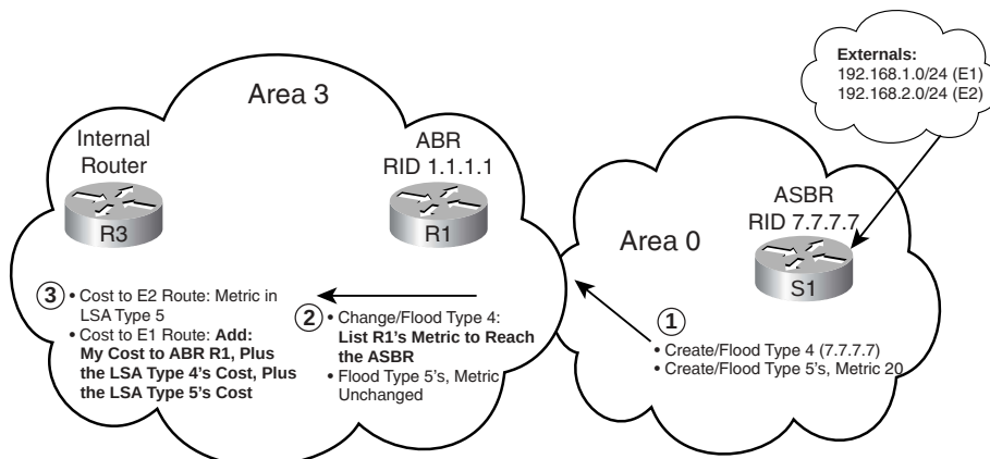
Figure 10-9 LSA Types 4 and 5 Propagation and the Effect on Type 1 External Routes
