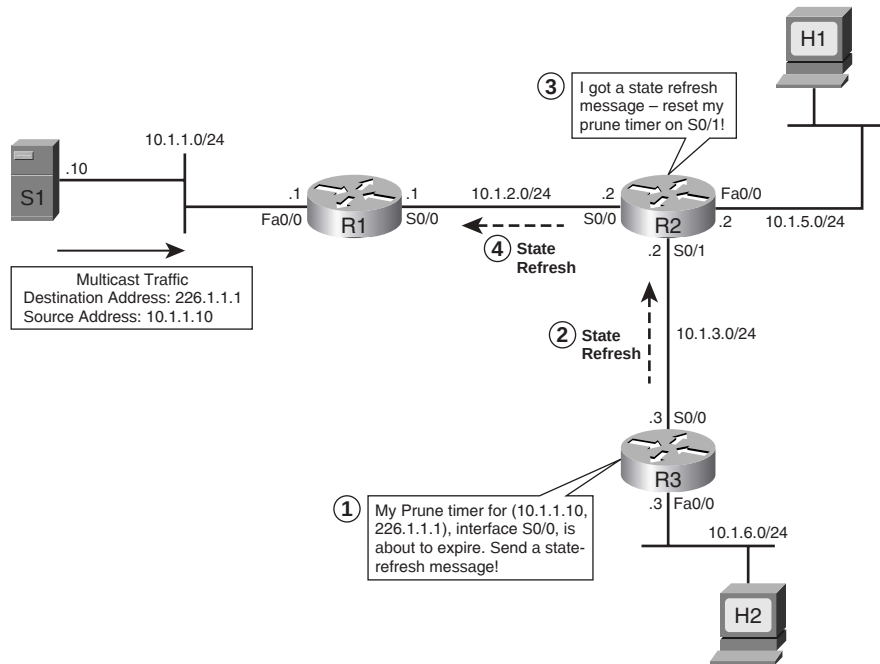
Figure 20-9 How PIM-DM Version 2 Uses State Refresh Messages
