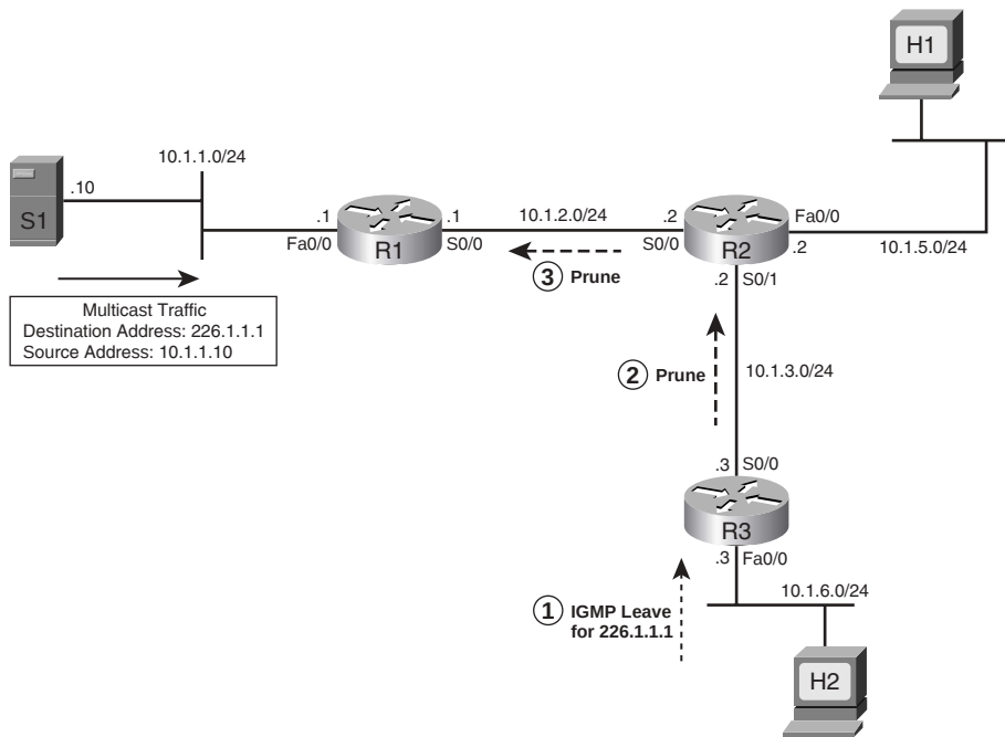
Figure 20-8 R3 and R2 Sending Prune Messages
