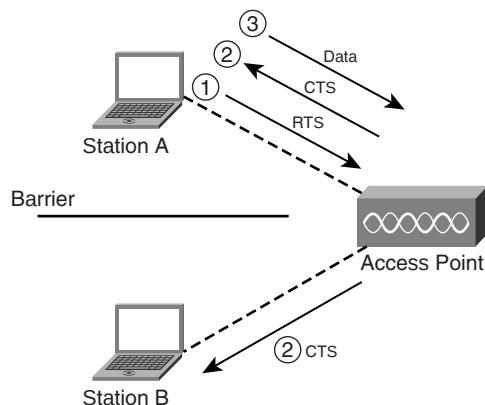
Figure 22-8 Hidden-Node Problem in Wireless LANs
