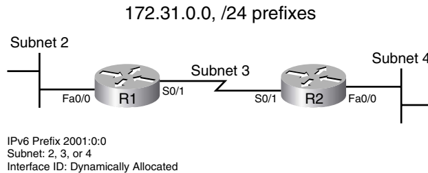
Figure 4-9 Sample Dual-Stack IPv4/IPv6 Network
