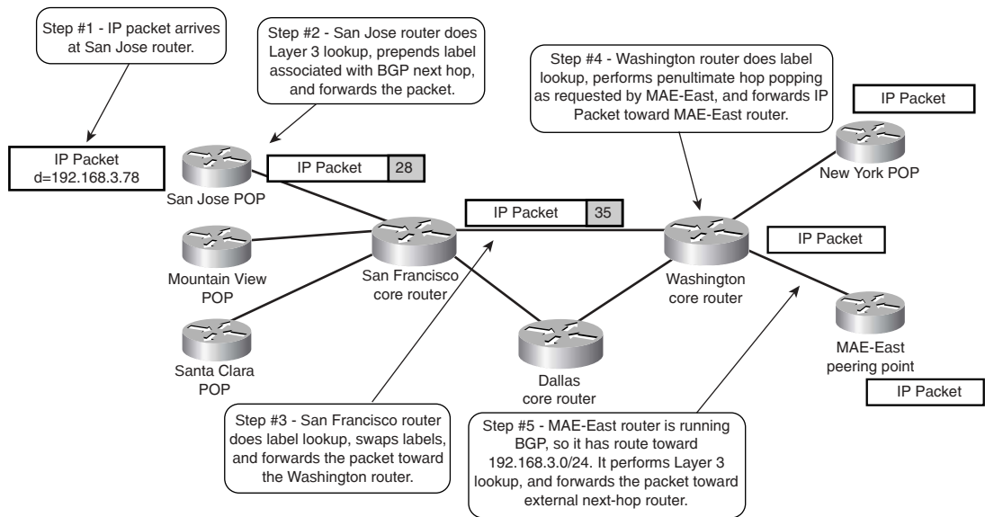
Figure C-18 Packet Propagation Toward BGP Destination in MPLS-enabled Network
