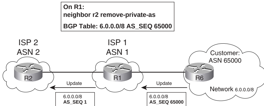
Figure 13-9 Typical Use of Private ASNs and the neighbor remove-private-as Command
