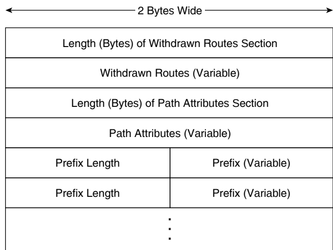
Figure 12-5 BGP Update Message Format
