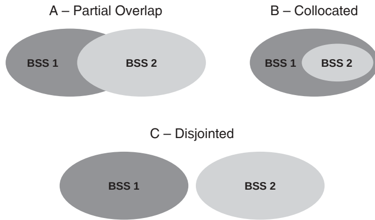
Figure 22-2 Various 802.11 Radio Cell Configurations
