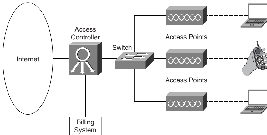
Figure 23-6 Typical Public Wireless LAN Configuration
