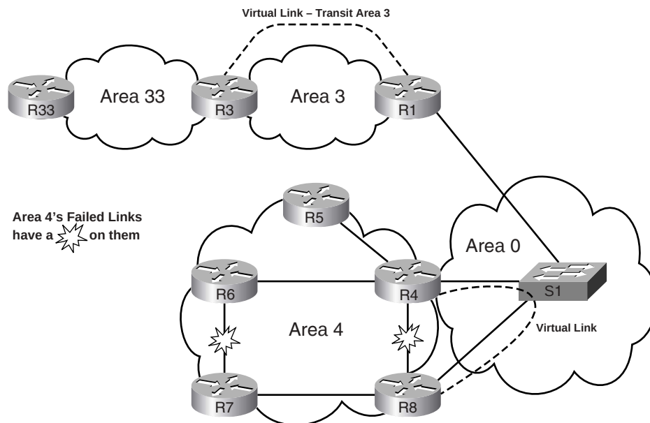
Figure 10-10 The Need for Virtual Links
