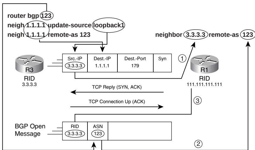
Figure 12-3 BGP Neighbor Parameter Checking
