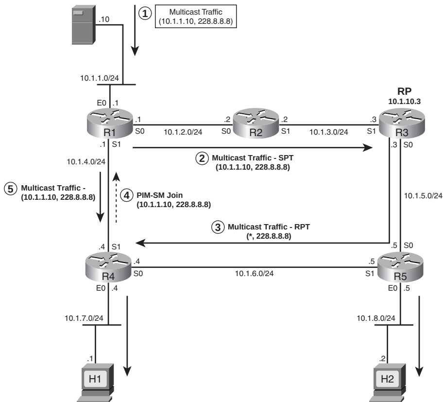
Figure 20-17 R4 Initializing Switchover from RPT to SPT by Sending a PIM-SM Join to R1
