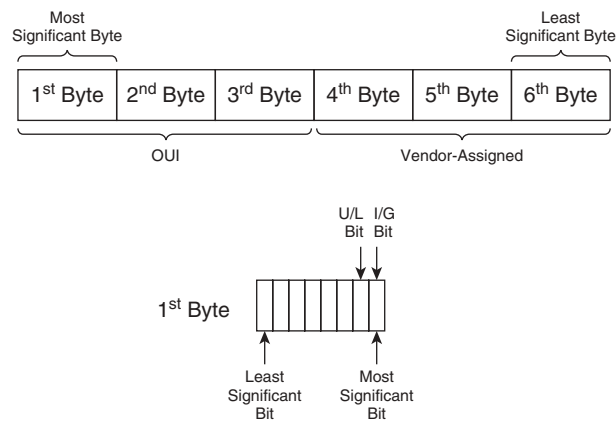
Figure 1-5 Ethernet Address Format
