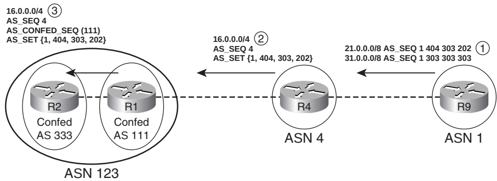
Figure 13-3 AS_SET and AS_CONFED_SEQ Example
