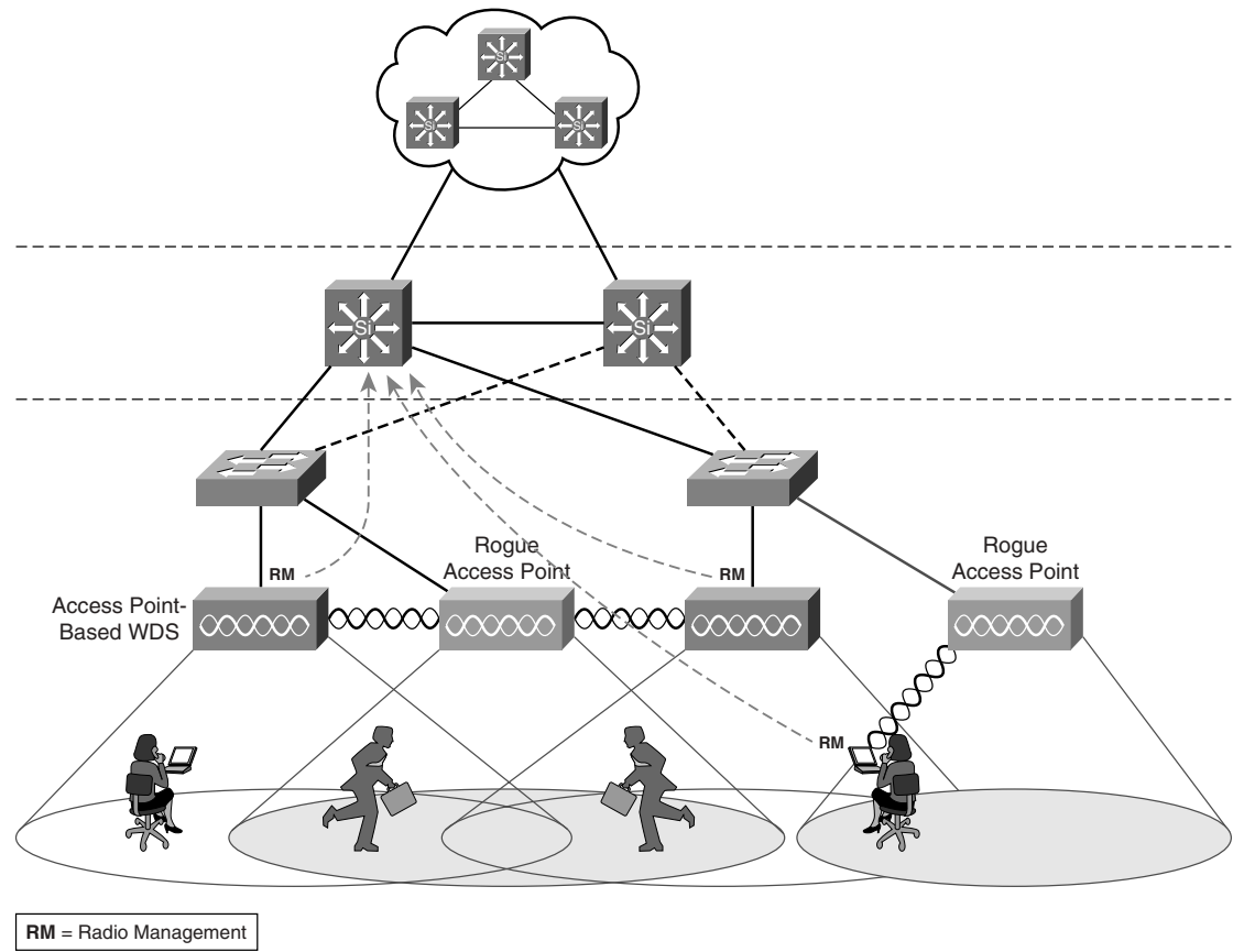
Figure 23-3 Cisco IDS with Client Scanning
