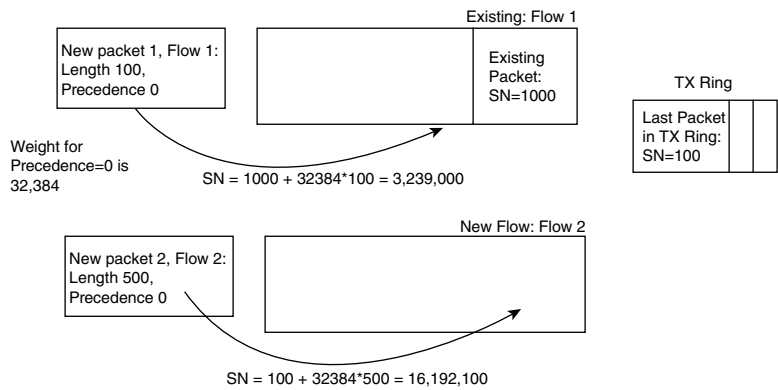
Figure 15-3 WFQ Sequence Number Assignment Example
