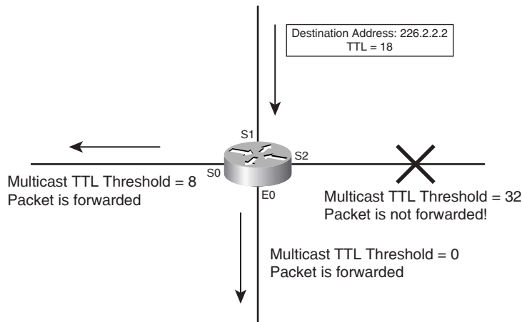
Figure 20-5 Multicast Scoping Using TTL Thresholds
