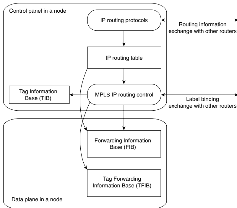
Figure C-6 Edge-LSR Architecture Using Cisco IOS Terms
