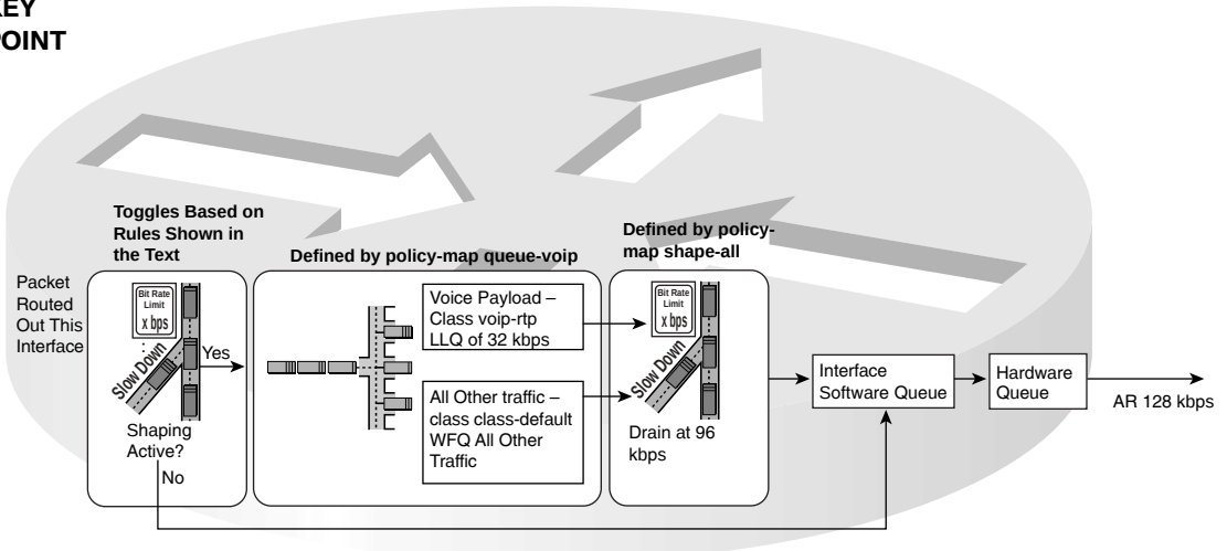
Figure 16-4 Interaction Between Shaping Policy Map shape-all and Queuing Policy Map queue-voip
