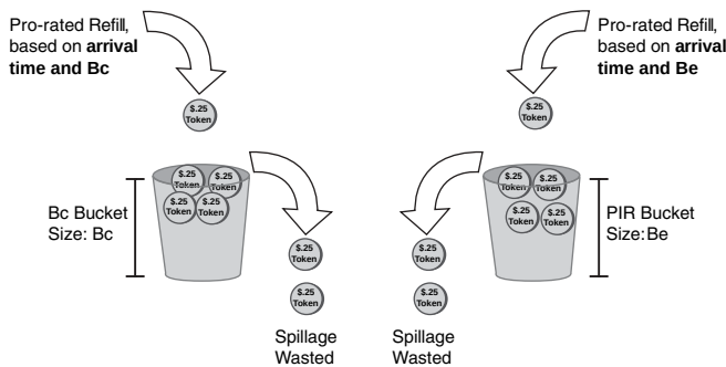
Figure 16-7 Refilling CIR and PIR Dual Token Buckets
