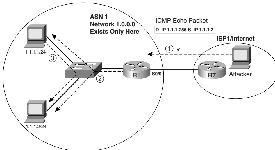
Figure 21-9 Smurf Attack
