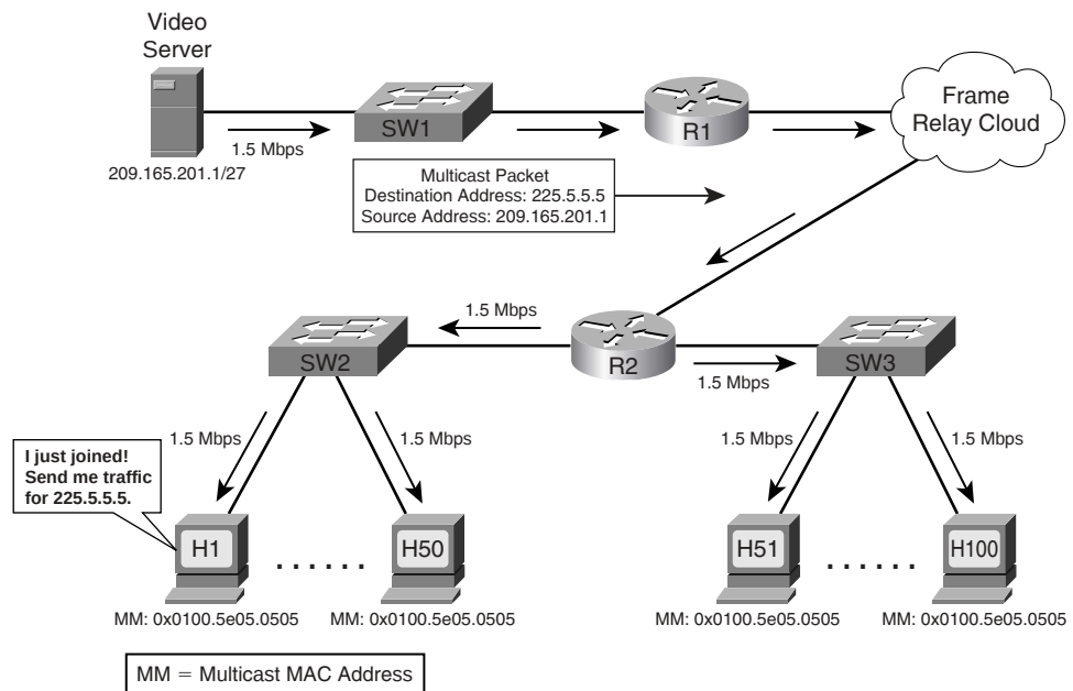
Figure 19-5 Multicasting Is Scalable
