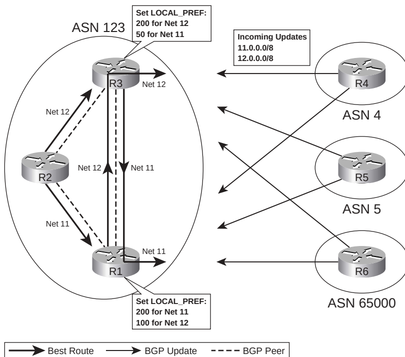
Figure 13-8 Typical Use of LOCAL_PREF to Influence Exit Point from AS 123.
