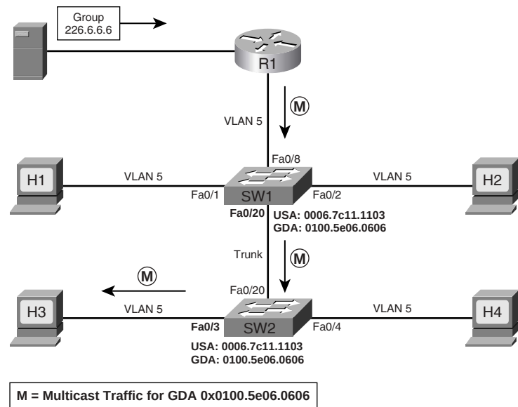
Figure 19-18 Switches Map GDA to Port Numbers and Don't Flood All the Hosts in a Broadcast Domain
