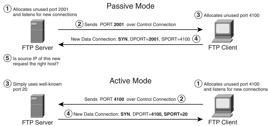
Figure 6-5 Passive and Active FTP Behavior
