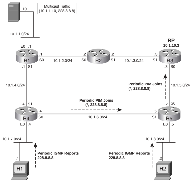
Figure 20-16 Host H2 Sends an IGMP Join Message
