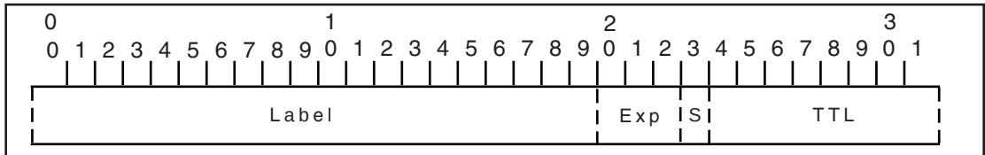
Figure C-12 MPLS Label Stack Header
