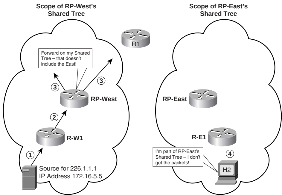
Figure 20-23 The Anycast RP Problem (Later Solved with MSDP)
