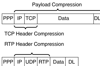
Figure 17-4 Fields Compressed with Compression Features
