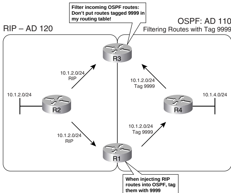
Figure 11-6 Filtering with Reliance on Route Tags
