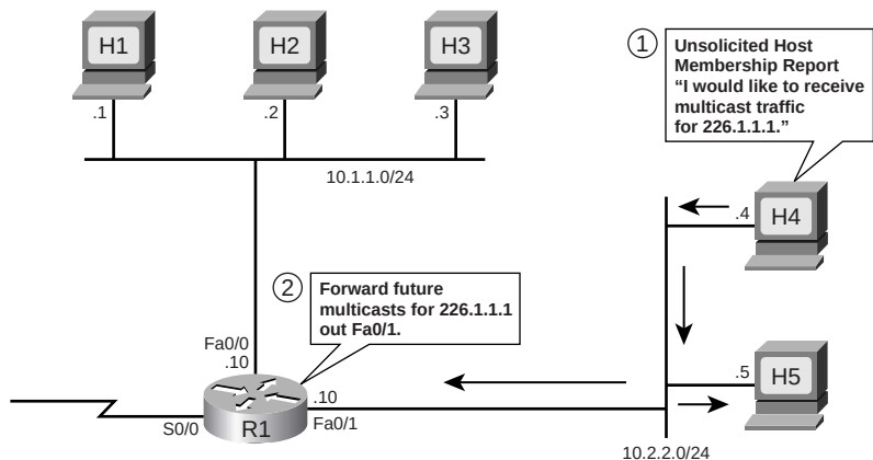
Figure 19-11 H4 Sends IGMPv1 Unsolicited Host Membership Report
