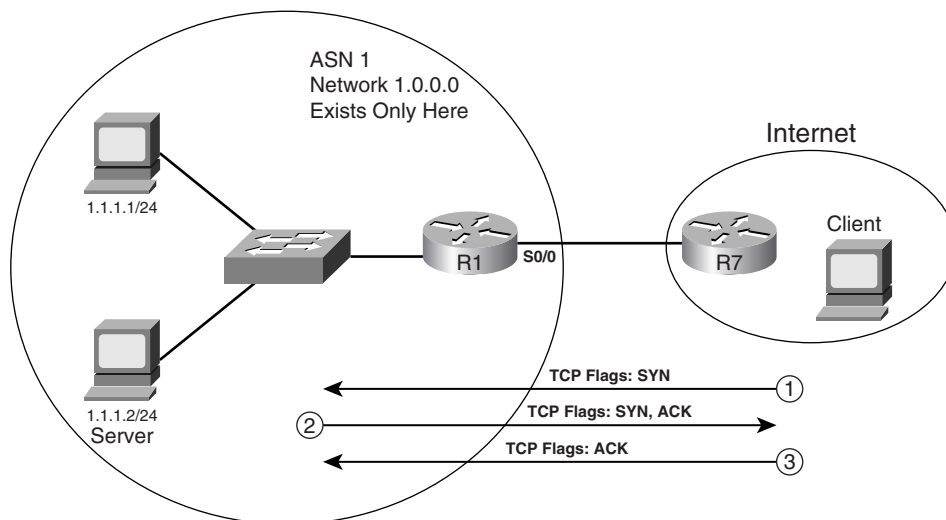
Figure 21-10 Example Network: TCP Clients in the Internet
