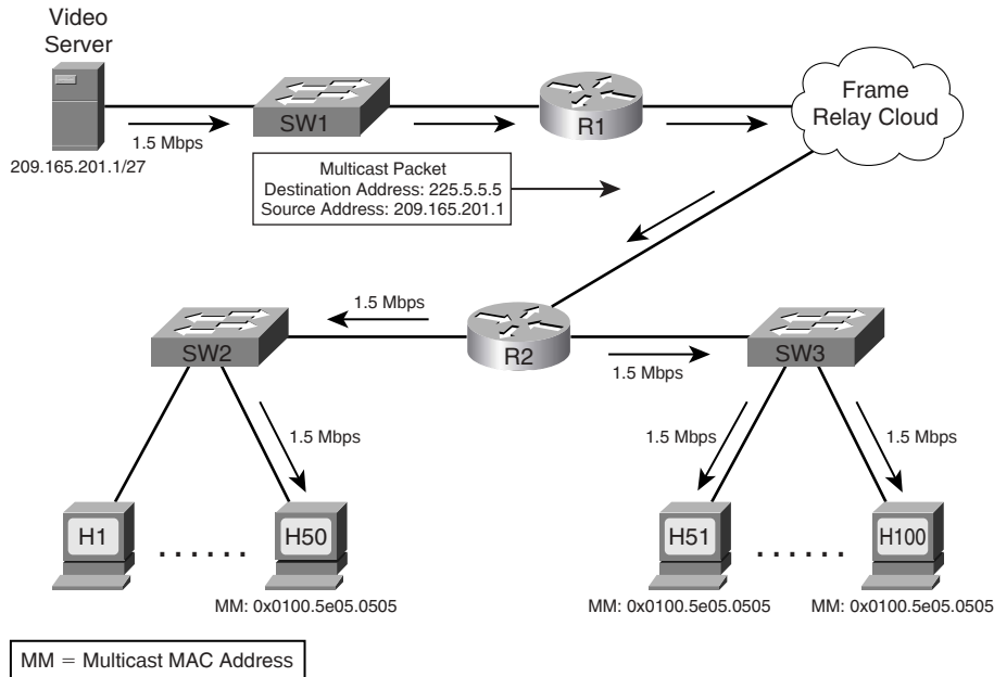
Figure 19-4 How Multicast Delivers Traffic to Selected Users
