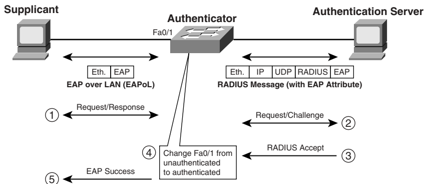
Figure 21-7 802.1X for LAN User Authentication
