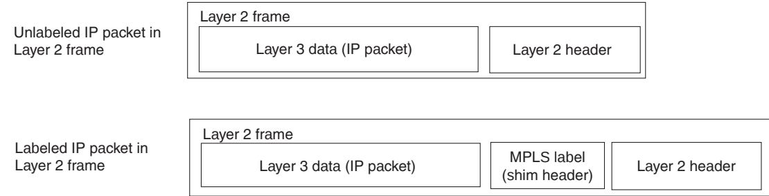
Figure C-11 Position of the MPLS Label in a Layer 2 Frame
