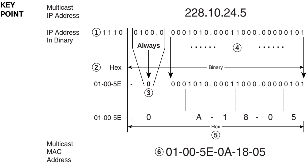
Figure 19-6 Calculating a Multicast Destination MAC Address from a Multicast Destination IP Address
