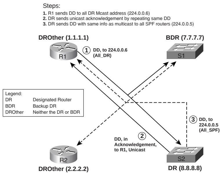
Figure 10-2 DR Optimization on a LAN
