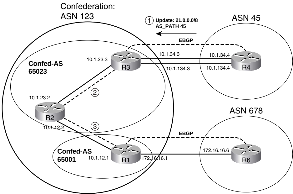
Figure 12-9 Internetwork Topology with Confederations in ASN 123
