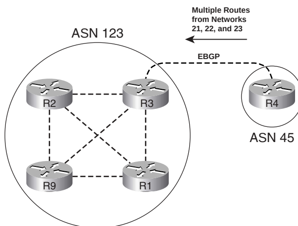
Figure 13-1 iBGP Full Mesh in AS 123 with Routes Learned from AS 45
