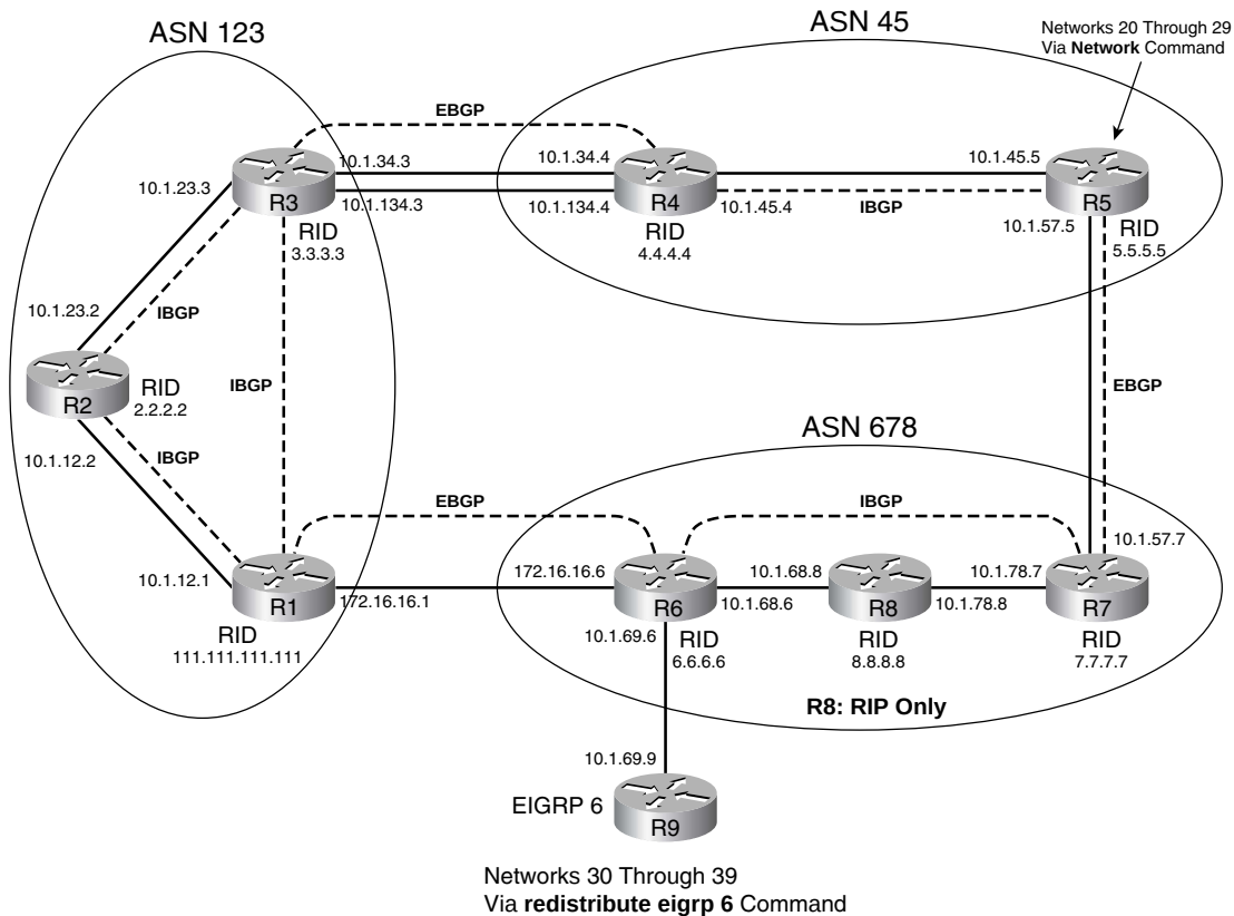
Figure 12-4 Sample BGP Network, with IP Addresses
