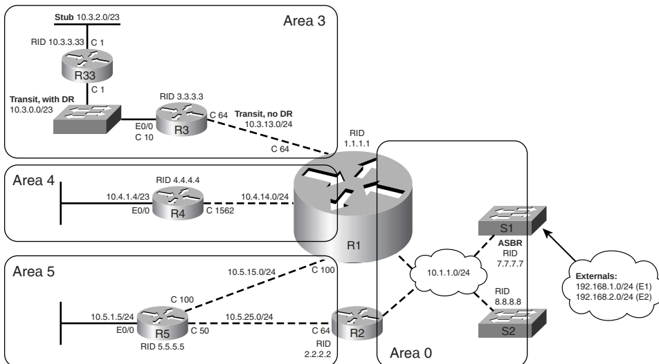
Figure 10-6 Network Used in LSA Examples
