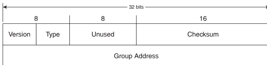
Figure 19-7 IGMPv1 Message Format
