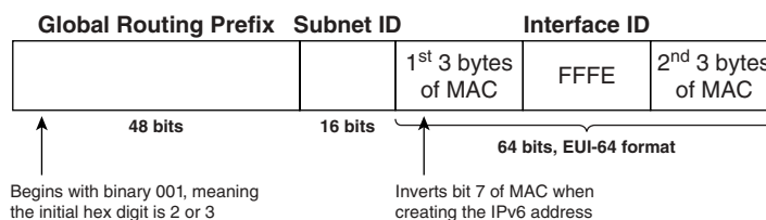
Figure 4-8 Aggregatable Global Address Format
