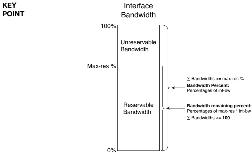
Figure 15-6 Bandwidth Percent and Bandwidth Remaining Percent Concepts
