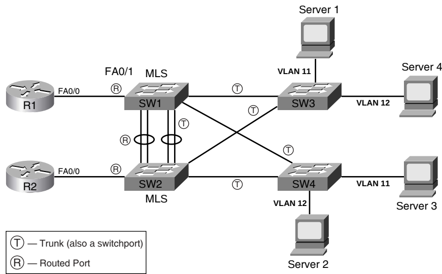
Figure 7-4 Physical Topology: Example Using MLS
