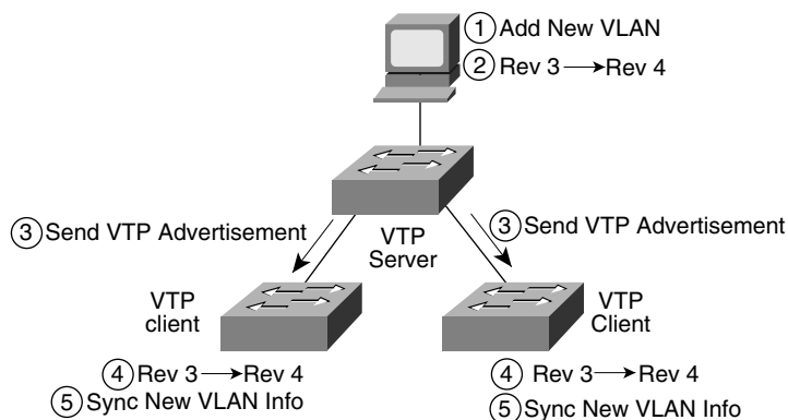
Figure 2-2 VTP Revision Number Basic Operation
