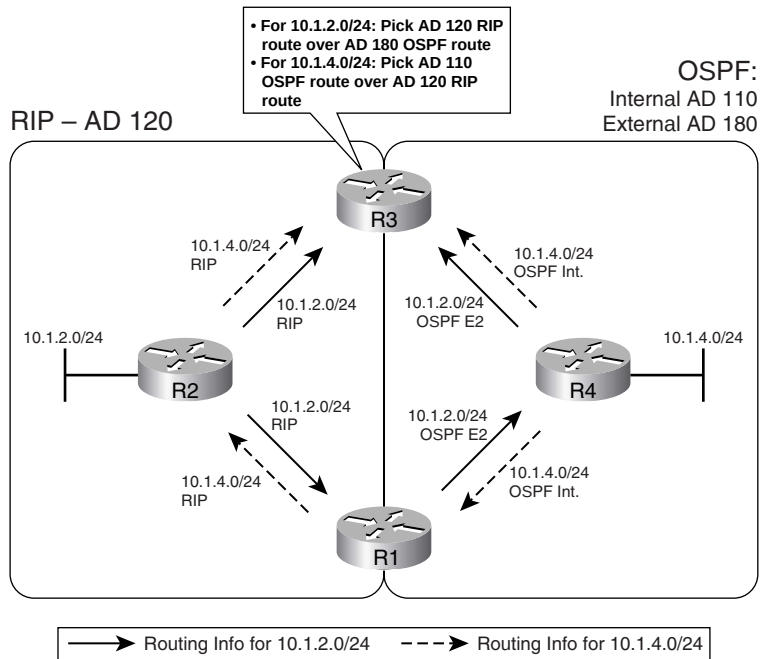
Figure 11-5 The Effect of Differing ADs for Internal and External Routes
