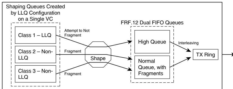
Figure 18-5 Interface Dual FIFO Queues with FRTS Plus FRF.12
