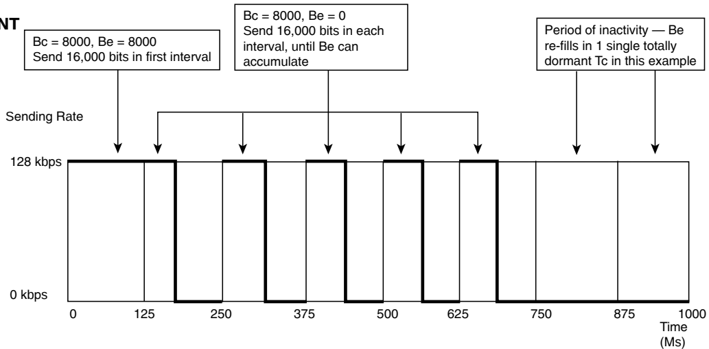
Figure 16-2 Bc and Be, After a Period of Inactivity
