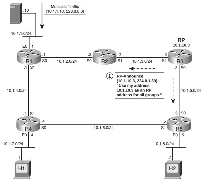
Figure 20-19 R3 Sends RP-Announce Messages
