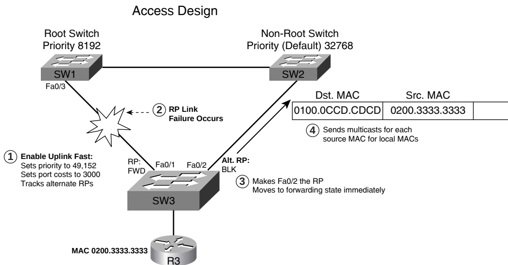
Figure 3-7 UplinkFast Operations
