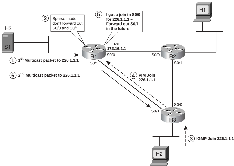
Figure 20-4 R1 Forwarding a Multicast Packet Using a Sparse-Mode Routing Protocol
