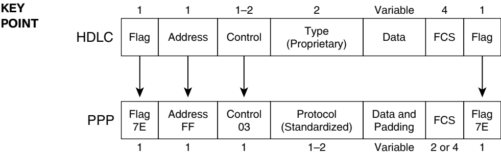
Figure 17-2 HDLC and PPP Framing Compared
