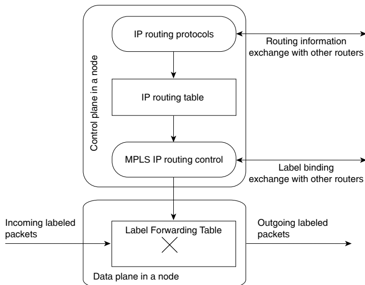
Figure C-3 Basic Architecture of an MPLS Node Performing IP Routing
