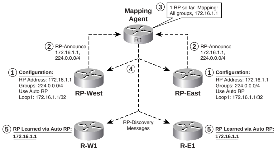
Figure 20-22 Learning the RP Address with Anycast RP
