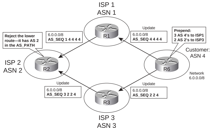
Figure 13-10 Options for Prepending ASNs
