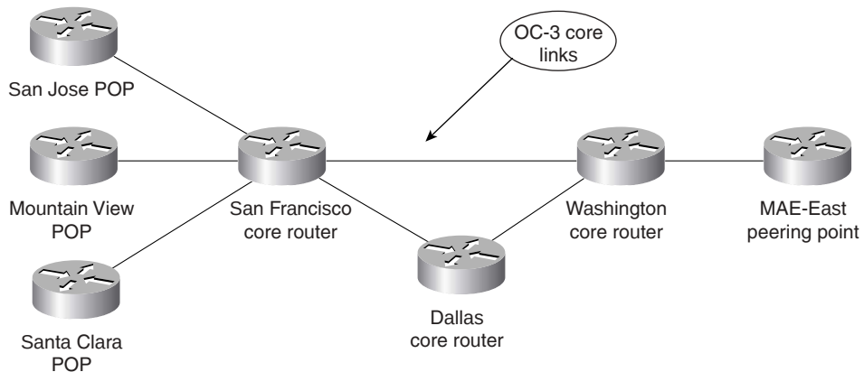
Figure C-2 Sample Network that Would Benefit from Traffic Engineering
