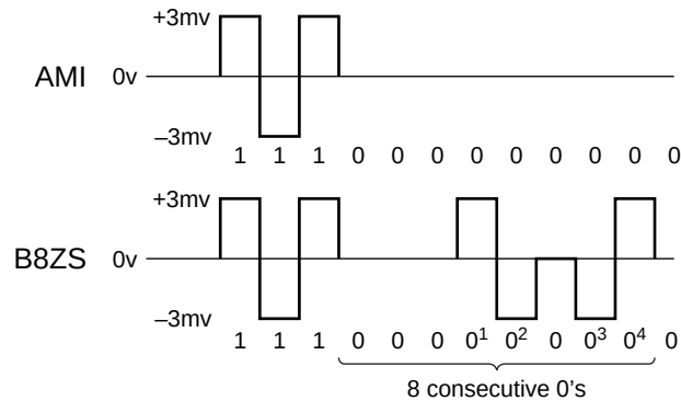
Figure 17-1 Comparing AMI and B8ZS
