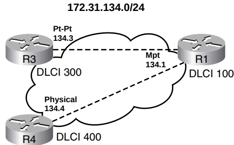
Figure 7-3 Frame Relay Topology for Frame Relay InARP Examples
