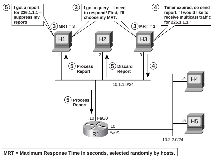
Figure 19-9 IGMPv1 Solicited Host Membership Report and Report Suppression Processes
