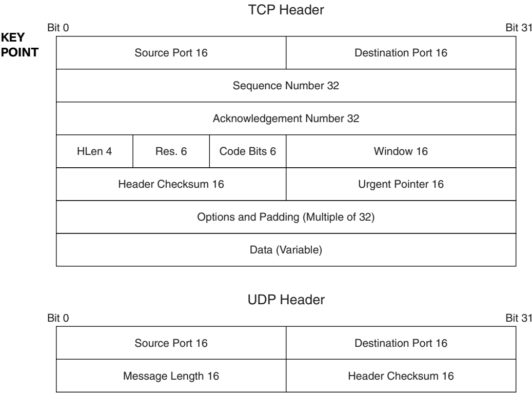
Figure 6-1 TCP and UDP Headers
