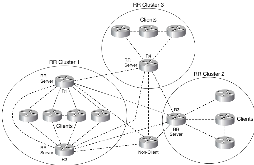
Figure 12-11 Multiple RR Clusters with Full Mesh Among RRs and Nonclients
