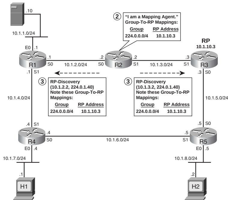
Figure 20-20 R2 Creates Group-to-RP Mappings and Sends Them in RP-Discovery Messages
