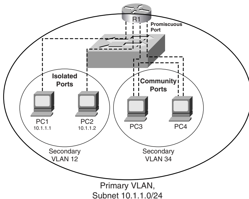
Figure 21-8 Private VLAN Allowed Flows
