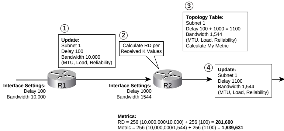
Figure 9-3 EIGRP Update and Computing the Metric
