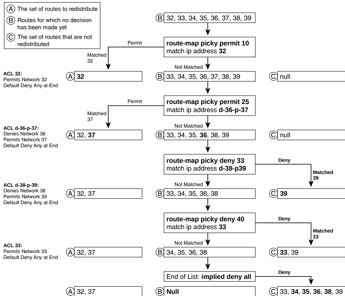
Figure 11-1 Route Map Logic Example
