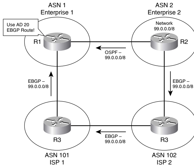
Figure 12-6 The Need for BGP Backdoor Routes
