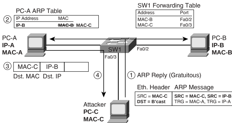
Figure 21-5 Man-in-the-Middle Attack Using Gratuitous ARP's
