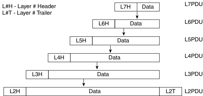
Figure 24-3 OSI Encapsulation and Protocol Data Units
