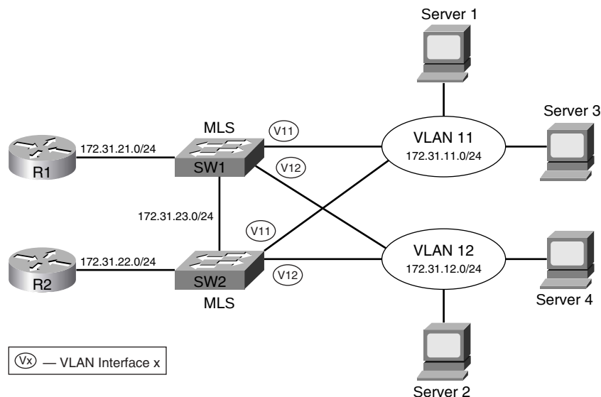
Figure 7-5 Layer 3 Topology View: Example Using MLS
