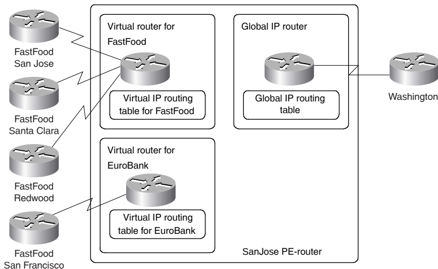
Figure C-20 Virtual Routers Created in a PE-router
