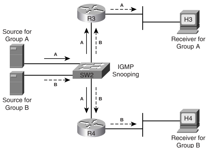
Figure 19-22 IGMP Snooping Without RGMP
