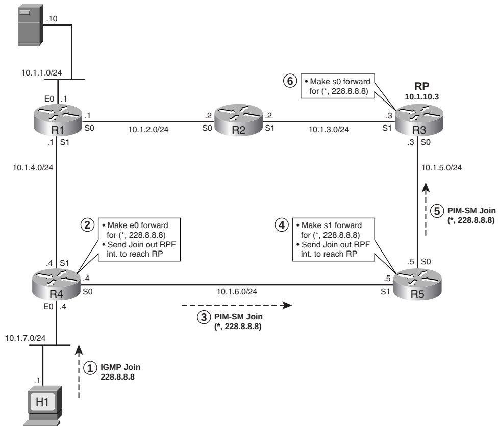
Figure 20-14 Creating a Shared Tree for (*,228.8.8.8)
