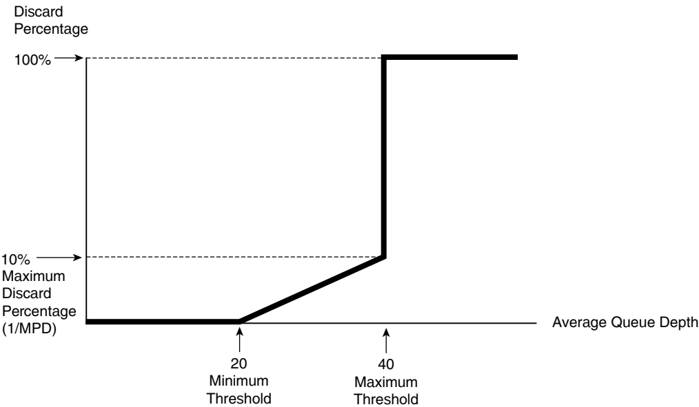
Figure 15-9 WRED Discard Logic with Defaults for IPP 0
