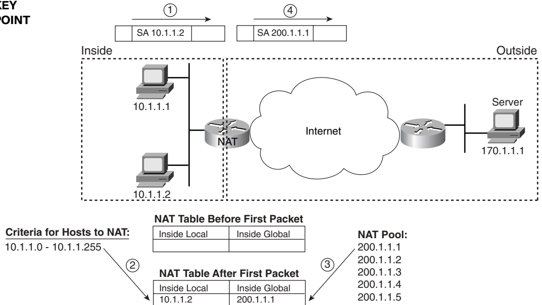
Figure 4-7 Dynamic NAT
