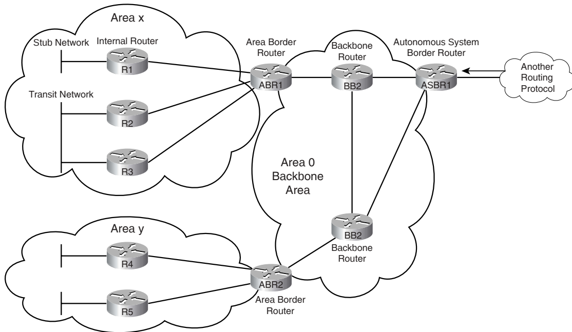
Figure 10-5 OSPF Design Terminology
