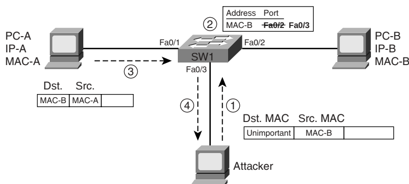
Figure 21-2 Claiming to Use Another Host's MAC Address
