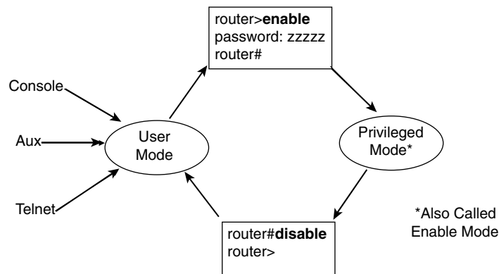
Figure 21-1 Router User and Enable Modes
