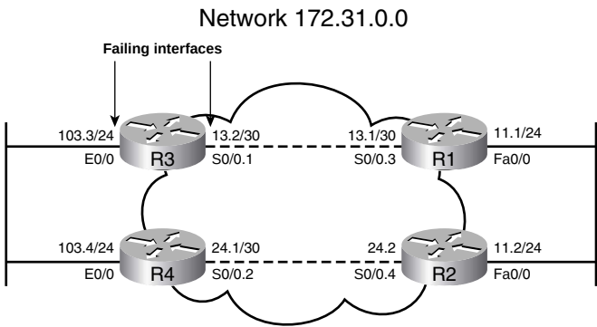
Figure 8-1 Sample Internetwork Used for Loop-Prevention Examples
