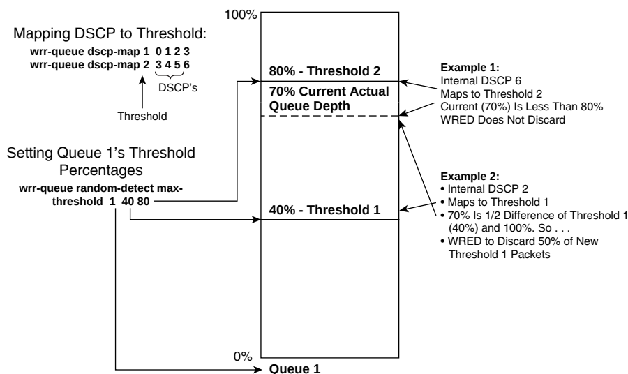
Figure 15-11 Cisco 3550 WRED Logic and Commands
