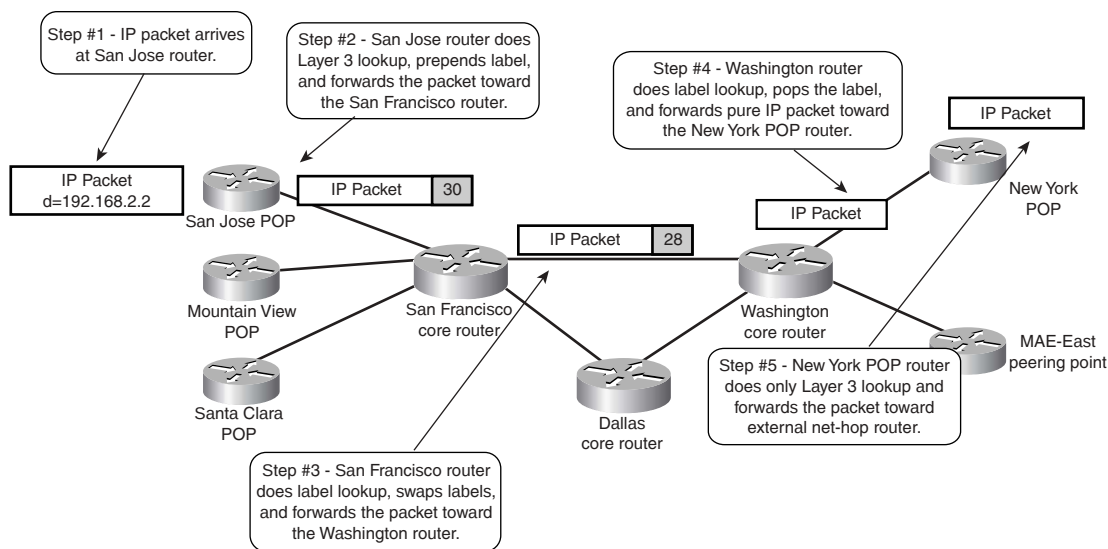
Figure C-16 Penultimate Hop Popping in the SuperNet Network
