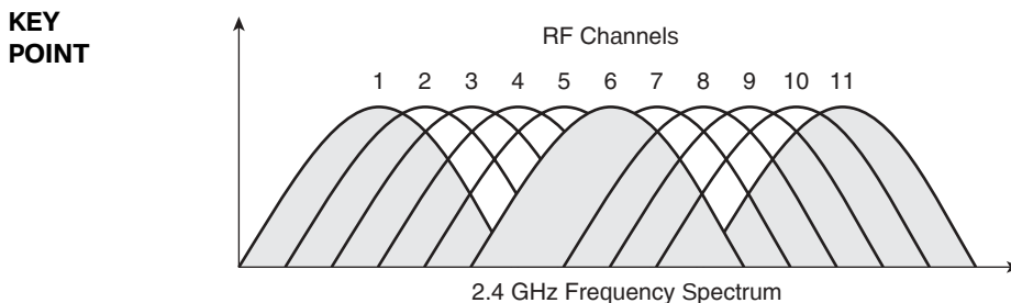
Figure 22-7 Overlapping 802.11 RF Channels in the 2.4-GHz Band
