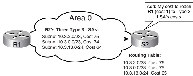
Figure 10-8 Representation of Area 3 Subnets as Type 3 LSAs in Area 0
