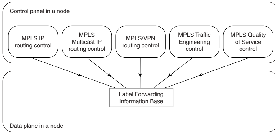
Figure C-7 Various MPLS Applications and Their Interactions
