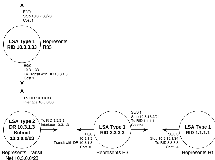
Figure 10-7 Graph of Type 1 and 2 LSAs for Area 3
