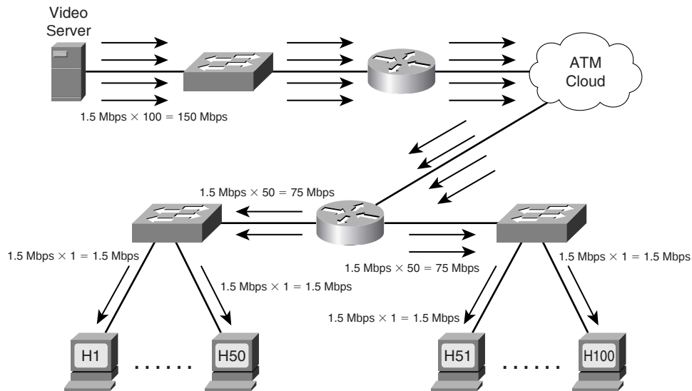
Figure 19-2 Unicast Does Not Scale to Large Numbers of Receivers
