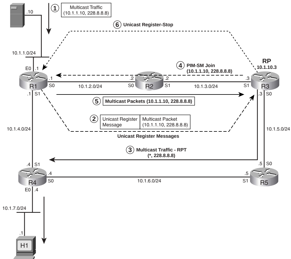
Figure 20-15 Source Registration when the RP Needs to Receive Packets Sent to that Group
