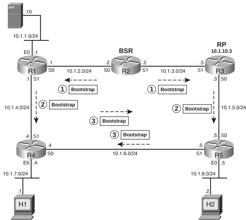
Figure 20-21 BSR Flooding Bootstrap Messages
