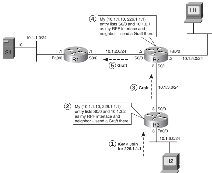
Figure 20-10 R3 and R2 Send Graft Messages
