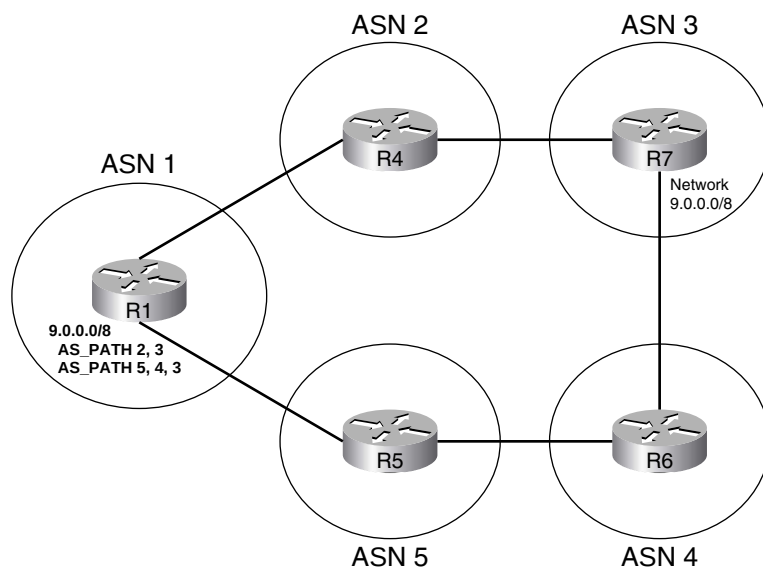
Figure 12-1 BGP AS_PATHs and Path Vector Logic
