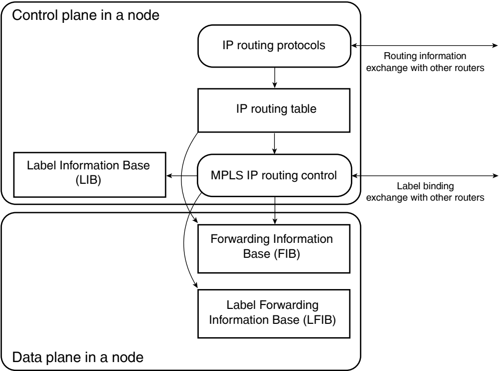
Figure C-8 Edge-LSR Architecture
