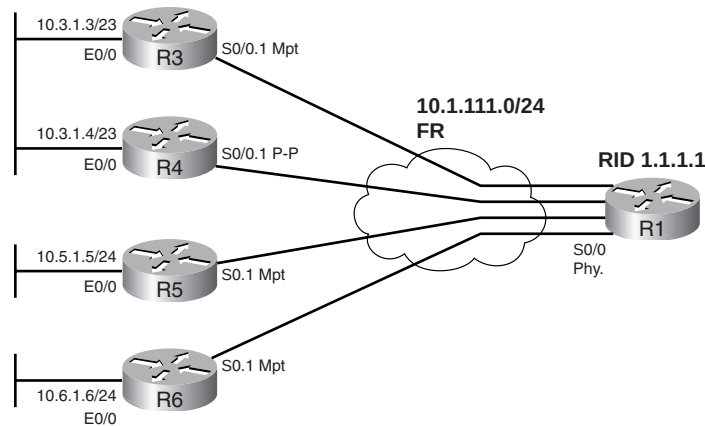
Figure 10-3 Network Used in the Frame Relay Priority and Network Type Example
