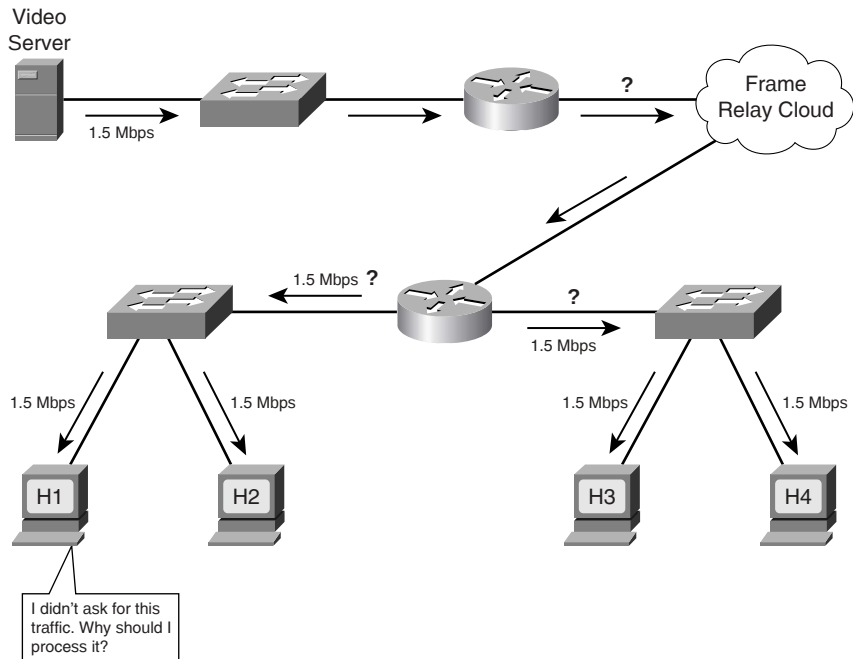
Figure 19-3 Broadcast Wastes Bandwidth and Increases Processing Load on CPU
