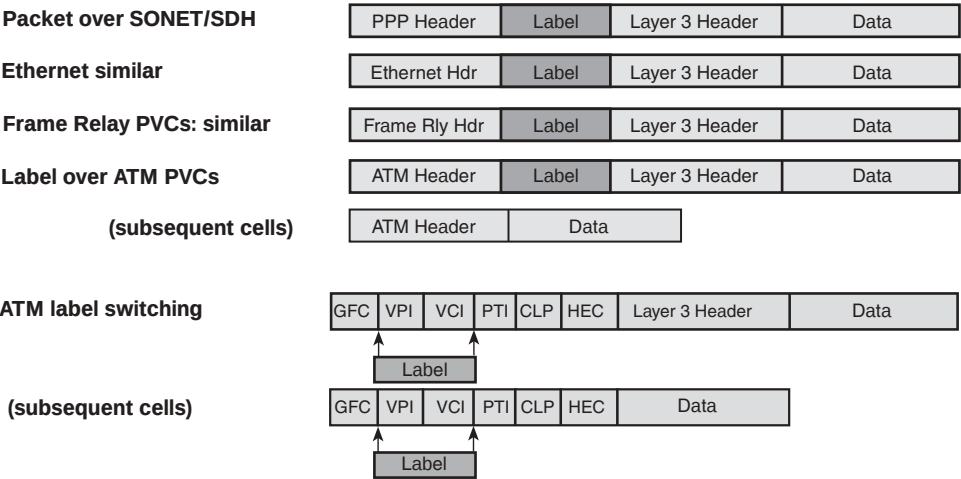
Figure C-13 Summary of MPLS Encapsulation Techniques
