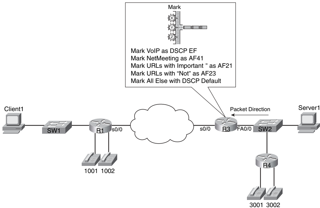
Figure 14-5 Sample Network for CB Marking Examples
