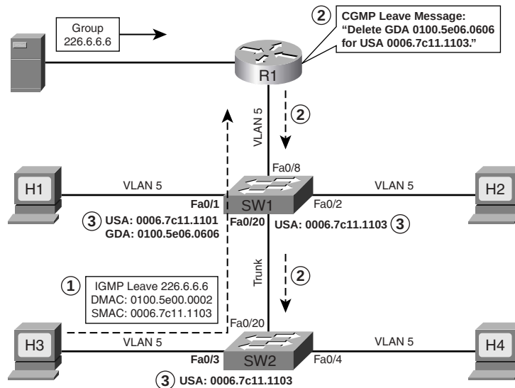
Figure 19-19 CGMP Leave Message Process
