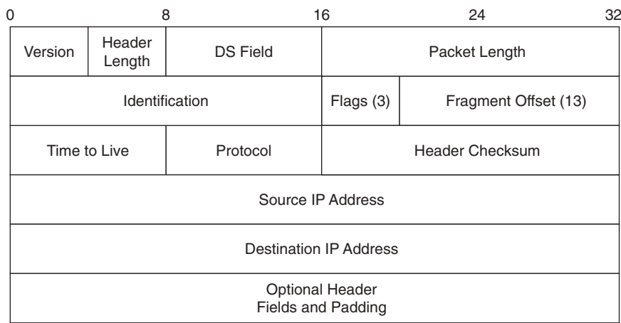
Figure 4-10 IP Header
