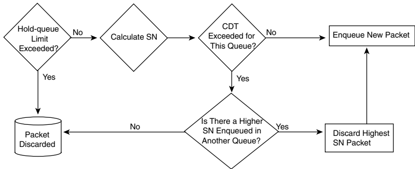
Figure 15-4 WFQ Modified Tail Drop and Congestive Discard Threshold
