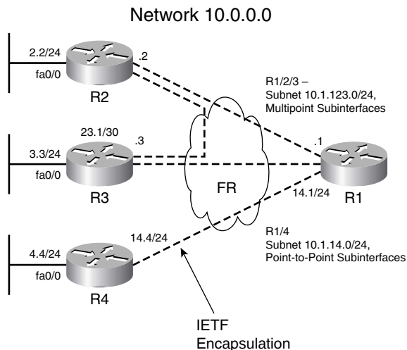
Figure 18-4 Sample FR Network for Configuration Examples
