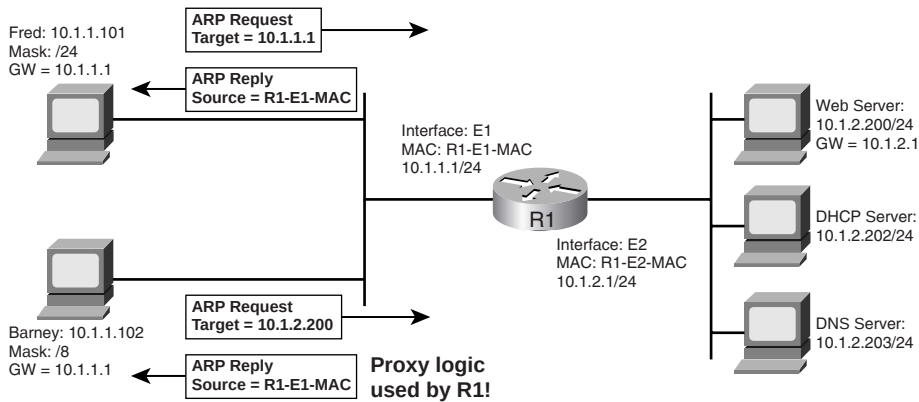
Figure 5-3 Comparing ARP and Proxy ARP
