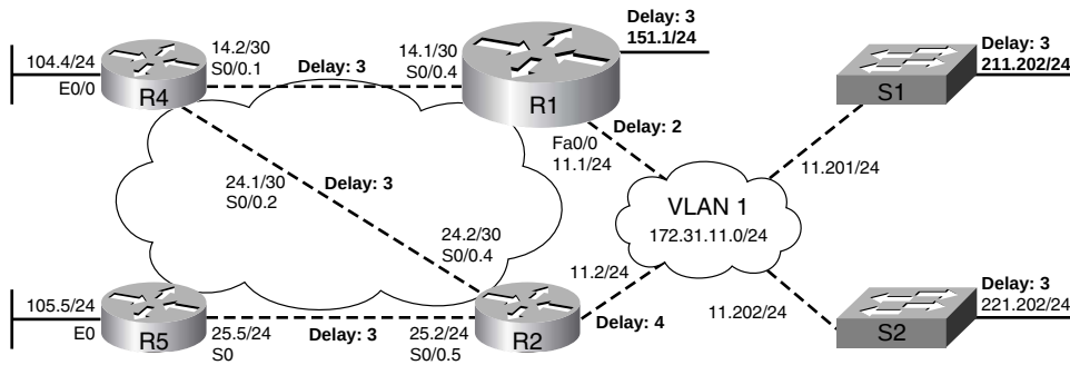
Figure 9-4 Network Used for EIGRP Convergence Examples
