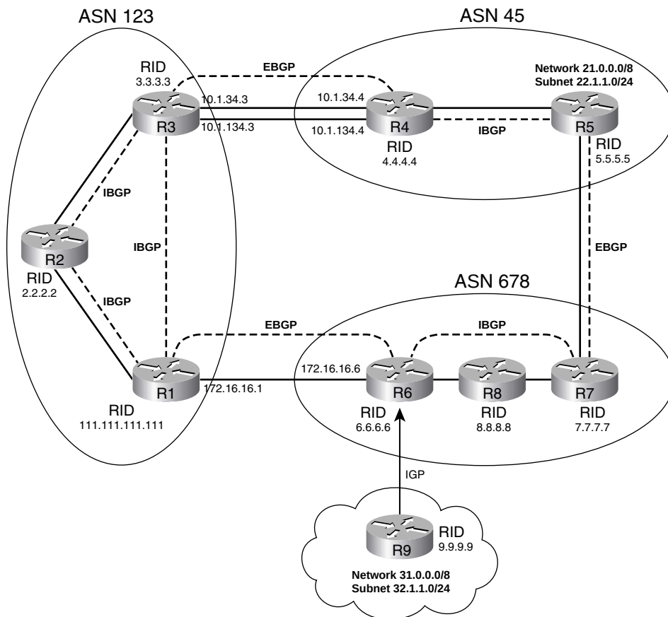
Figure 12-2 Sample Network for BGP Neighbor Configuration
