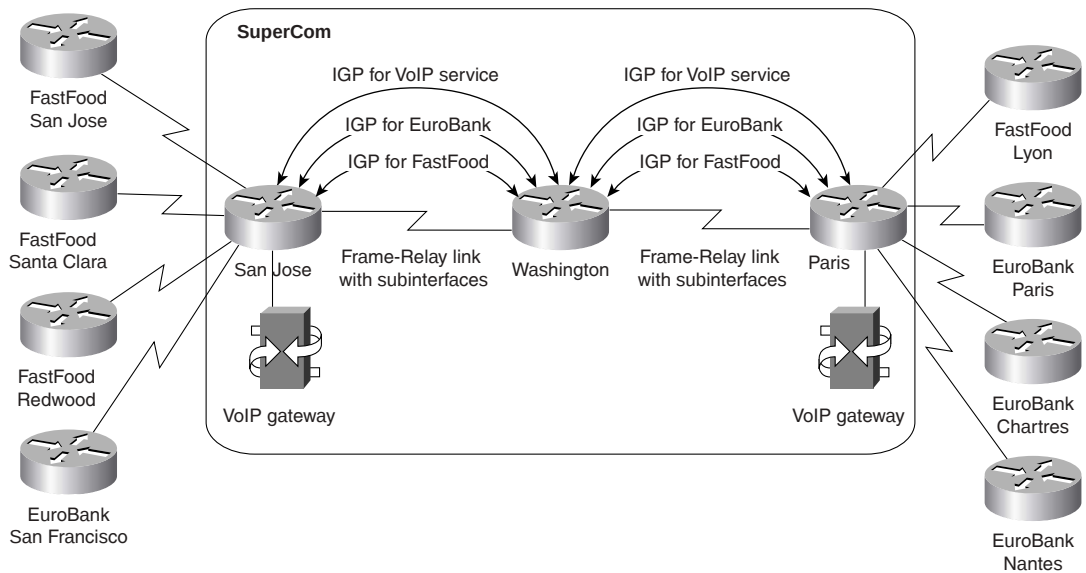
Figure C-23 SuperCom Network with One IGP per VPN
