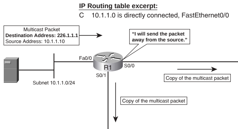
Figure 20-2 R1 Forwarding a Multicast Packet Using a Dense-Mode Routing Protocol
