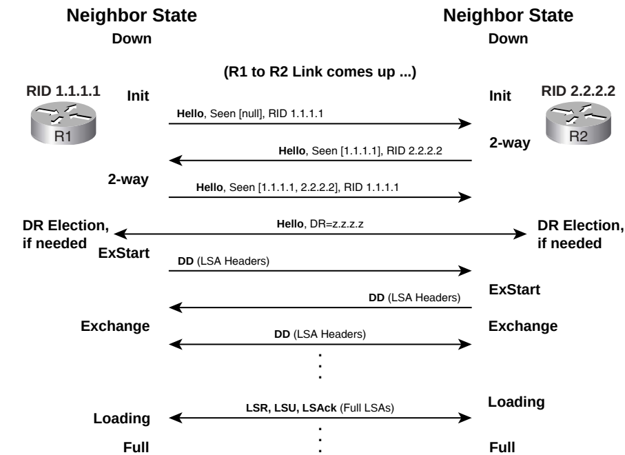
Figure 10-1 Overview of OSPF LSDB Exchange
