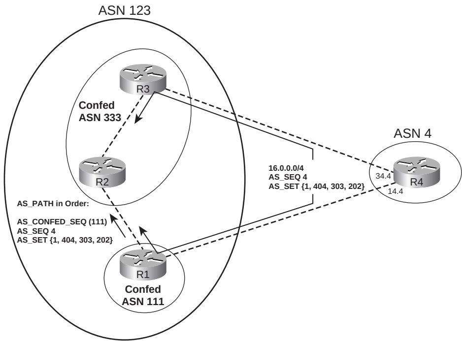
Figure 13-5 Generating AS_SET and AS_CONFED_SEQ
