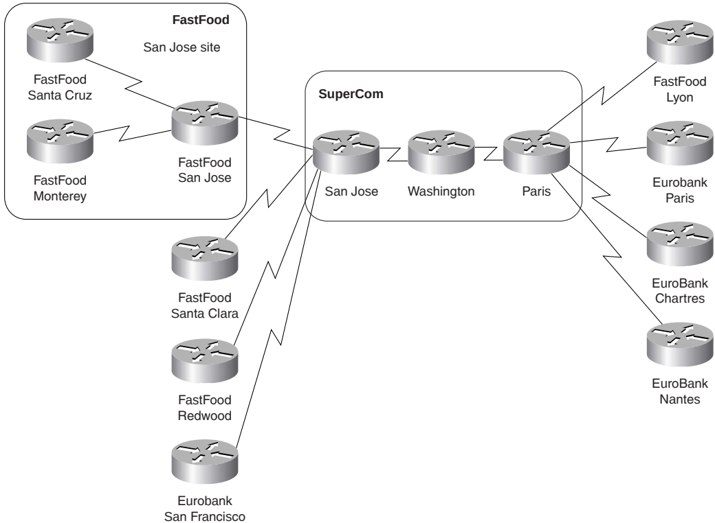
Figure C-19 SuperCom Network and Its Customers
