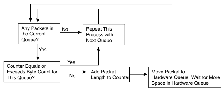
Figure 15-2 CQ Scheduling Logic for Current Queue
