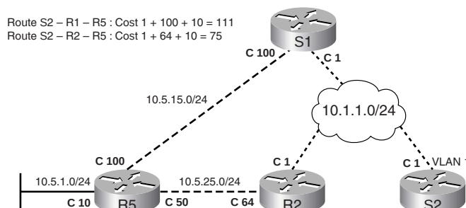
Figure 10-4 Single-Area SPF Calculation: Conceptual View
