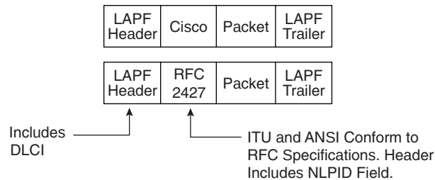
Figure 18-2 Frame Relay Encapsulation Options
