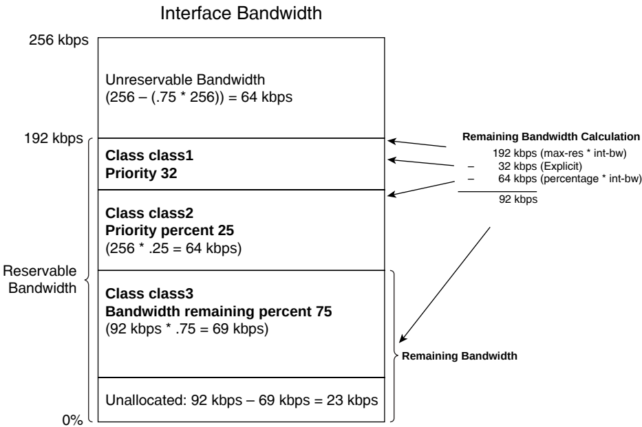
Figure 15-8 Priority, Priority Percent, and Bandwidth Remaining Percent
