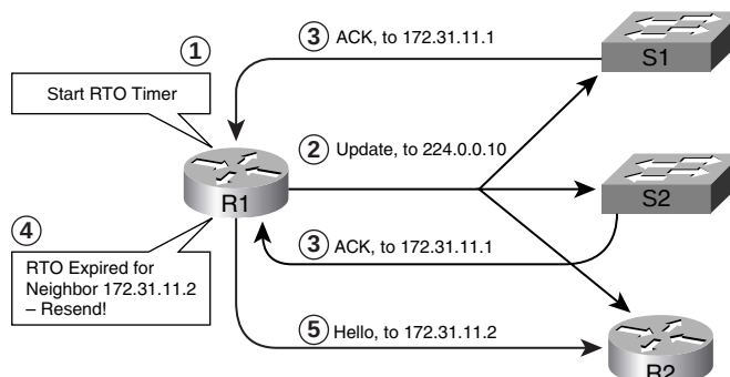
Figure 9-2 EIGRP Use of RTP on a LAN
