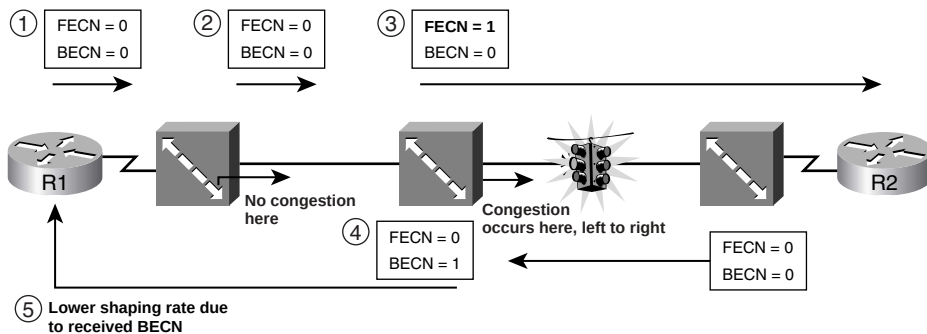
Figure 18-3 Basic Operation of FECN and BECN
