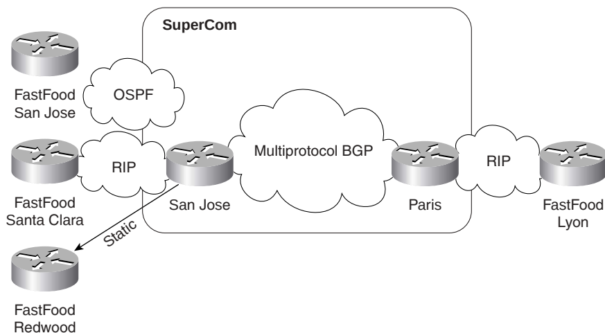
Figure C-24 Routing Protocols Used in FastFood VPN
