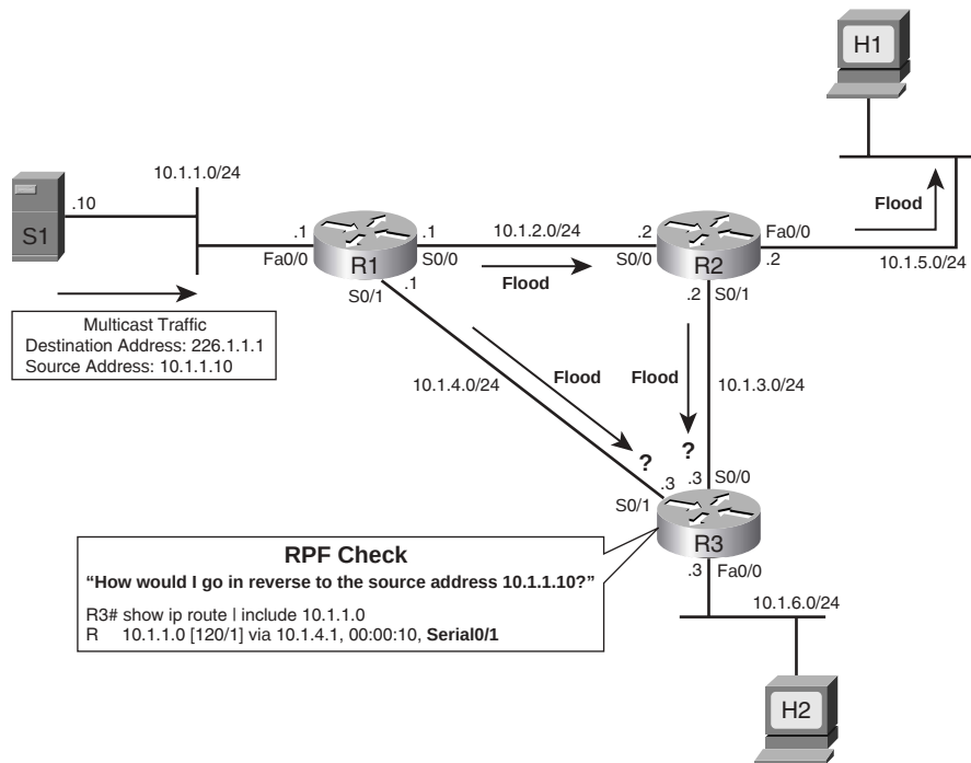
Figure 20-3 R3 Performs the RPF Check
