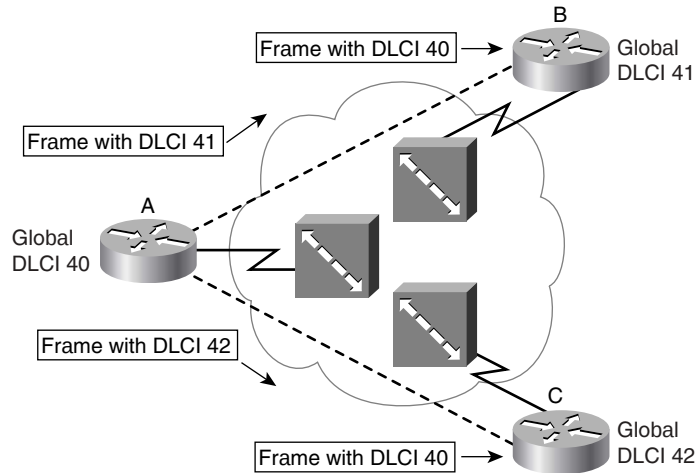
Figure 18-1 Comparing Local and Global Frame Relay DLCIs
