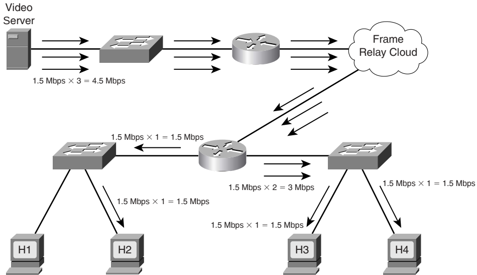
Figure 19-1 Unicast
