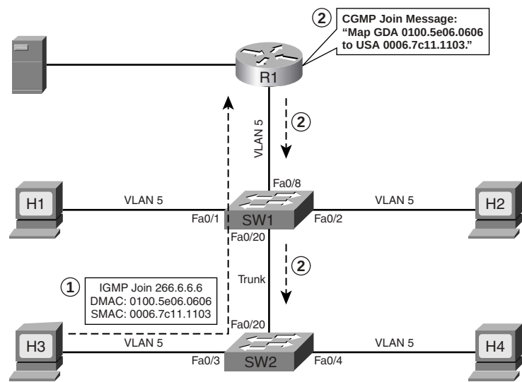
Figure 19-17 CGMP Join Message Process
