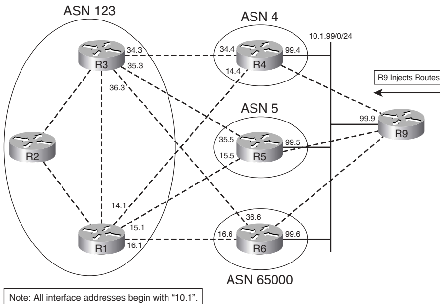
Figure 13-7 Sample Network: AS 123 Without Confederations
