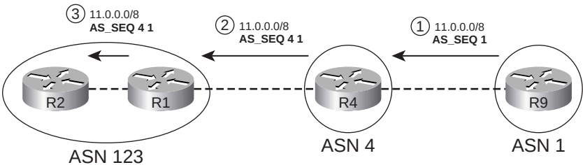
Figure 13-2 AS_PATH (AS_SEQUENCE) Prepending
