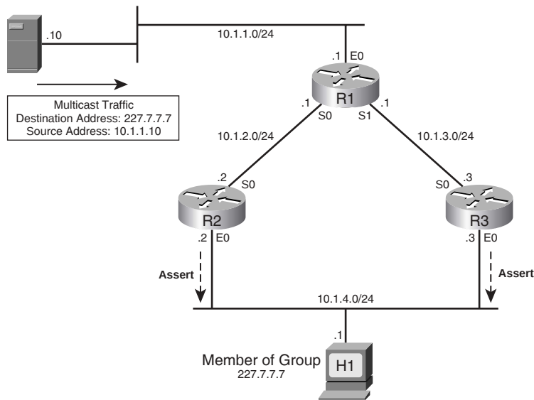
Figure 20-12 R2 and R3 Sending Assert Messages
