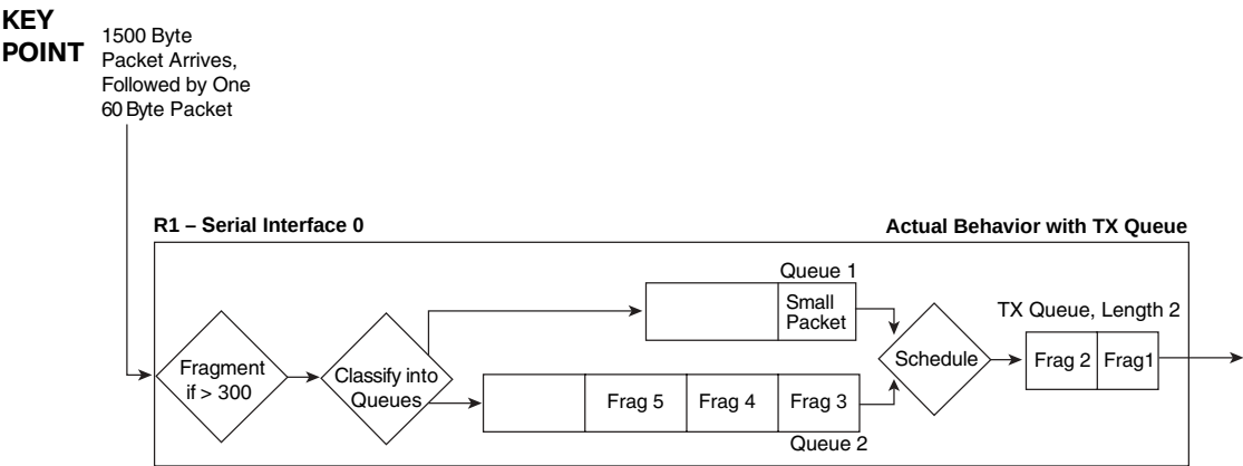
Figure 17-3 MLP LFI Concept
