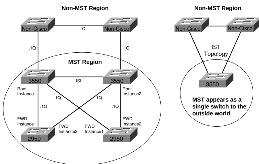
Figure 3-8 MST Operations
