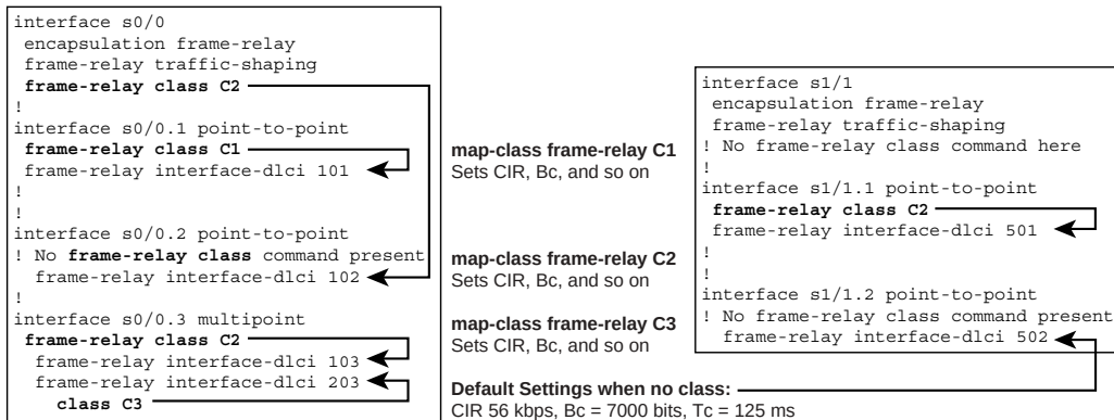
Figure 16-5 Assignment of Map Classes to DLCIs with FRTS
