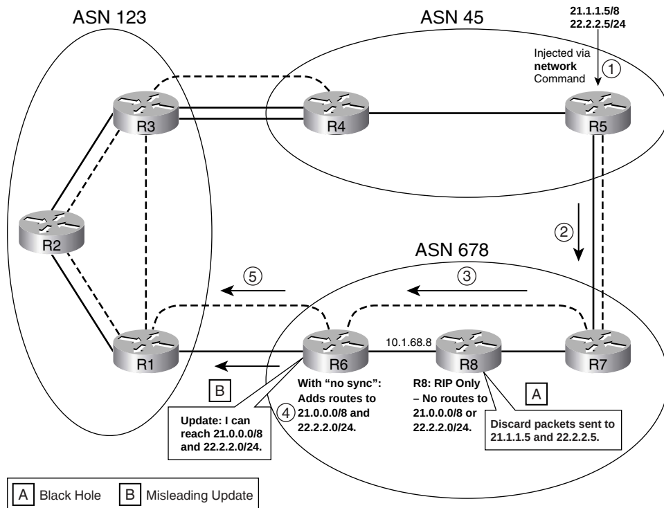
Figure 12-7 Problem: Routing Black Hole Due to Not Using BGP Sync
