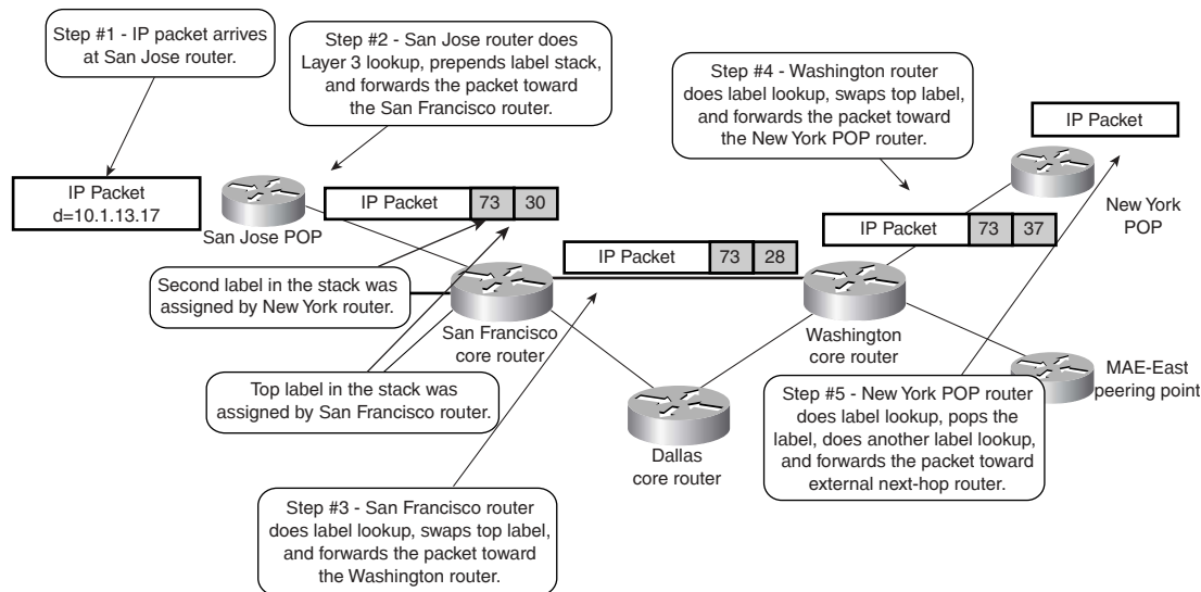
Figure C-14 Label Switching with the MPLS Label Stack
