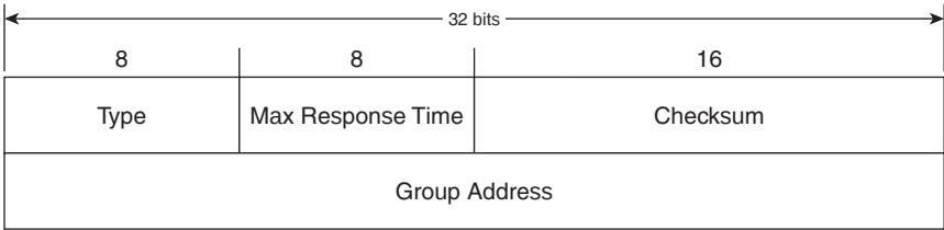
Figure 19-12 IGMPv2 Message Format
