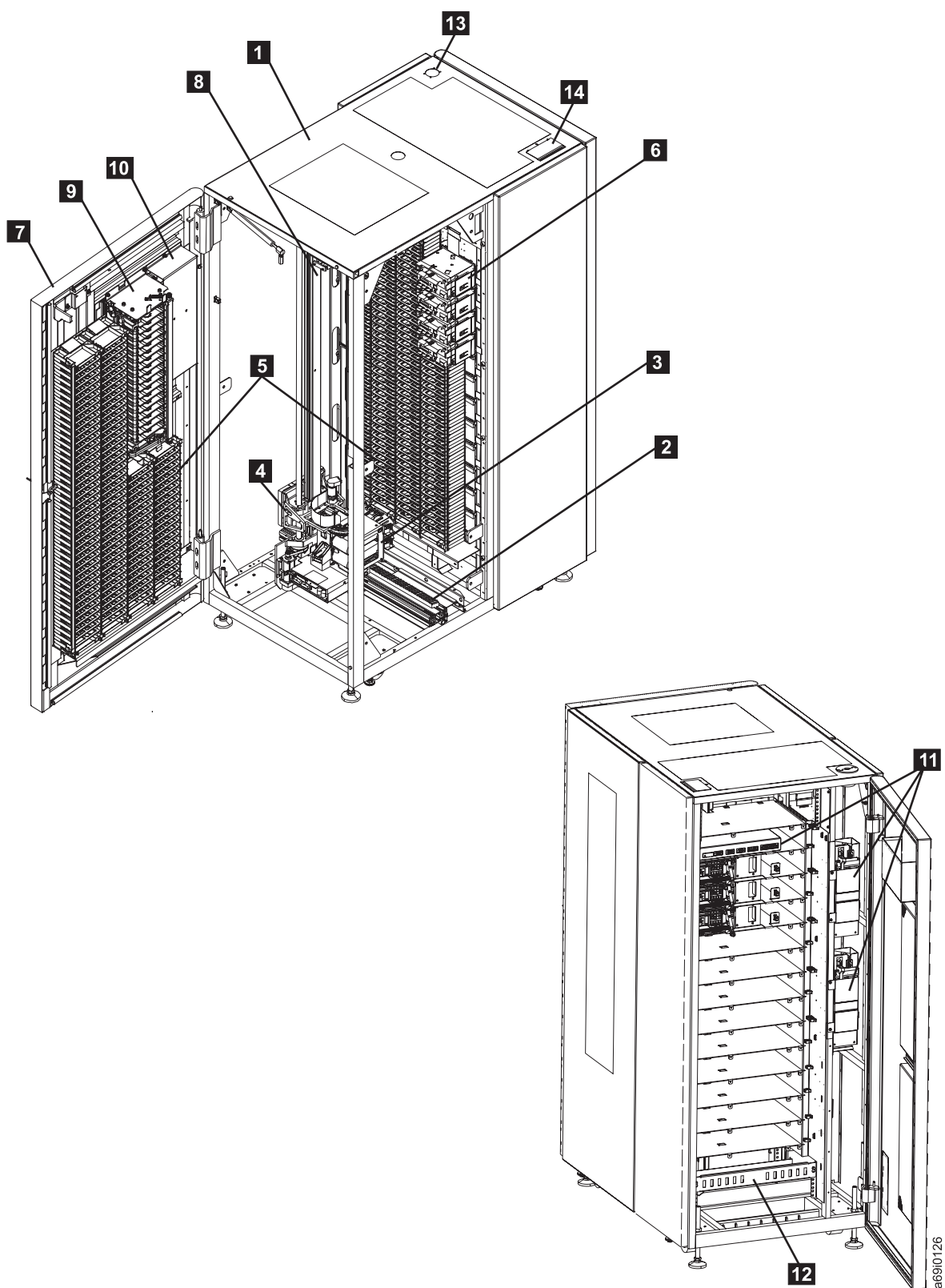
Figure 7. Components of the IBM System Storage TS3500 Tape Library. The front of a Model L53 is shown at the top. The rear of Model L53 is shown on the bottom.
