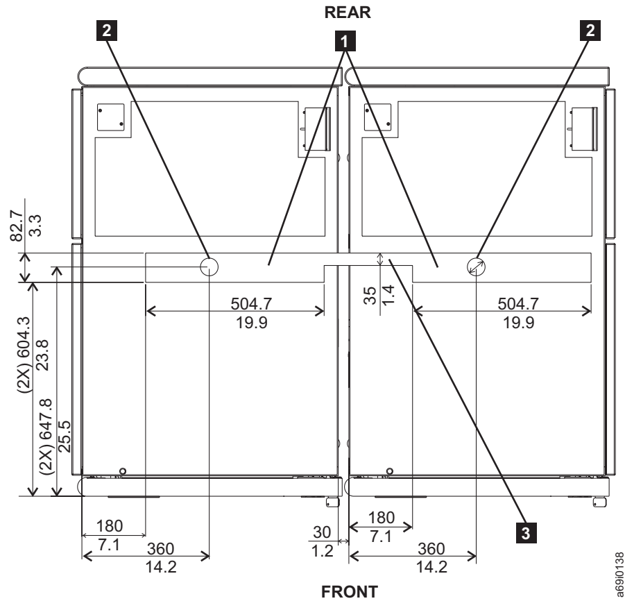
Figure 27. Allowable area for mounting fire-suppression equipment (top view of Models L22, D22, L23, D23, L52, D52, L53, D53, S24, S54, or the HA1 frame)
