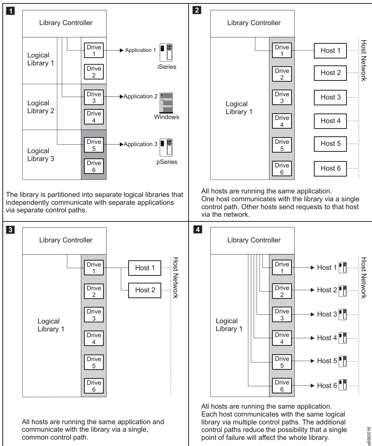
Figure 11. Examples of configurations for sharing an IBM System Storage TS3500 Tape Library. Lines from one or more drives to the library controller represent control paths.
