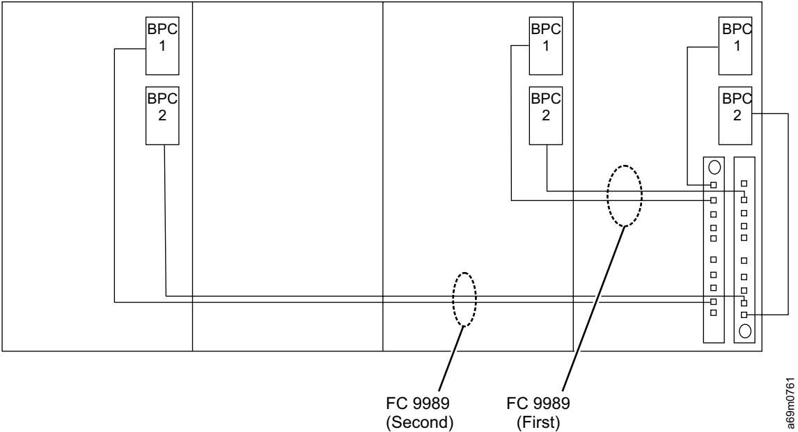
Figure 32. FC 9989 cable positions
