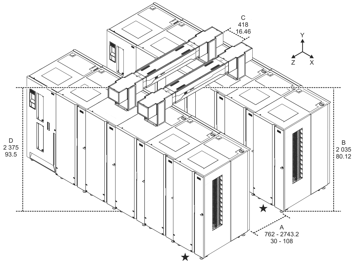
Figure 21. Shuttle complex dimensions and clearances
