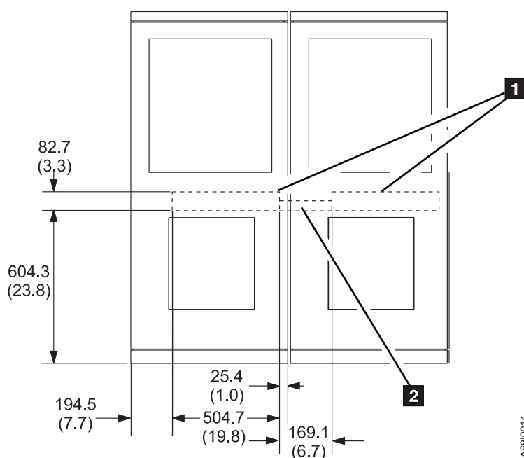
Figure 26. Allowable area for mounting fire-suppression equipment (top view of Model L32 or D32 frames)
