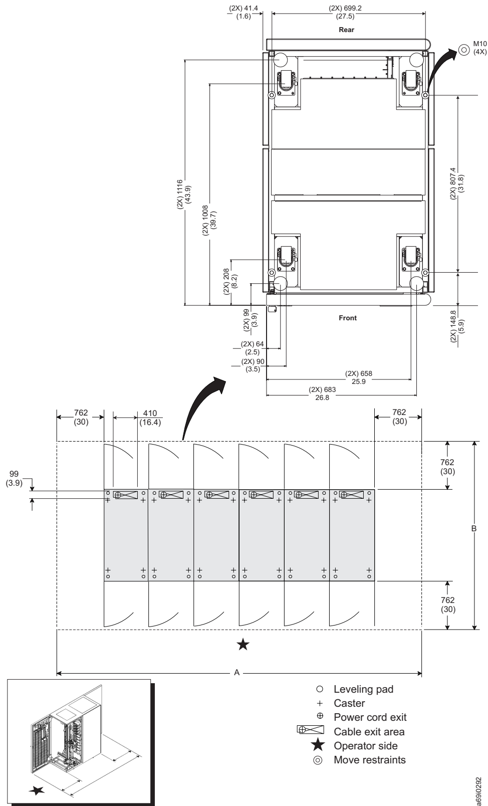
Figure 19. Size of operator and service clearances for the IBM System Storage TS3500 Tape Library, Models L22, D22, L23, D23, L52, D52, L53, D53, S24, S54, and the service bays. The top measurements are in millimeters; the bottom measurements are in inches. The service clearance area (and operator clearance area at the front of both frames) is denoted by dotted lines.
