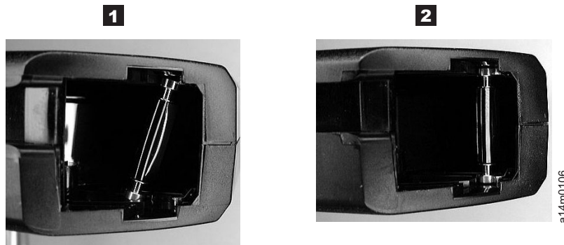
Figure 56. Leader pin in the incorrect and correct positions in a 3592 tape cartridge. The cartridge door is open and the leader pin is visible inside the cartridge.
