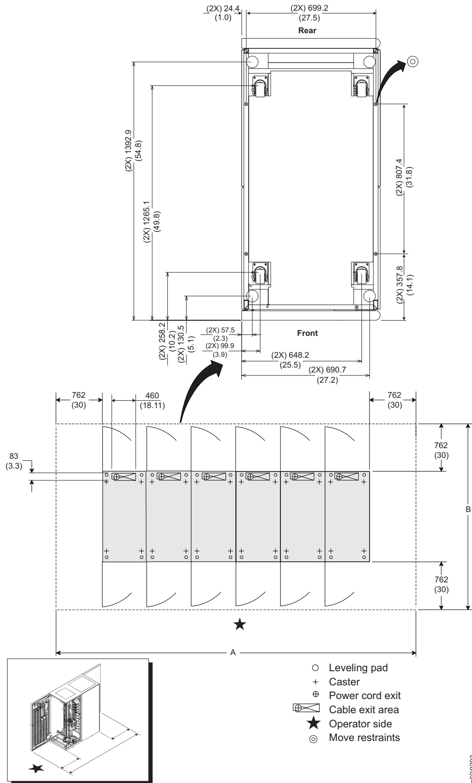
Figure 20. Size of operator and service clearances for the IBM System Storage TS3500 Tape Library, Models L32 and D32. The top measurements are in millimeters; the bottom measurements are in inches. The service clearance area (and operator clearance area at the front of both frames) is denoted by dotted lines.
