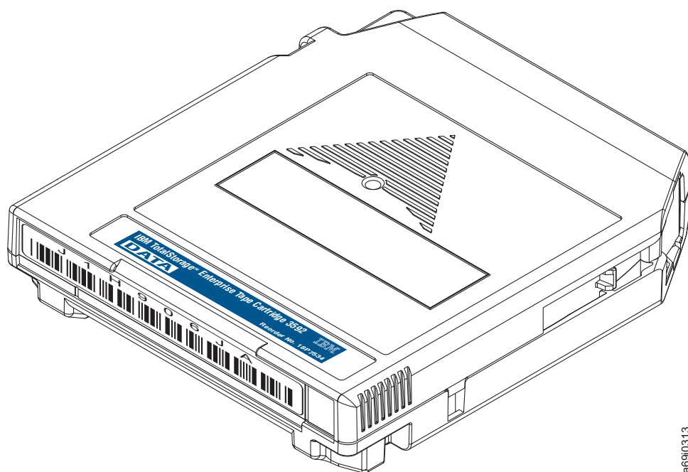
Figure 49. Components of the IBM TotalStorage 3592 Enterprise Tape Cartridge
