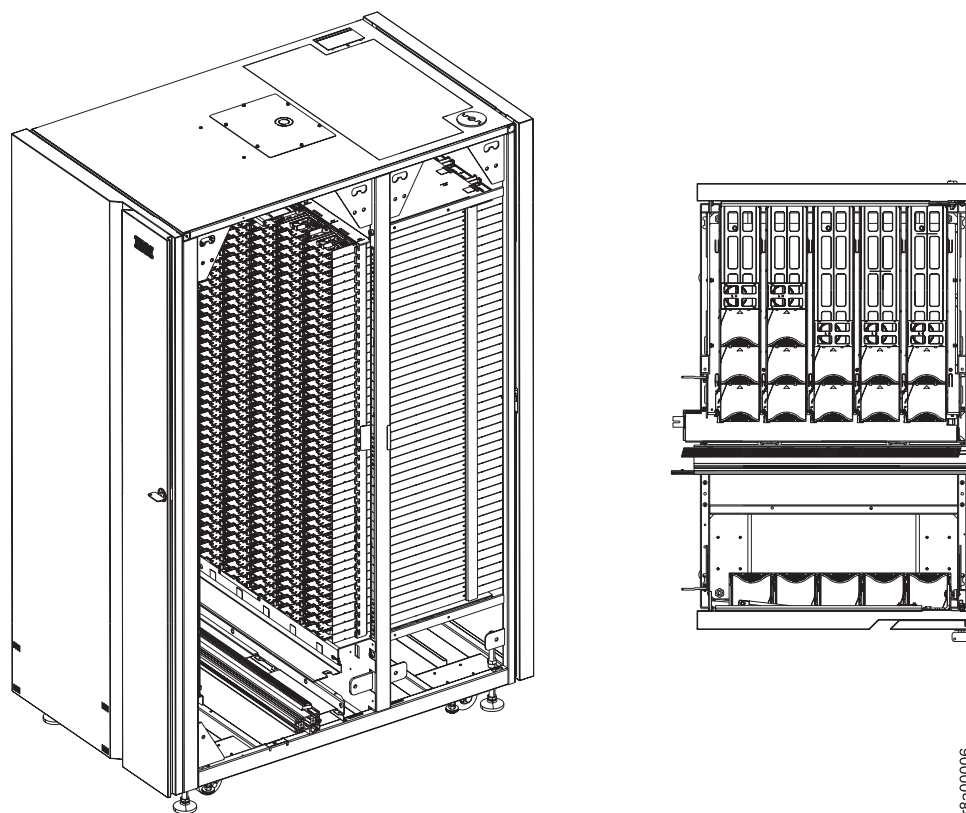
Figure 6. The HD frame (left) and top-down view of row in an HD frame (right)
