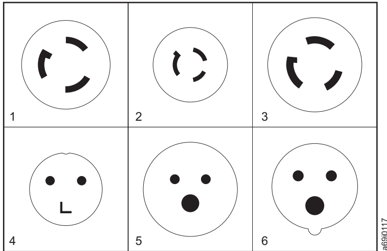
Figure 30. Types of receptacles for power cords used by Models L22, D22, L52, and D52 of the TS3500 Tape Library
