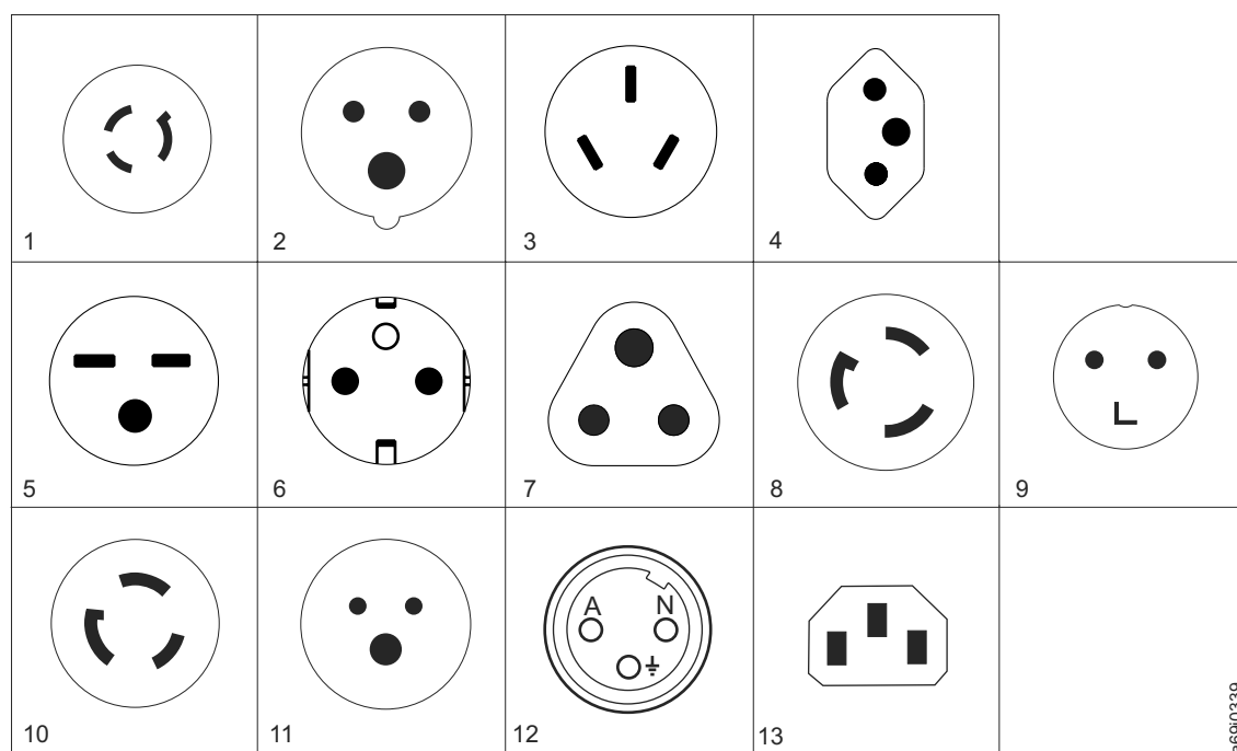
Figure 31. Types of receptacles for Models L23, D23, L53, and D53 of the TS3500 Tape Library
