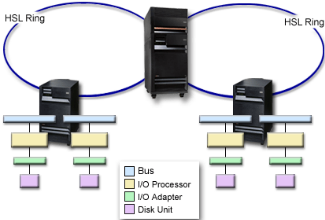
Figure 8. Ring-level protection
