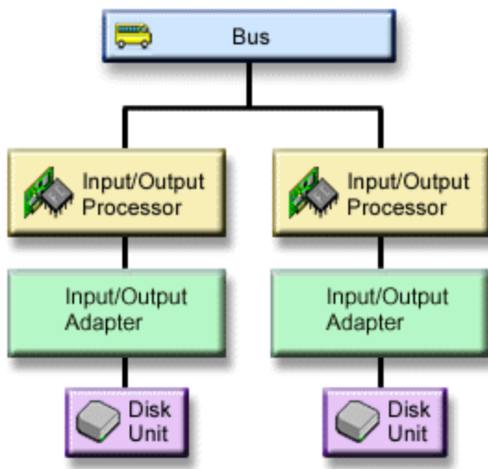
Figure 5. IOP-level protection
