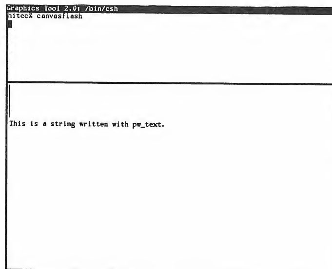
Figure 10-1: canvasflash Output
