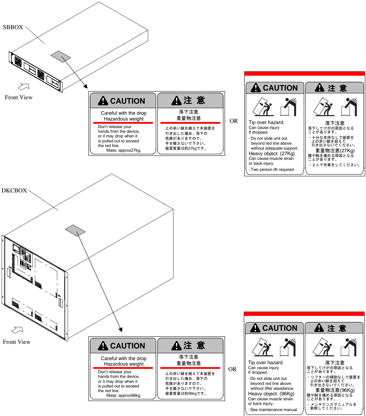
Fig. 3-1 Attachment Position of Safety Labels
