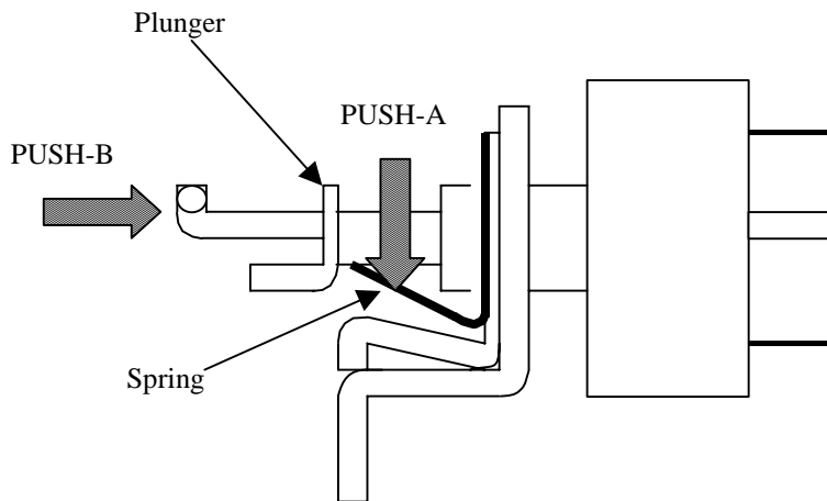
Fig. 1.5.1-1 Emergency condition
