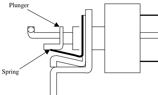
Fig. 1.5.1-2 Normal condition
