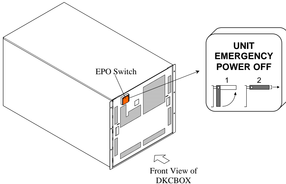
Fig. 1.5-1 Operation of UNIT EMERGENCY POWER OFF switch
