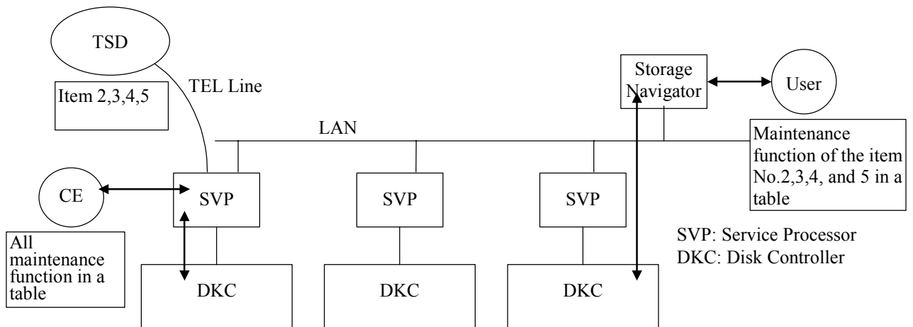
Fig. 1.4-1 Maintenance Execution Route when CVS Is Used
