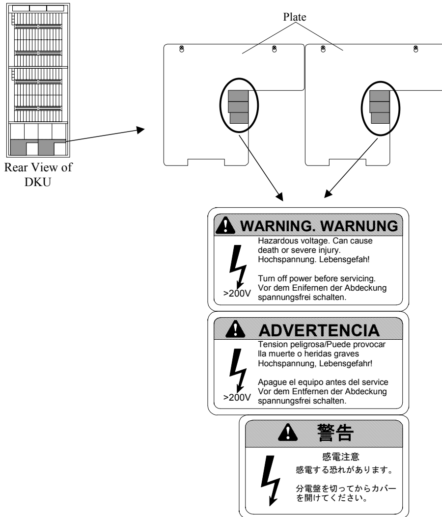
Fig.4-7 Attachment Position of Safety Labels
