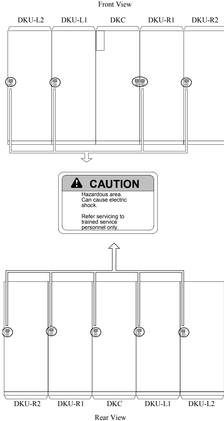
Fig.4-1 Attachment Position of Safety Labels
