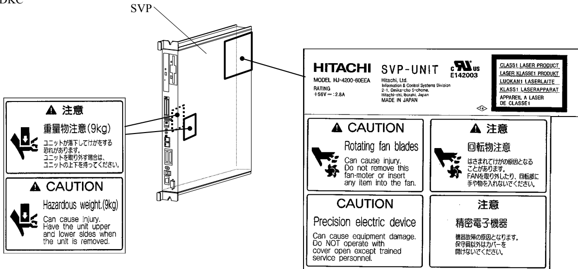
Fig.4-5 Attachment Position of Safety Labels
