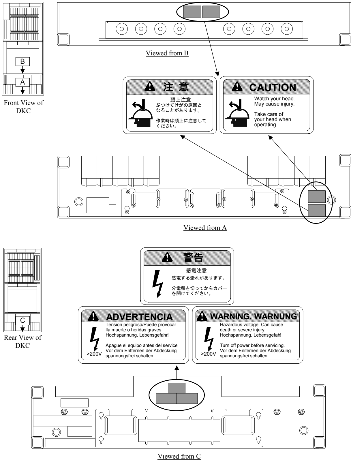
Fig.4-3 Attachment Position of Safety Labels
