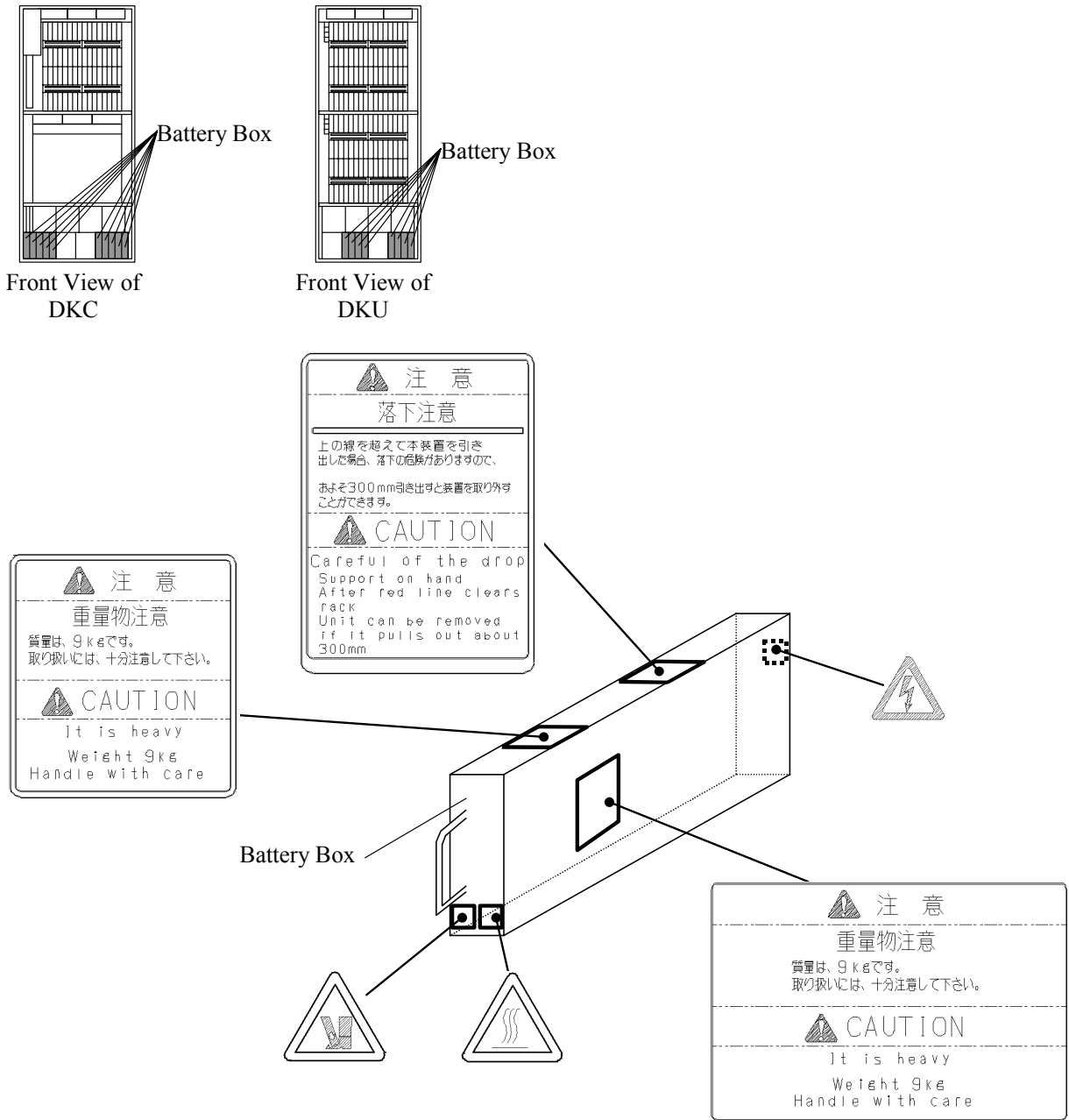
Fig.4-4 Attachment Position of Safety Labels
