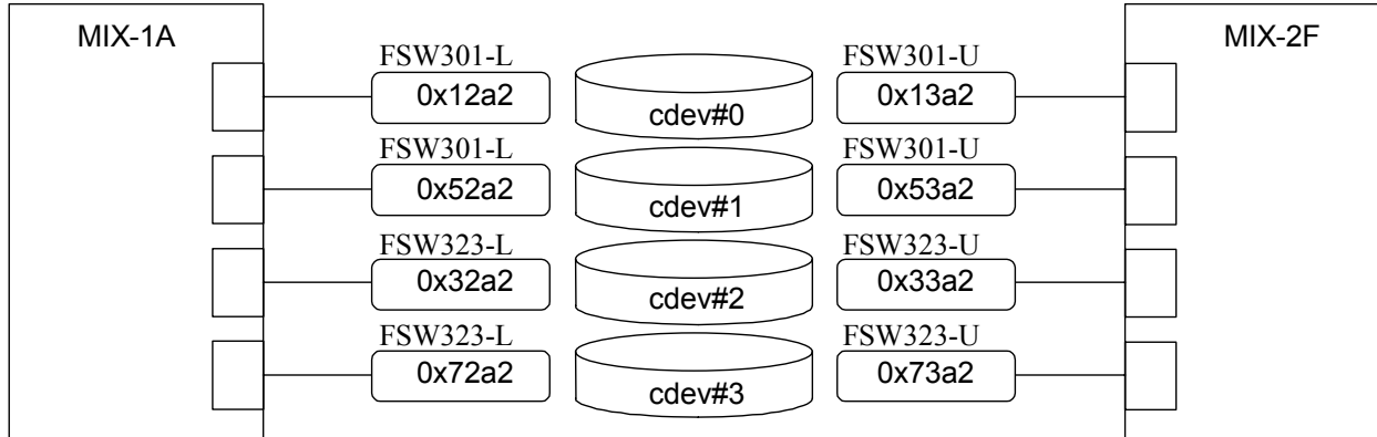
Fig. 6.2-4 HBC Bus Address mapping (DKU-RK3 Unit)
