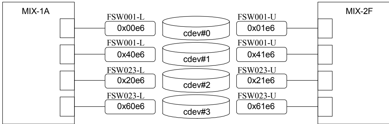
Fig. 6.2-1 HBC Bus Address mapping (DKU-RK0 Unit)
