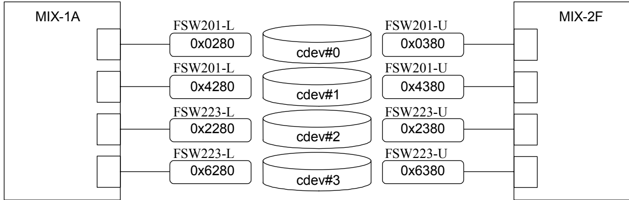
Fig. 6.2-3 HBC Bus Address mapping (DKU-RK2 Unit)
