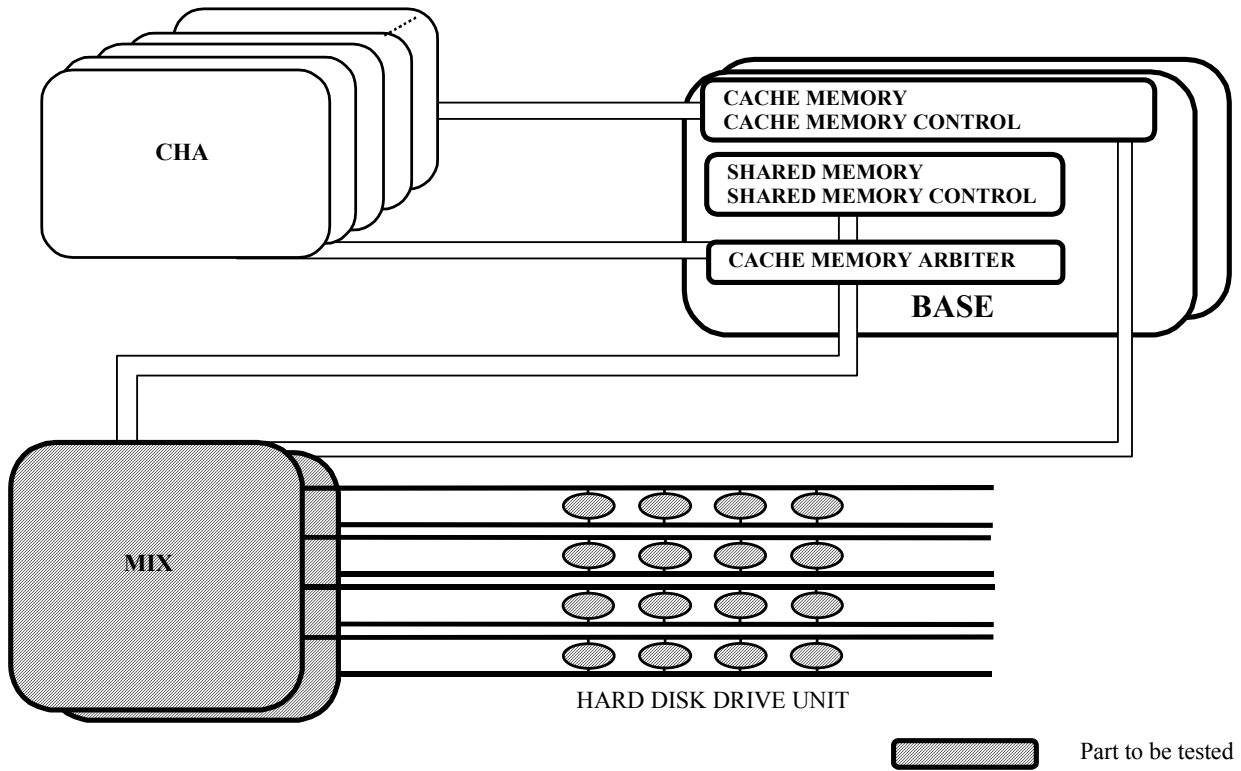
Fig. 3-3 Parts Subject to DKU INLINE Tests
