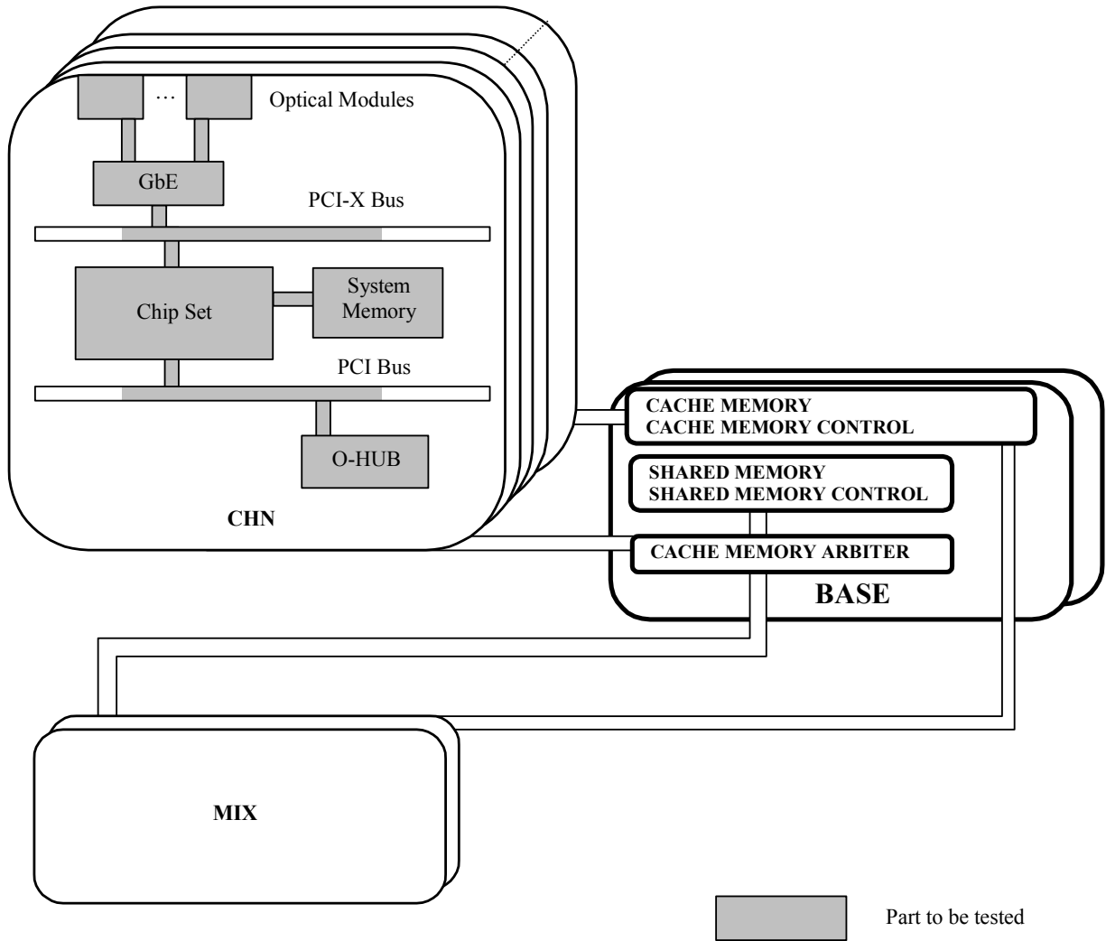
Fig. 3-8 Parts Subject to PCDG4 Tests
