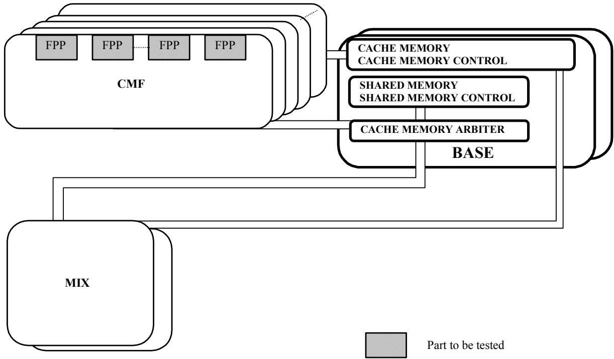
Fig. 3-7 Parts Subject to FCDG4 Tests
