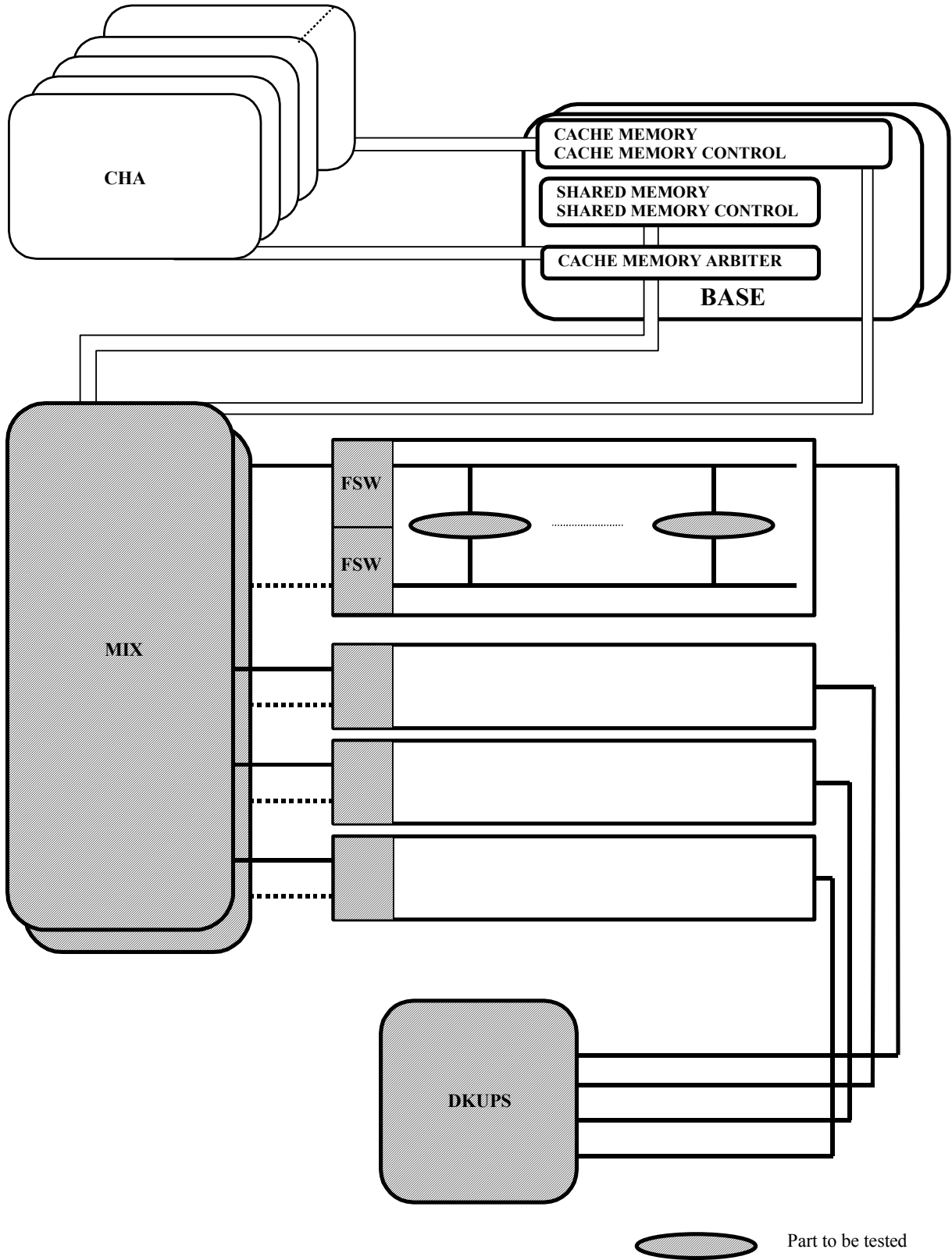
Fig. 3-4 Parts Subject to DKU PATH INLINE Tests
