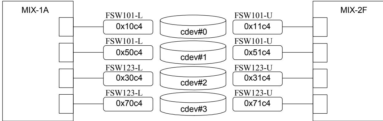
Fig. 6.2-2 HBC Bus Address mapping (DKU-RK1 Unit)
