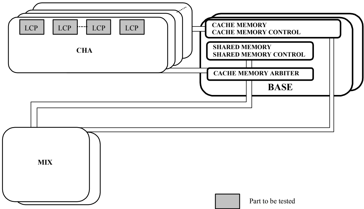
Fig. 3-6 Parts Subject to LCDG4 Tests
