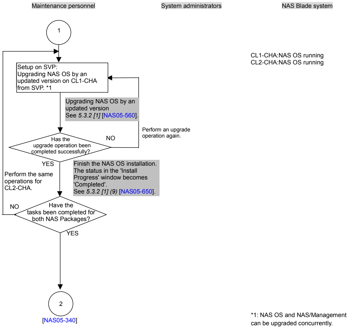
Figure 5.3-4 Upgrading NAS OS by an Updated Version (Preventive Upgrade: While the Cluster is Stopped) (3/4)
