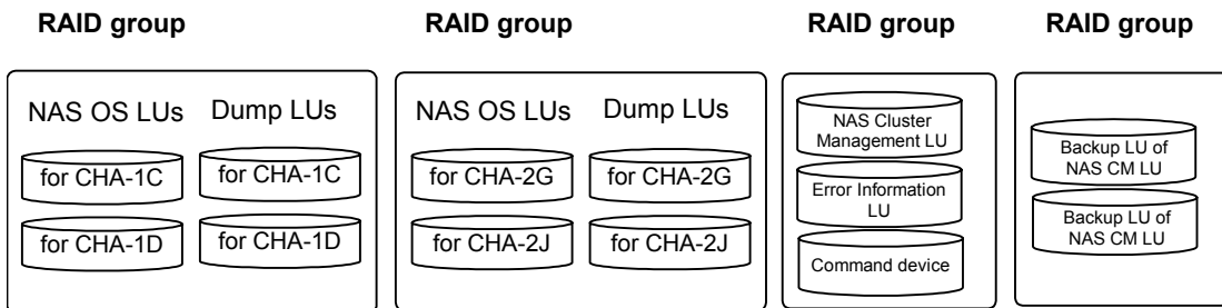
Figure 3.2-1 Examples of NAS System LU Configurations
