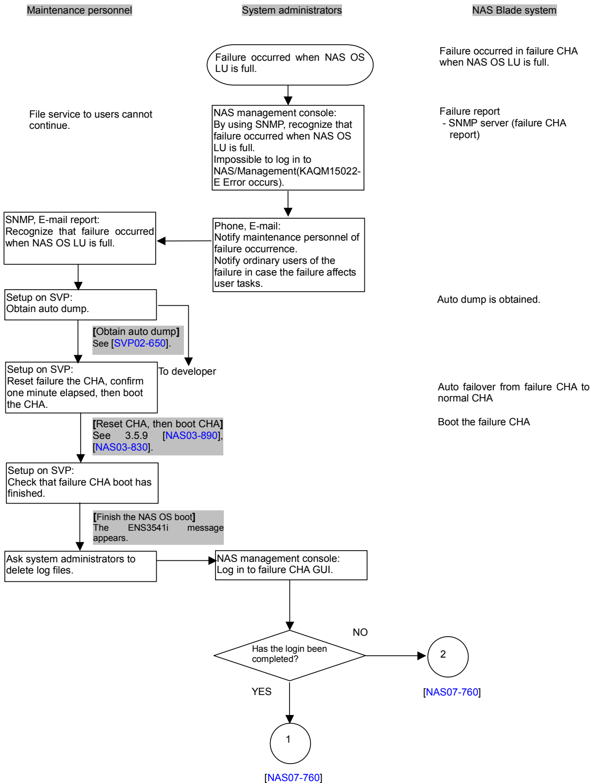
Figure 7.4-20 Failure when NAS OS LU is full (2/3)
