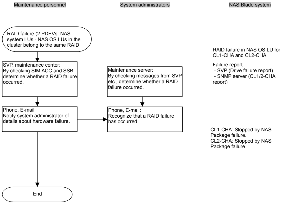
Figure 7.4-5 RAID Failure (2 PDEVs: NAS System LUs — NAS OS LUs in the Cluster Belong to the Same RAID Group) (2/2)
