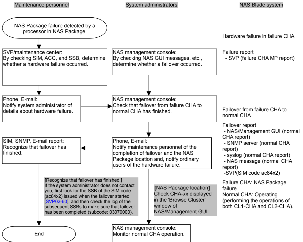
Figure 7.4-1 NAS Package Failure Detected By a Processor in the NAS Package (2/2)
