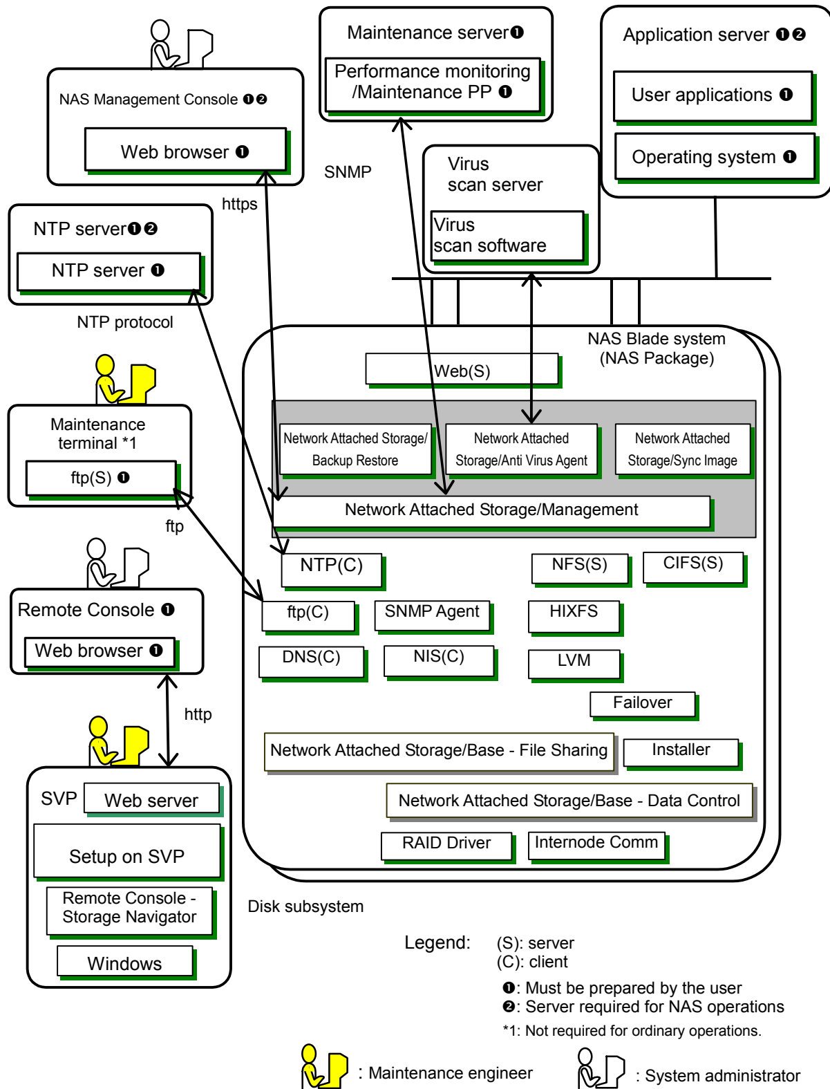
Figure 2.3-1 Basic Configuration of the NAS Blade System
