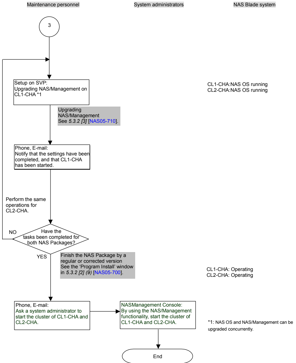
Figure 5.3-5 Replacing the NAS OS By a Patch Version — Restarting the NAS OS Is Not Required (Preventive Upgrade: While the Cluster is Stopped) (4/7)
