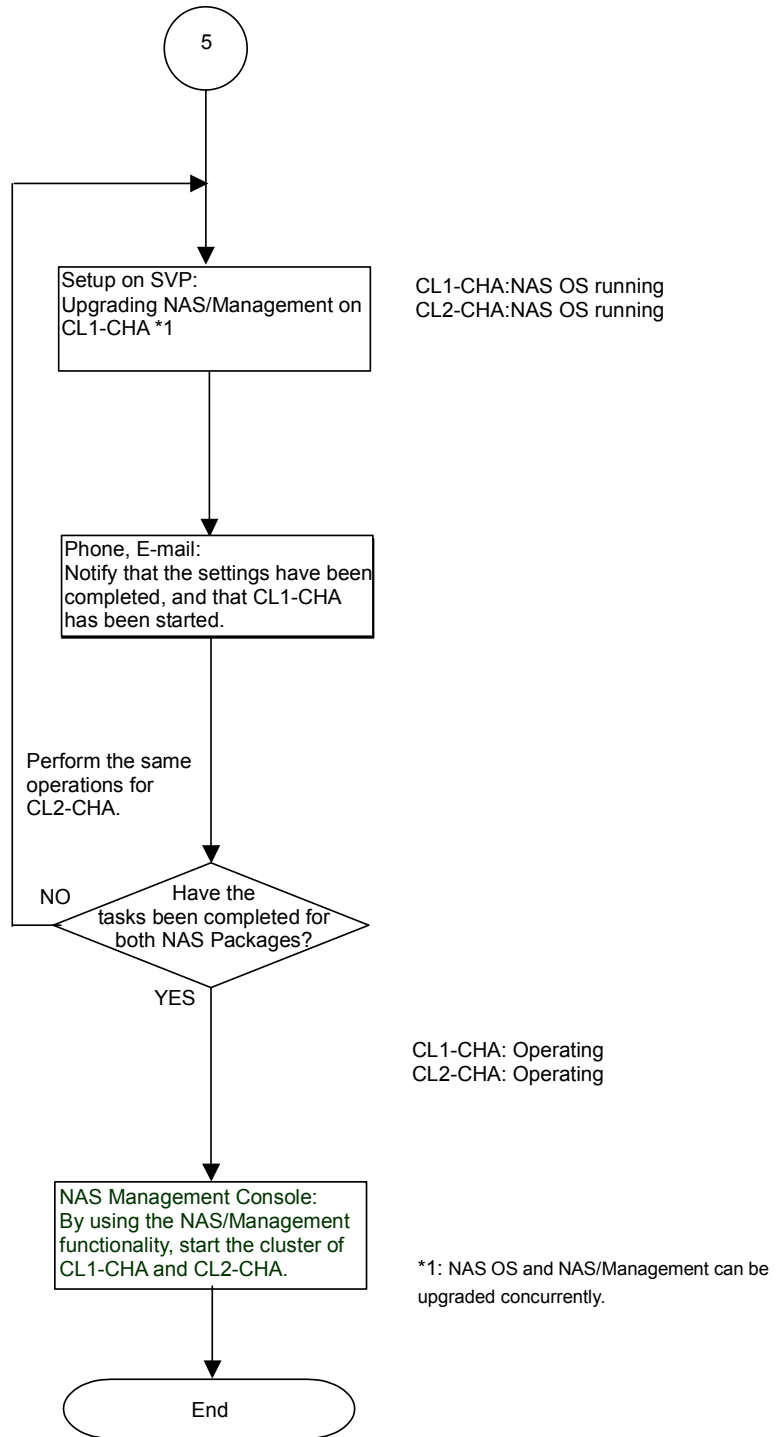
Figure 5.3-6 Replacing the NAS OS By a Patch Version — Restarting the NAS OS Is Required (Preventive Upgrade: While the Cluster is Stopped) (7/7)
