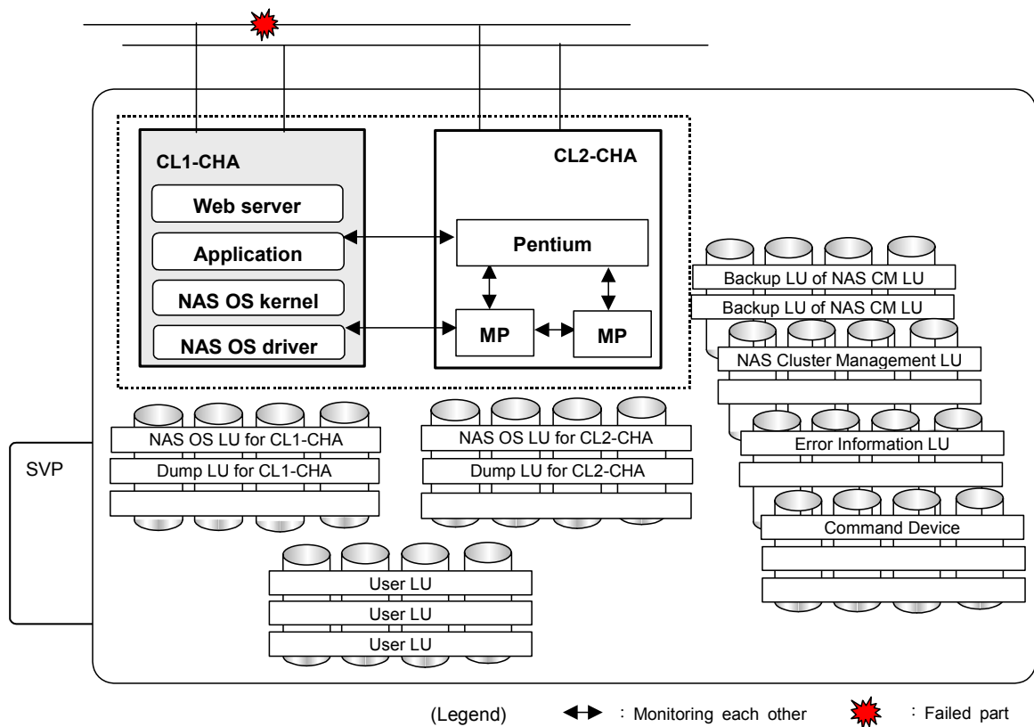
Figure 7.4-12 Network Failure (Network Settings Failed) (1/3)
