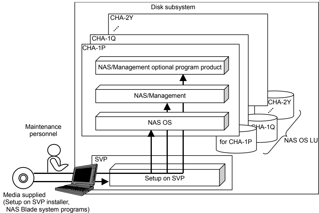
Figure 3.5-1 Entire Configuration of Setup on SVP (for a Multi-Cabinet Model)
