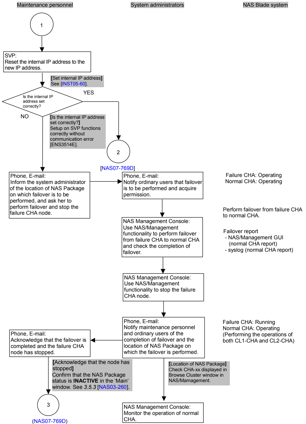
Figure 7.4-24 NAS OS Application Failure (Unable to Set Internal IP Address) (3/4)
