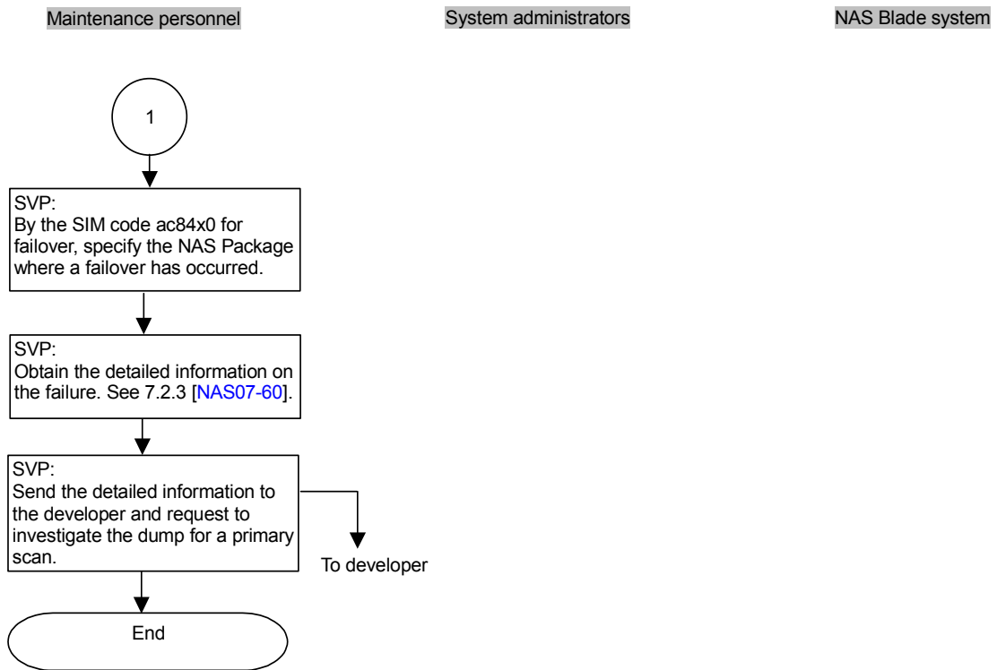
Figure 7.4-19 NAS OS Failure (In Start/Stop Processing) (3/3)
