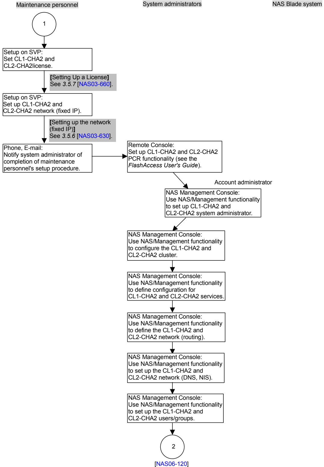
Figure 6.2-3 Adding a NAS Package (3/4)
