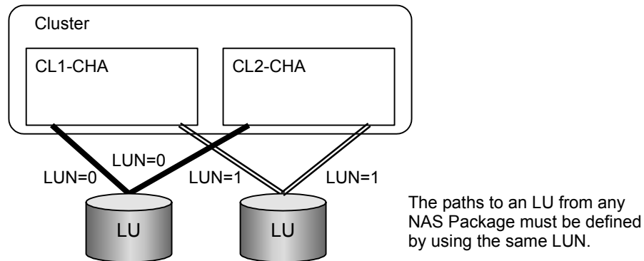
Figure 3.2-2 Example of How Paths to User LUs are Defined
