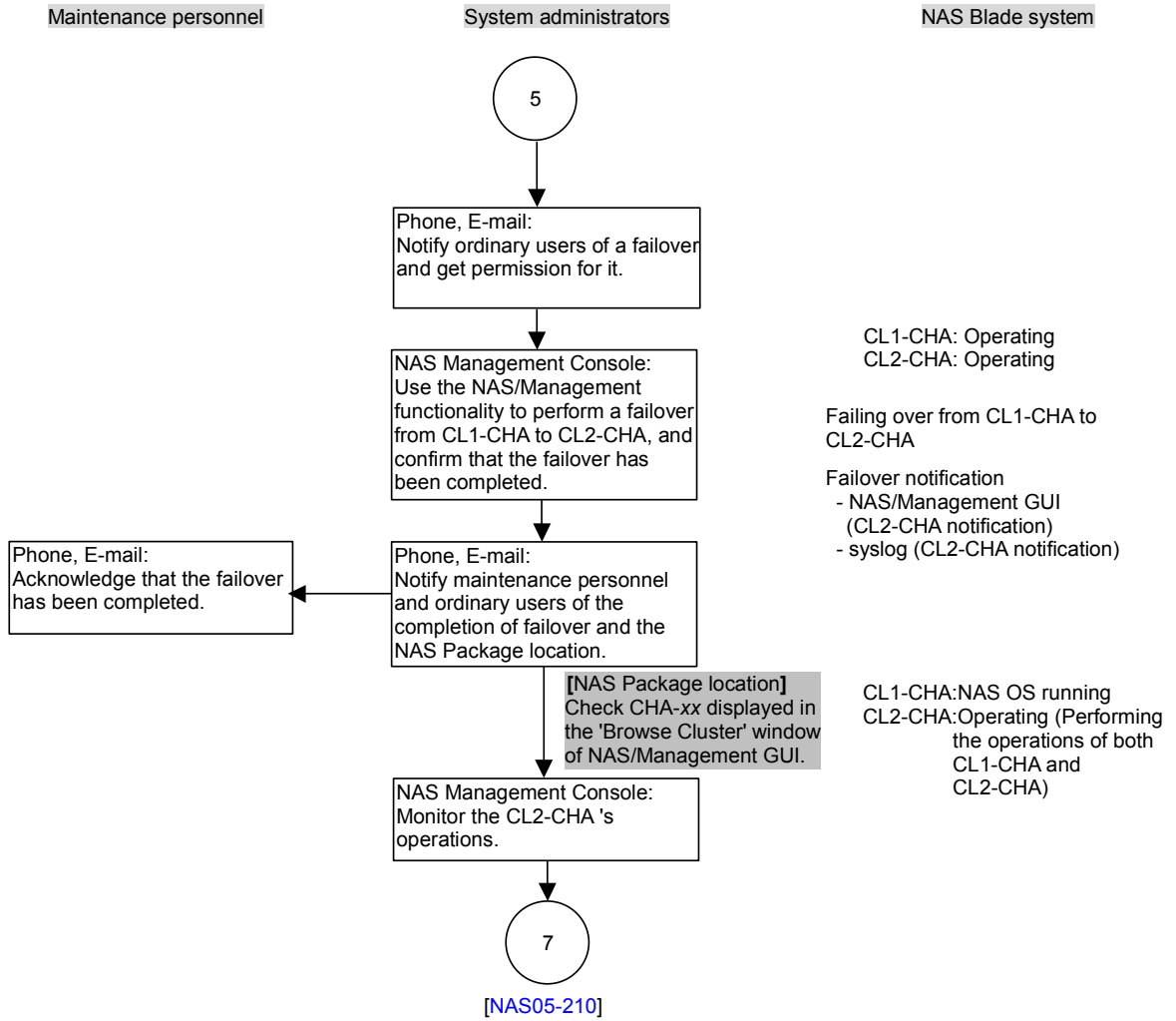
Figure 5.3-2 Upgrading NAS OS By a Patch Version — Restarting the NAS OS Is Not Required (Preventive Upgrade: While Operating) (6/9)
