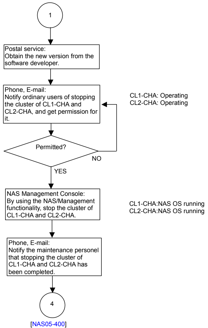
Figure 5.3-5 Replacing the NAS OS By a Patch Version — Restarting the NAS OS Is Not Required (Preventive Upgrade: While the Cluster is Stopped) (5/7)
