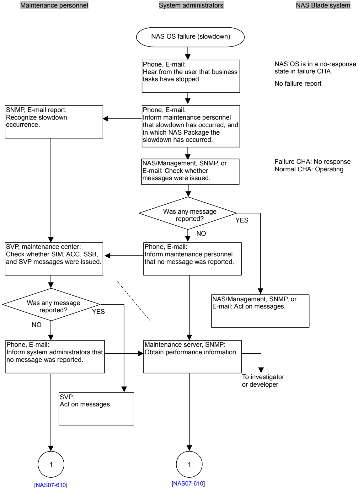
Figure 7.4-15 NAS OS Failure (Slowdown) (2/3)
