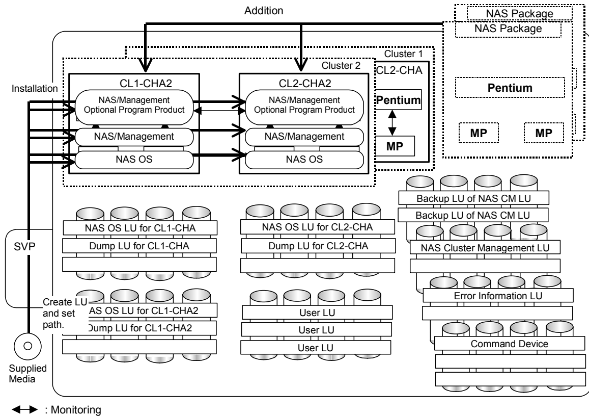
Figure 6.2-3 Adding a NAS Package (1/4)
