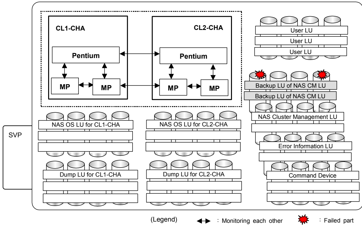
Figure 7.4-10 RAID Failure (2 PDEVs: Backup LUs of NAS Cluster Management LUs) (1/2)
