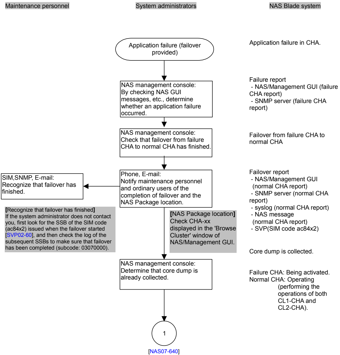
Figure 7.4-16 Application Failure (Failover Provided) (2/3)
