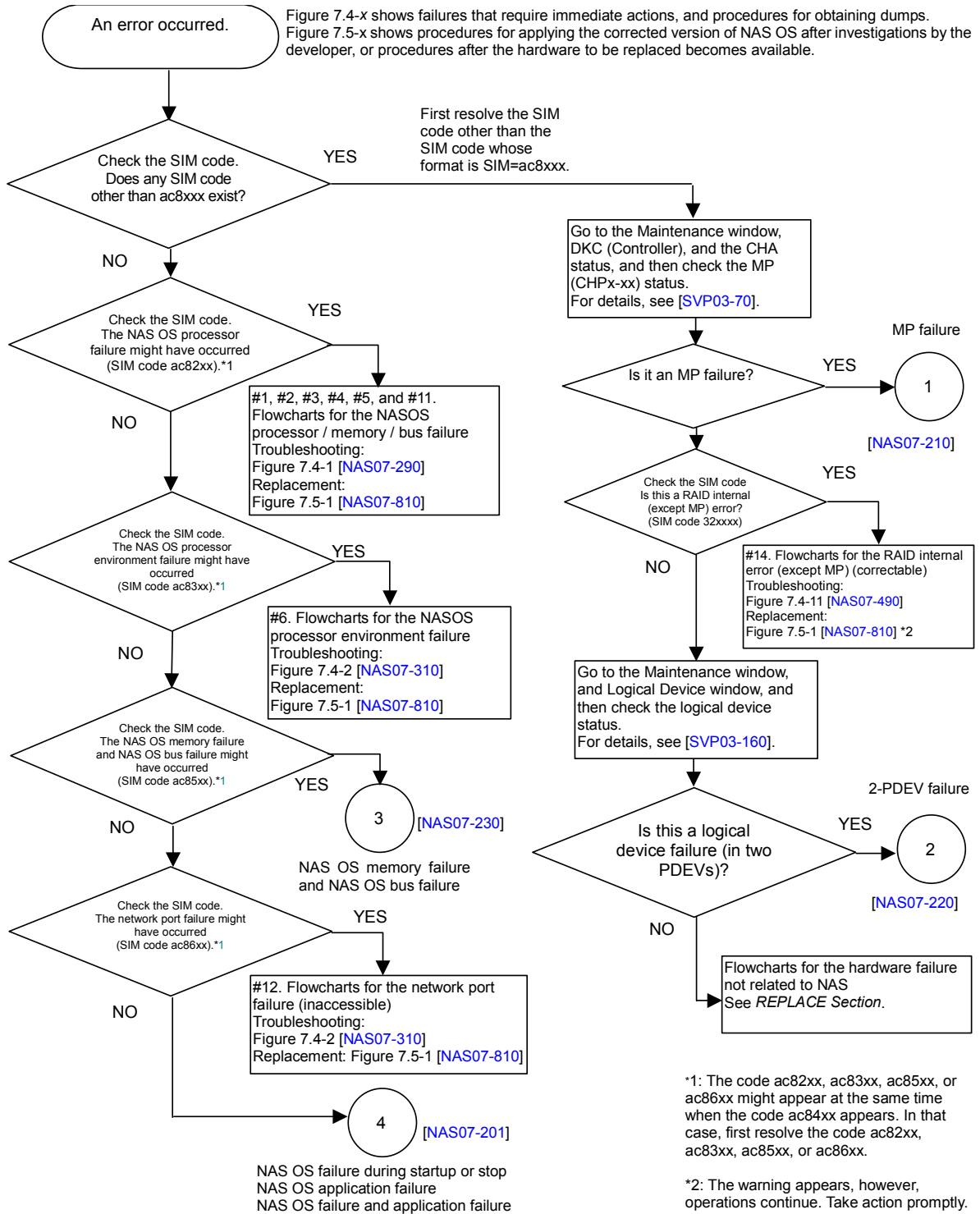
Figure 7.4-0 Flowcharts for Troubleshooting Related to Failure Phenomena (1/11)
