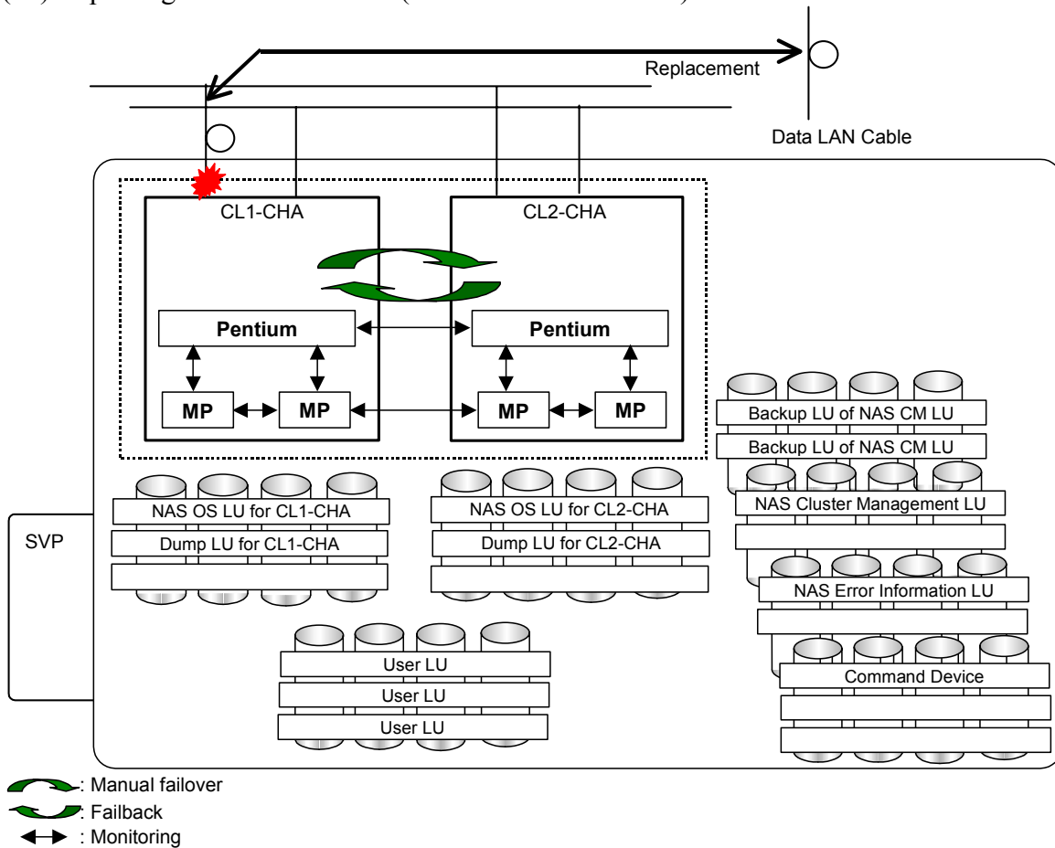
Figure 7.5-11 Replacing Data LAN Cables (When a Failure Occurs) (1/3)
