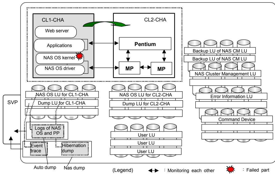
Figure 7.4-15 NAS OS Failure (Slowdown) (1/3)
