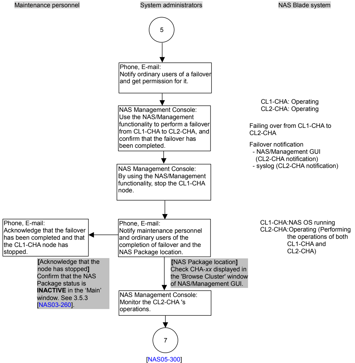
Figure 5.3-3 Upgrading NAS OS By a Patch Version — Restarting the NAS OS Is Required (Preventive Upgrade: While Operating) (6/9)
