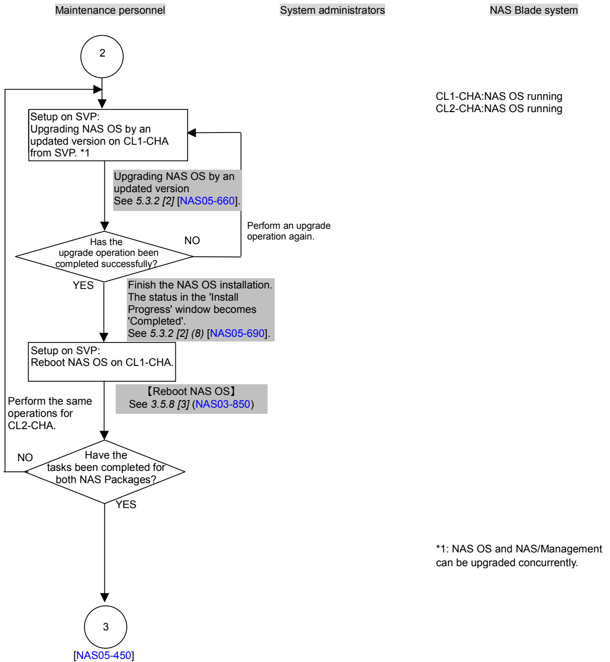
Figure 5.3-6 Replacing the NAS OS By a Patch Version — Restarting the NAS OS Is Required (Preventive Upgrade: While the Cluster is Stopped) (3/7)
