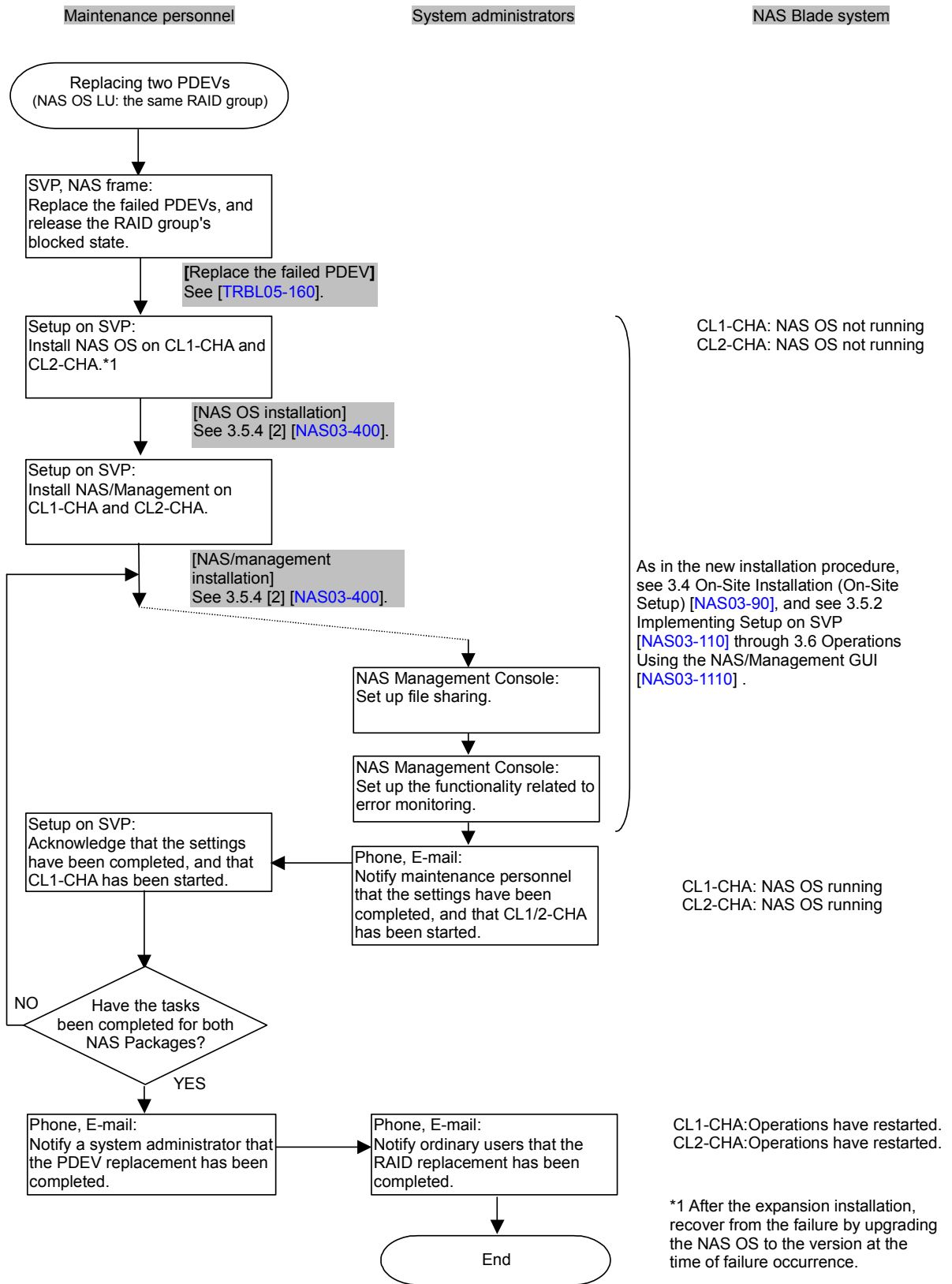
Figure 7.5-5 Replacing Two PDEVs (NAS OS LU: When the NAS OS LUs for CL1-CHA and CL2-CHA Belong to the Same RAID Group) (2/2)
