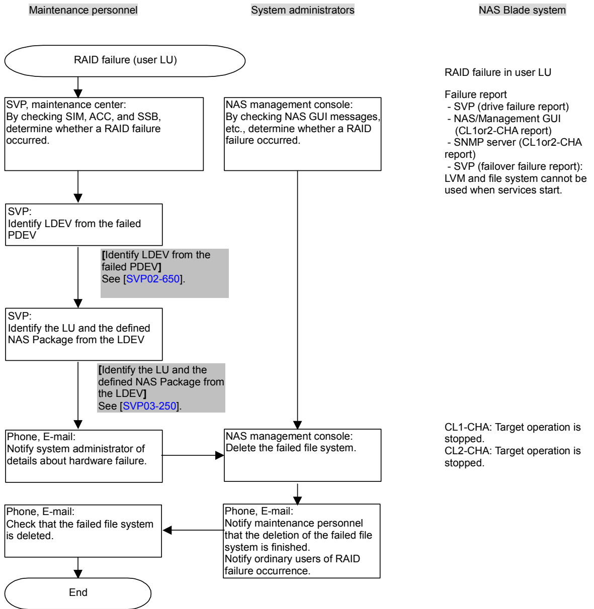
Figure 7.4-3 RAID Failure (User LU) (2/2)
