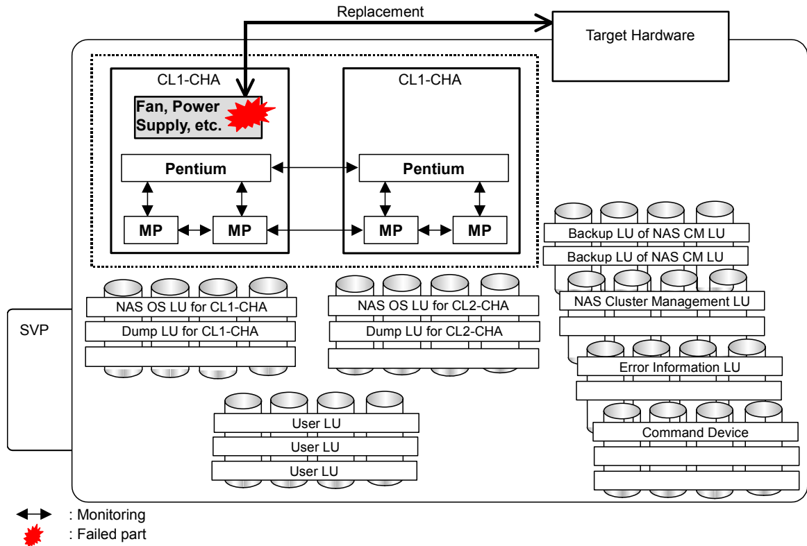
Figure 4.2-3 Hot-Replacing Hardware Other than the NAS Package(1/2)
