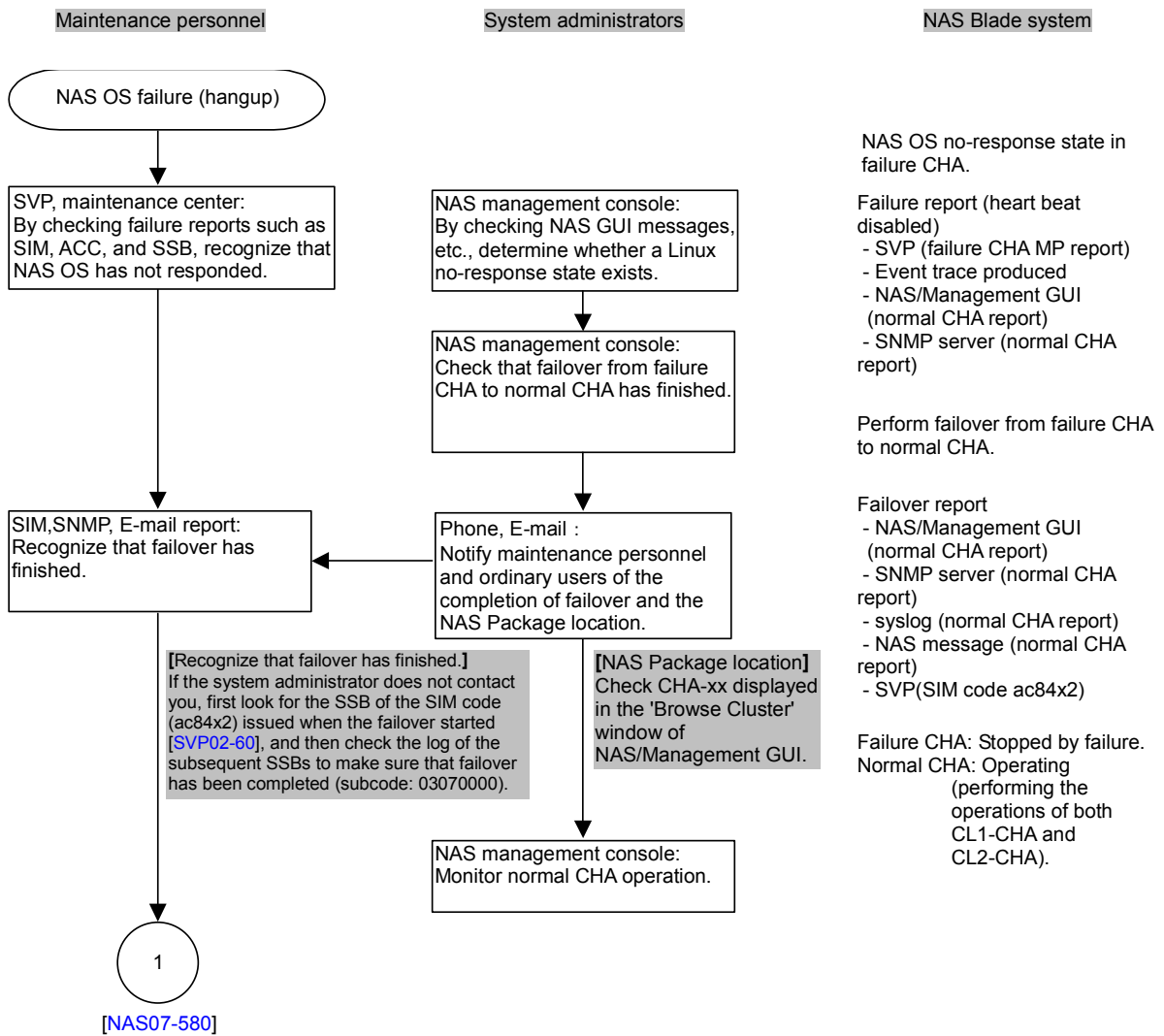
Figure 7.4-14 NAS OS Failure (Hangup) (2/3)
