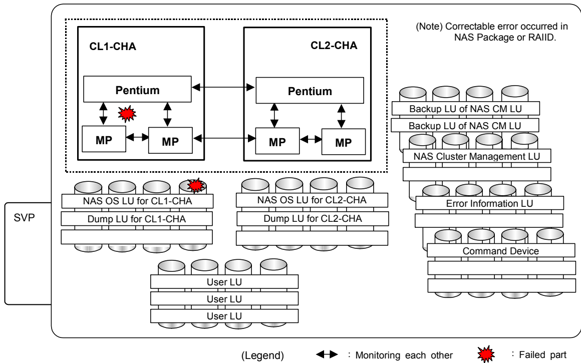
Figure 7.4-11 Hardware Failure (Correctable) (1/2)
