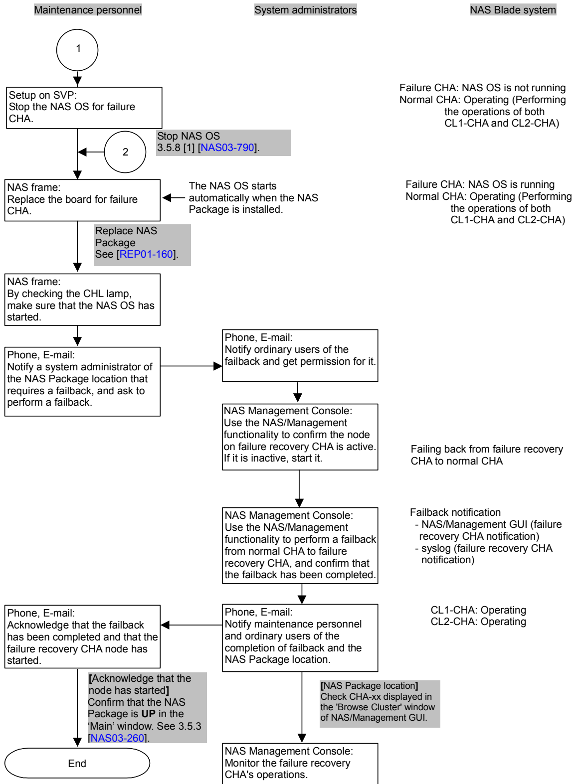
Figure 7.5-1 Replacing the NAS Package (When a Failure Occurs) (3/3)
