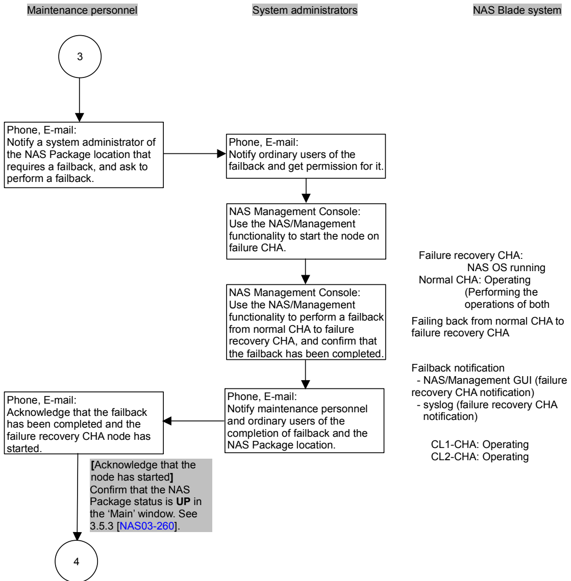
Figure 7.5-7 Replacing Two PDEVs (Dump LUs) (4/5)
