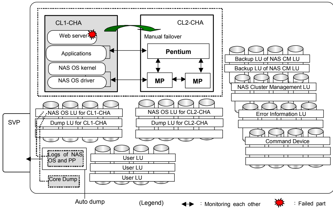
Figure 7.4-18 Application Failure in the Web Server (Failover Not Provided) (1/3)
