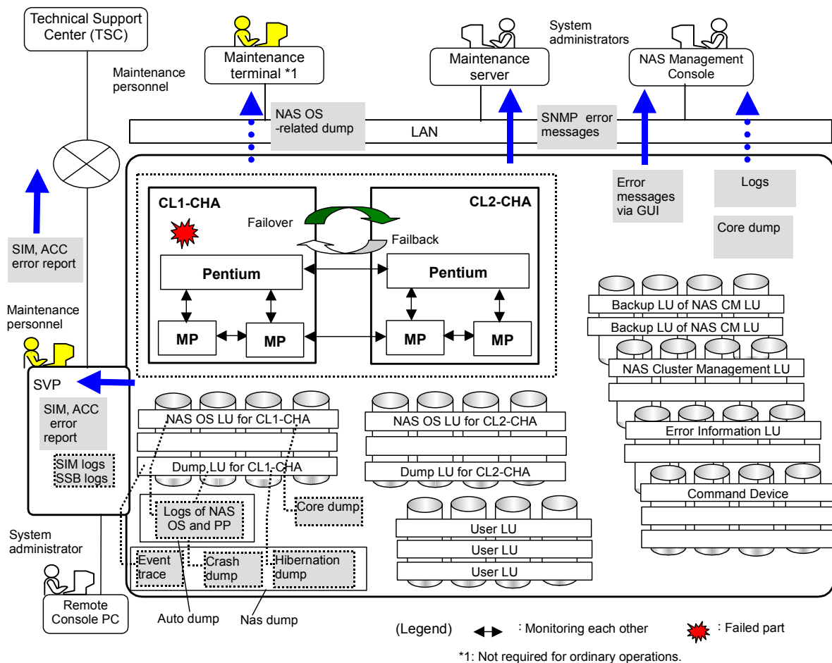
Figure 7.1-1 Detecting Failures and Obtaining Error Information
