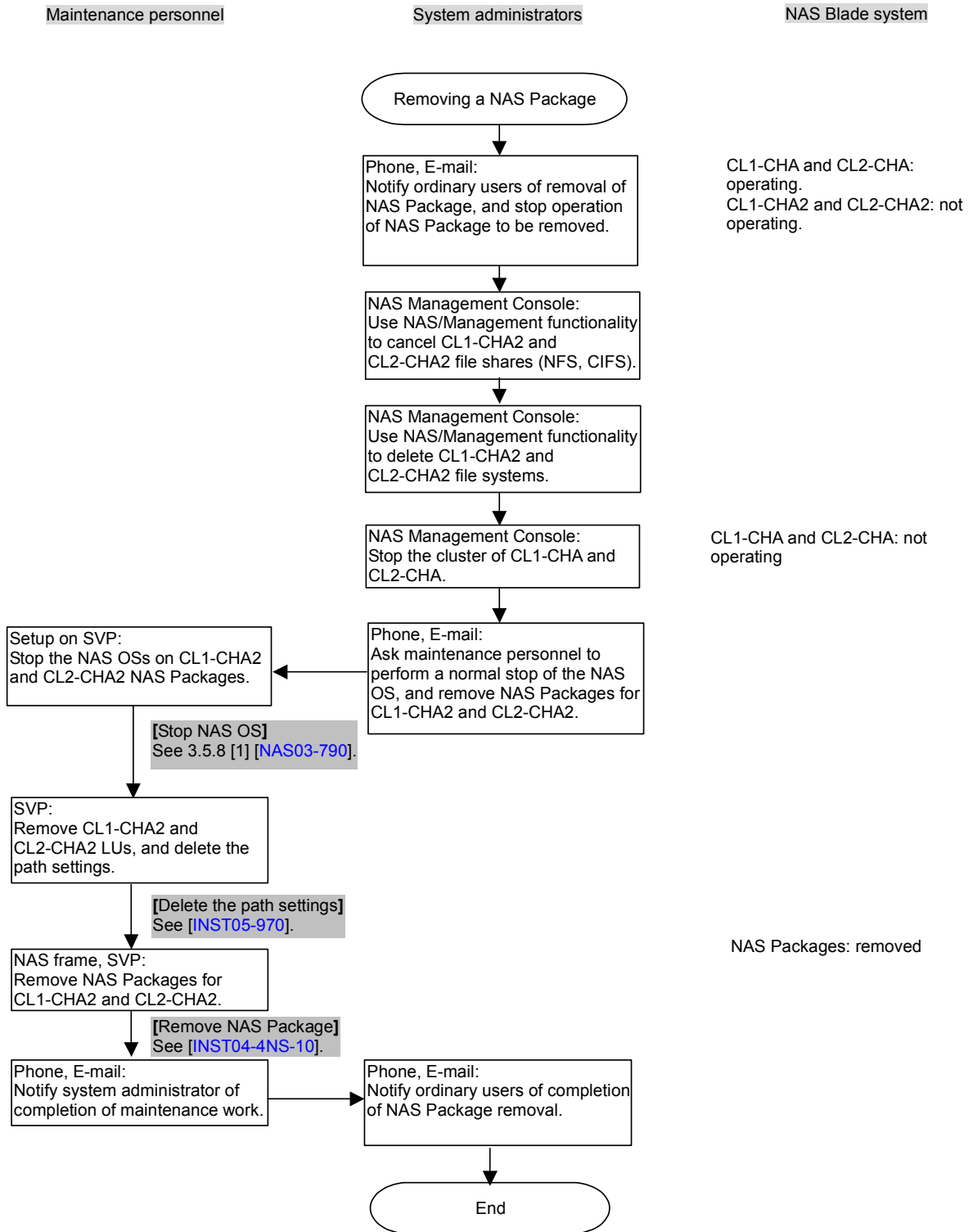
Figure 6.2-4 Removing a NAS Package (2/2)
