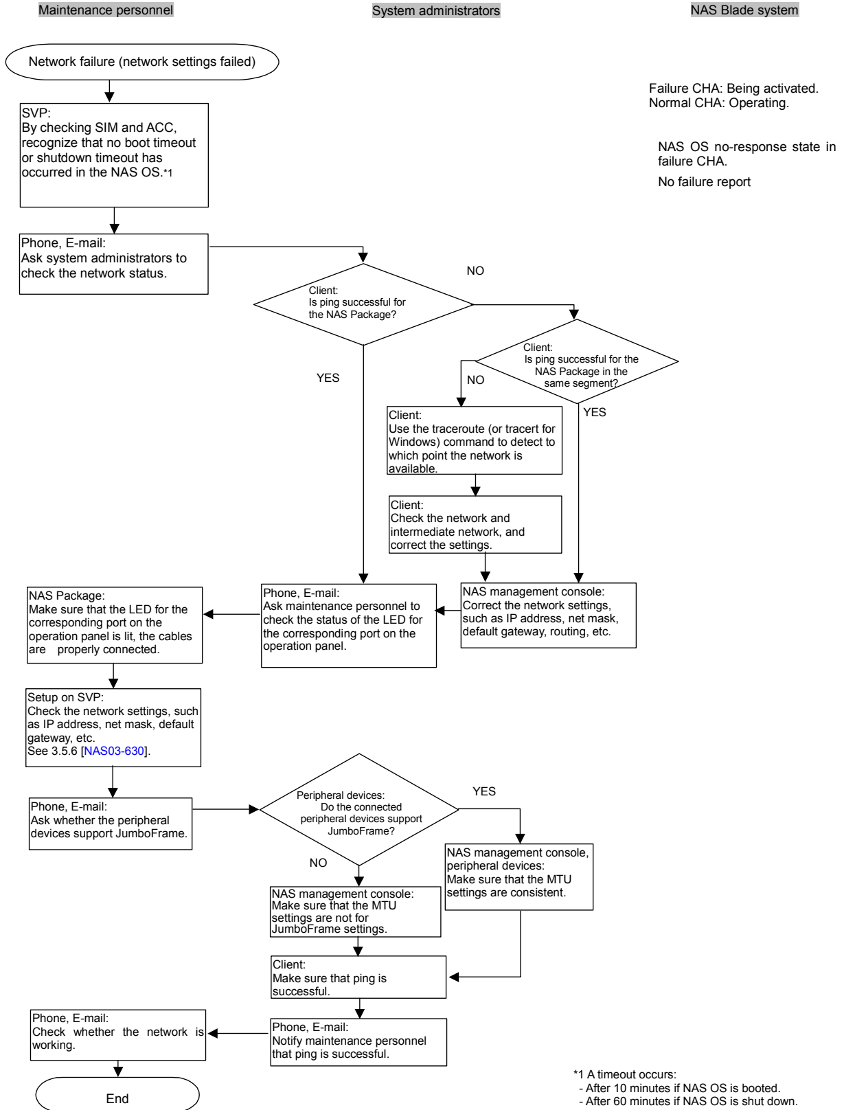
Figure 7.4-12 Network Failure (Network Settings Failed) (2/3)
