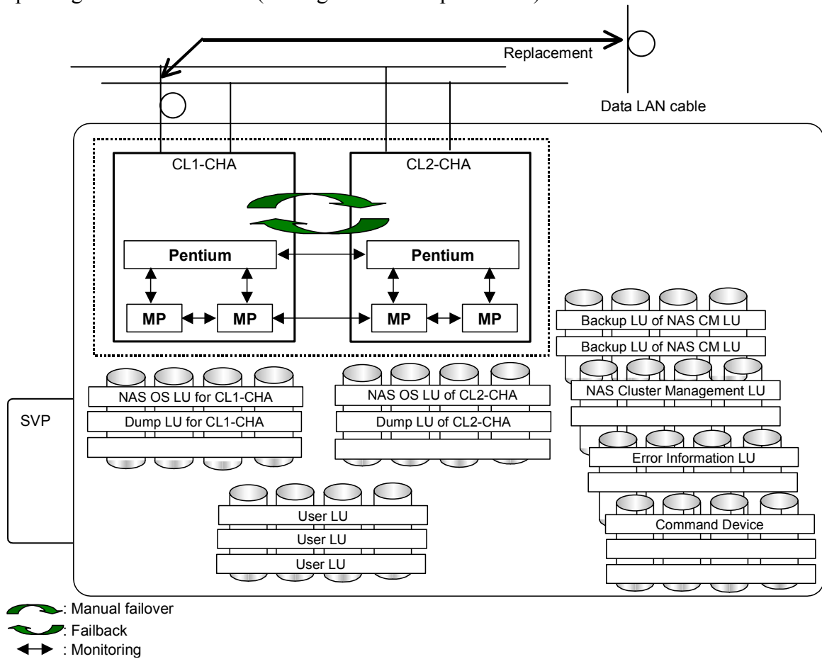
Figure 4.2-2 Replacing Data LAN Cables (During Periodic Replacement) (1/4)
