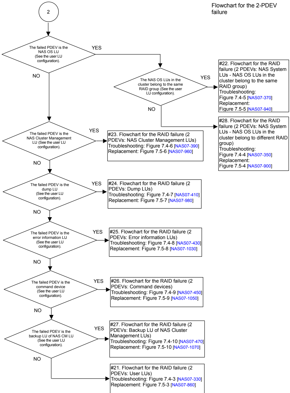
Figure 7.4-0 Flowcharts for Troubleshooting Related to Failure Phenomena (5/11)
