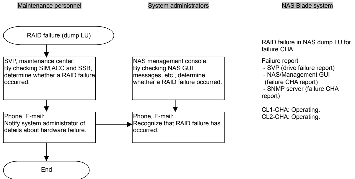
Figure 7.4-7 RAID Failure (2 PDEVs: Dump LUs) (2/2)
