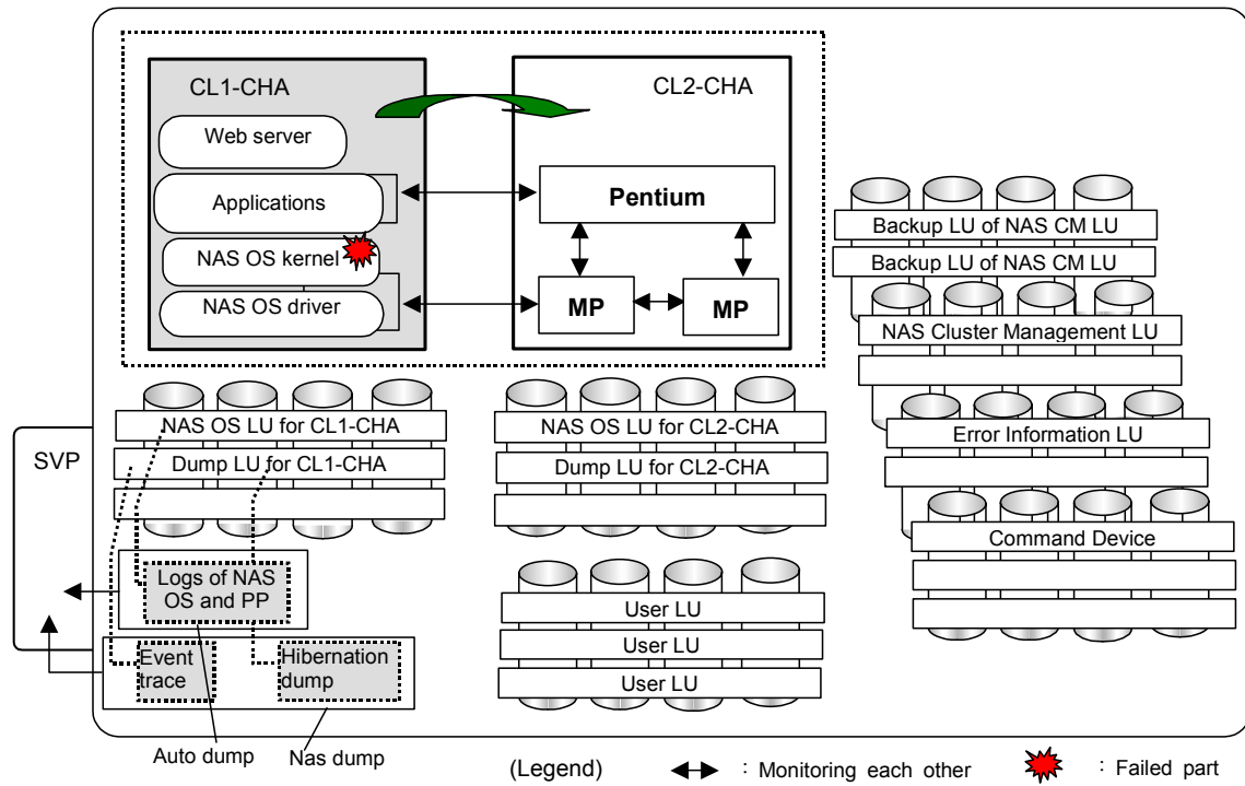
Figure 7.4-14 NAS OS Failure (Hangup) (1/3)
