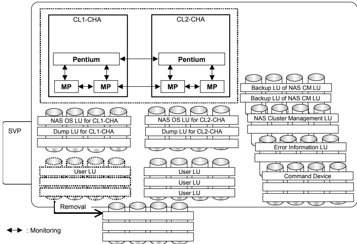
Figure 6.2-2 Removing a RAID Group (User LU)(1/2)
