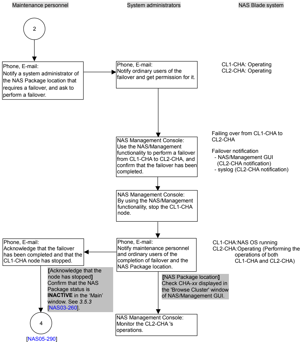
Figure 5.3-3 Upgrading NAS OS By a Patch Version — Restarting the NAS OS Is Required (Preventive Upgrade: While Operating) (3/9)
