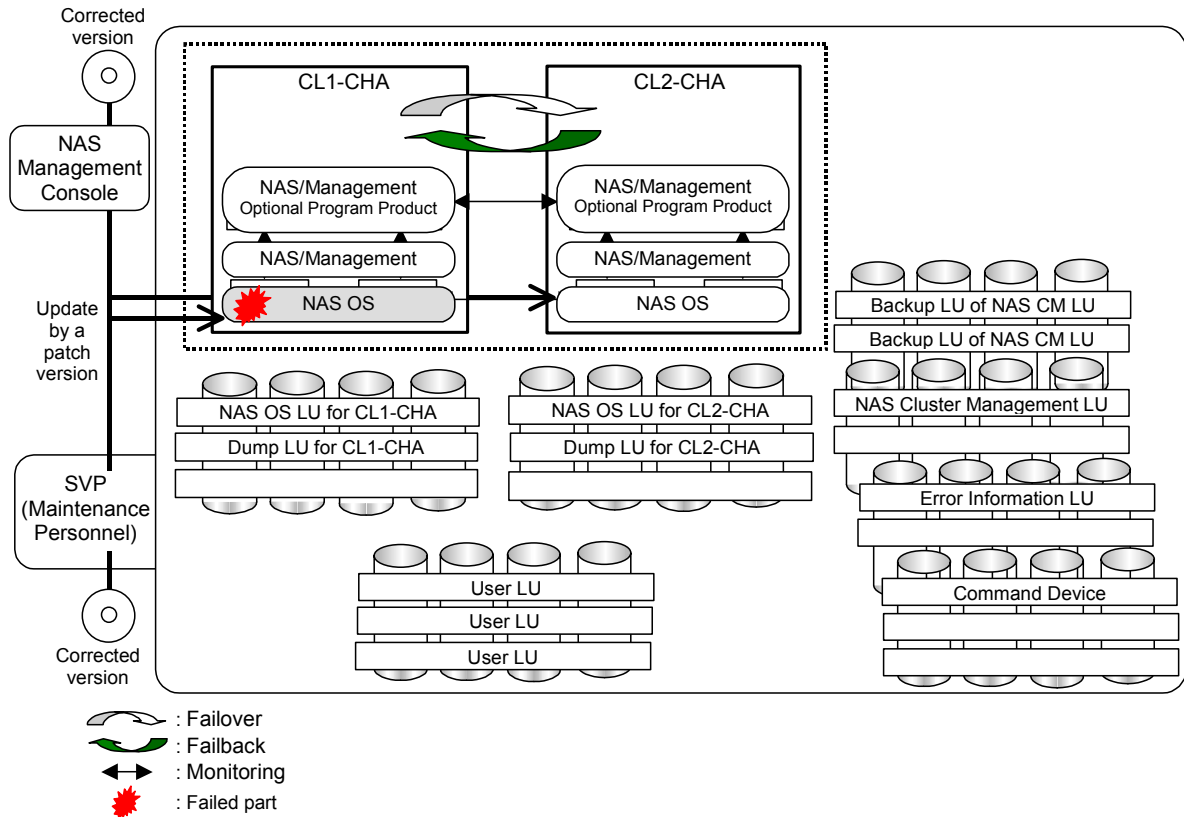
Figure 7.5-14 Upgrading the NAS OS By a Patch Version — Restarting the NAS OS Is Required (When a Failure Occurs) (1/6)
