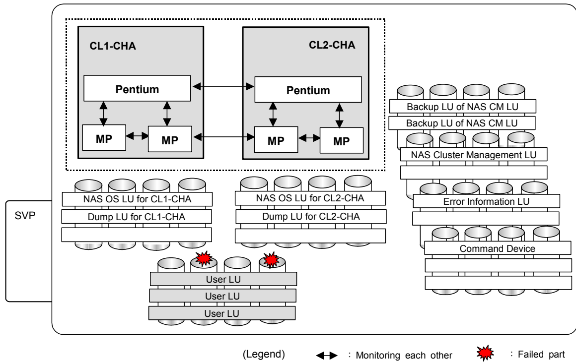
Figure 7.4-3 RAID Failure (User LU) (1/2)
