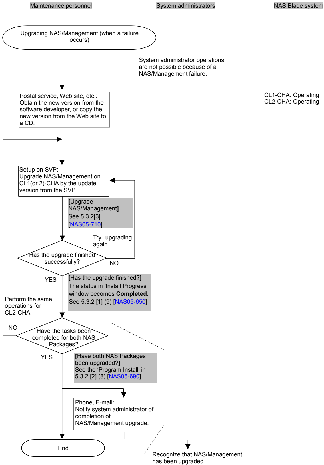
Figure 7.5-15 Upgrading NAS/Management (When a Failure Occurs) (2/2)
