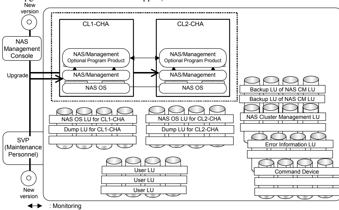
Figure 5.3-6 Replacing the NAS OS By a Patch Version — Restarting the NAS OS Is Required (Preventive Upgrade: While the Cluster is Stopped) (1/7)
