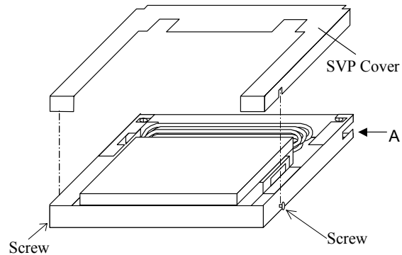
FLORA270HX/FLORA270W type1
