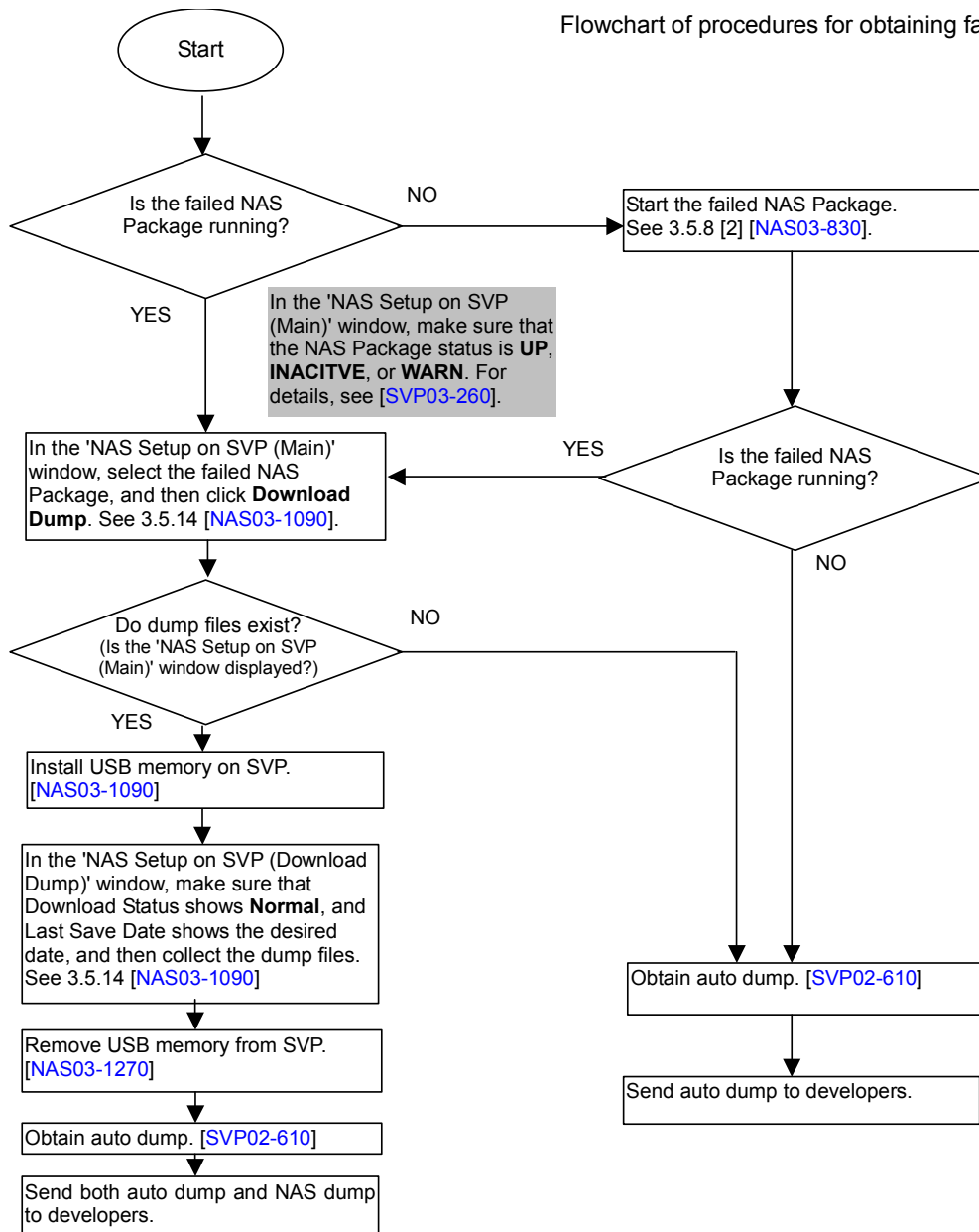
Figure 7.2-1 Flowchart of Procedures for Obtaining Failure Information
