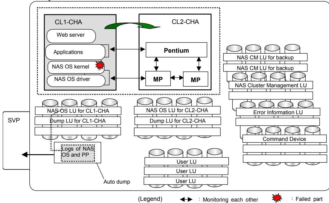
Figure 7.4-21 NAS OS File System Failure (1/3)
