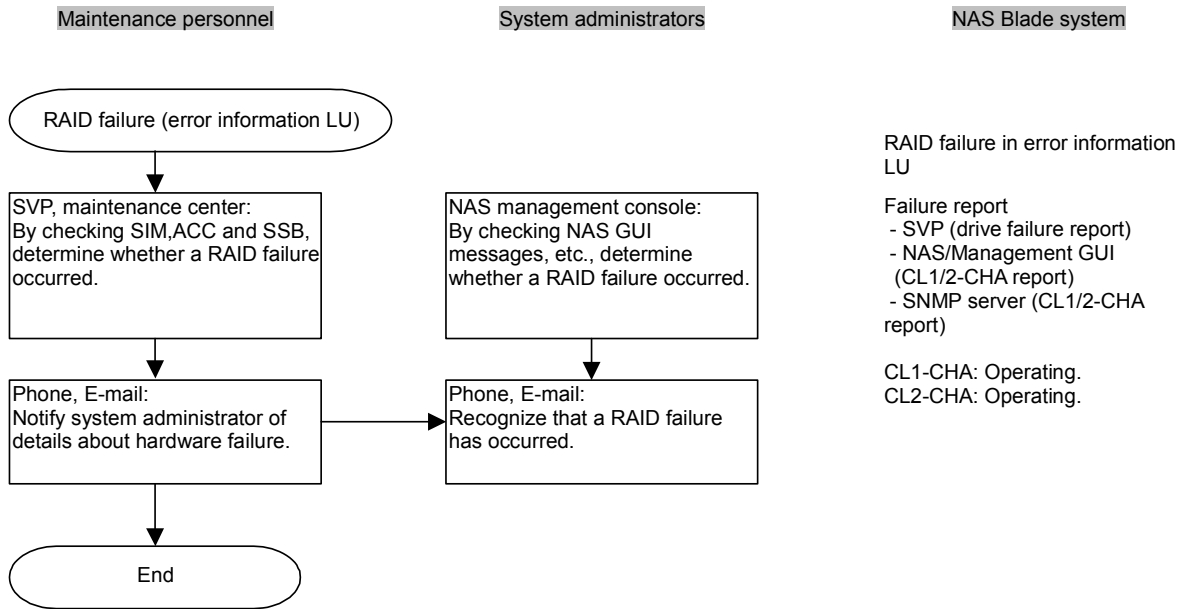
Figure 7.4-8 RAID Failure (2 PDEVs: Error Information LUs) (2/2)
