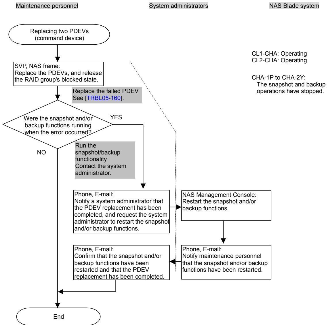
Figure 7.5-9 Replacing Two PDEVs (Command Device) (2/2)
