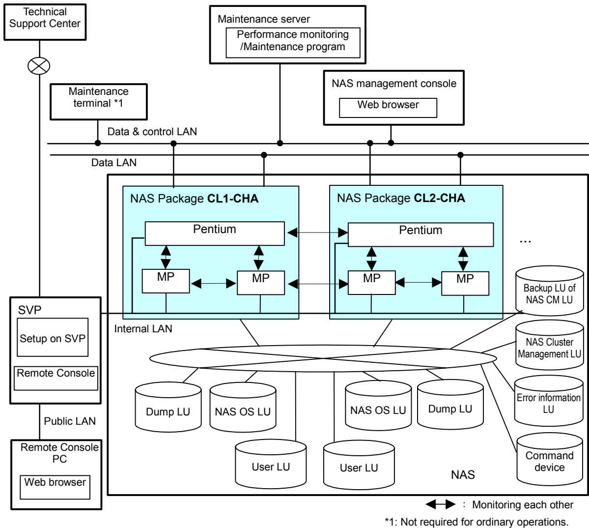
Figure 2.2-1 Hardware Configuration of the NAS Blade System
