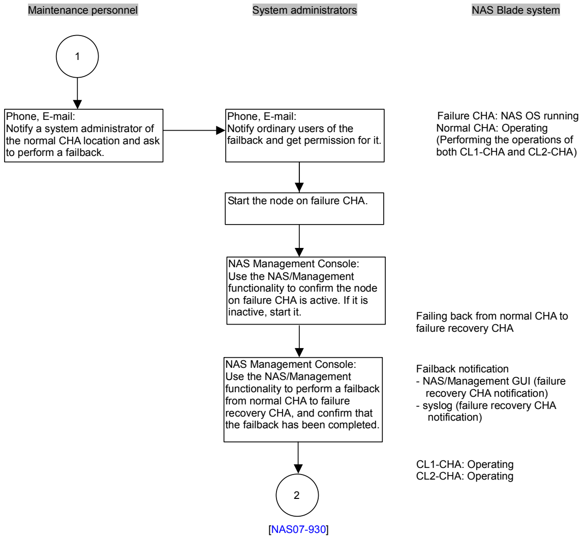
Figure 7.5-4 Replacing Two PDEVs (NAS OS LUs: When the NAS OS LU and the Dump LU Belong to Different RAID Groups) (3/4)
