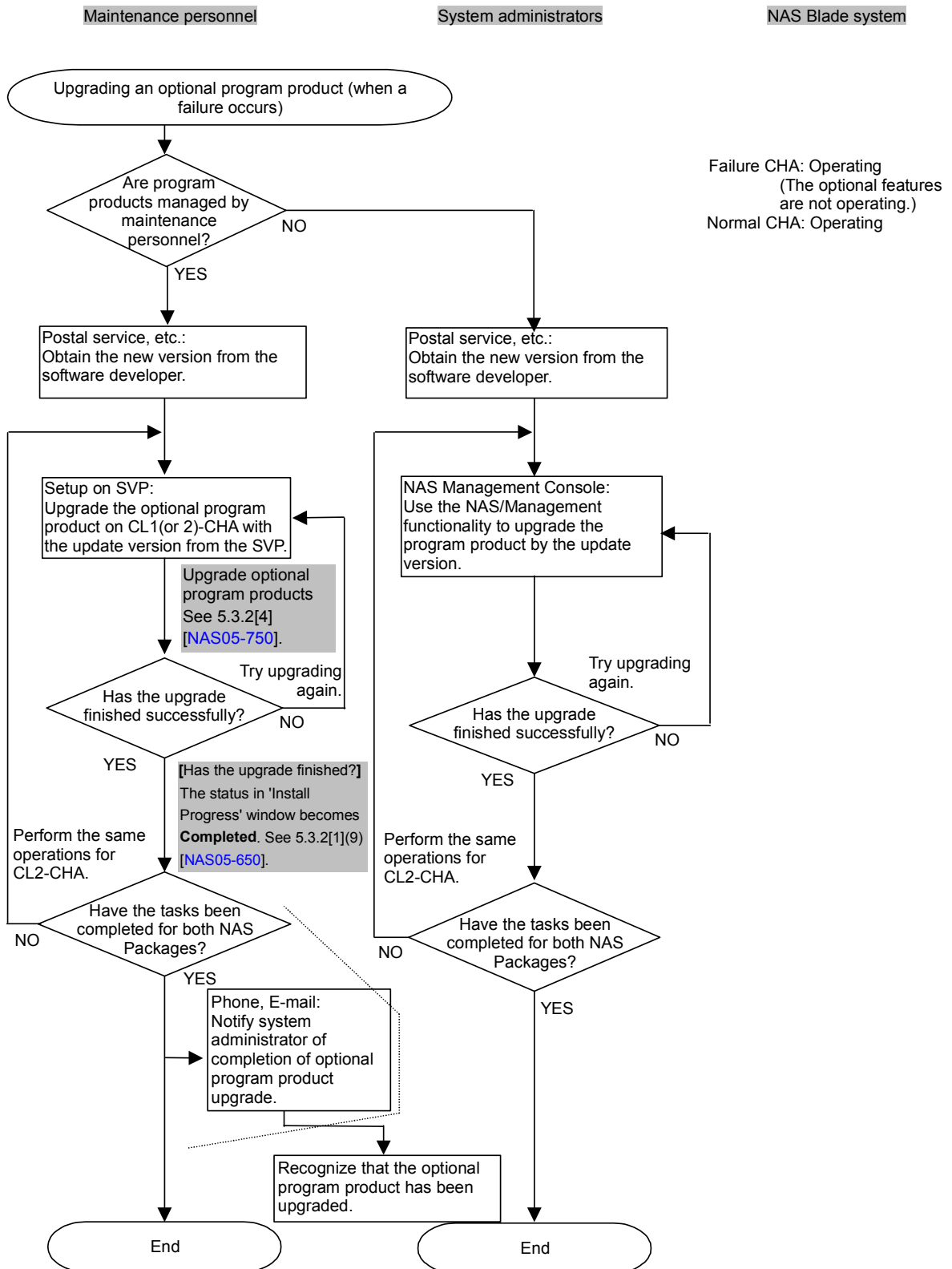
Figure 7.5-16 Upgrading an Optional Program Product (When a Failure Occurs) (2/2)
