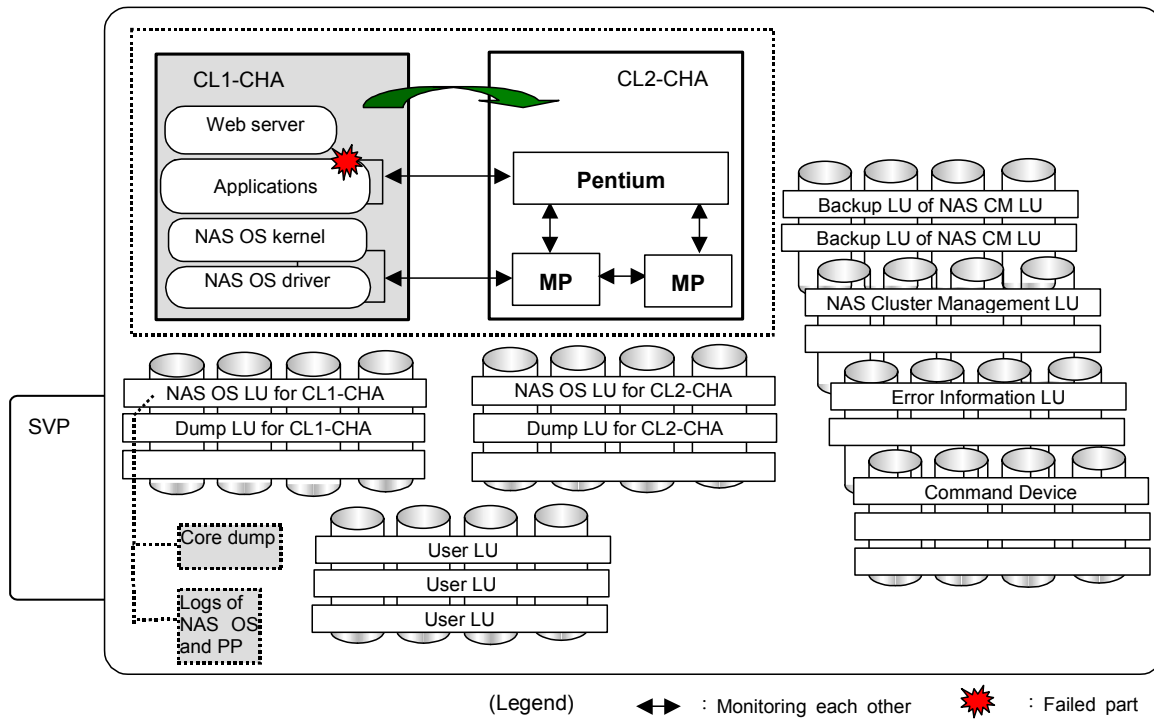
Figure 7.4-16 Application Failure (Failover Provided) (1/3)
