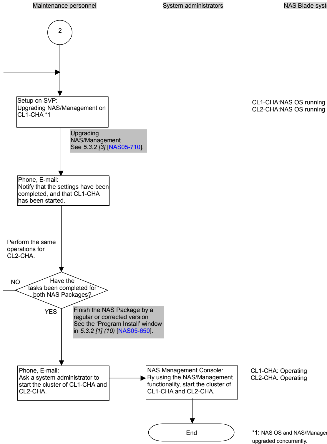
Figure 5.3-4 Upgrading NAS OS by an Updated Version (Preventive Upgrade: While the Cluster is Stopped) (4/4)
