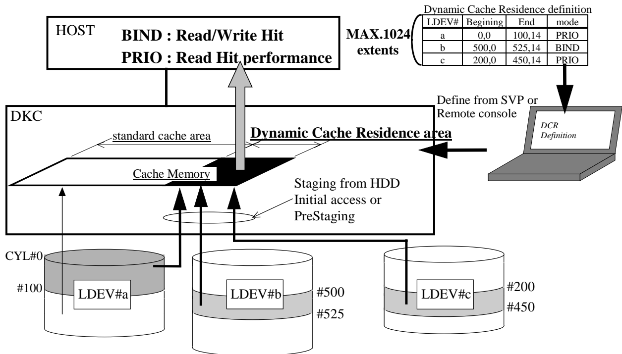
Fig. 2.2 Conceptual Diagram of DCR
