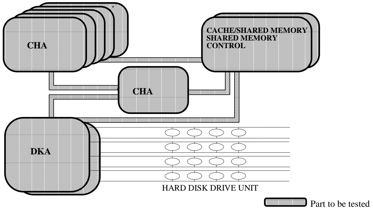
Fig. 3-1 Parts that are Subject to CUDG3/CUDG4 Tests
