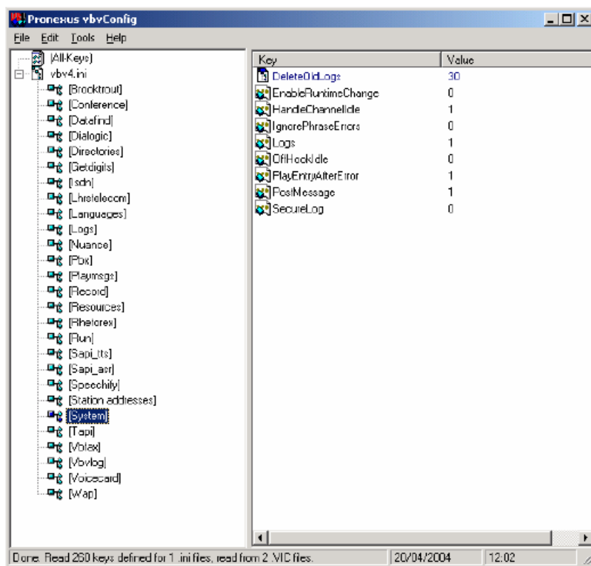
Figure 133: vbvConfig - System
