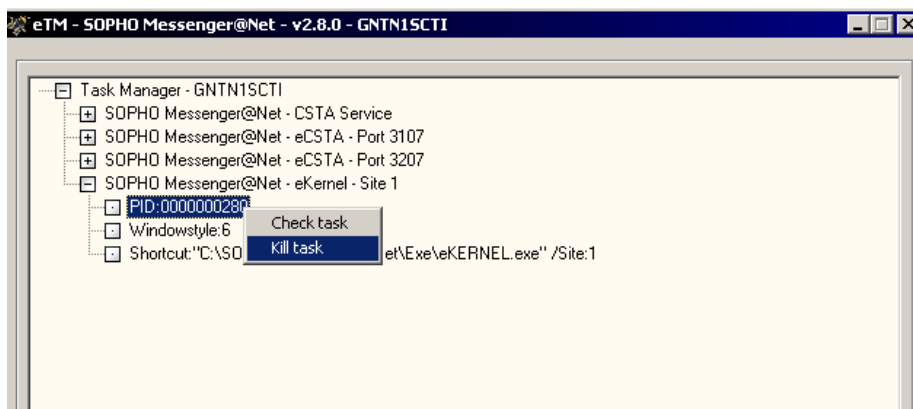
Figure 86: Kill Task
