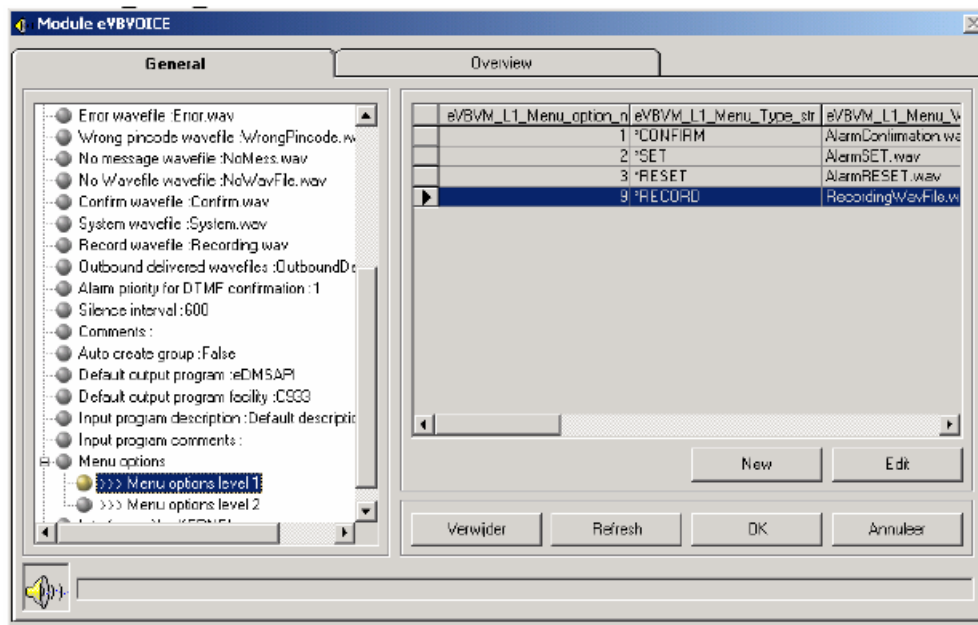
Figure 104: eVBVOICE_Menu_L1
