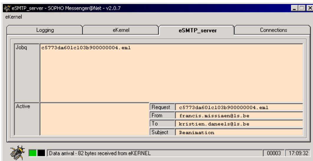
Figure 27: Mail processing
