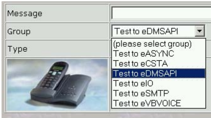
Figure 147: Group list
