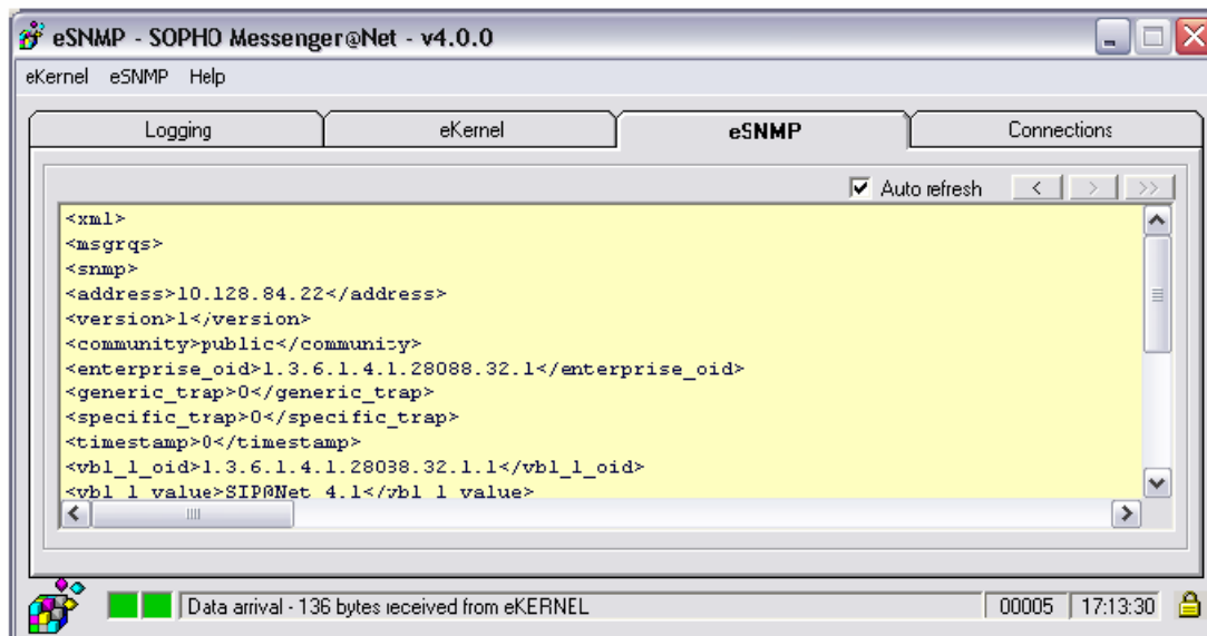
Figure 40: eSNMP traps
