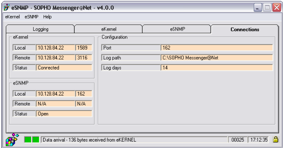
Figure 39: eSNMP connections
