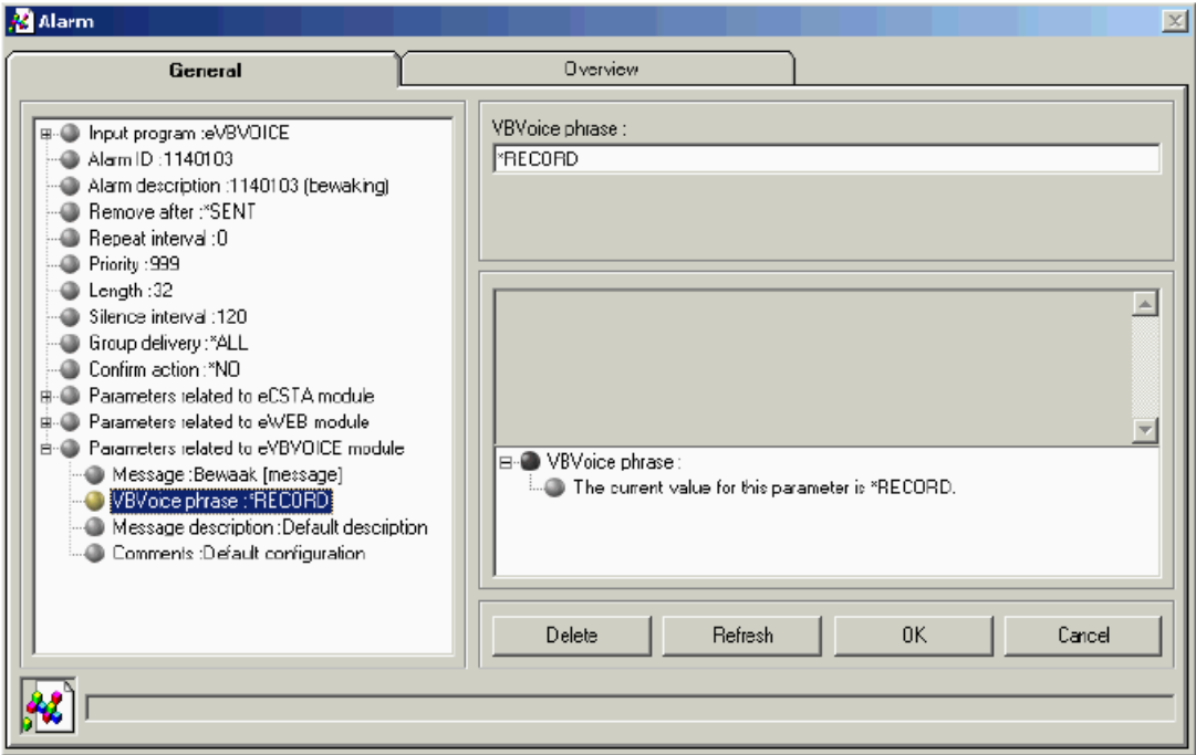
Figure 136: RECORD
