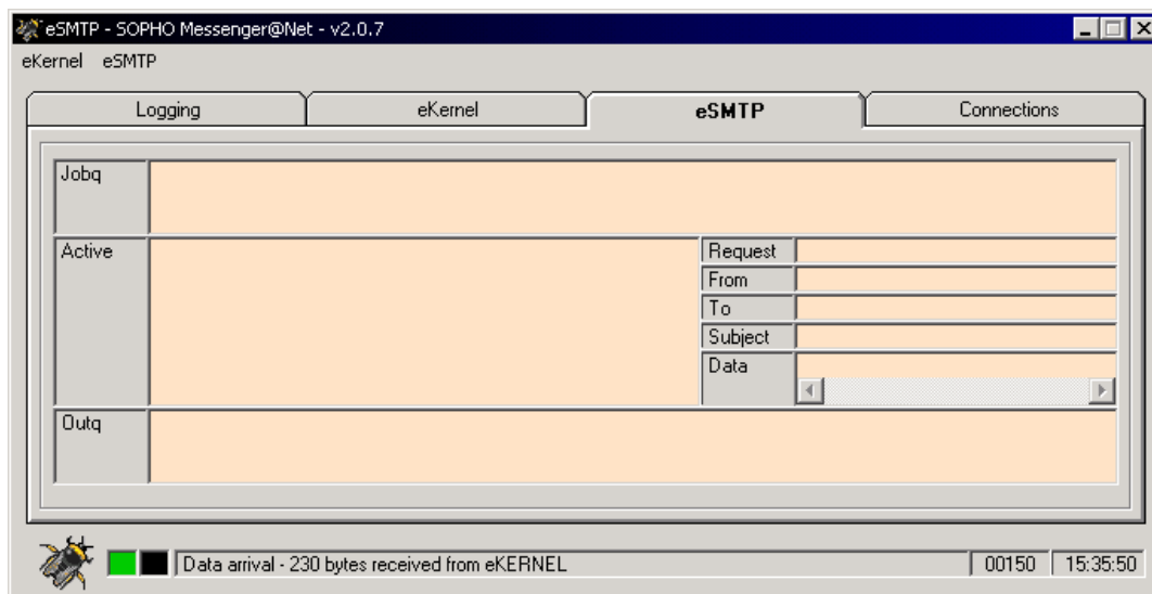
Figure 5: eSMTP tab
