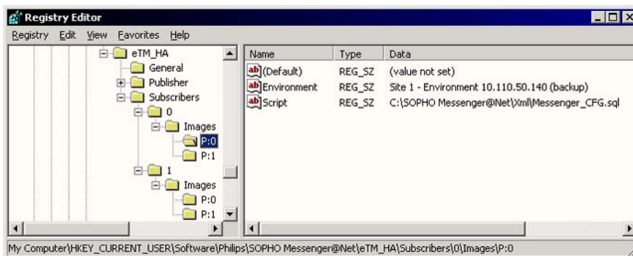
Figure 92: Registry definitions
