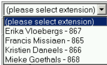
Figure 143: Local extensions
