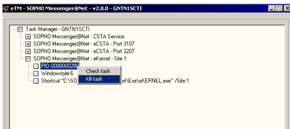
Figure 66: Kill Task
