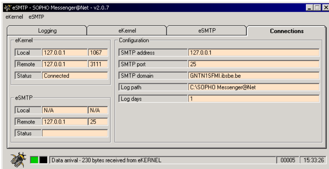
Figure 3: Configuration information
