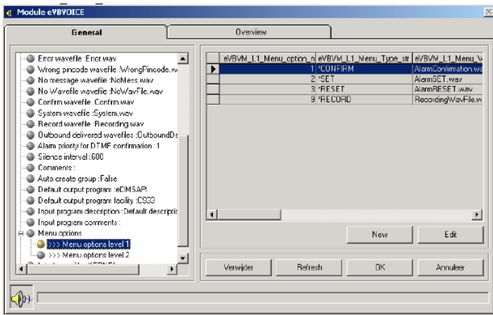
Figure 105: eVBVOICE_Menu_L2
