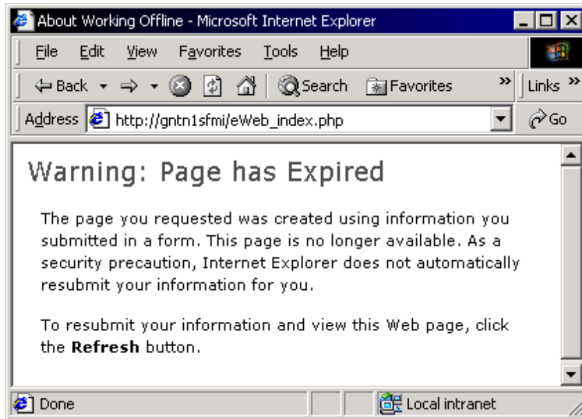
Figure 142: Expired login
