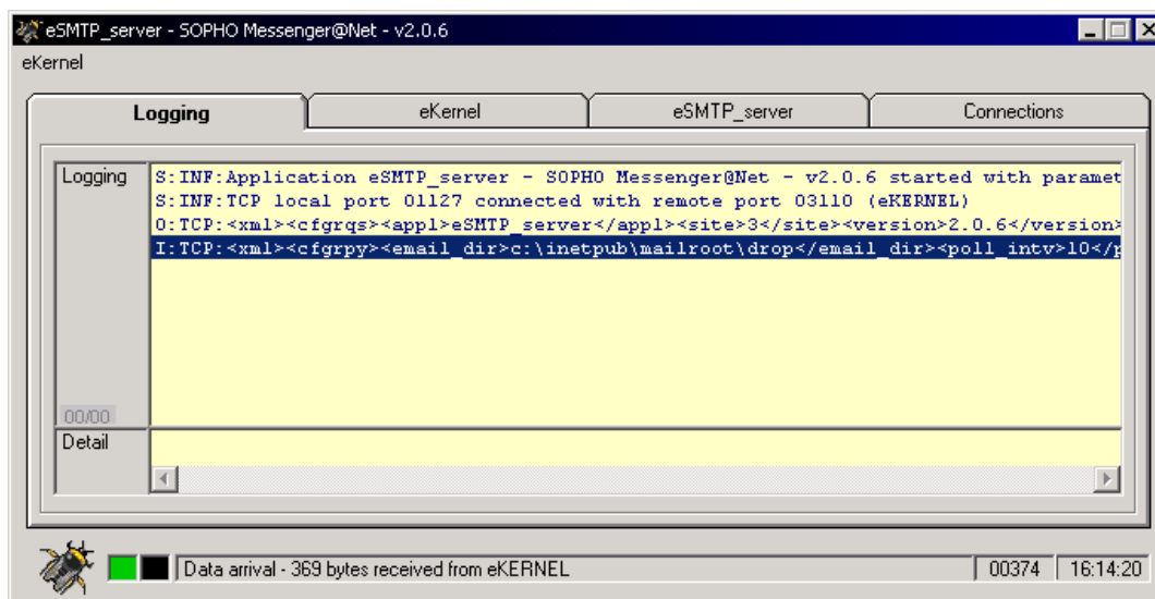
Figure 33: On-screen logging
