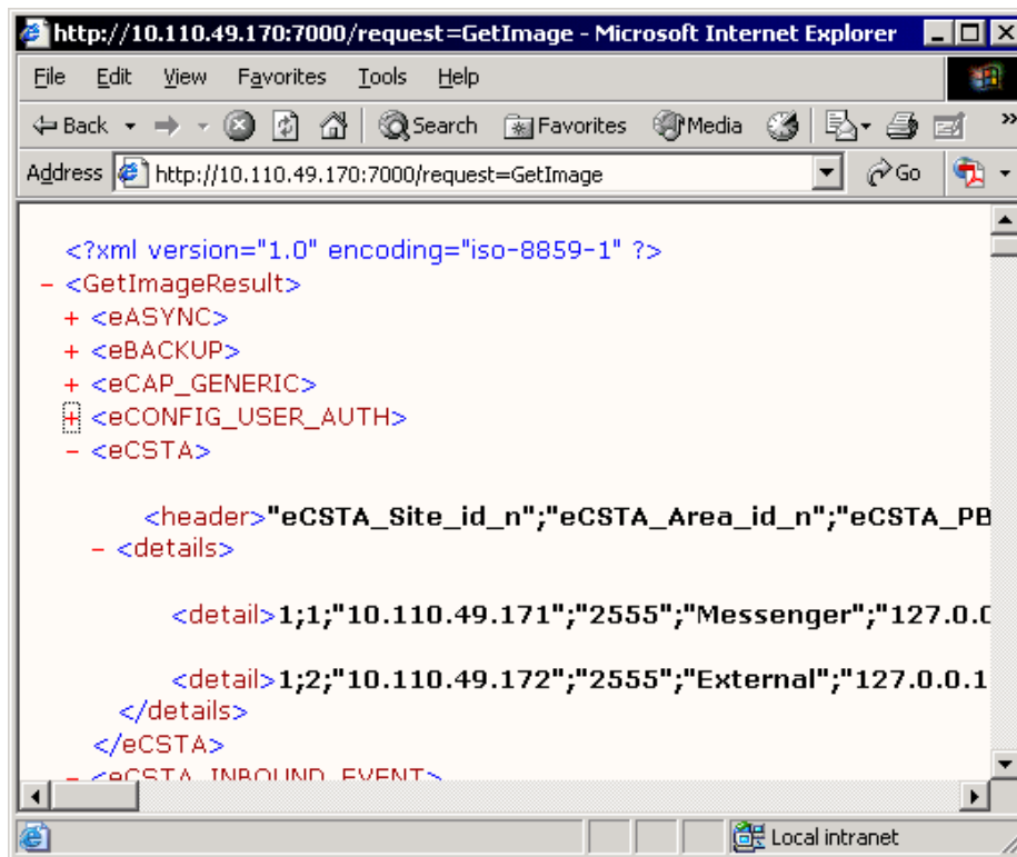
Figure 91: Expanded information
