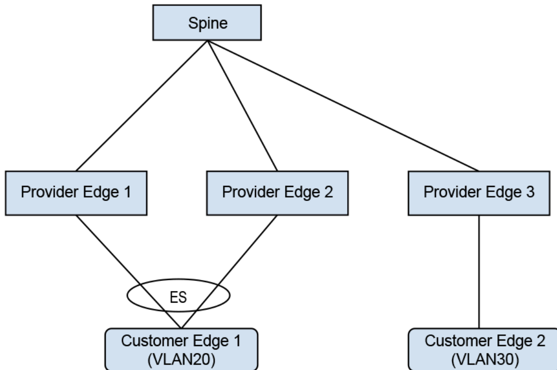
Figure 18-44: Asymmetric IRB with IPv4
