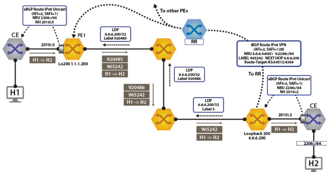
Figure 18-70: IPv6 VPN Forwarding Over LDP MPLS
