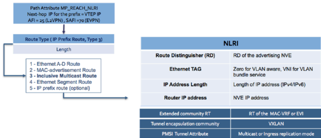
Figure 18-16: EVPN Type-3 IMET Route Format
