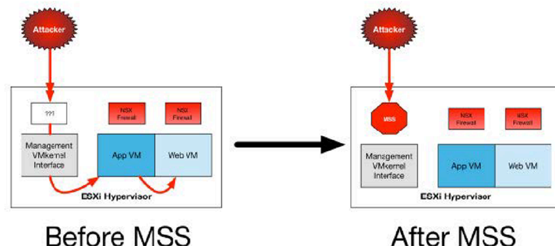
Figure 9-12: Monitoring and Securing management traffic
