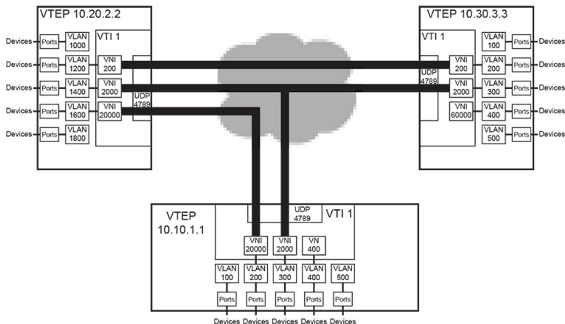
Figure 17-2: VXLAN Implementation
