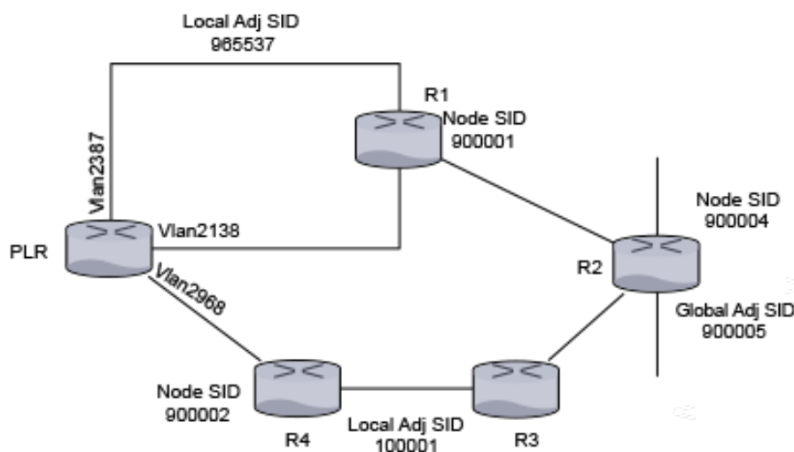
Figure 15-12: Sample Configuration
