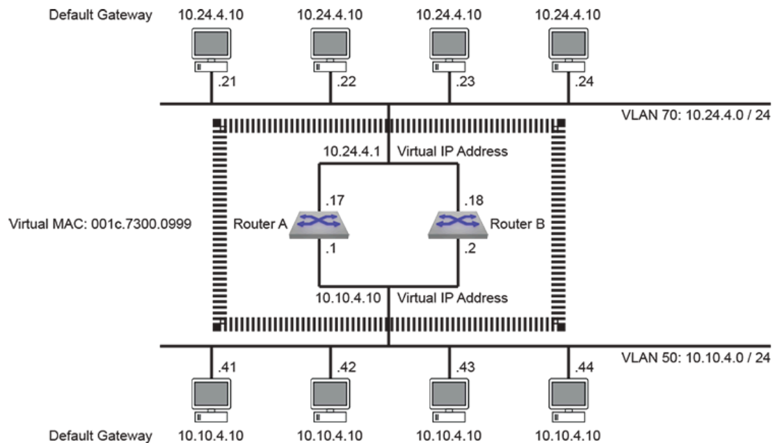
Figure 13-6: VARP Example Network Diagram
