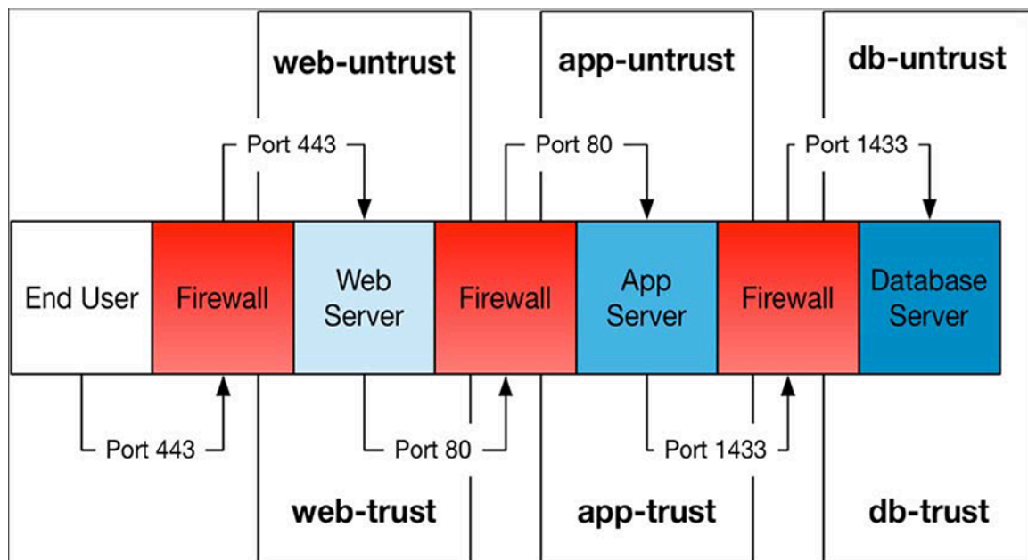
Figure 9-15: Traffic flow in an MSS deployment
