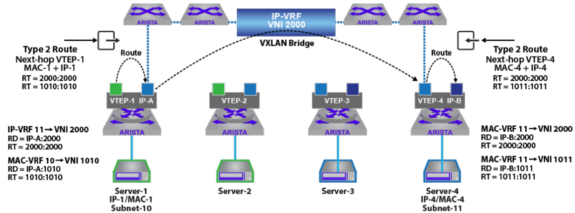
Figure 18-20: EVPN Symmetric IRB
