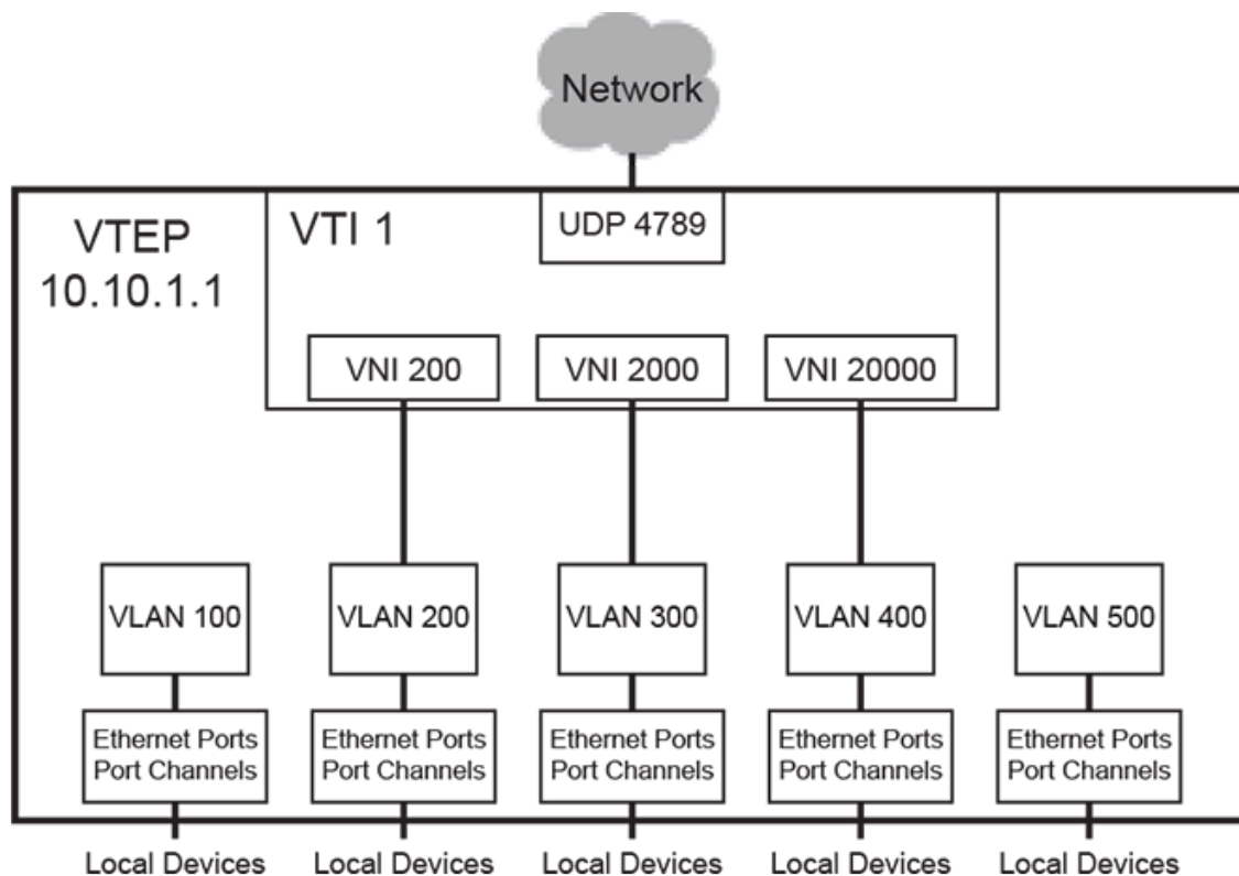
Figure 17-1: VXLAN Architecture
