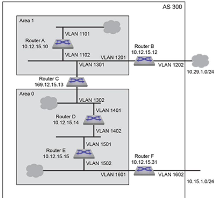
Figure 15-10: OSPFv3 Example 3
