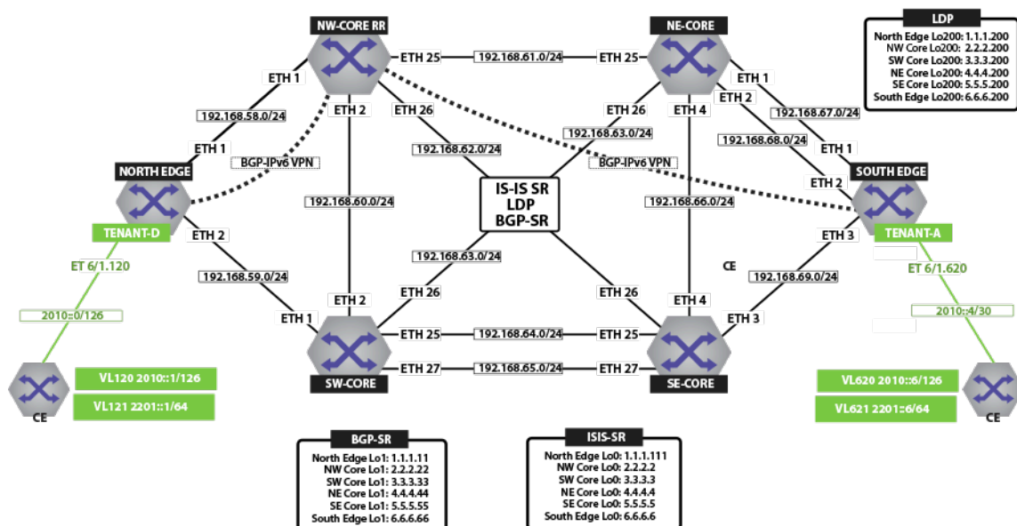
Figure 18-64: IPv6 VPN Physical Topology
