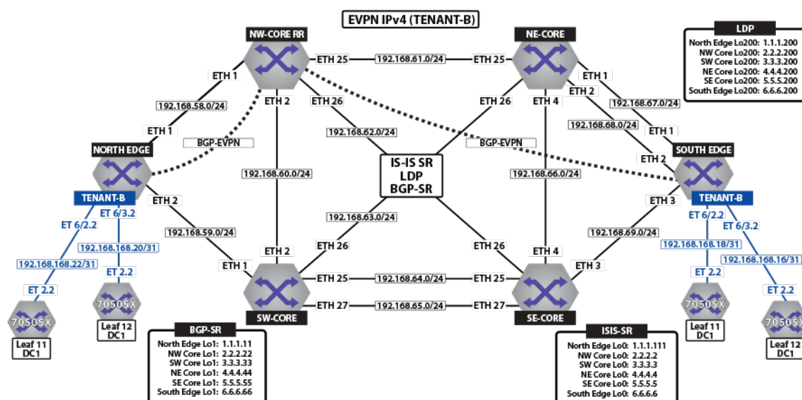
Figure 18-31: Tenant-B DCI
