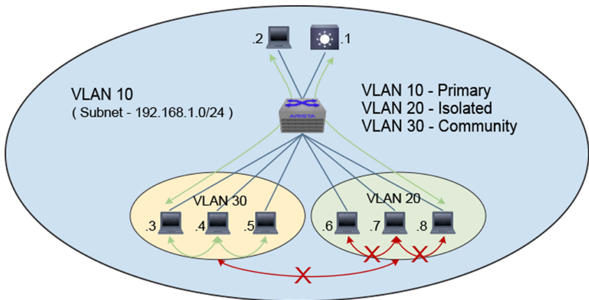
Figure 12-2: Support for Private VLAN
