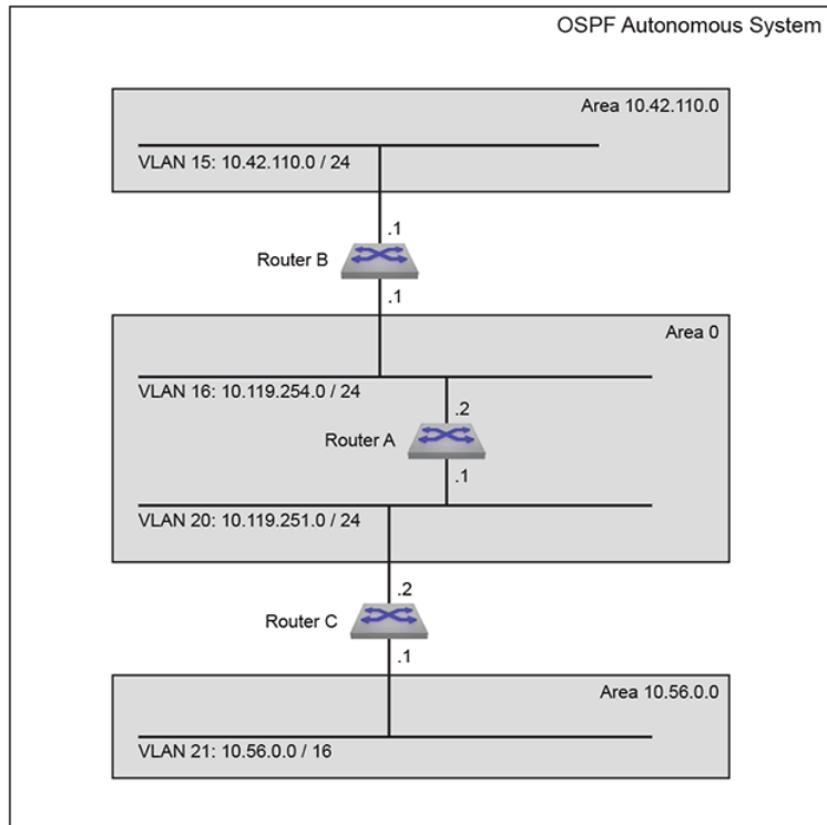
Figure 15-4: OSPFv2 Example 2
