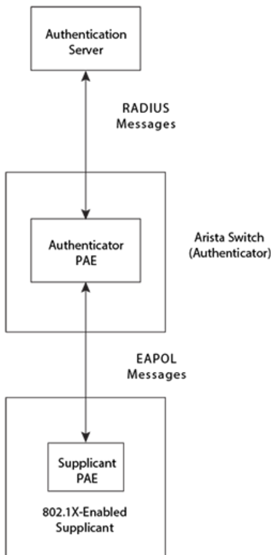
Figure 9-4: Authenticator PAE and Supplicant PAE
