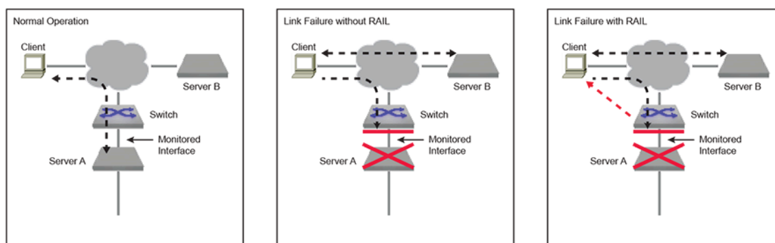
Figure 11-5: RAIL Scenarios
