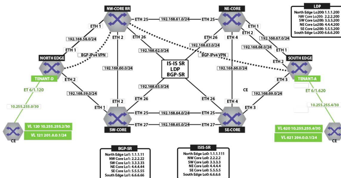
Figure 18-63: IPv4 VPN Physical Topology
