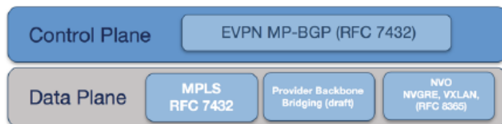
Figure 18-2: VXLAN Control Plane and Data-plane Definitions
