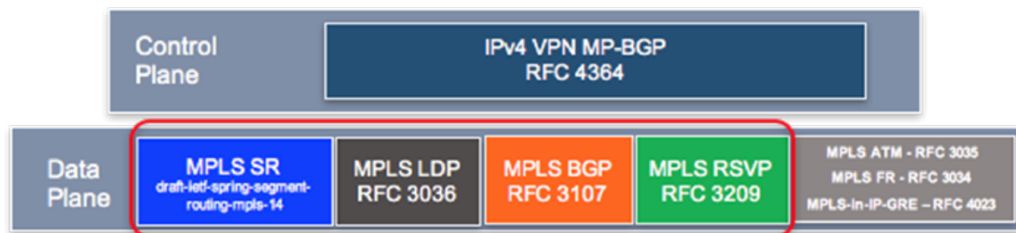
Figure 18-23: MPLS Data-Plane
