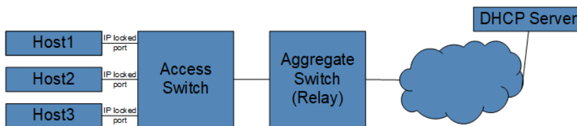
Figure 12-3: IP Address Locking
