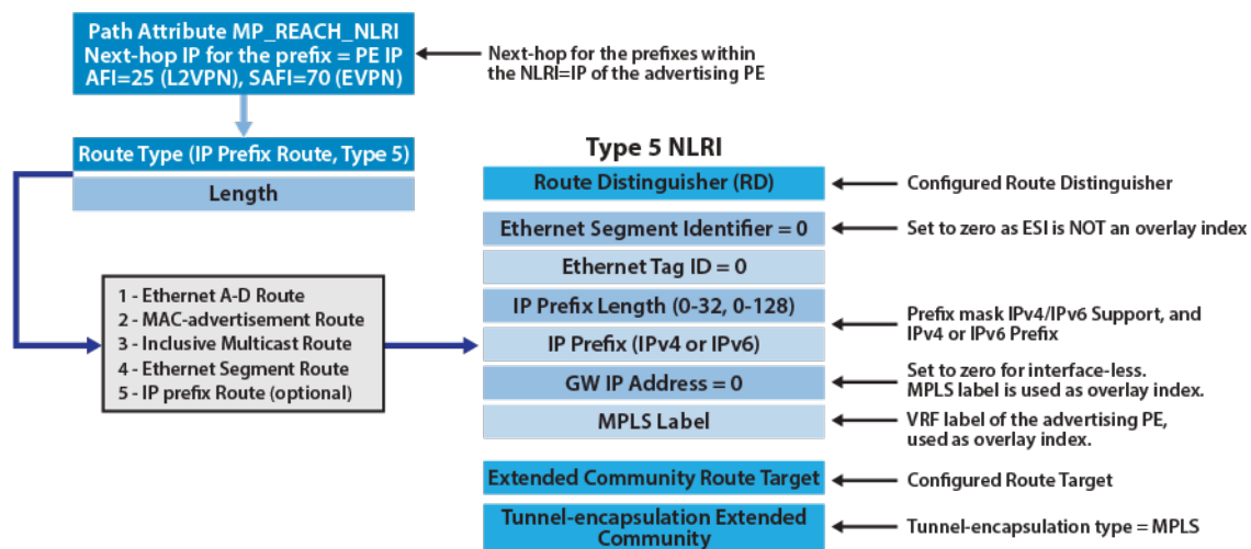
Figure 18-10: EVPN Route Type-5, for Advertisement of IP-Prefixes over MPLS
