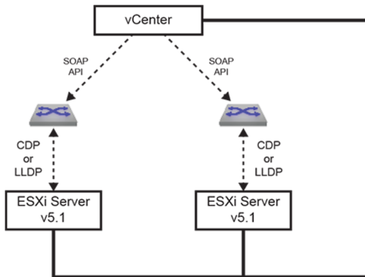
Figure 20-3: VM Tracer Topology – Monitoring VLAN Based Configurations
