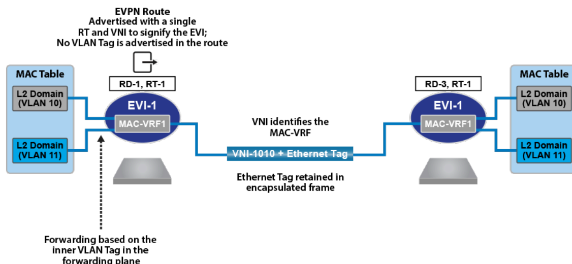
Figure 18-7: VLAN Bundle Service Interface
