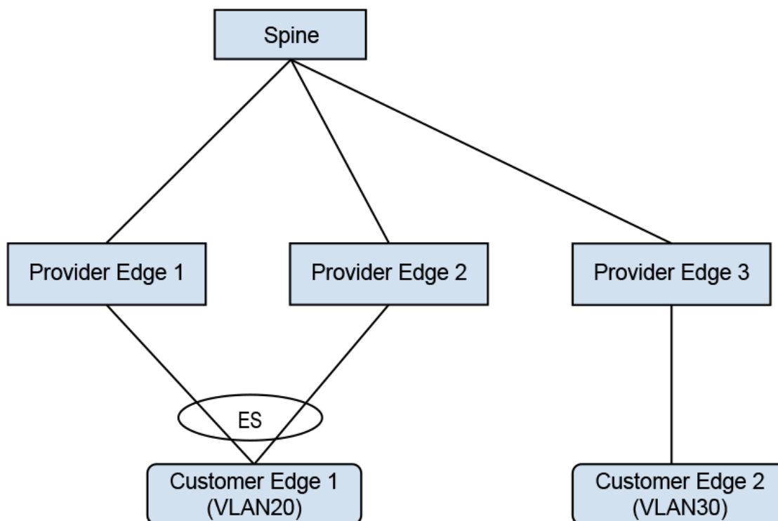
Figure 18-49: Asymmetric IRB with IPv4
