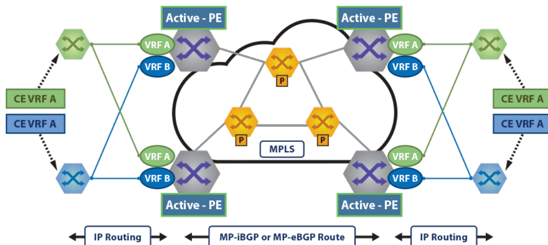
Figure 18-28: MPLS Layer 3 VPN Topology
