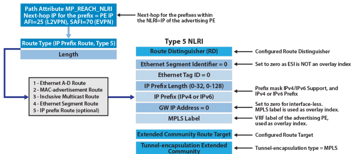
Figure 18-39: EVPN Route Type-5, for Advertisement of IP Prefixes
