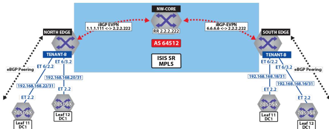
Figure 18-55: Control Plane Tenant-B over ISIS-SR
