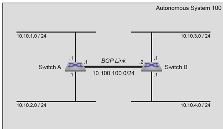
Figure 15-16: BGP Example 1
