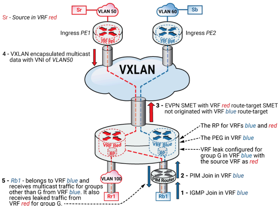
Figure 18-48: Figure 2 - Multicast Traffic Flow with VRF Leaking on the PEG
