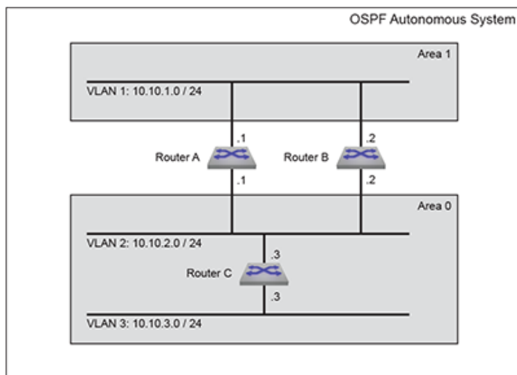
Figure 15-3: OSPFv2 Example 1
