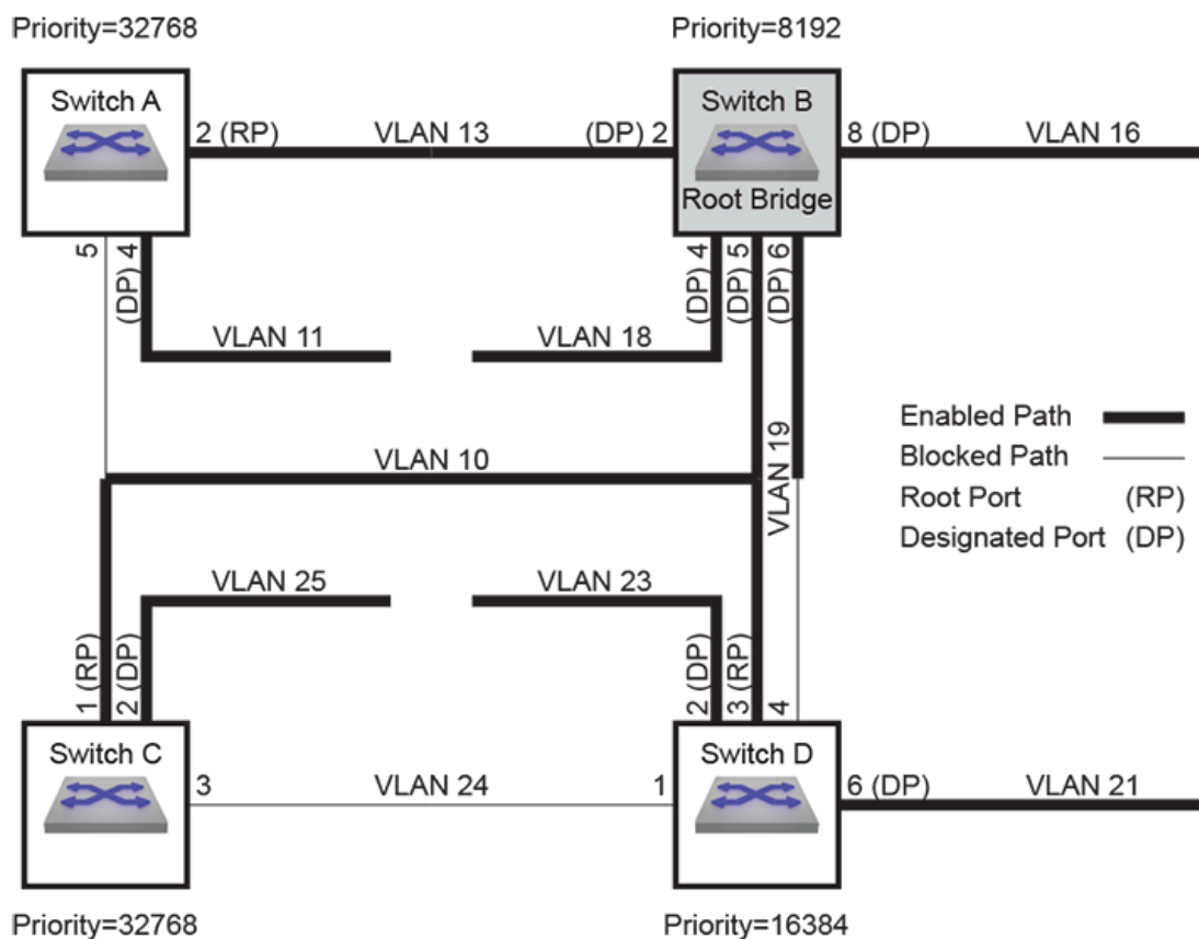
Figure 12-1: Spanning Tree Network Example
