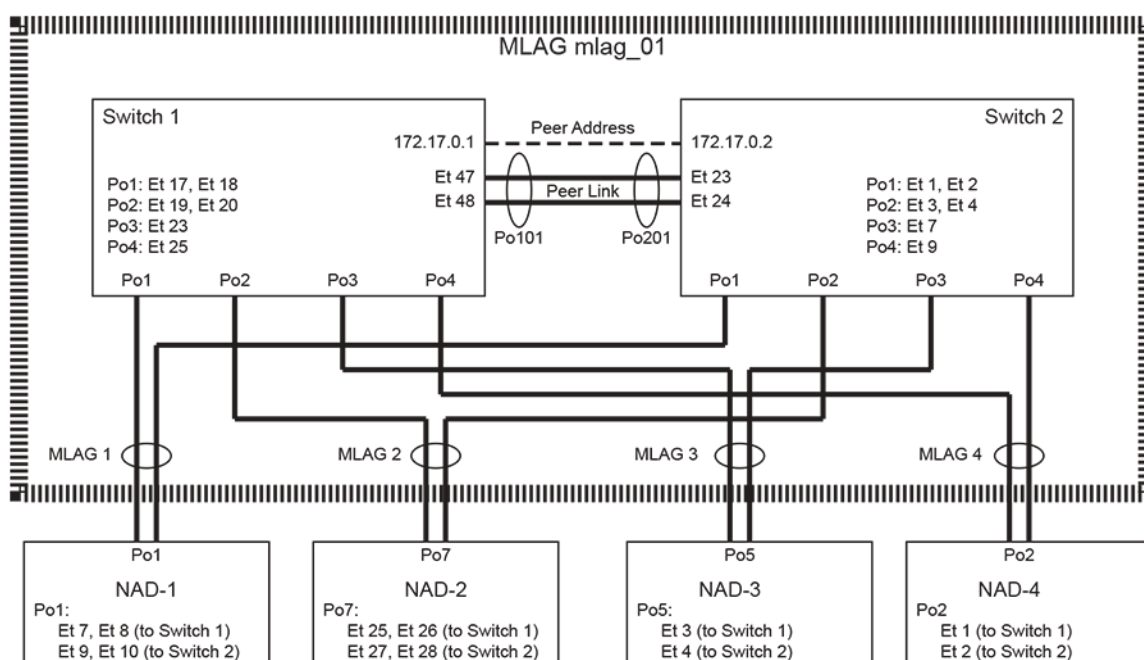
Figure 11-3: MLAG Implementation Example
