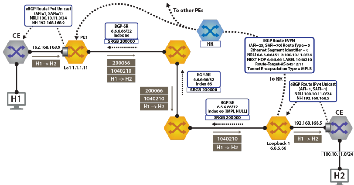
Figure 18-62: Control Plane and Forwarding Tenant-A Over BGP-SR
