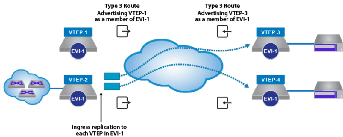
Figure 18-15: EVPN type-3 IMET Route Behavior for Ingress Replication
