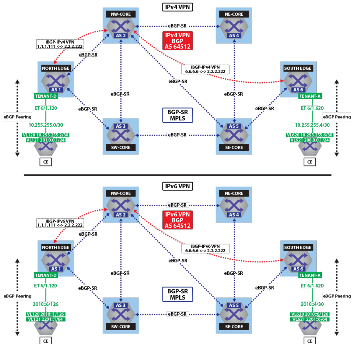
Figure 18-71: IPv4 VPN and IPv6 VPN Over BGP-SR MPLS
