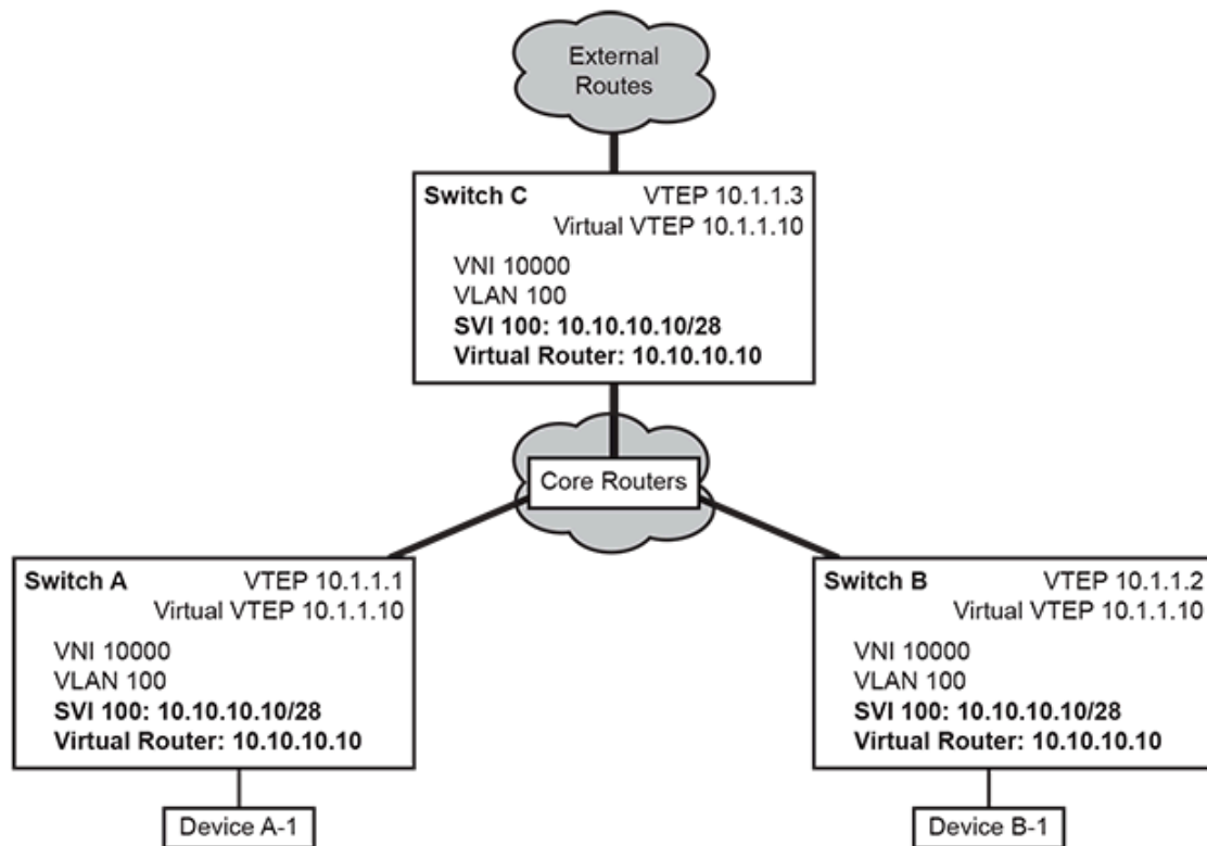
Figure 17-4: Direct VXLAN Routing
