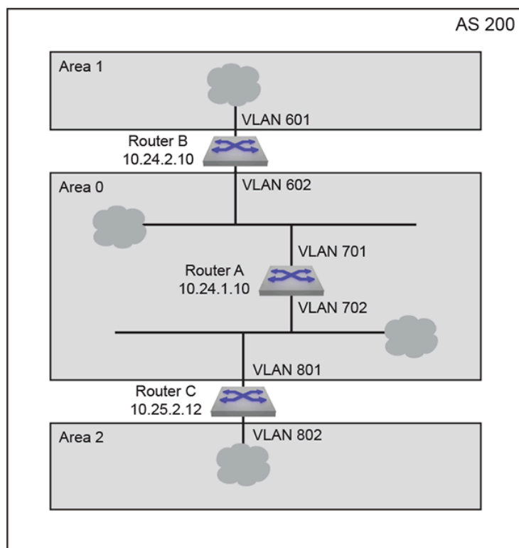
Figure 15-9: OSPFv3 Example 2
