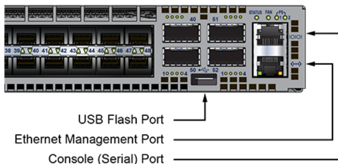
Figure 3-1: Switch Ports
