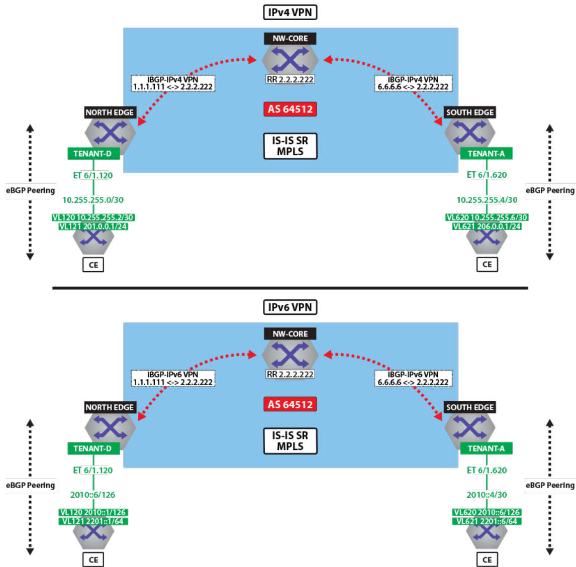
Figure 18-65: IPv4 VPN and IPv6 VPN Over ISIS-SR MPLS
