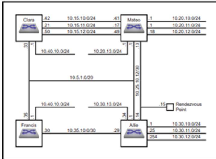
Figure 16-4: Multicast Example
