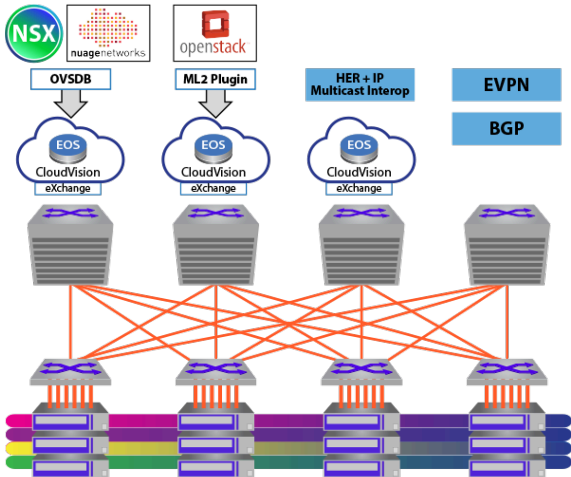
Figure 18-1: Different VXLAN Control Planes
