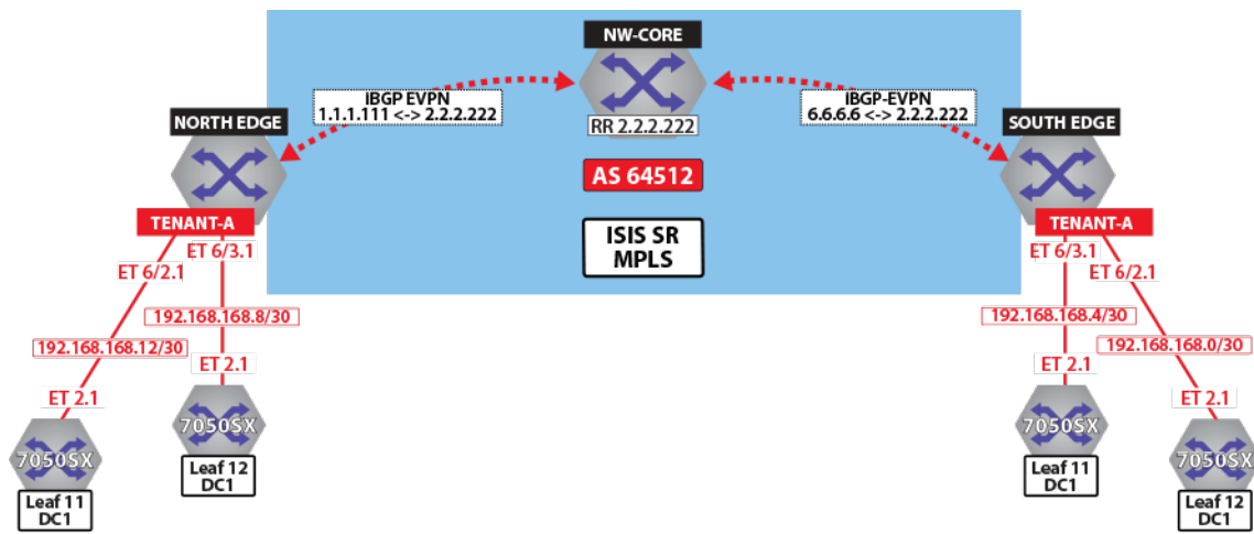
Figure 18-57: Control Plane Tenant-A Over LDP
