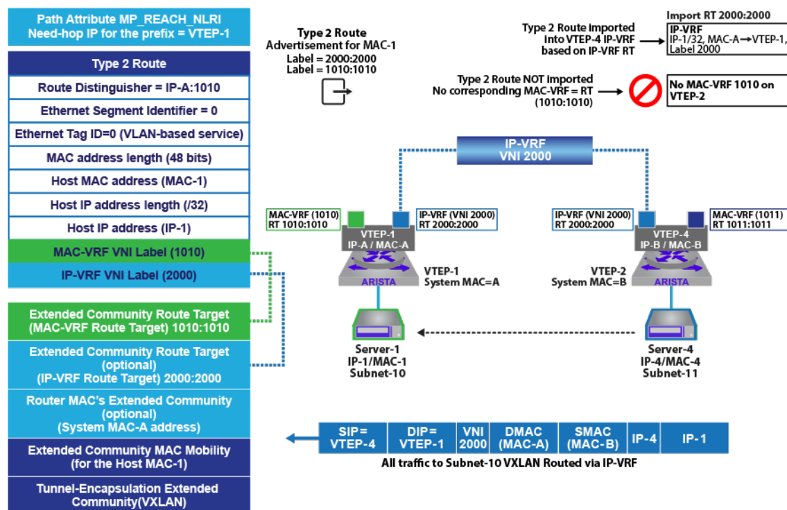
Figure 18-22: EVPN Type 2 Route in Symmetric IRB - MAC-VRF Only Exists on Sending VTEP
