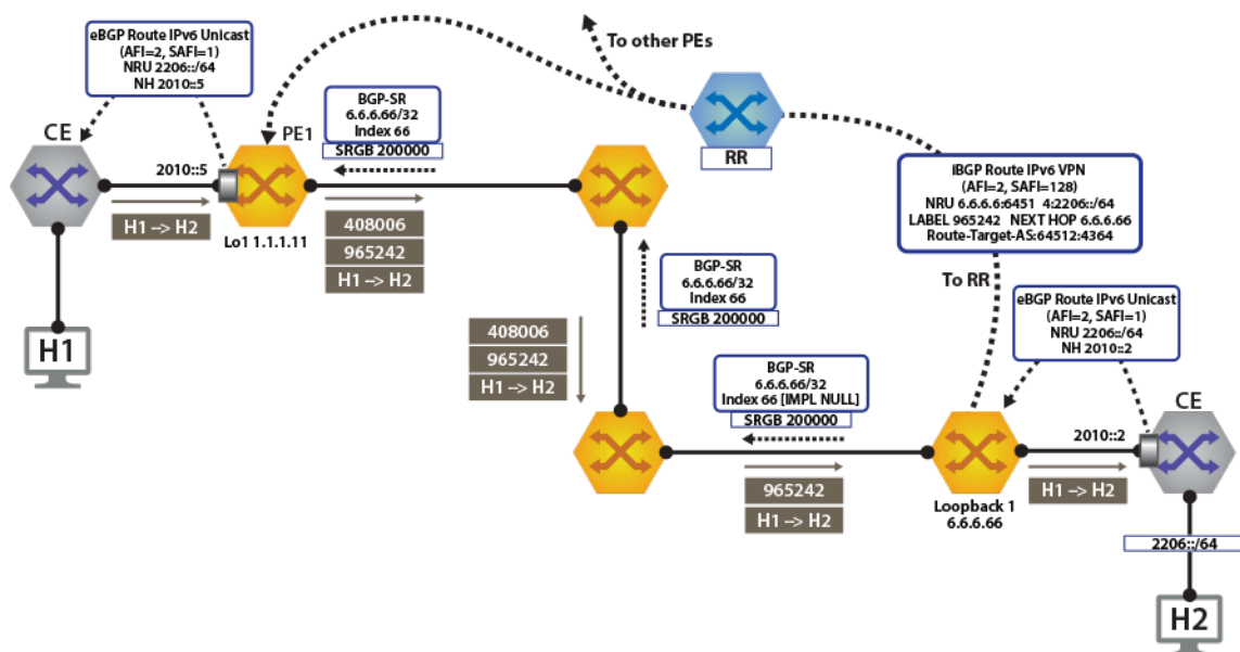
Figure 18-73: IPv6 VPN Forwarding Over BGP-SR MPLS
