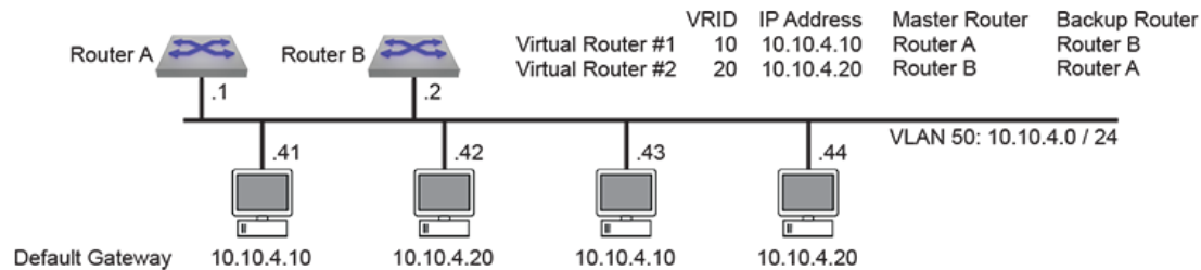
Figure 13-4: VRRP Example 2 Network Diagram
