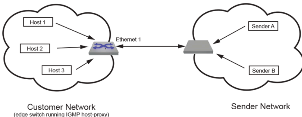
Figure 16-3: IP IGMP Host Proxy Implementation
