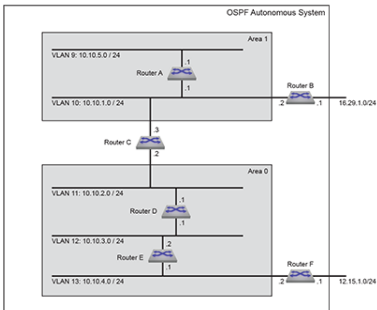
Figure 15-5: OSPFv2 Example 3
