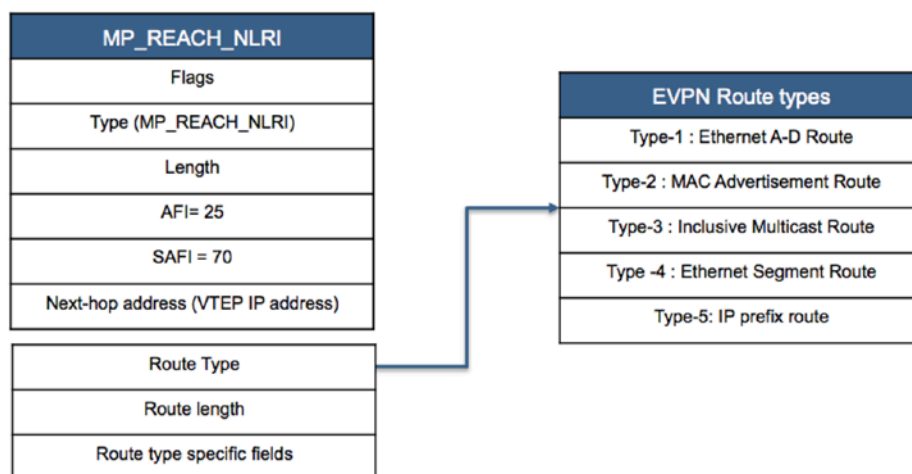
Figure 18-4: EVPN NLRI Route Format
