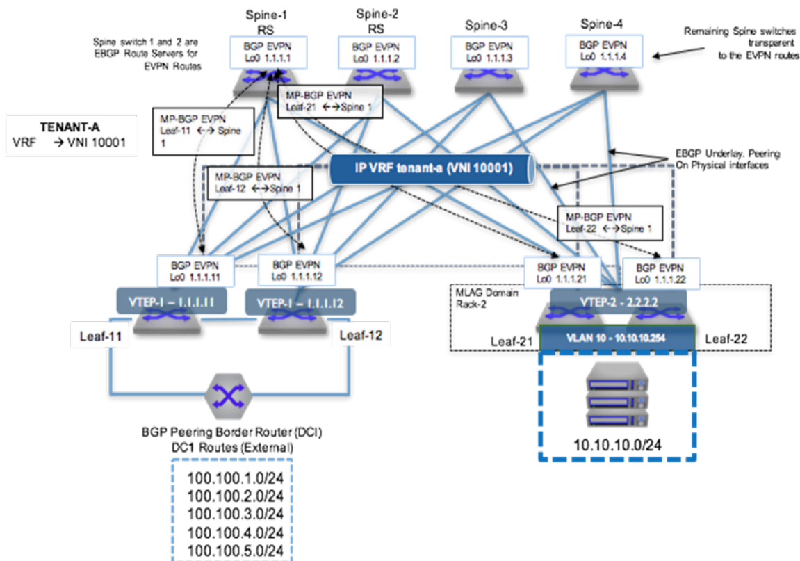
Figure 18-50: Layer 3 EVPN Configuration
