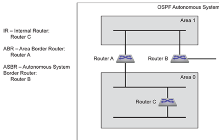
Figure 15-1: OSPFv2 Router Types
