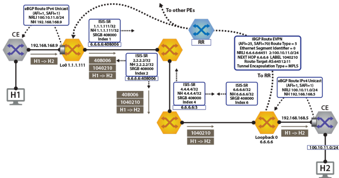
Figure 18-56: Control Plane and Forwarding Tenant-A Over ISIS-SR
