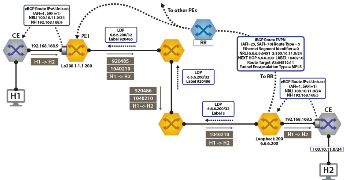
Figure 18-59: Control Plane & Forwarding Tenant-A Over LDP
