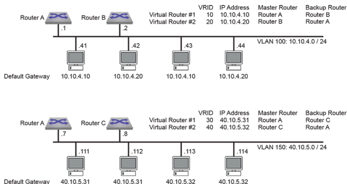
Figure 13-5: VRRP Example 3 Network Diagram
