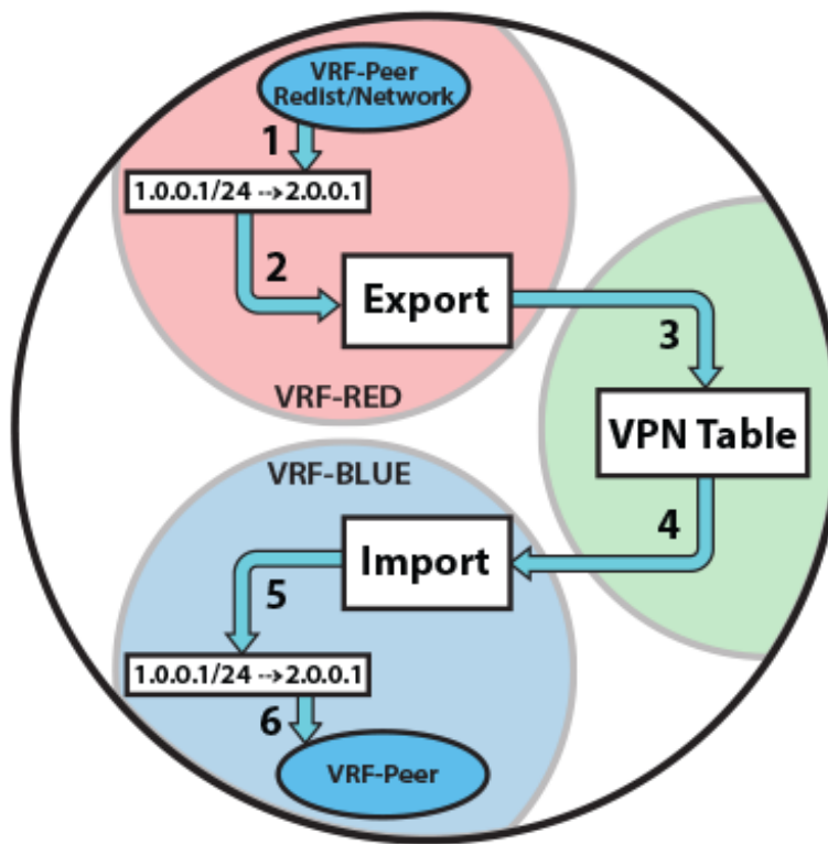
Figure 18-45: Inter-VRF Local Route Leaking using Local VPN Table
