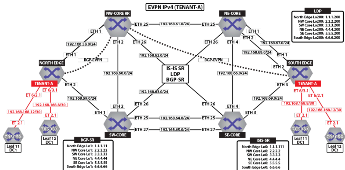
Figure 18-30: Tenant-A DCI
