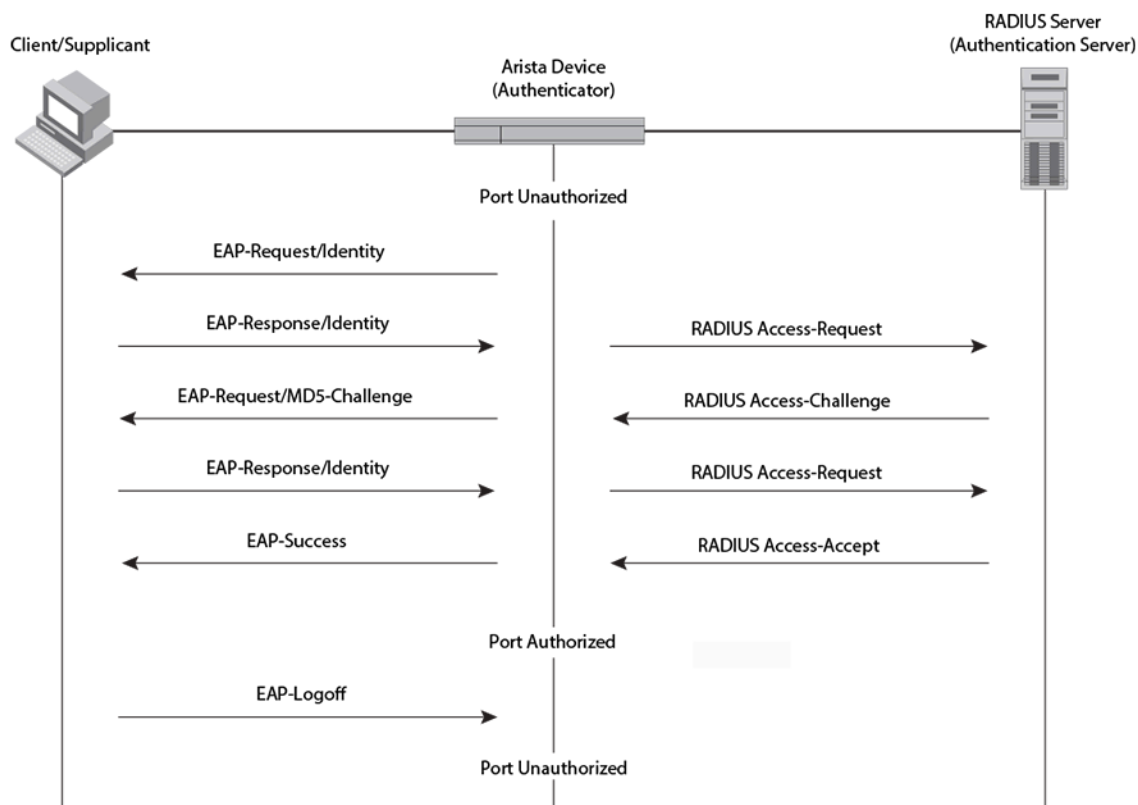
Figure 9-6: Message Exchange During Authentication
