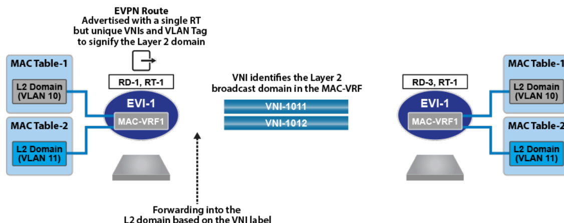
Figure 18-8: VLAN Aware Bundle Service
