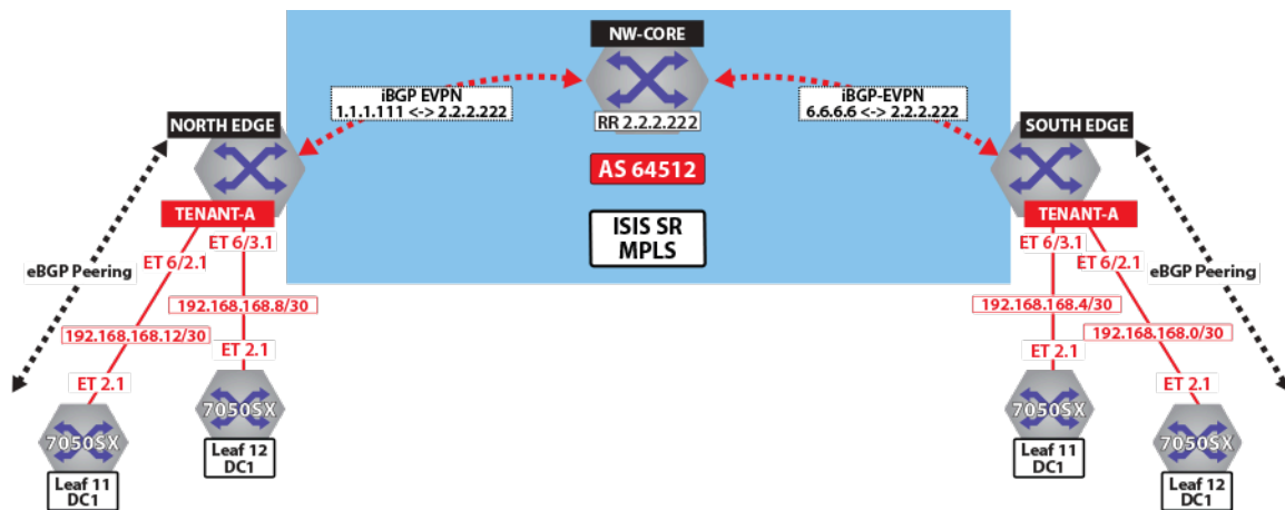
Figure 18-54: Control Plane Tenant-A Over ISIS-SR
