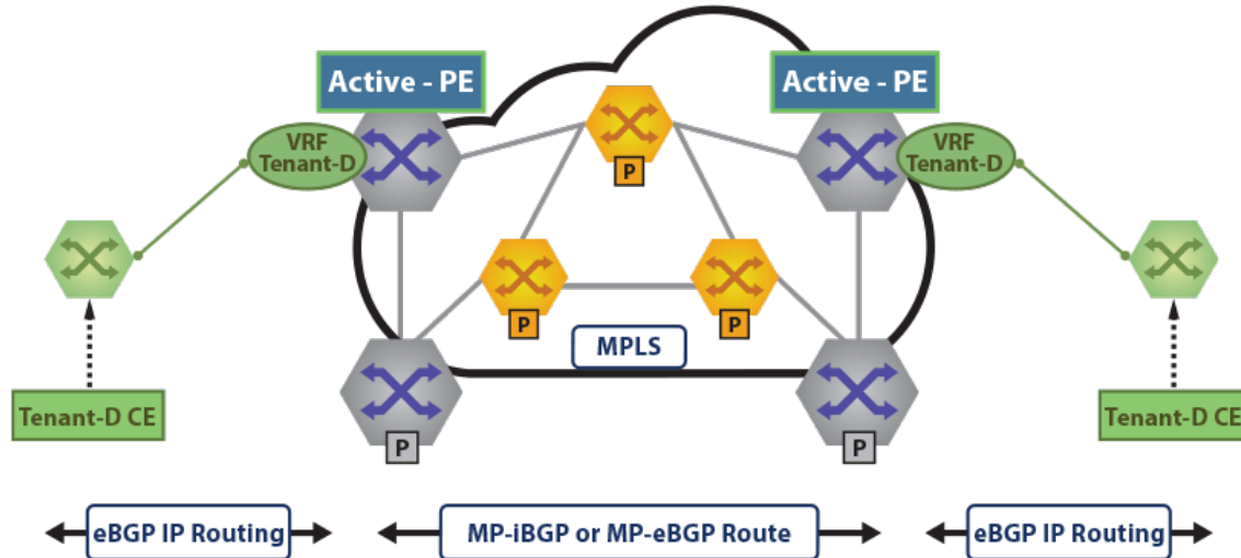
Figure 18-32: IPv4 & IPv6 VPN Sample Topology
