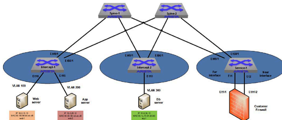
Figure 9-16: Physical Topology of the MSS
