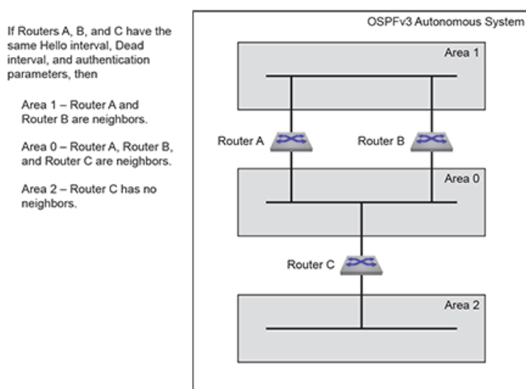
Figure 15-7: OSPFv3 Neighbors
