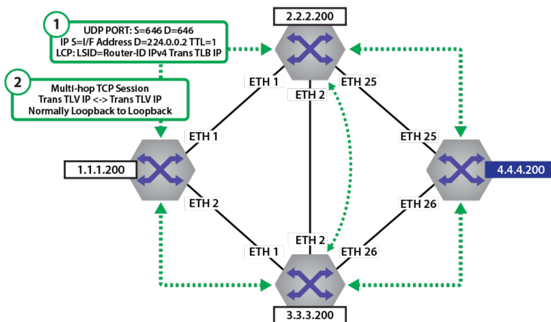
Figure 18-35: LDP Peering Establishment
