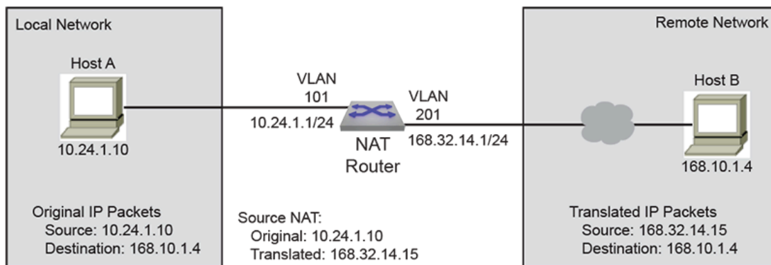
Figure 9-8: Source NAT Example
