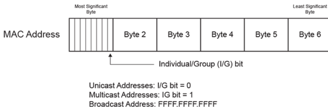
Figure 11-4: MAC Address Format
