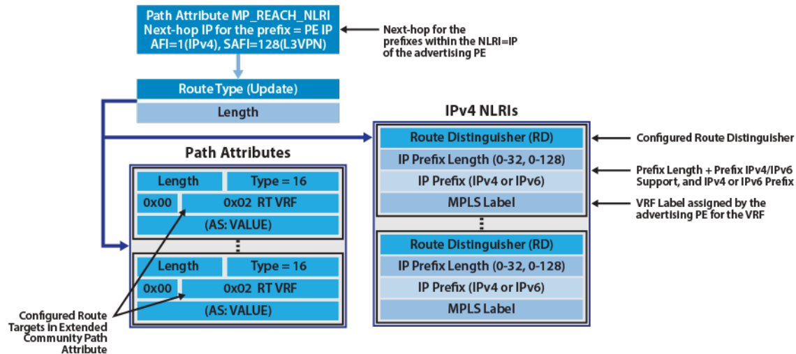
Figure 18-25: IPv4 and IPv6 VPN Update Route Detail
