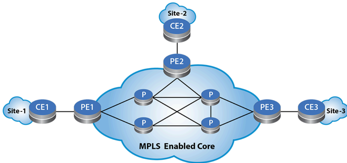
Figure 19-2: MPLS Enabled Core Schematic
