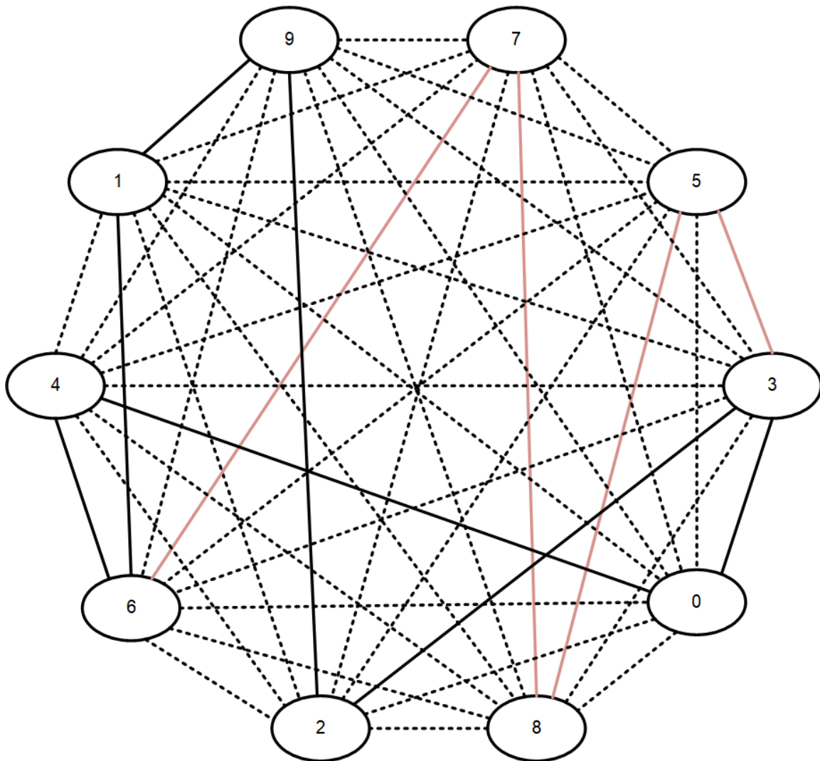
Figure 15-11: Flooding Topology
