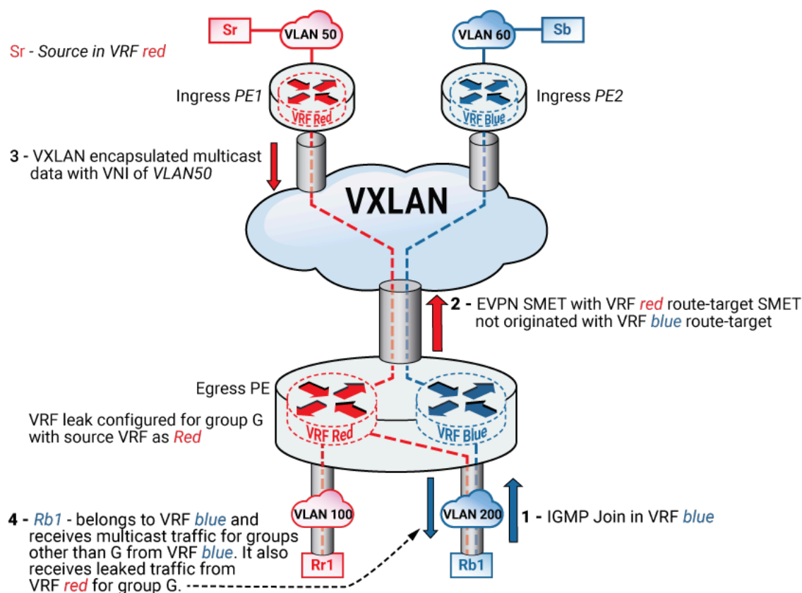
Figure 18-47: Figure 1 - EVPN Multicast Traffic Flow with VRF
