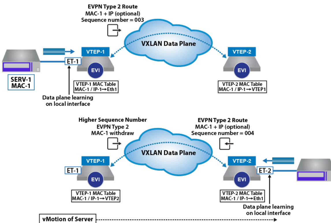
Figure 18-14: EVPN type-2 MAC Mobility Behavior
