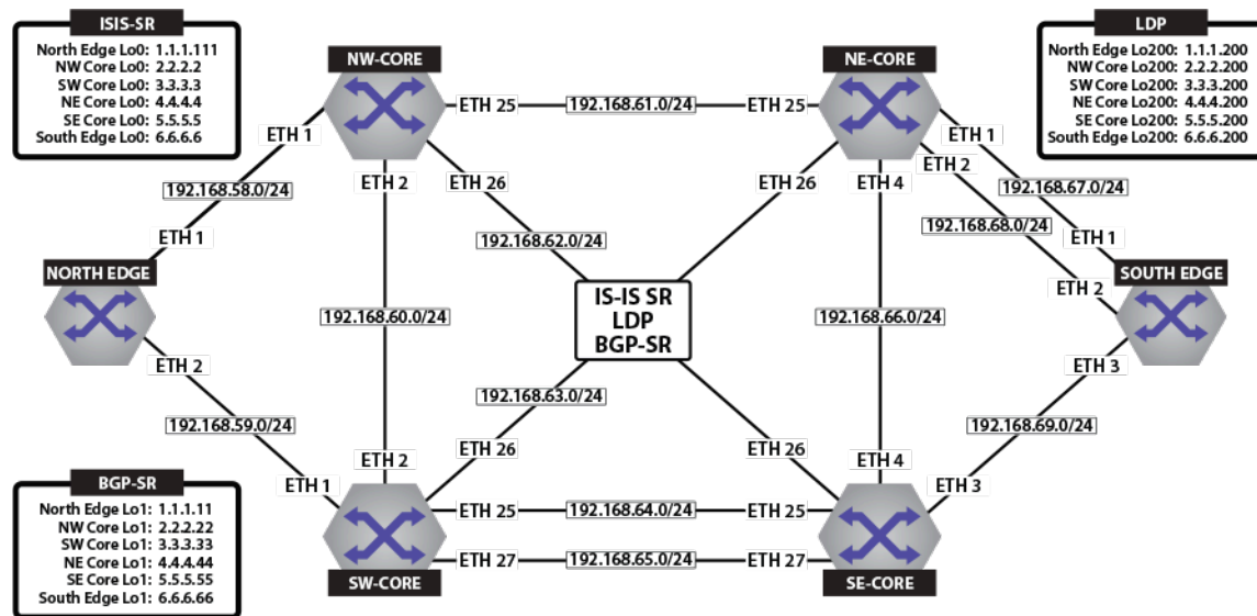
Figure 18-29: Physical Topology For ISIS-SR, LDP and BGP-SR Transport
