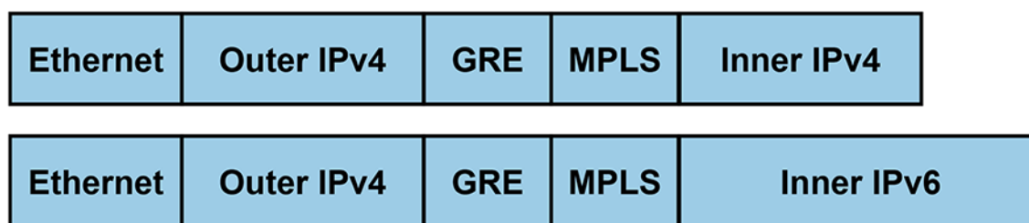
Figure 19-1: Header Format of Packets
