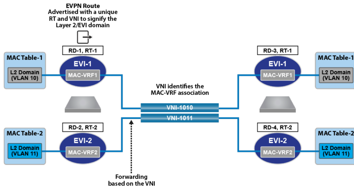
Figure 18-6: VLAN-Based Service Interface
