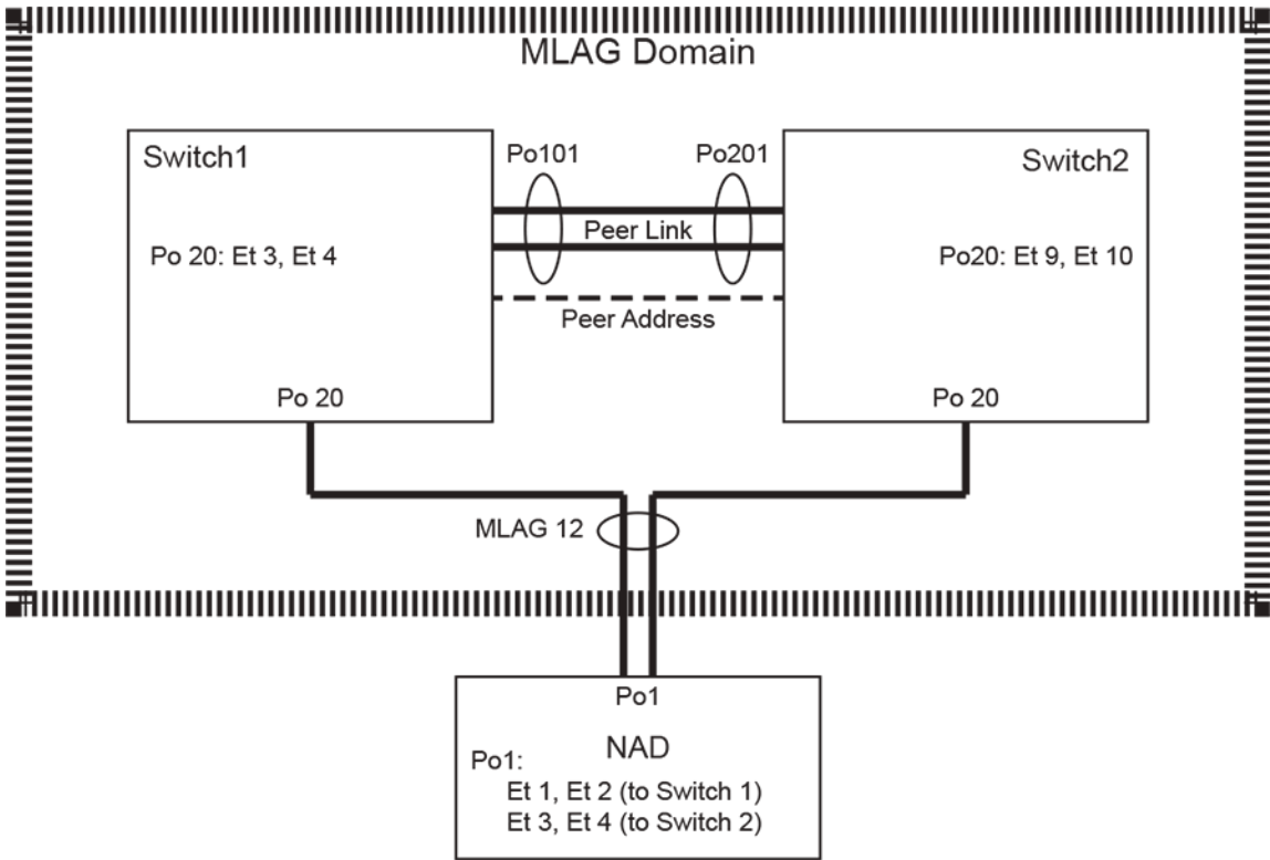
Figure 11-2: MLAG Interface Configuration
