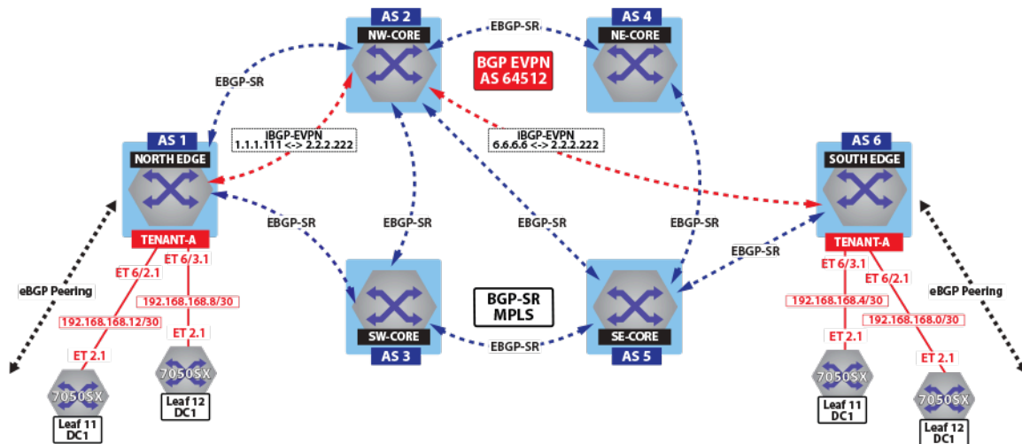
Figure 18-60: Control Plane Tenant-A Over BGP-SR
