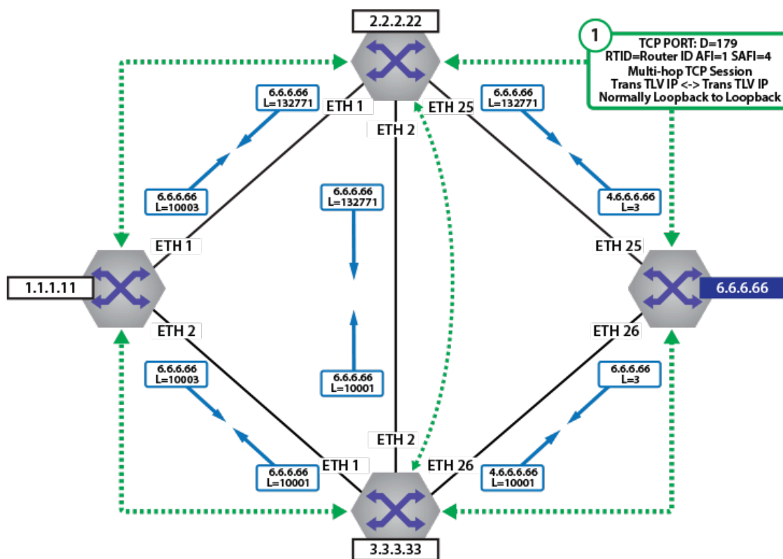
Figure 18-37: BGP-LU Label Distribution
