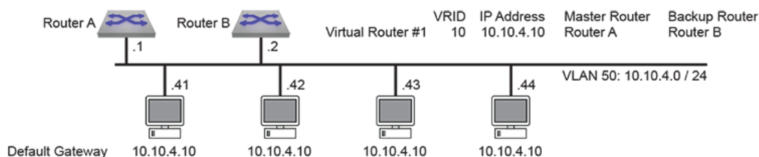
Figure 13-3: VRRP Example 1 Network Diagram
