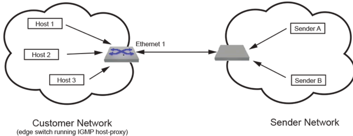
Figure 16-2: IP IGMP Host Proxy Implementation
