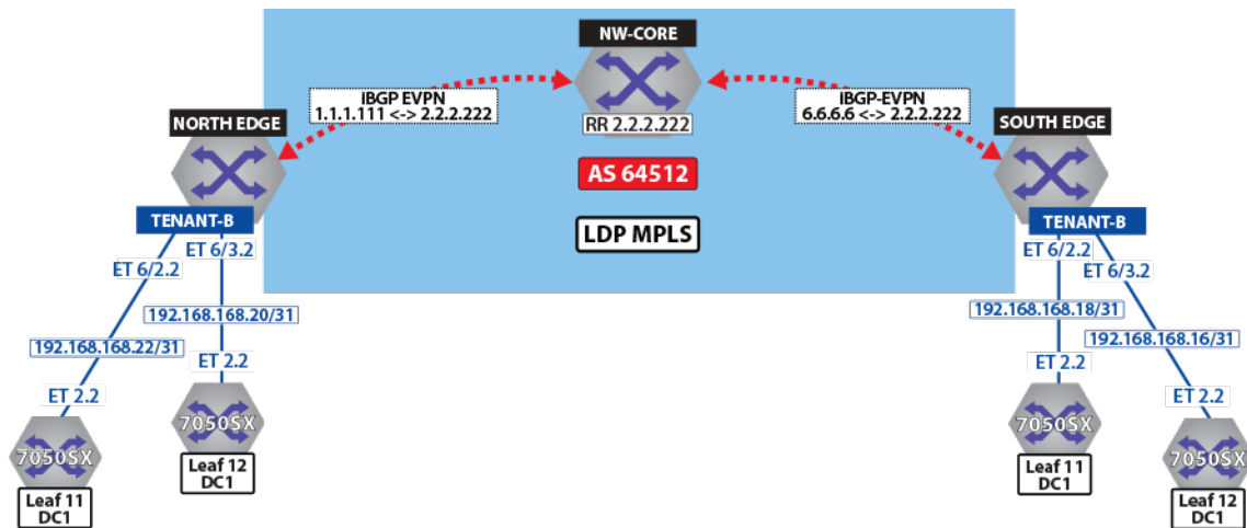
Figure 18-58: Control Plane Tenant-B over LDP
