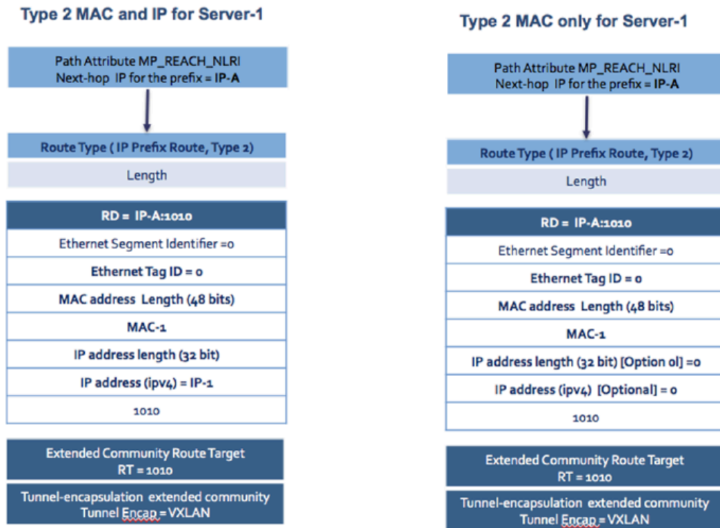
Figure 18-18: EVPN Comparison of MAC & MAC+IP Type 2 Route in Asymmetric IRB
