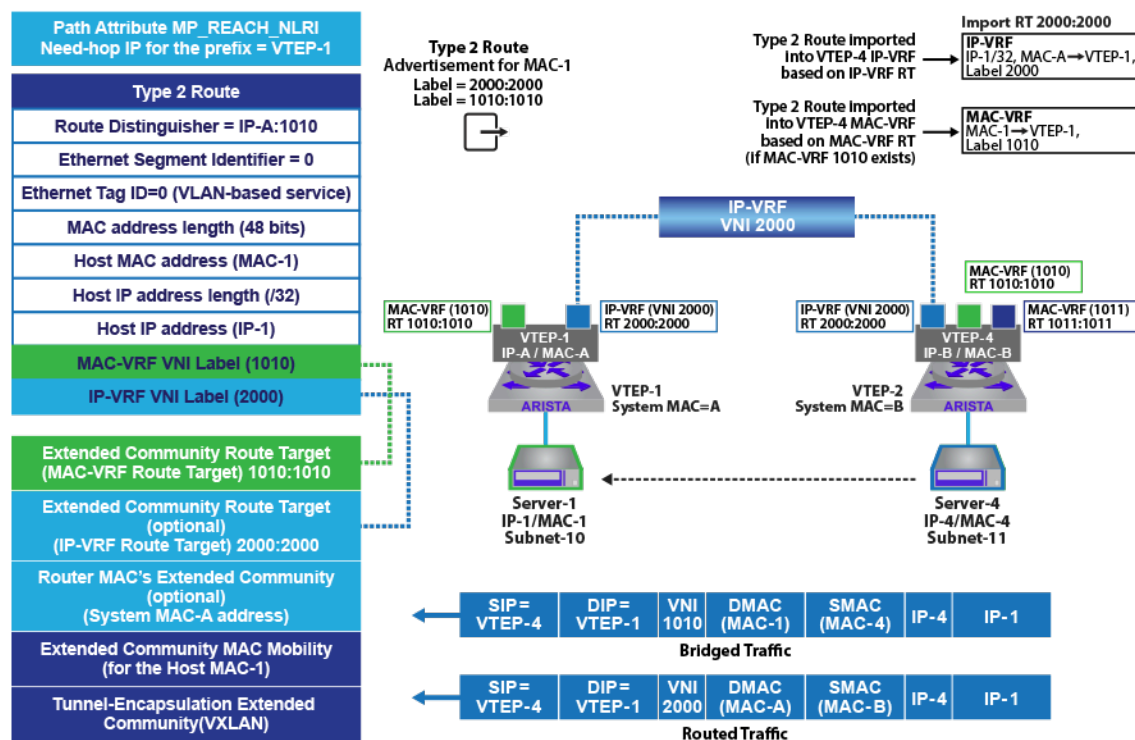
Figure 18-21: EVPN Type 2 Route in Symmetric IRB - MAC-VRF on Both VTEPs
