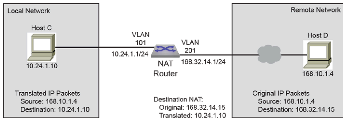
Figure 9-9: Destination NAT Example
