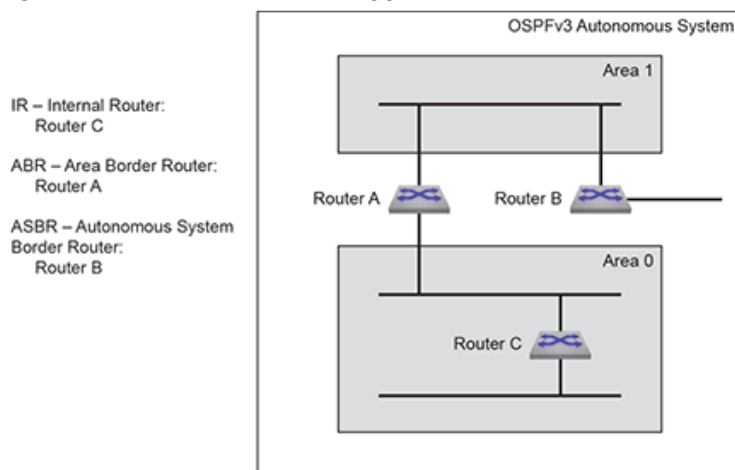
Figure 15-6: OSPFv3 Router Types
