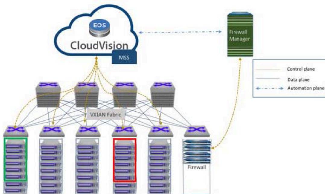
Figure 9-11: Securing server-server traffic
