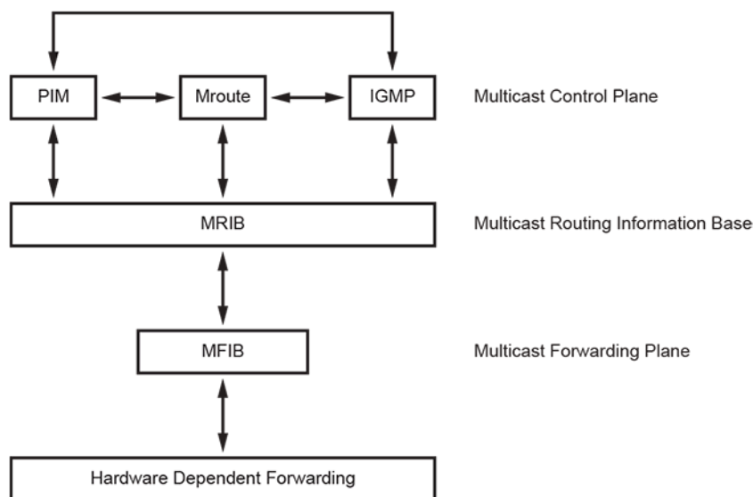
Figure 16-1: Multicast Architecture
