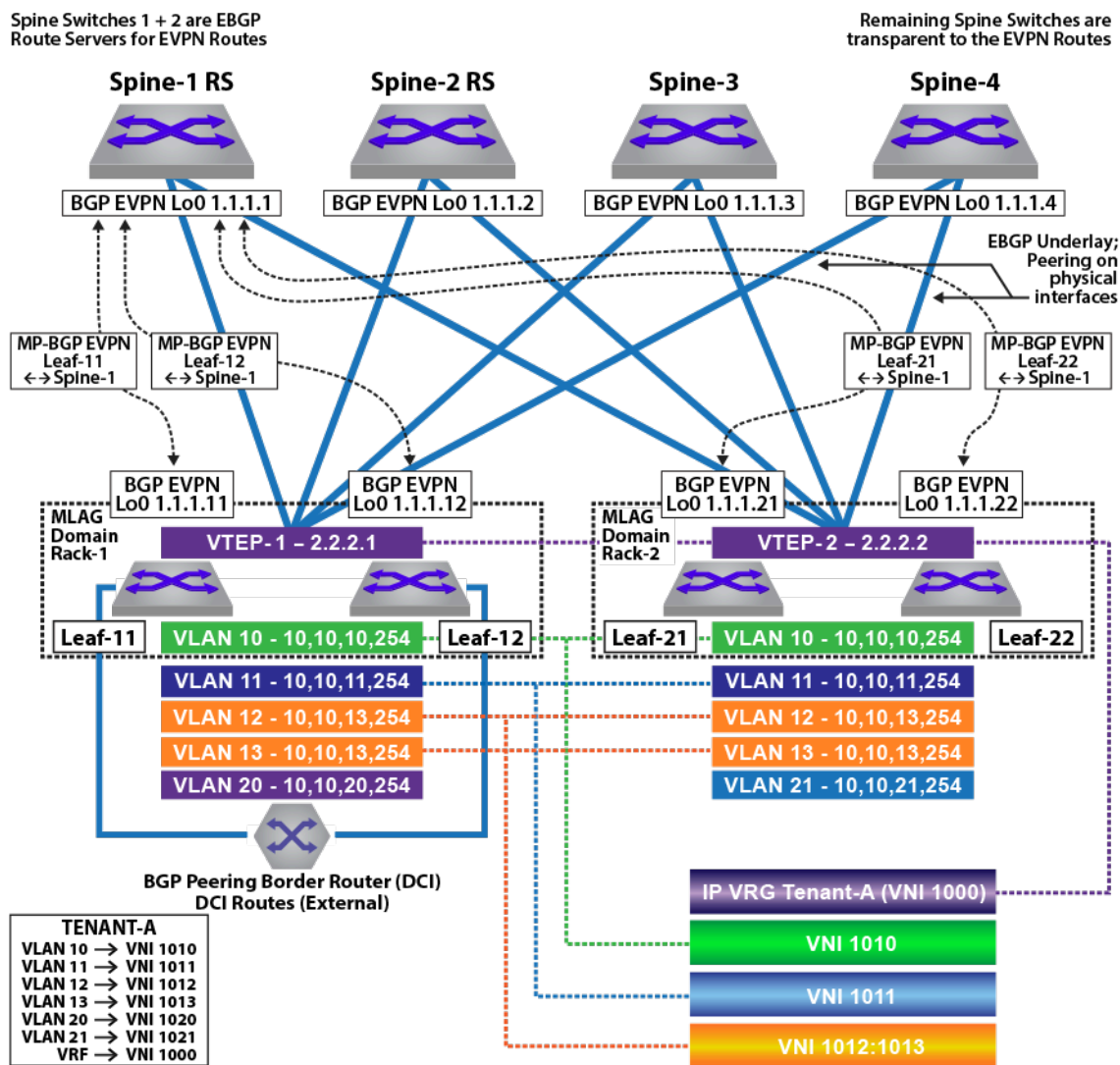
Figure 18-51: Tenant-A: Symmetric IRB
