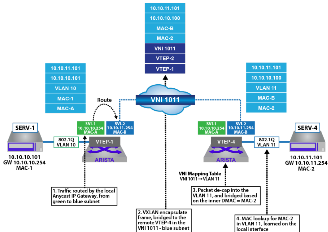
Figure 18-19: EVPN Asymmetric IRB VXLAN Data-plane Forwarding Detail
