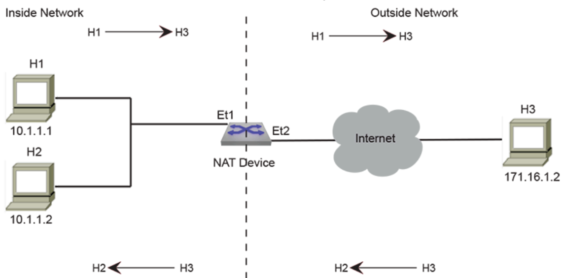
Figure 9-10: Dynamic NAT Scenario
