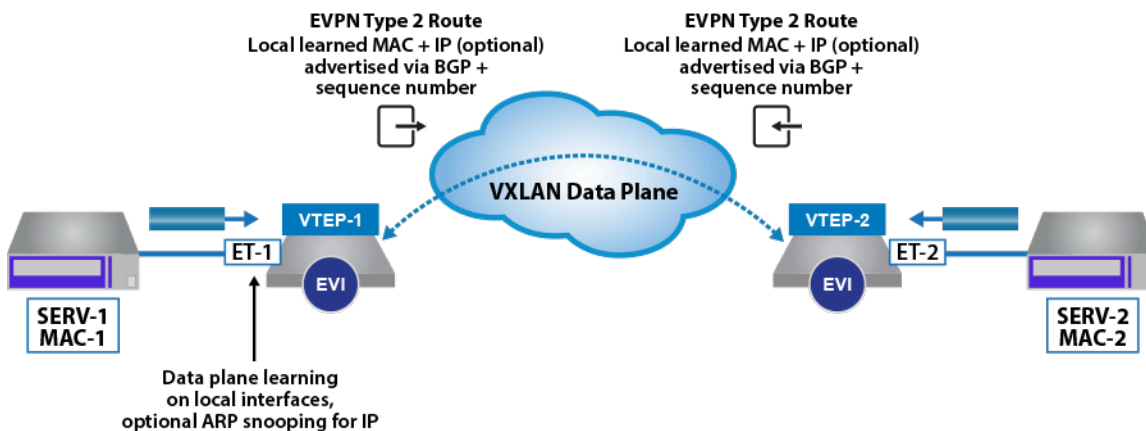
Figure 18-12: EVPN Type 2 Route Announcement
