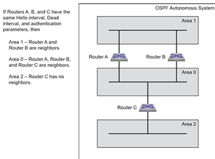
Figure 15-2: OSPFv2 Neighbors
