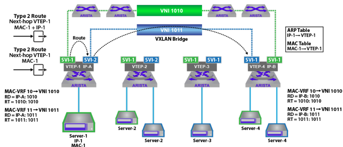
Figure 18-17: EVPN Asymmetric IRB
