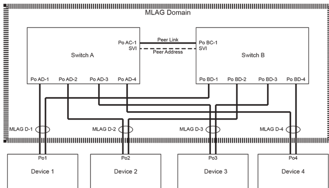
Figure 11-1: MLAG Domain Topology
