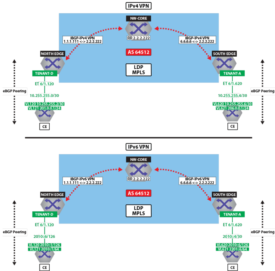
Figure 18-68: IPv4 VPN and IPv6 VPN Over LDP MPLS
