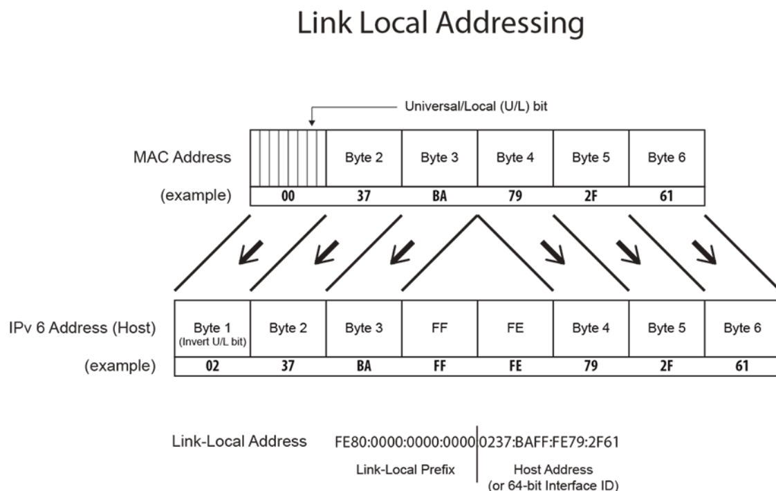
Figure 13-1: Link Local Address Derivation
