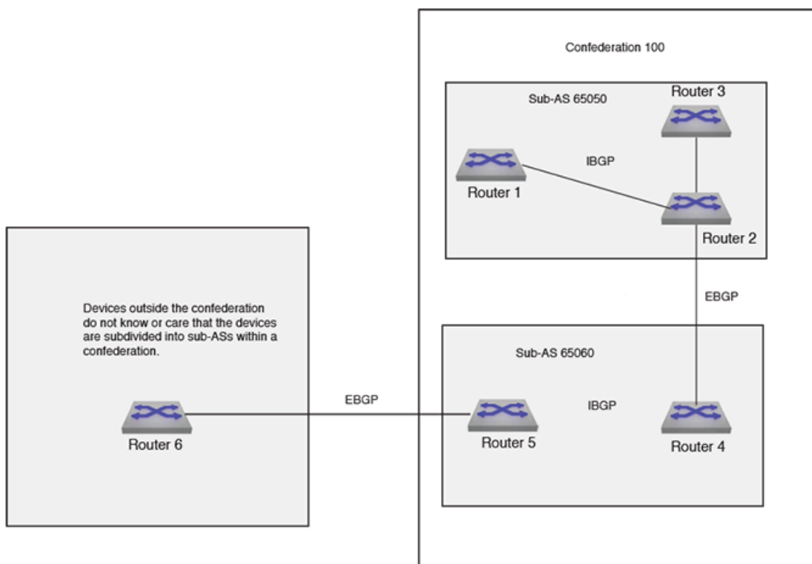
Figure 15-15: BGP Confederation Example
