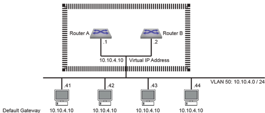
Figure 13-2: VARP Configuration
