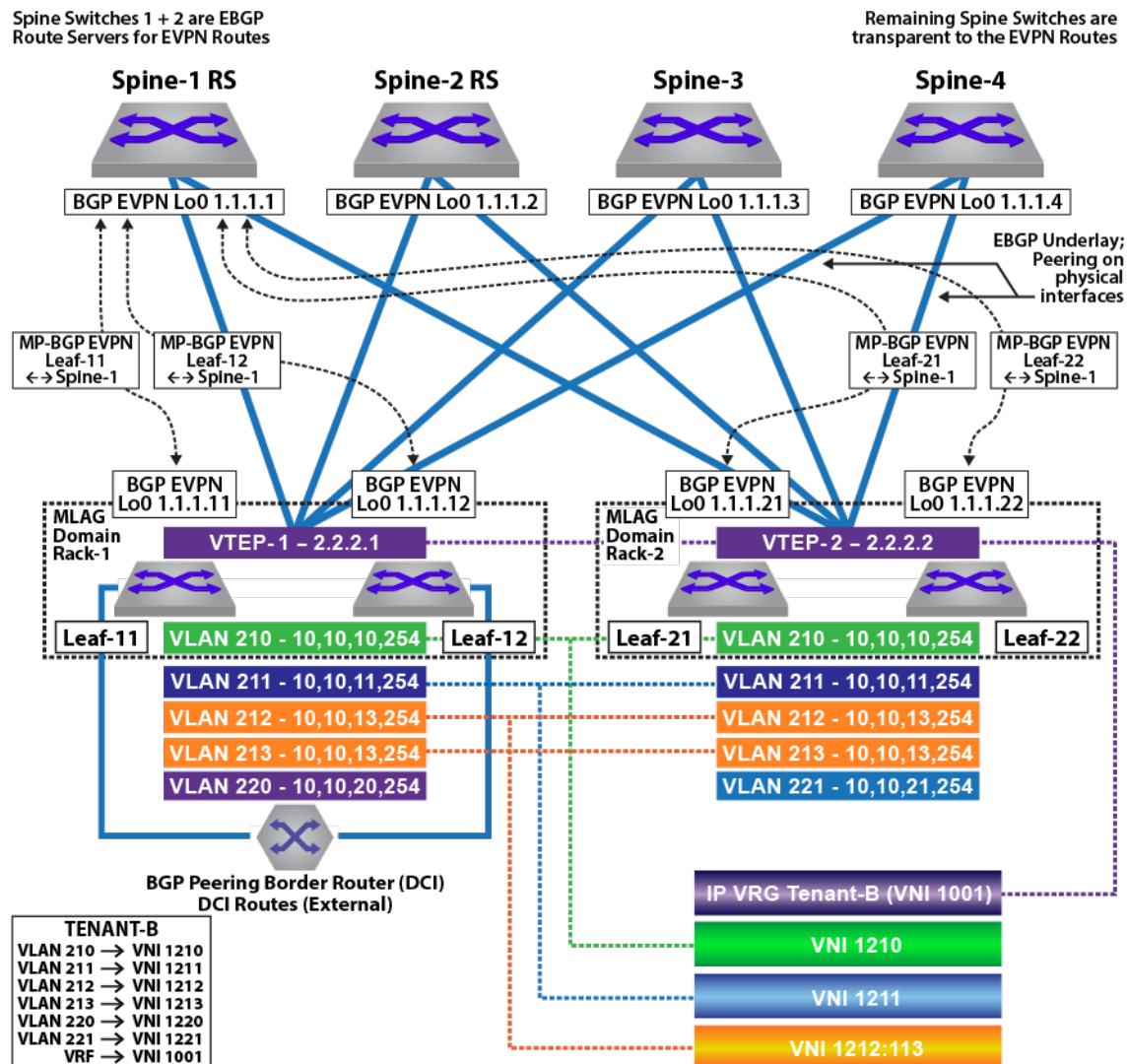
Figure 18-52: Tenant-B: Asymmetric IRB
