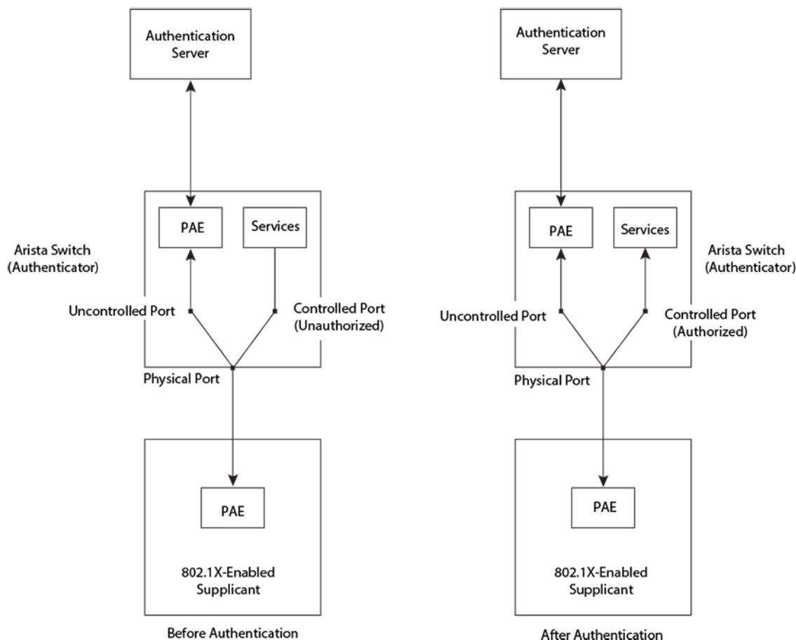
Figure 9-5: Ports Before and After Client Authentication
