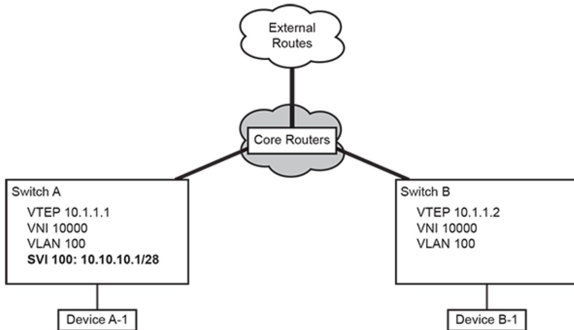
Figure 17-3: Implementing VXLAN Routing
