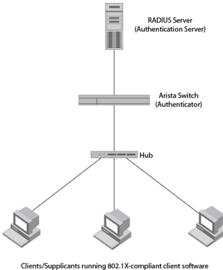
Figure 9-7: Multiple clients connected to a 802.1X-enabled port
