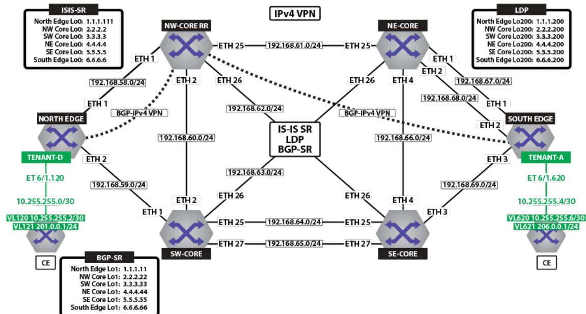
Figure 18-33: Tenant-D IPv4 VPN
