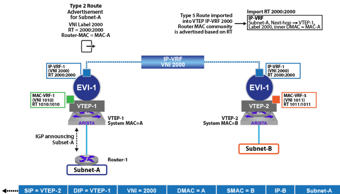
Figure 18-40: EVPN Route Type-5, Interface-less Update
