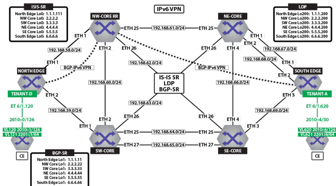
Figure 18-34: Tenant-D IPv6 VPN
