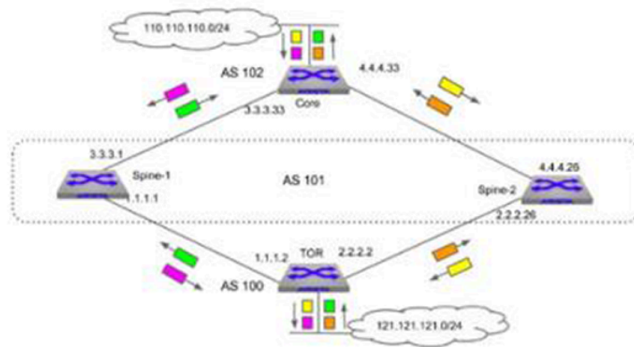
Figure 15-18: Traffic Flow Pattern Between TOR and Core Before Maintenance
