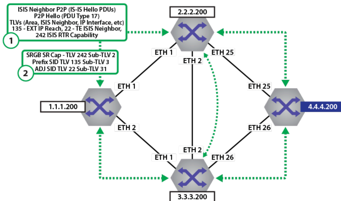
Figure 18-36: ISIS Neighbor Adj and TLVs
