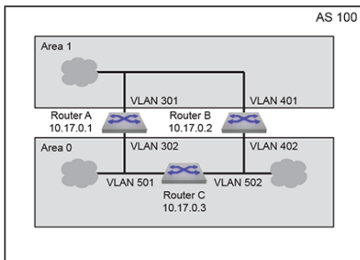
Figure 15-8: OSPFv3 Example 1
