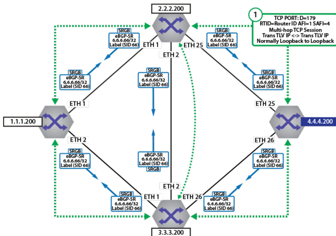
Figure 18-38: BGP-SR Index and SRGB Distribution
