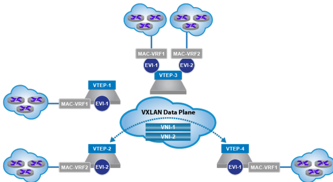
Figure 18-3: EVPN Terminology for a VXLAN Data Plane
