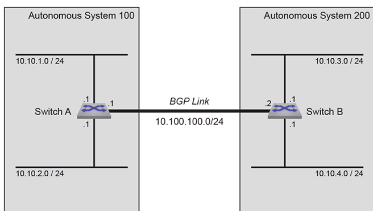
Figure 15-17: BGP Example 2
