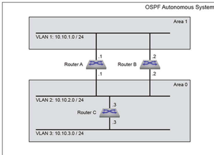
Figure 46: OSPFv2 Example 1
