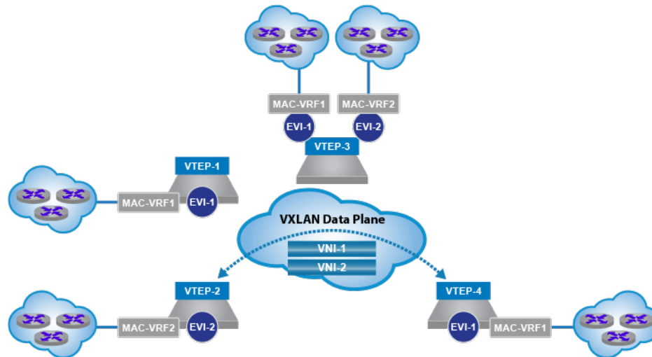
Figure 72: EVPN Terminology for a VXLAN Data Plane
