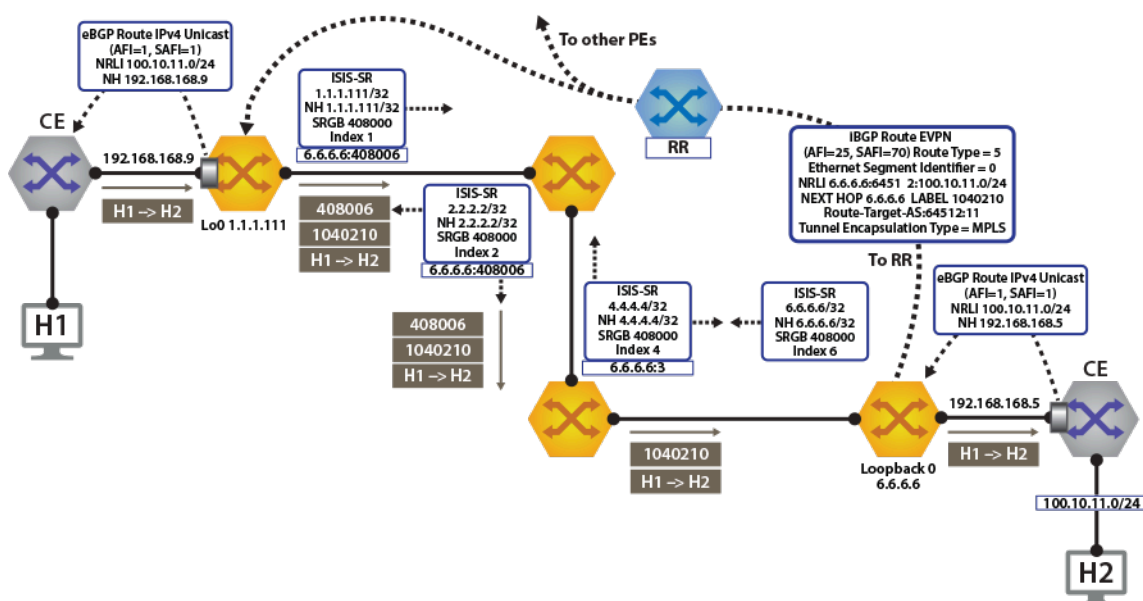
Figure 121: Control Plane & Forwarding Tenant-A Over ISIS-SR
