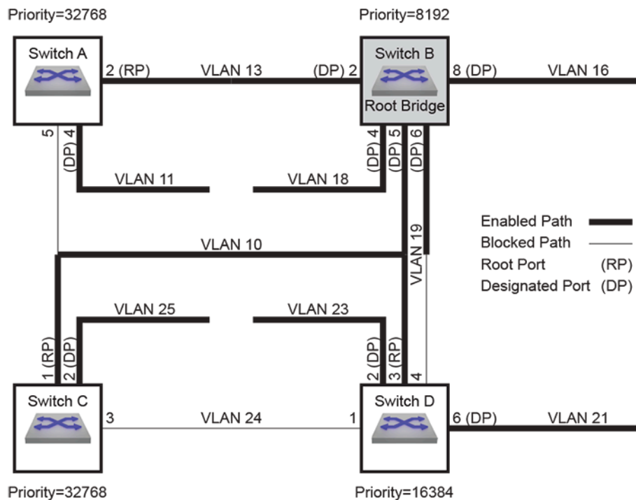
Figure 26: Spanning Tree Network Example
