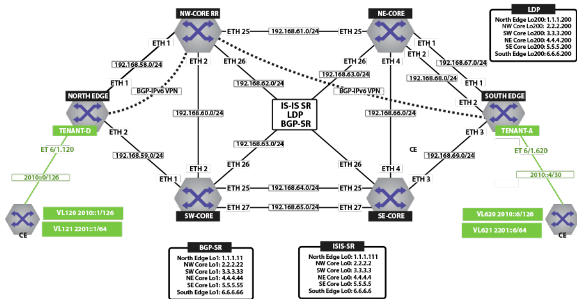
Figure 129: IPv6 VPN Physical Topology
