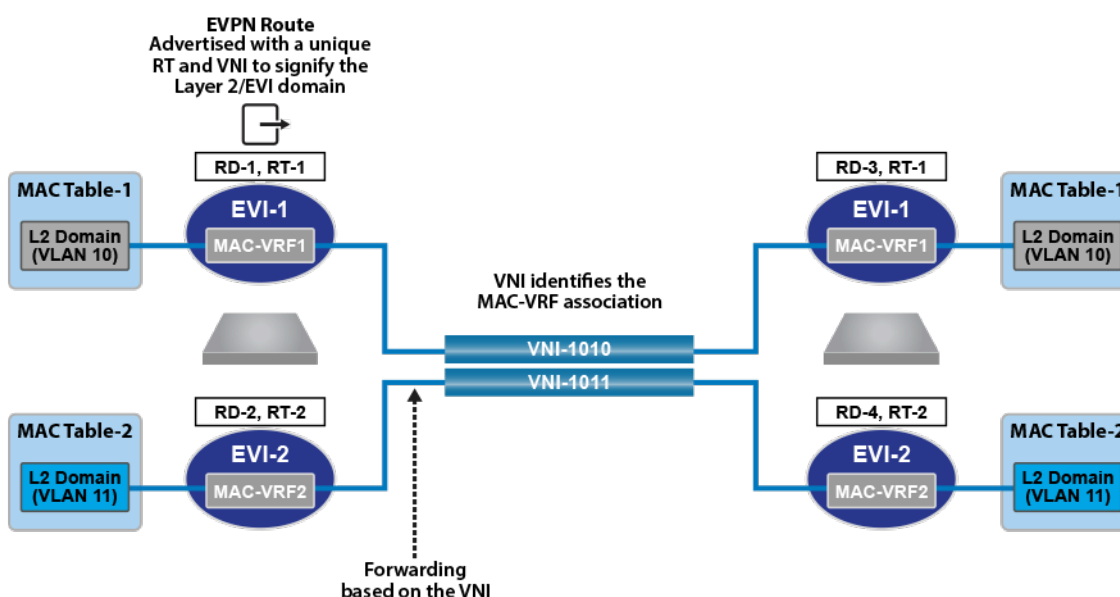
Figure 75: VLAN Based Service Interface
