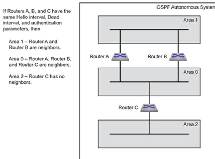
Figure 45: OSPFv2 Neighbors
