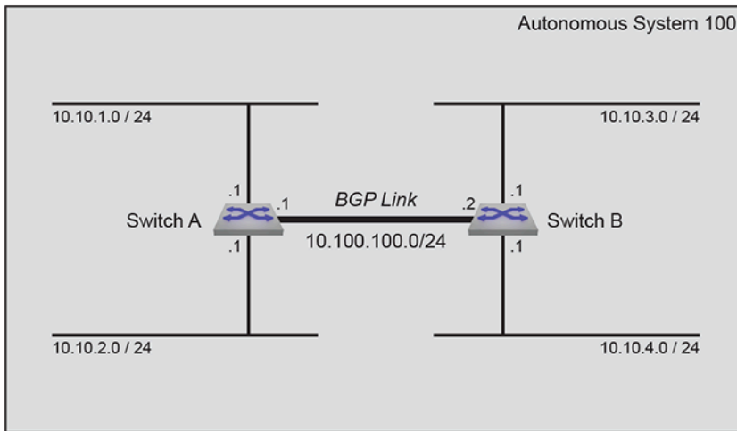
Figure 58: BGP Example 1
