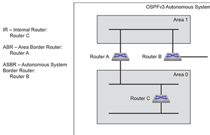
Figure 49: OSPFv3 Router Types
