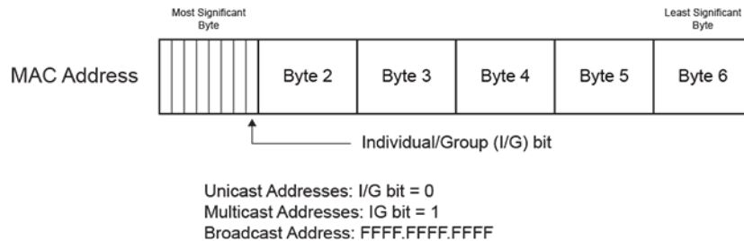
Figure 24: MAC Address Format
