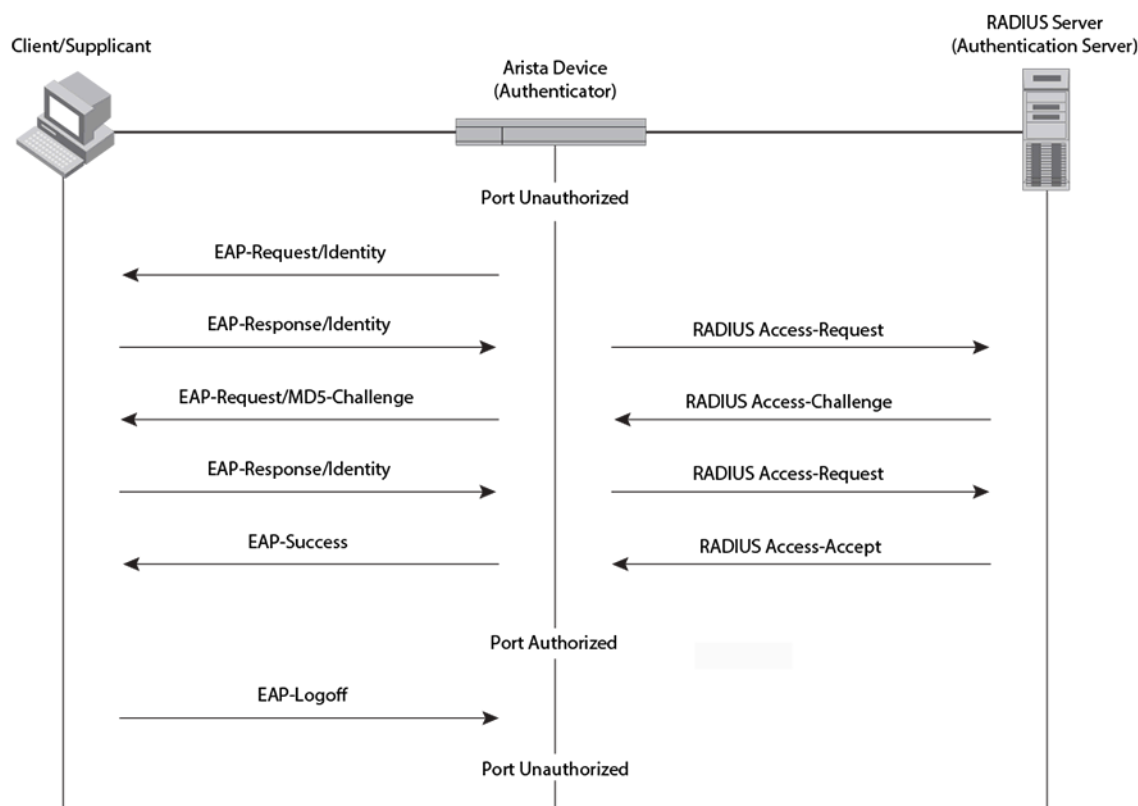
Figure 6: Message Exchange During Authentication
