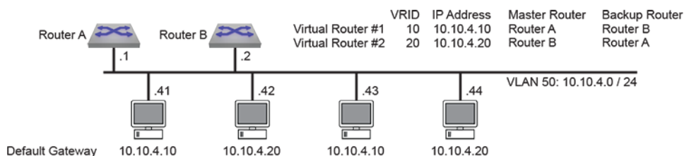
Figure 32: VRRP Example 2 Network Diagram
