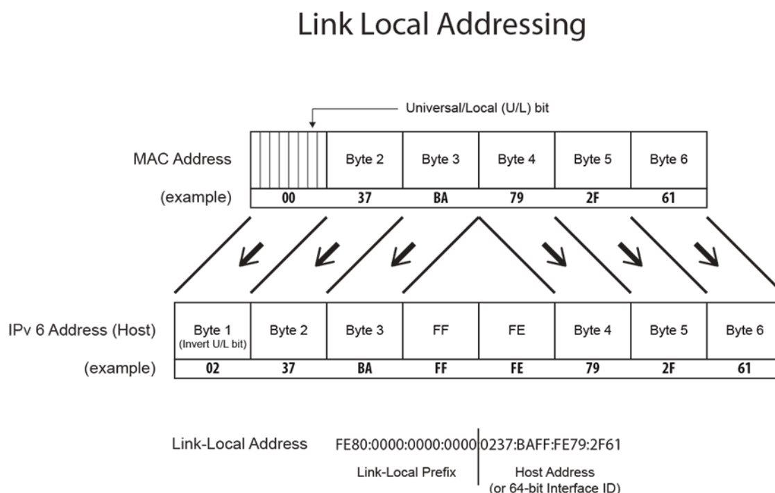
Figure 29: Link Local Address Derivation
