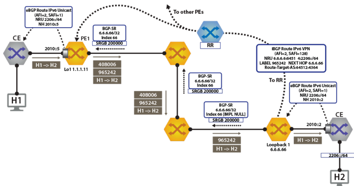
Figure 138: IPv6 VPN Forwarding Over BGP-SR MPLS
