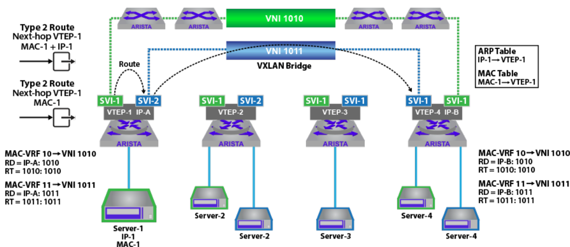
Figure 89: EVPN Symmetric IRB
