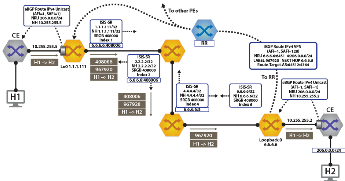
Figure 131: IPv4 VPN Forwarding Over ISIS-SR MPLS
