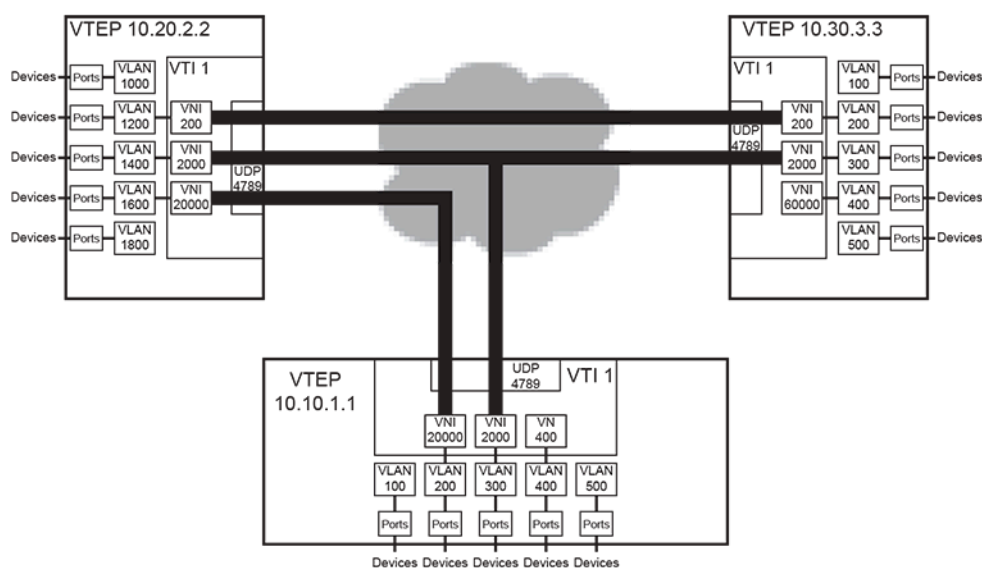
Figure 67: VXLAN Implementation
