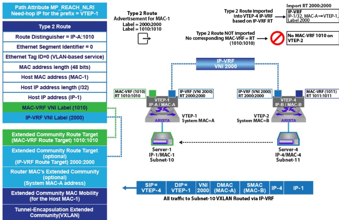
Figure 91: EVPN Type 2 Route in Symmetric IRB - MAC-VRF Only Exists on Sending VTEP
