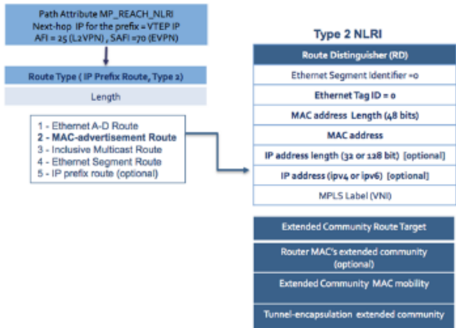
Figure 82: EVPN Type 2 MAC and IP Route Format
