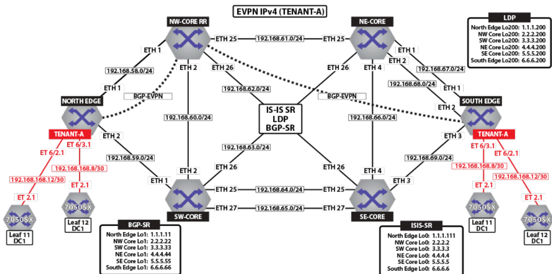
Figure 99: Tenant-A DCI
