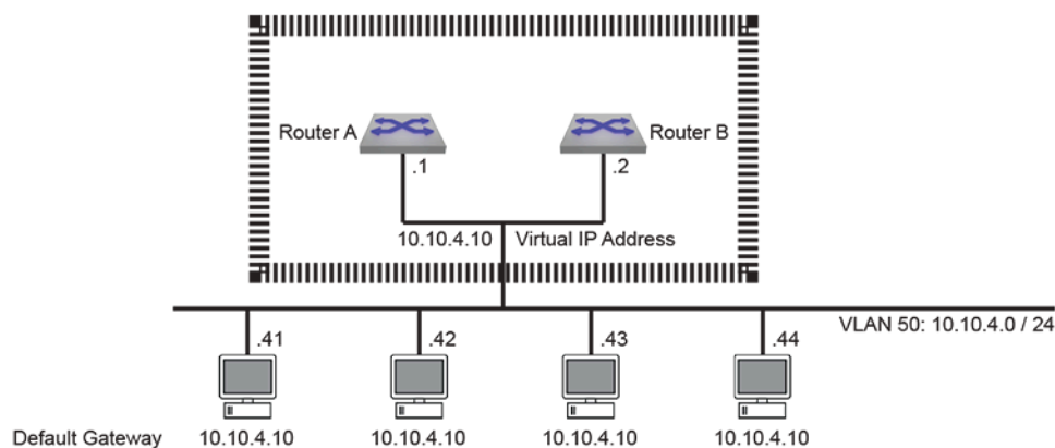
Figure 30: VARP Configuration
