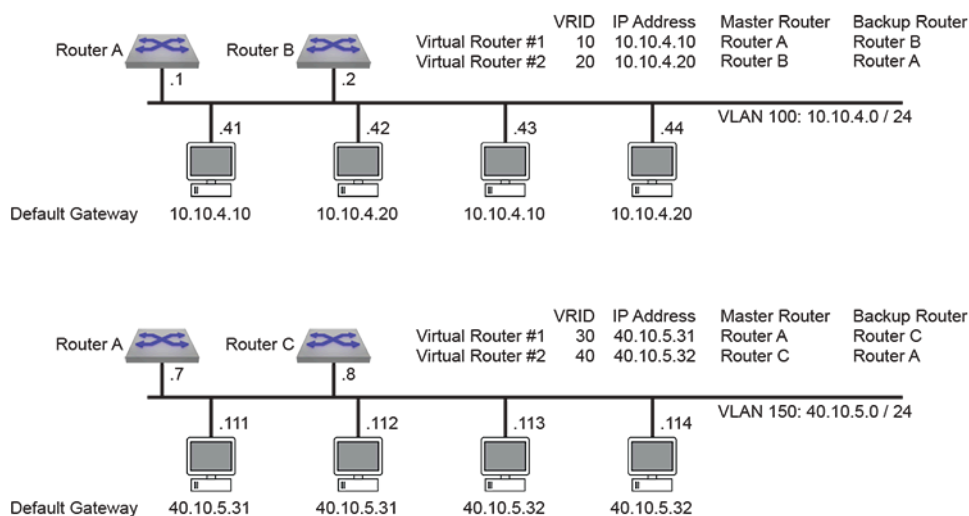
Figure 33: VRRP Example 3 Network Diagram
