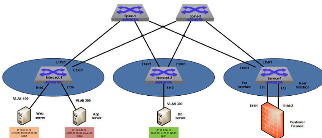
Figure 16: Physical topology of the MSS
