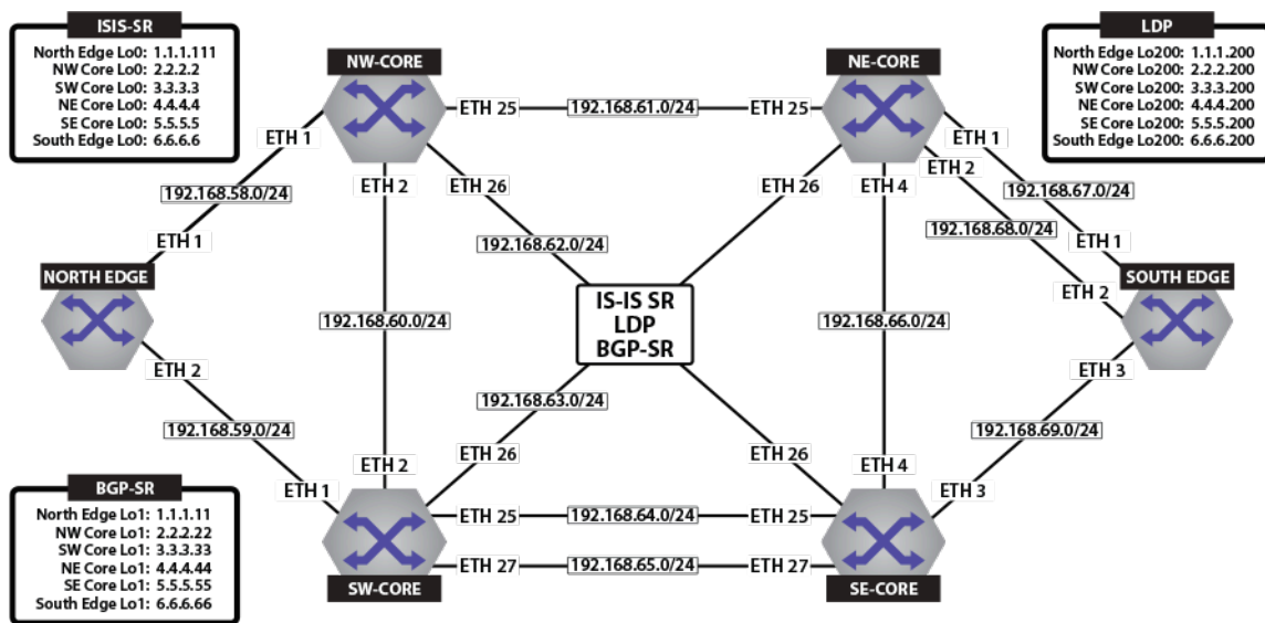
Figure 98: Physical Topology For ISIS-SR, LDP and BGP-SR Transport
