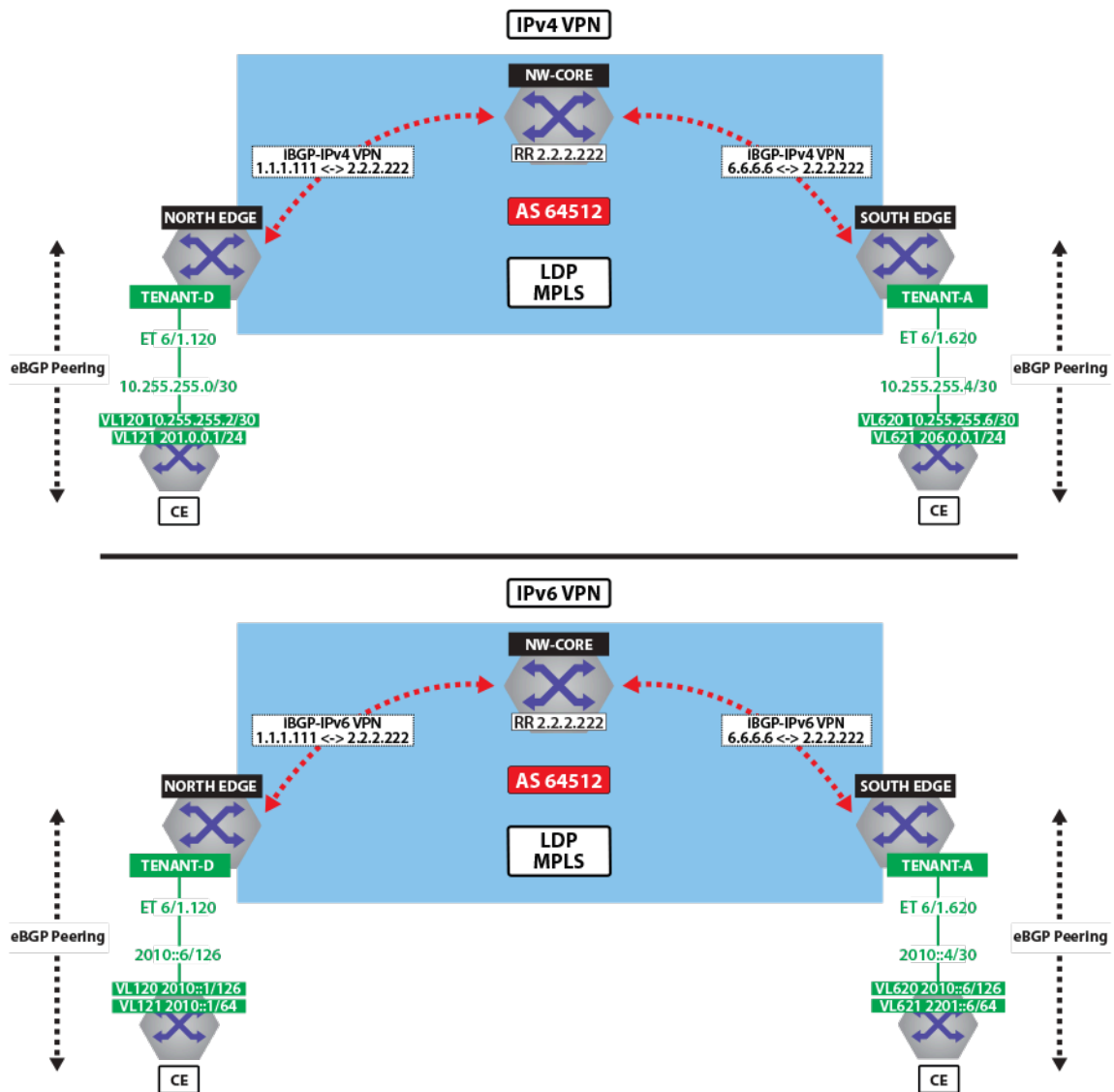
Figure 133: IPv4 VPN and IPv6 VPN Over LDP MPLS
