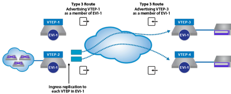
Figure 84: EVPN type-3 IMET Route Behavior for Ingress Replication
