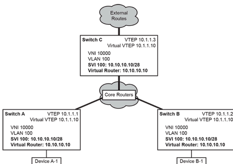
Figure 69: Direct VXLAN Routing
