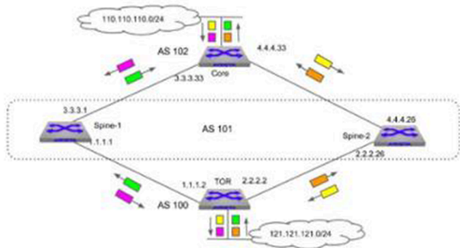
Figure 60: Traffic flow pattern between TOR and Core Before Maintenance
