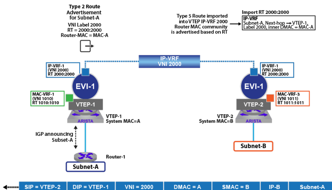
Figure 109: EVPN Route Type-5, Interface-less Update
