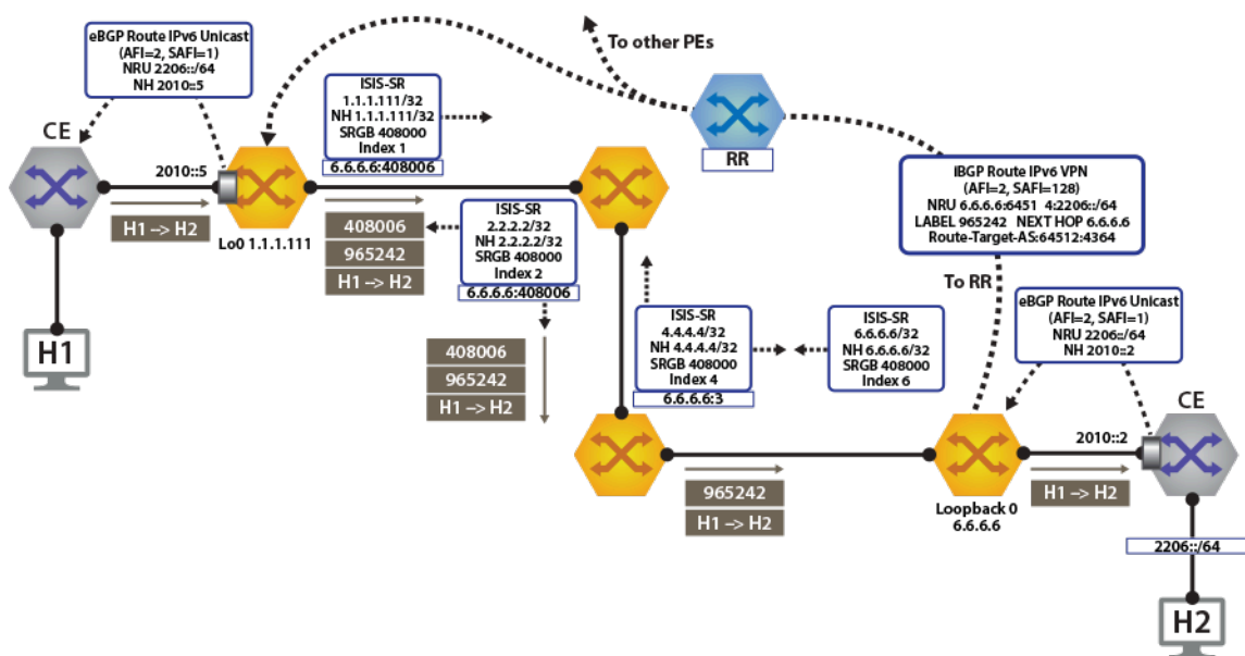
Figure 132: IPv6 VPN Forwarding Over ISIS-SR MPLS
