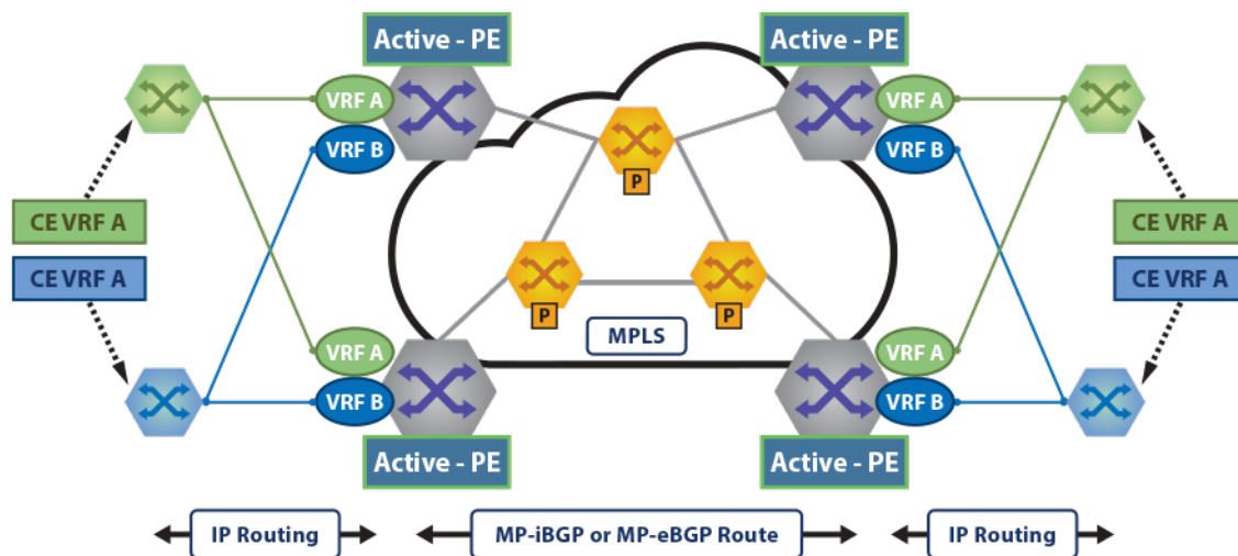
Figure 97: MPLS Layer 3 VPN Topology
