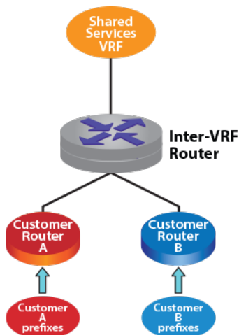
Figure 113: Accessing Shared Resources Across VPNs
