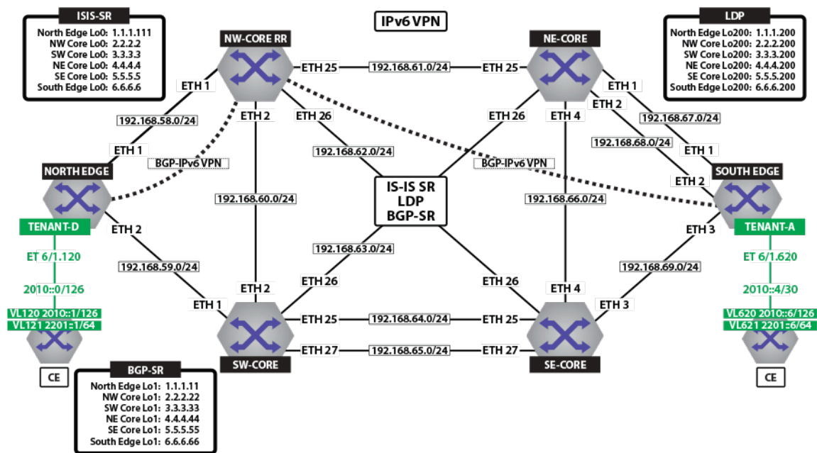
Figure 103: Tenant-D IPv6 VPN
