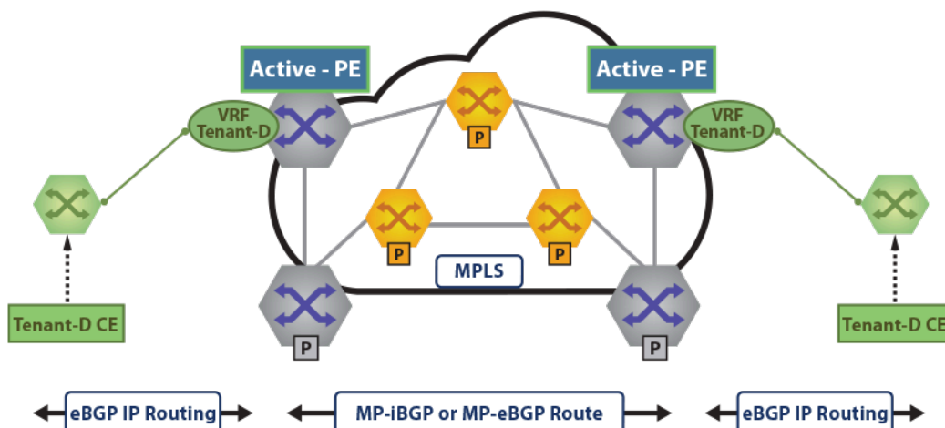
Figure 101: IPv4 & IPv6 VPN Sample Topology
