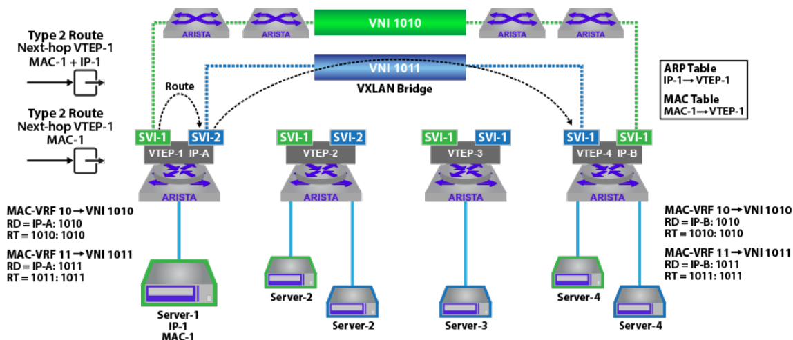
Figure 86: EVPN Asymmetric IRB
