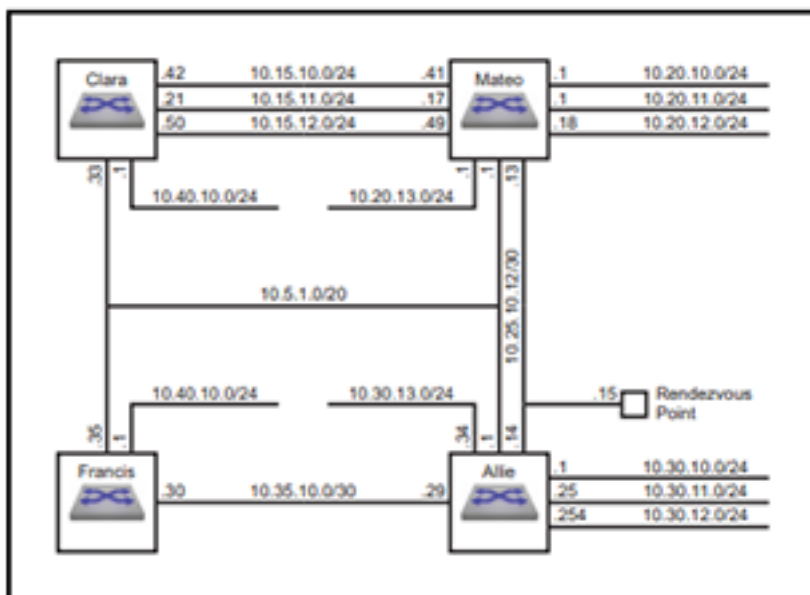
Figure 65: Multicast Example
