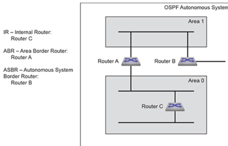
Figure 44: OSPFv2 Router Types
