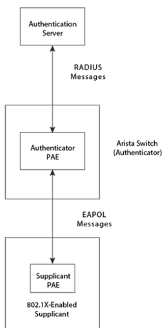
Figure 4: Authenticator PAE and Supplicant PAE
