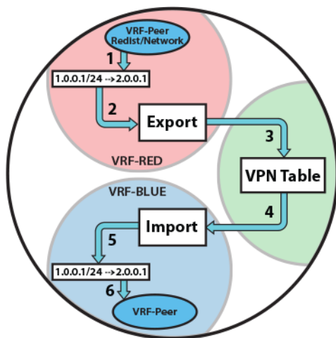
Figure 112: Inter-VRF Local Route Leaking using Local VPN Table
