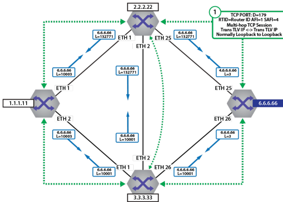
Figure 106: BGP-LU Label Distribution
