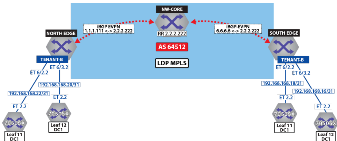
Figure 123: Control Plane Tenant-B over LDP
