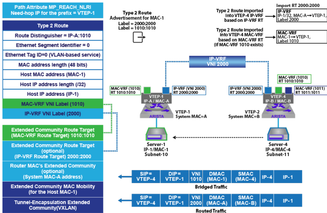
Figure 90: EVPN Type 2 Route in Symmetric IRB - MAC-VRF on Both VTEPs
