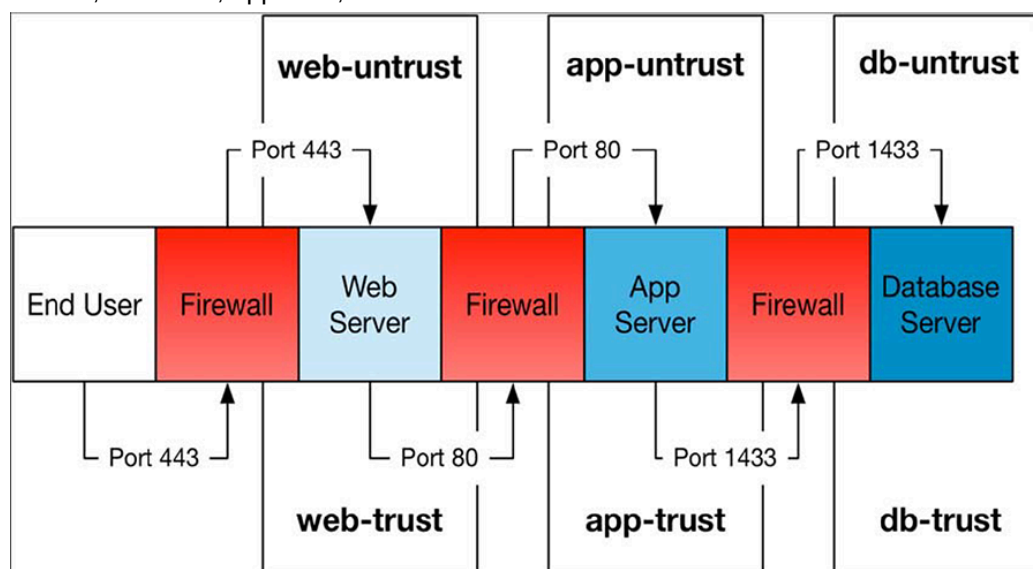
Figure 15: Traffic flow in an MSS deployment
