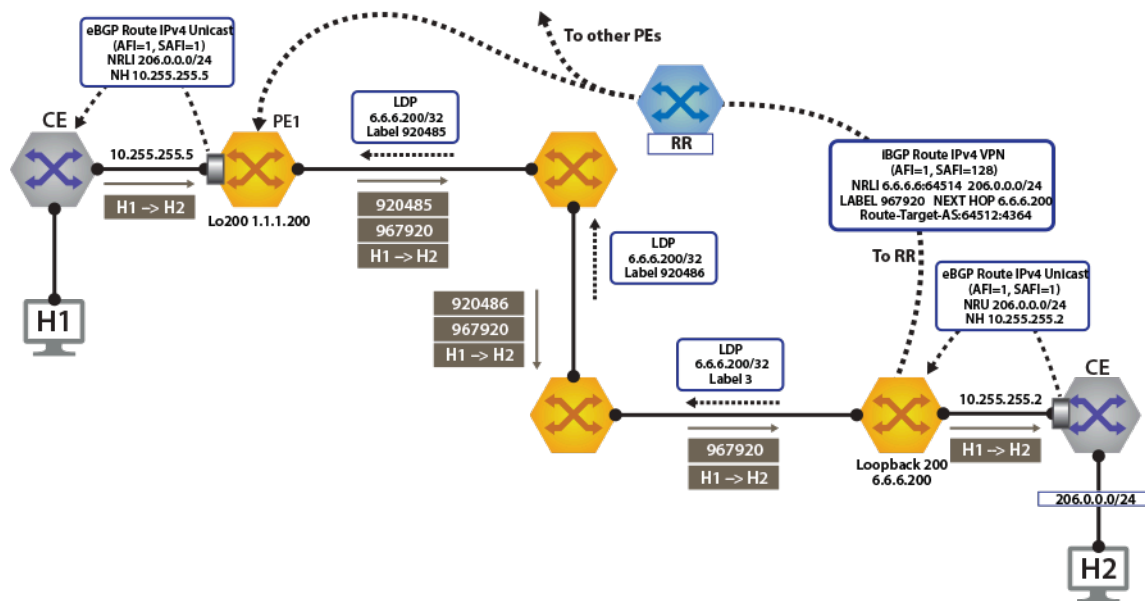
Figure 134: IPv4 VPN Forwarding Over LDP MPLS
