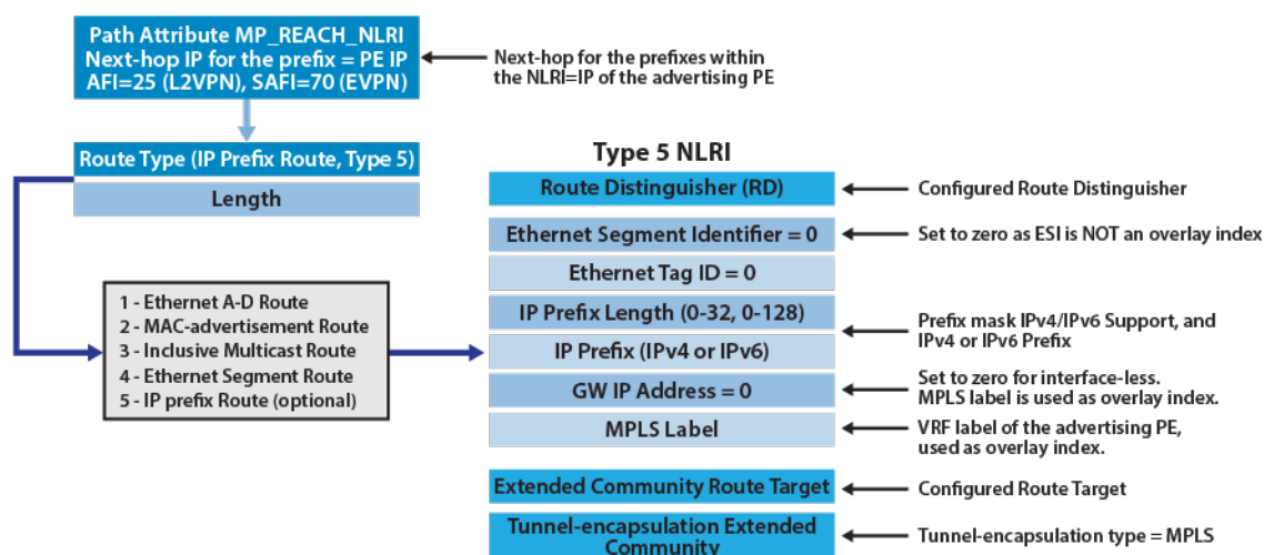
Figure 79: EVPN Route Type-5, for Advertisement of IP-Prefixes over MPLS
