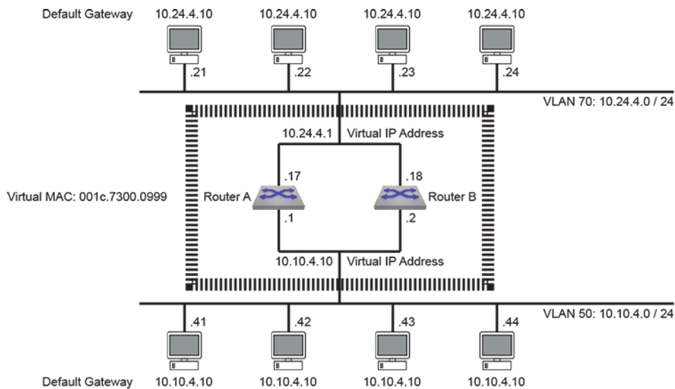
Figure 34: VARP Example Network Diagram
