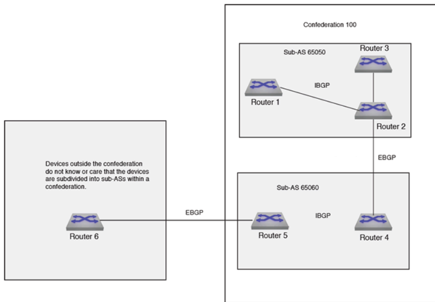
Figure 57: BGP Confederation Example
