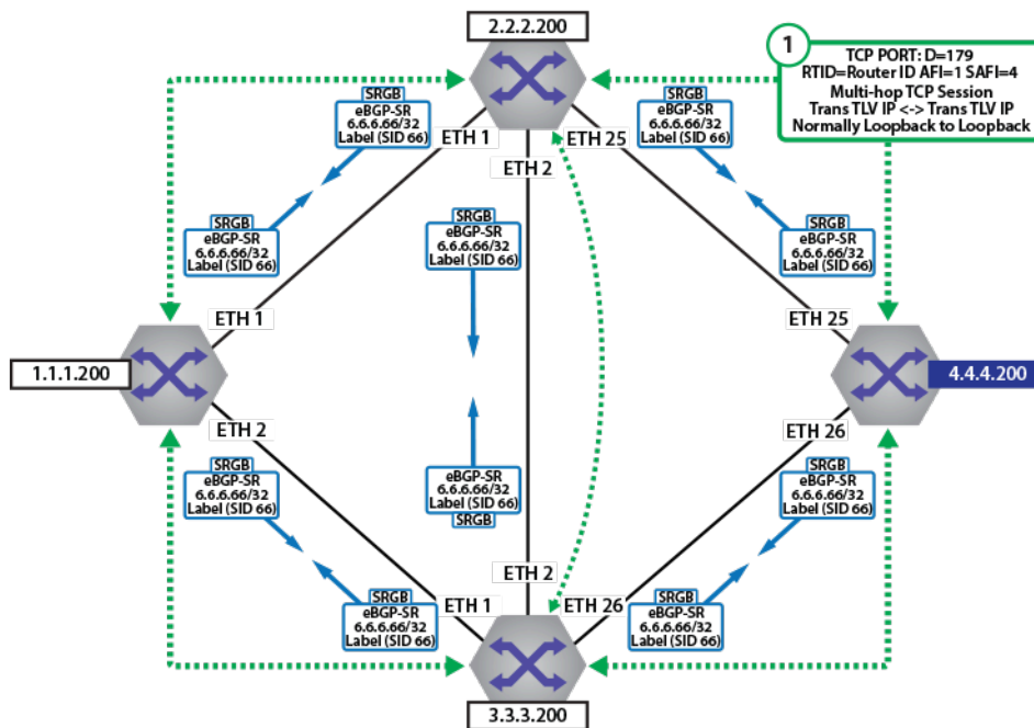
Figure 107: BGP-SR Index and SRGB Distribution
