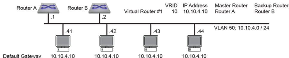
Figure 31: VRRP Example 1 Network Diagram
