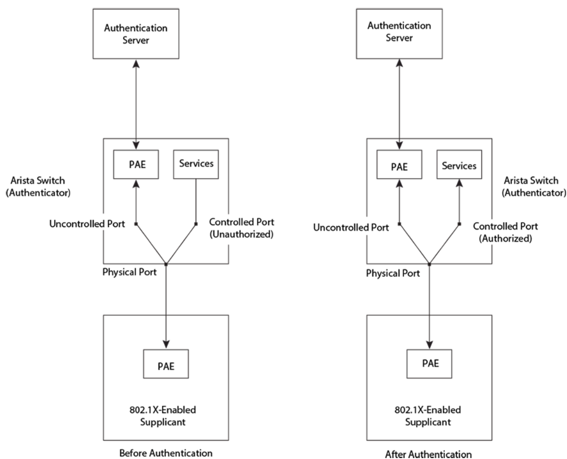
Figure 5: Ports Before and After Client Authentication
