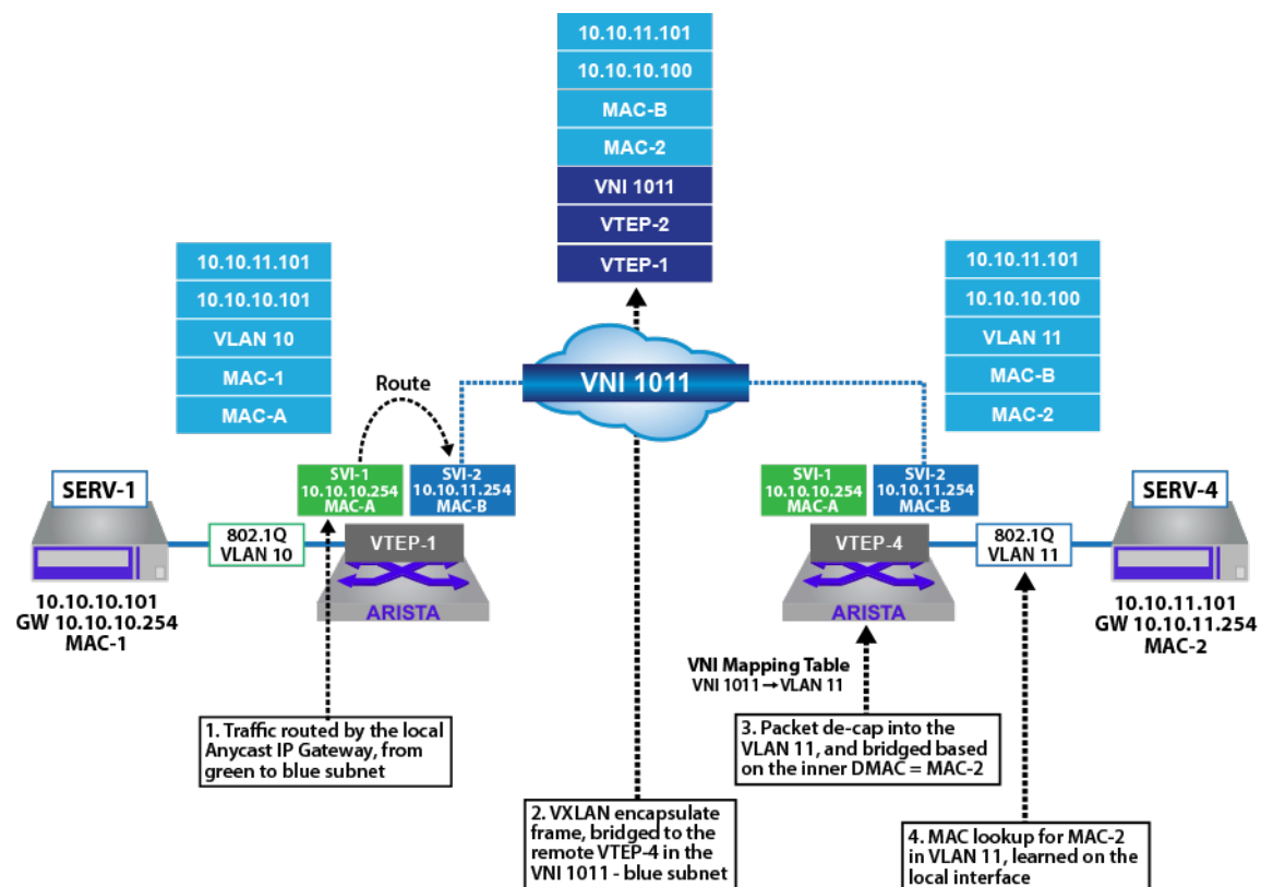
Figure 88: EVPN Asymmetric IRB VxLAN Data-plane Forwarding Detail
