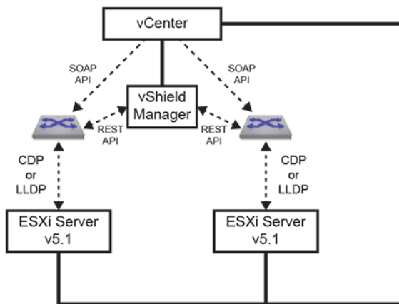
Figure 144: VM Tracer Topology – Monitoring VXLAN Based Configurations
