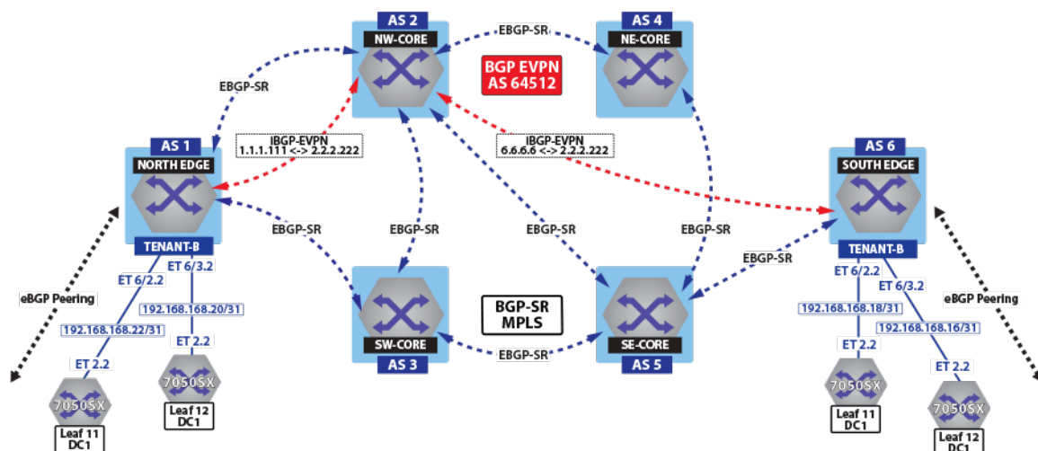
Figure 126: Control Plane Tenant-B Over BGP-SR
