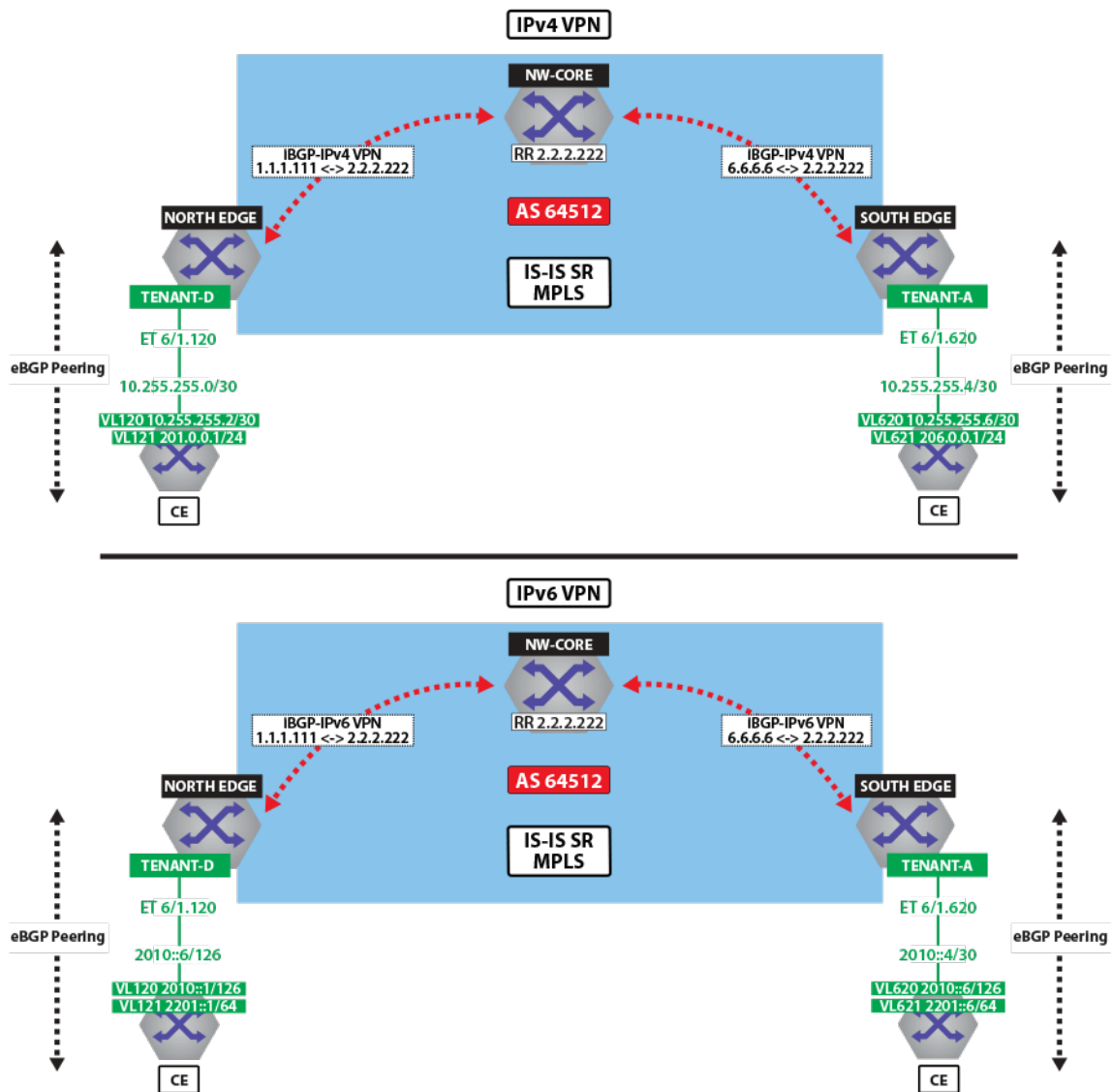
Figure 130: IPv4 VPN and IPv6 VPN Over ISIS-SR MPLS
