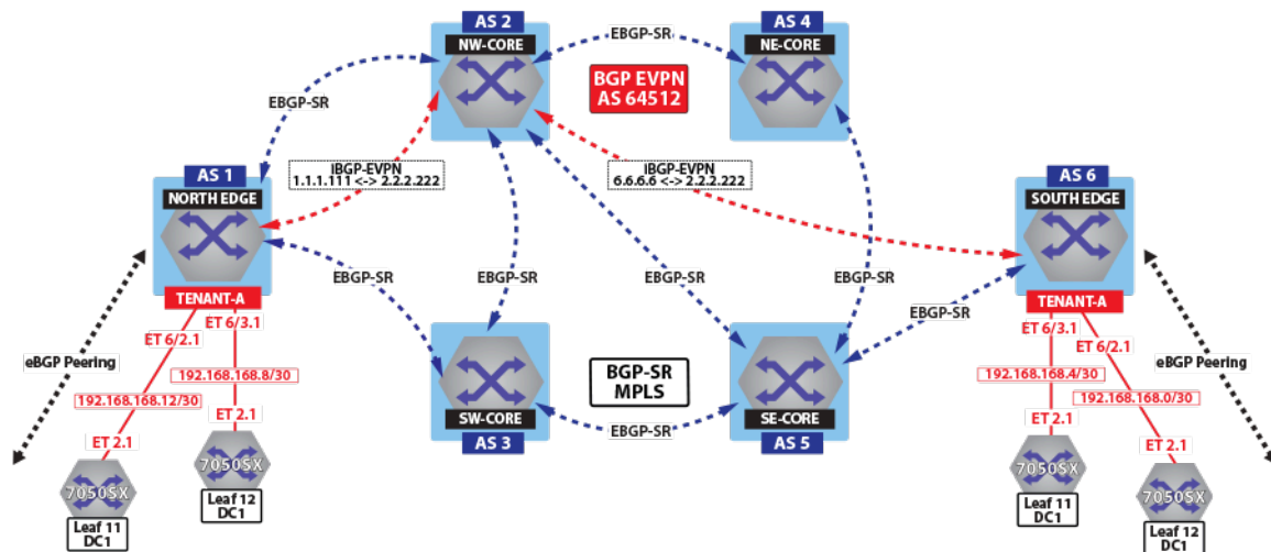
Figure 125: Control Plane Tenant-A Over BGP-SR
