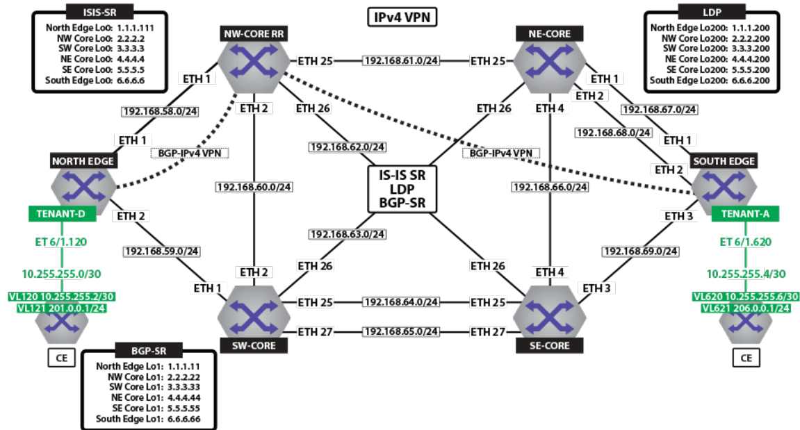
Figure 102: Tenant-D IPv4 VPN
