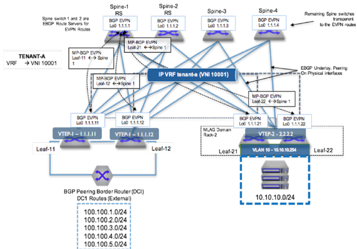
Figure 115: Layer 3 EVPN Configuration
