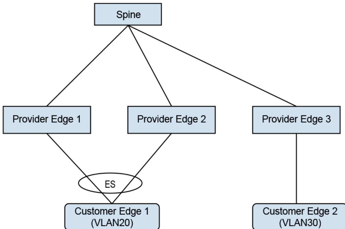
Figure 114: Asymmetric IRB with IPv4
