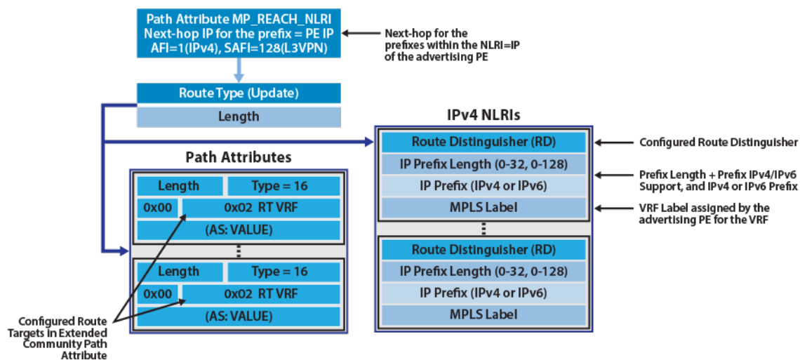
Figure 94: IPv4 and IPv6 VPN Update Route Detail
