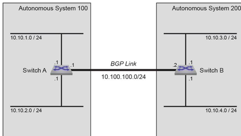
Figure 59: BGP Example 2
