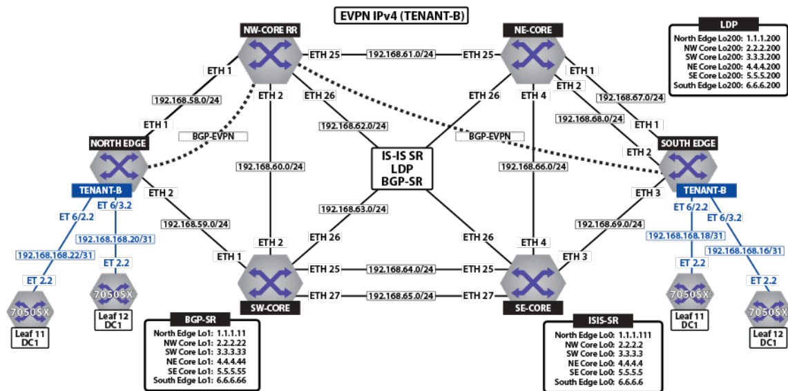
Figure 100: Tenant-B DCI
