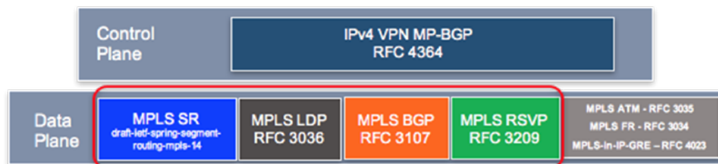
Figure 92: MPLS data-plane
