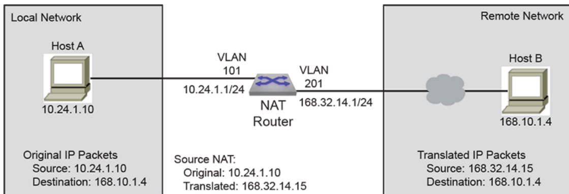
Figure 8: Source NAT Example
