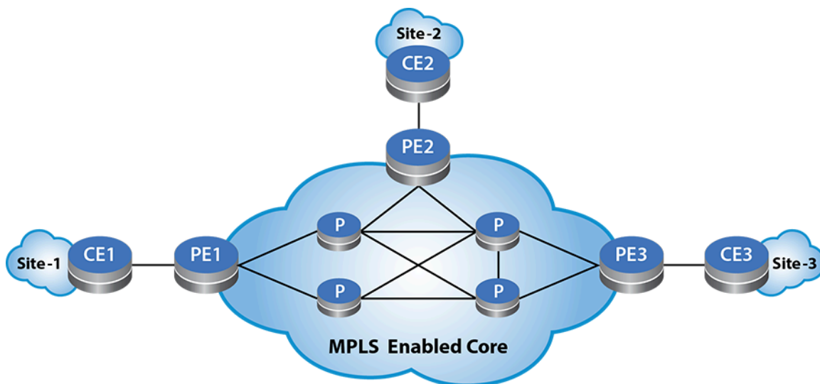
Figure 140: MPLS Enabled Core Schematic
