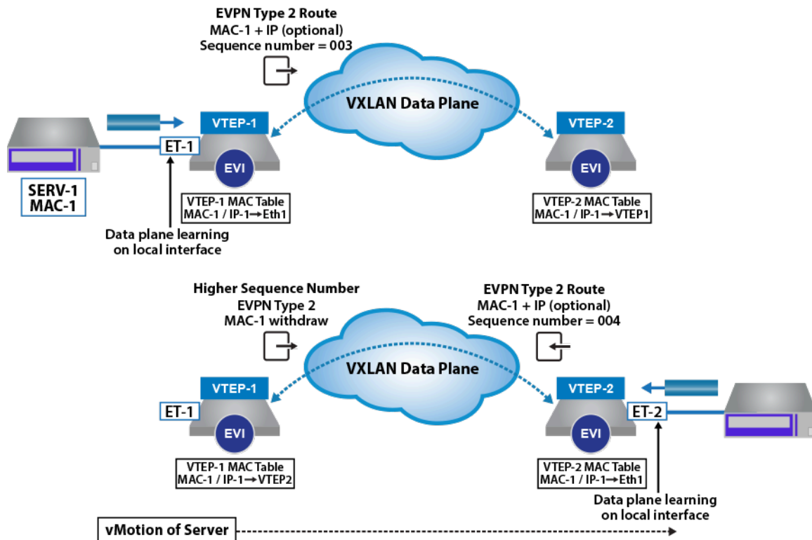
Figure 83: EVPN type-2 MAC Mobility Behavior
