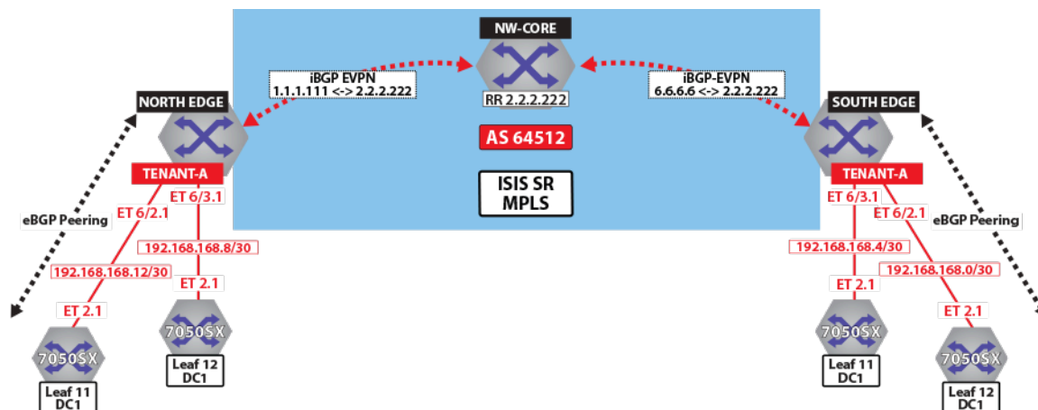
Figure 119: Control Plane Tenant-A Over ISIS-SR
