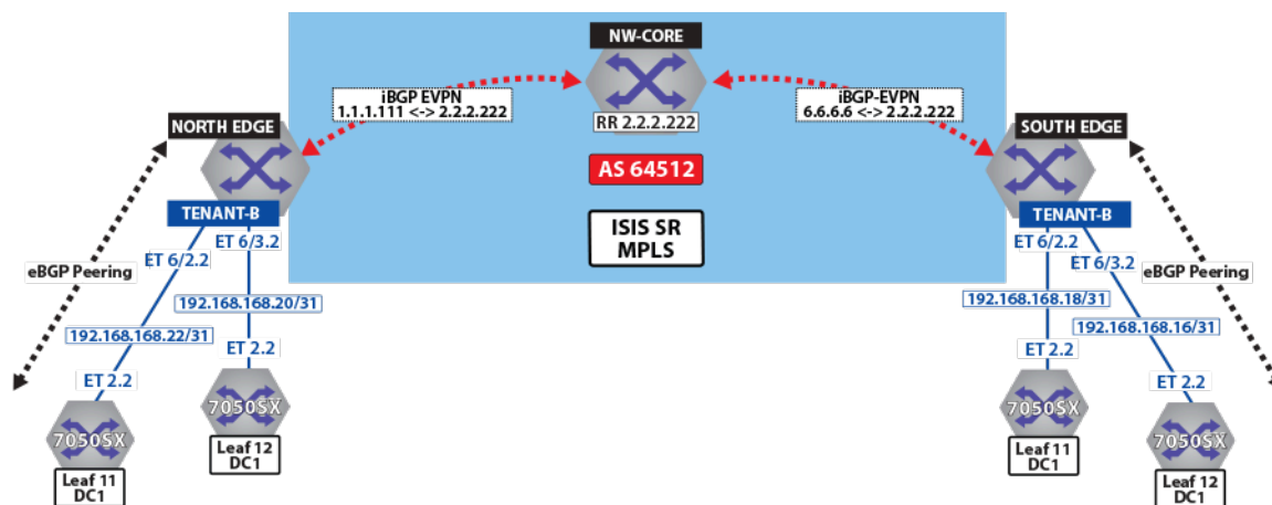
Figure 120: Control Plane Tenant-B over ISIS-SR
