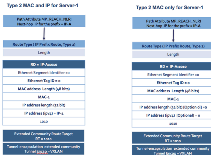
Figure 87: EVPN Comparison of MAC & MAC+IP Type 2 Route in Asymmetric IRB
