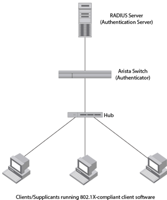
Figure 7: Multiple clients connected to a 802.1X-enabled port
