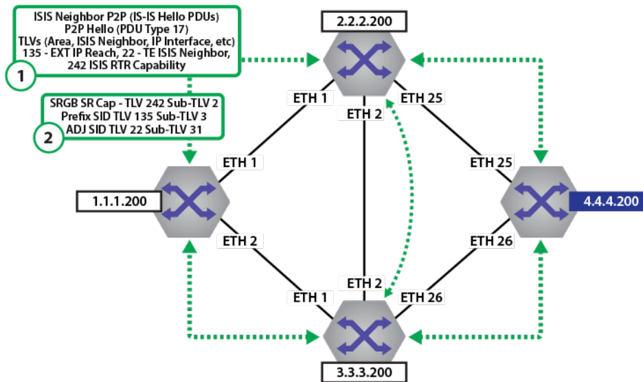
Figure 105: ISIS Neighbor Adj and TLVs
