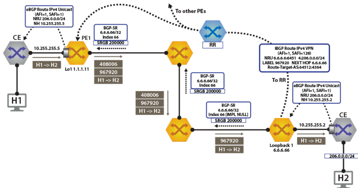
Figure 137: IPv4 VPN Forwarding Over BGP-SR MPLS
