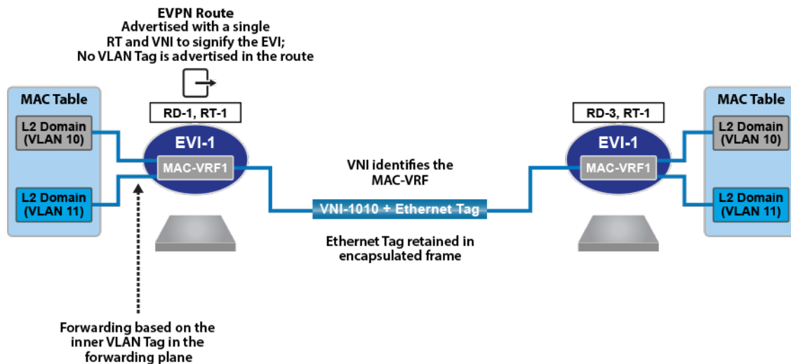
Figure 76: VLAN Bundle Service Interface
