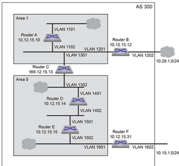
Figure 53: OSPFv3 Example 3
