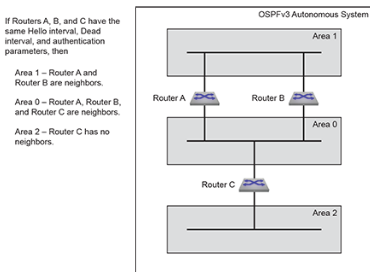
Figure 50: OSPFv3 Neighbors
