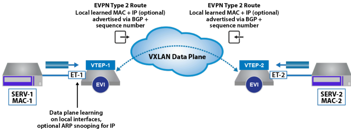
Figure 81: EVPN Type 2 Route Announcement
