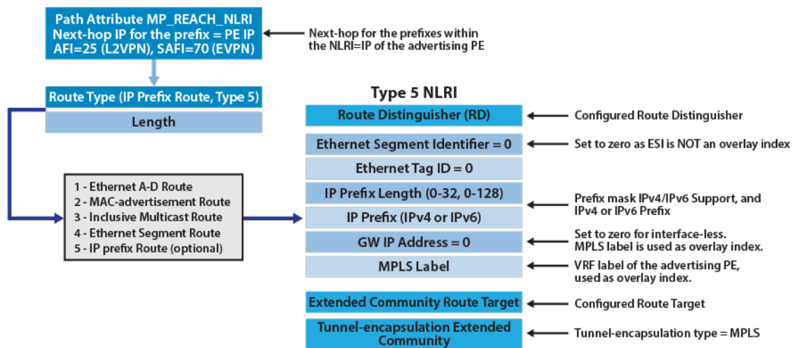
Figure 108: EVPN Route Type-5, for Advertisement of IP Prefixes
