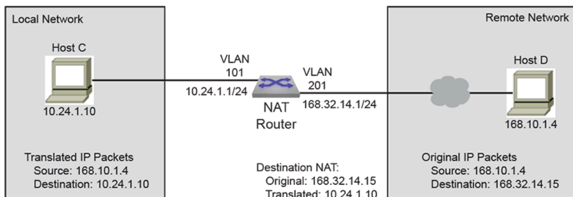
Figure 9: Detination NAT Example
