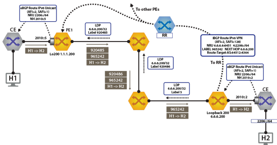
Figure 135: IPv6 VPN Forwarding Over LDP MPLS
