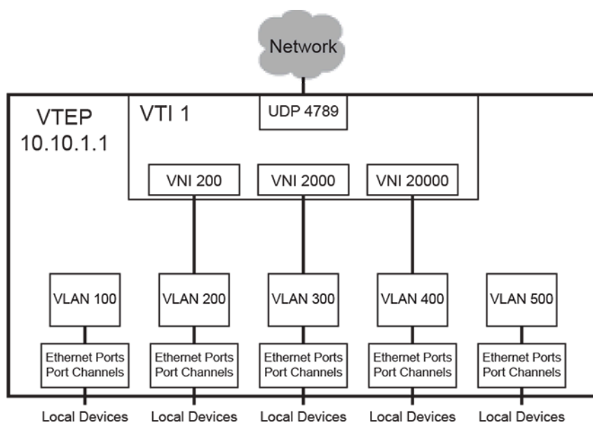
Figure 66: VXLAN Architecture
