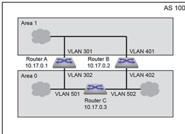
Figure 51: OSPFv3 Example 1
