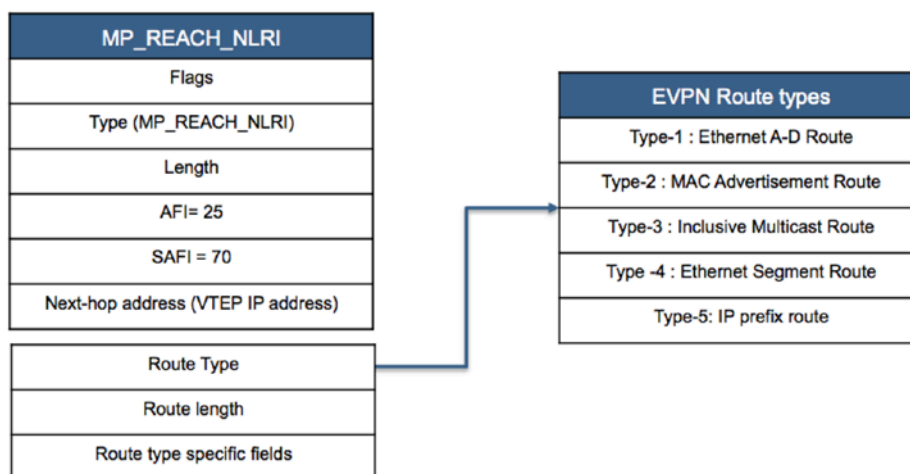
Figure 73: EVPN NLRI Route Format
