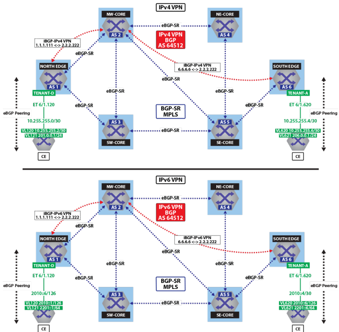
Figure 136: IPv4 VPN and IPv6 VPN Over BGP-SR MPLS
