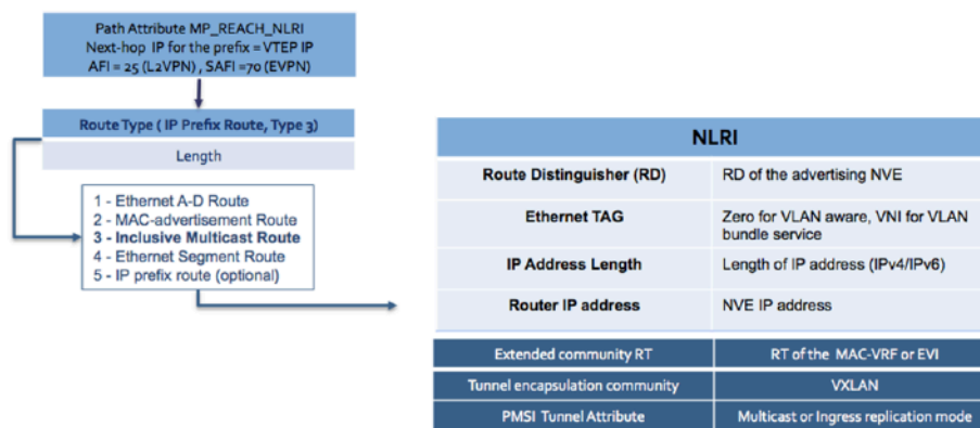
Figure 85: EVPN Type-3 IMET Route Format
