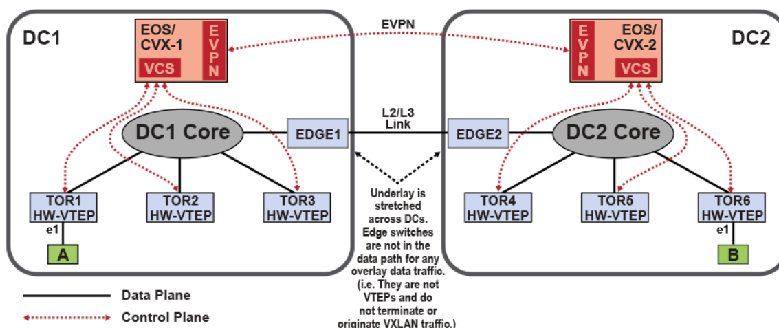
Figure 78: CVX Connected from Multiple DCs
