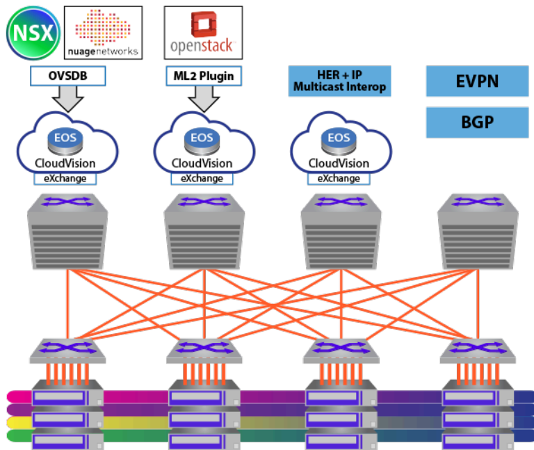
Figure 70: Different VXLAN Control Planes
