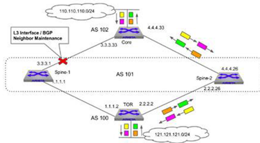
Figure 61: Traffic flow pattern between TOR and Core After unit on Spine-1 is put into Maintenance
