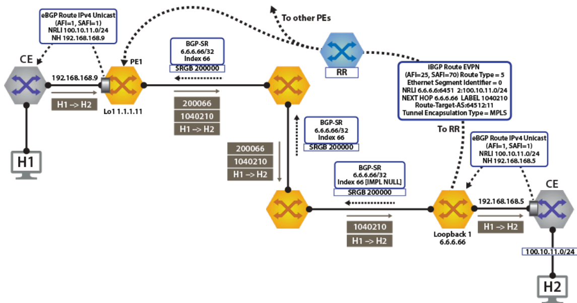
Figure 127: Control Plane & Forwarding Tenant-A Over BGP-SR
