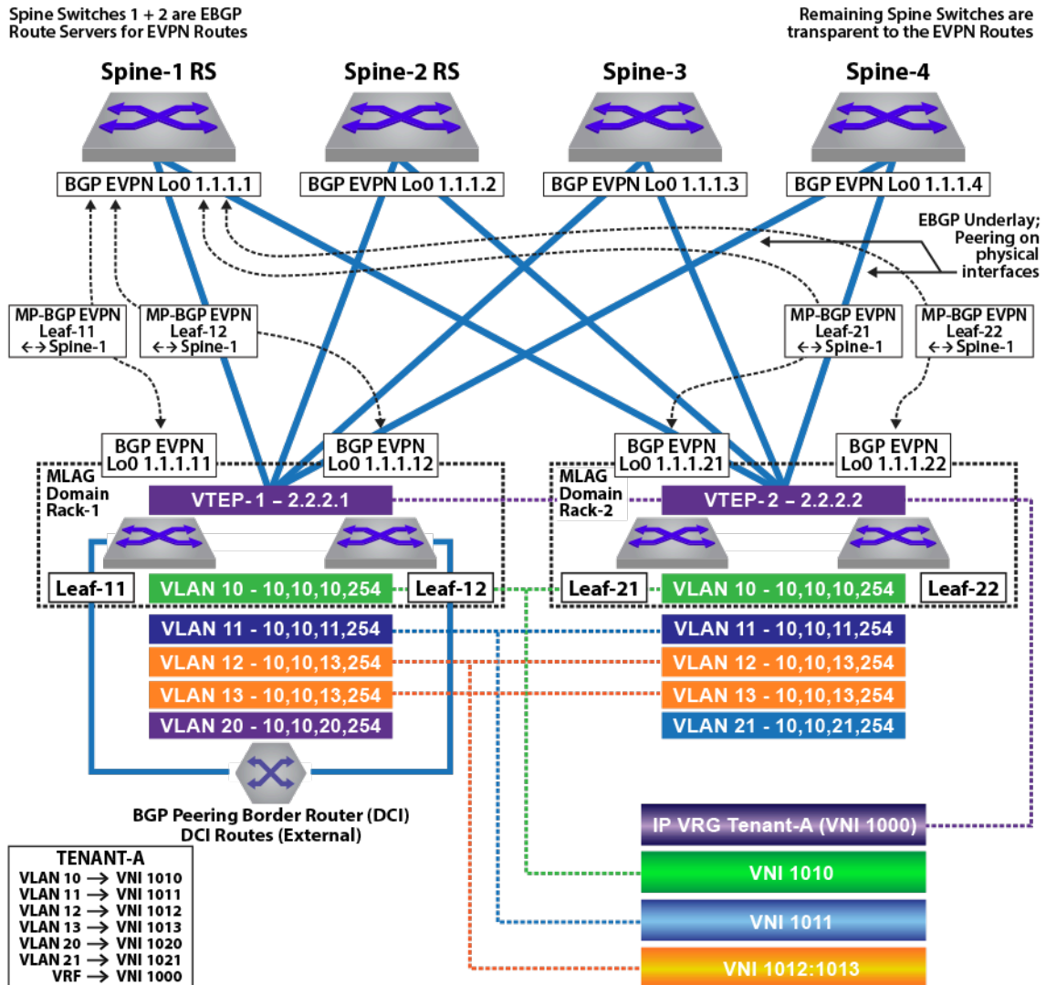
Figure 116: Tenant-A: Symmetric IRB
