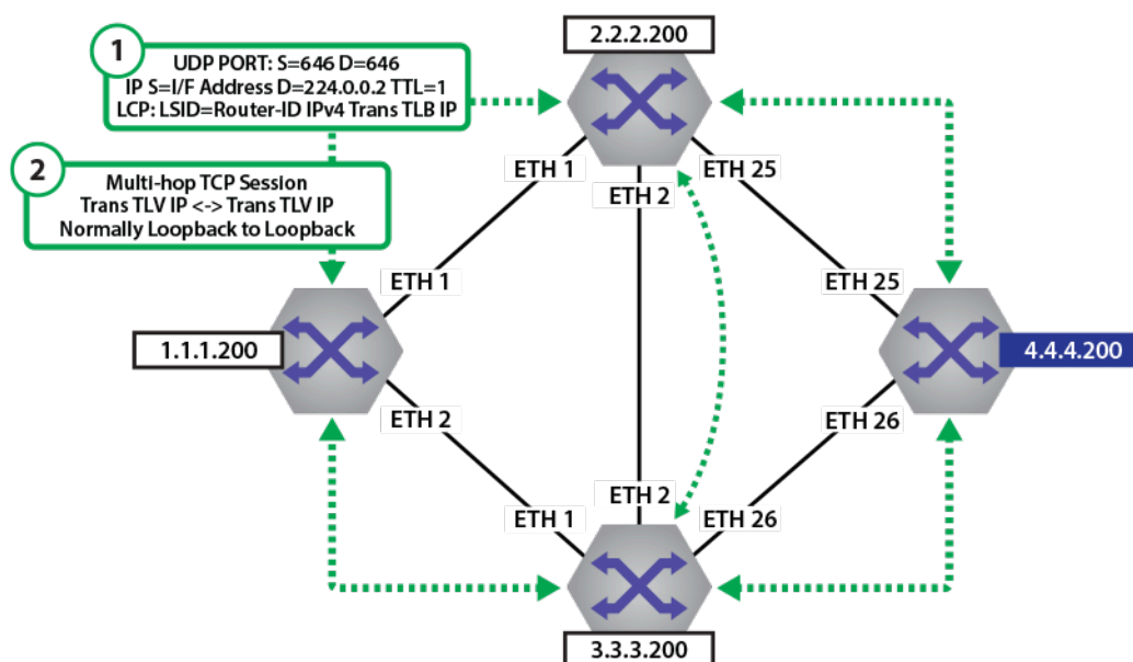
Figure 104: LDP Peering Establishment
