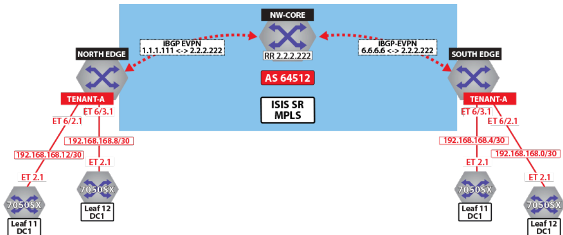
Figure 122: Control Plane Tenant-A Over LDP
