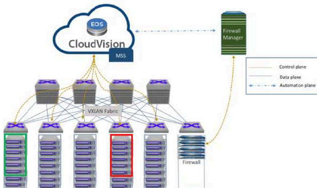
Figure 11: Securing server-server traffic
