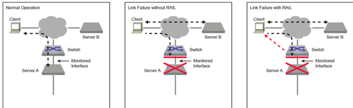
Figure 25: RAIL Scenarios
