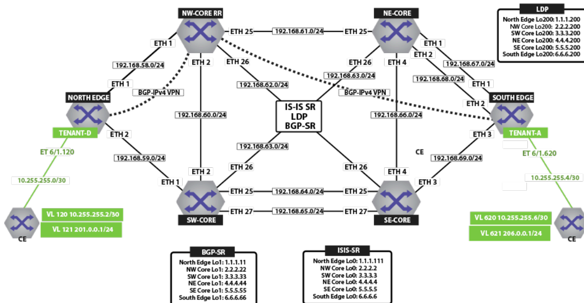
Figure 128: IPv4 VPN Physical Topology
