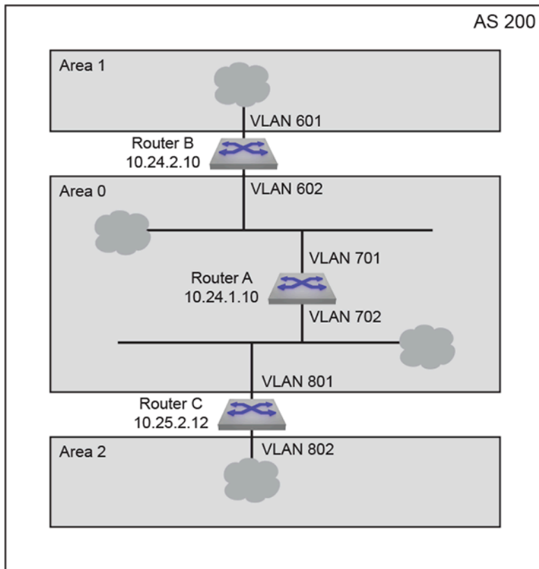
Figure 52: OSPFv3 Example 2
