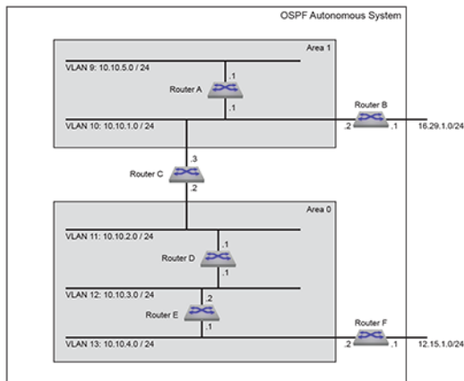
Figure 35: OSPFv2 Example 3
