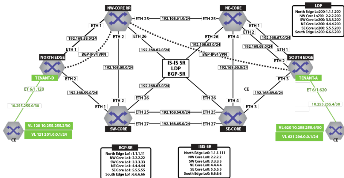
Figure 110: IPv4 VPN Physical Topology
