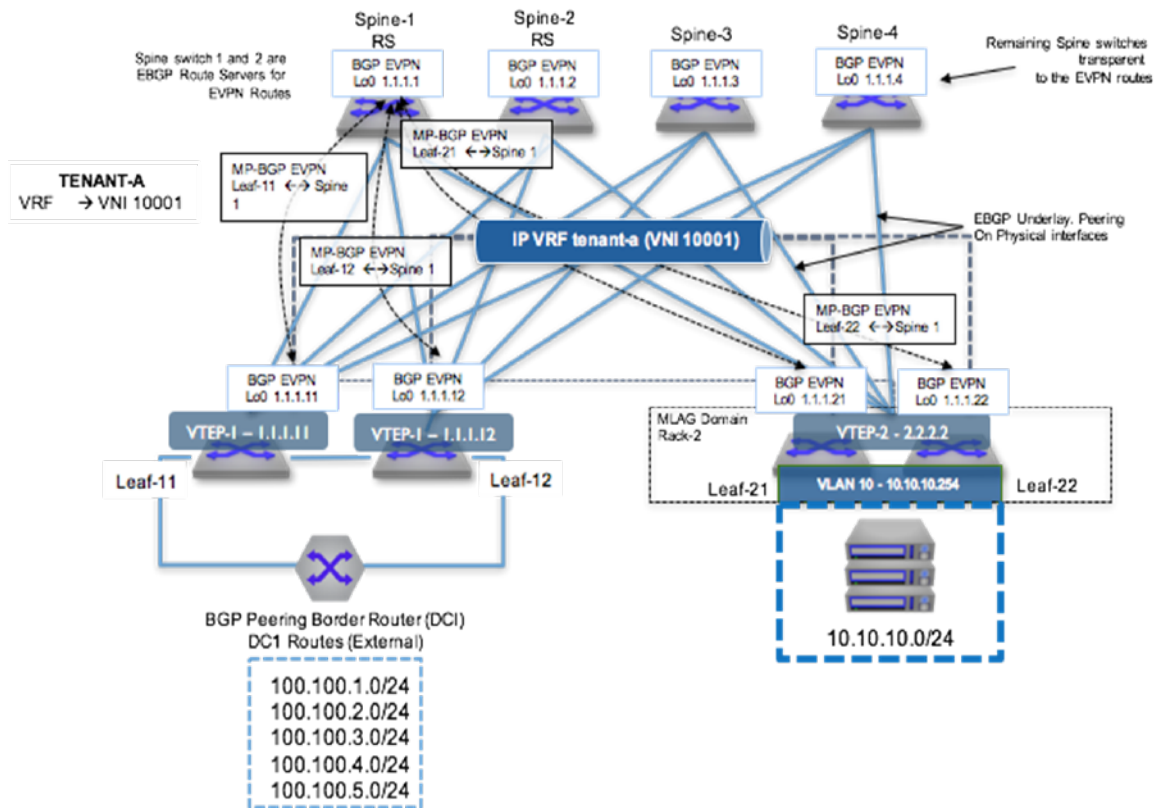
Figure 97: Layer 3 EVPN Configuration
