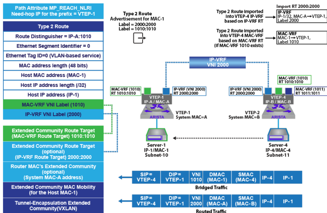
Figure 74: EVPN Type 2 Route in Symmetric IRB - MAC-VRF on Both VTEPs
