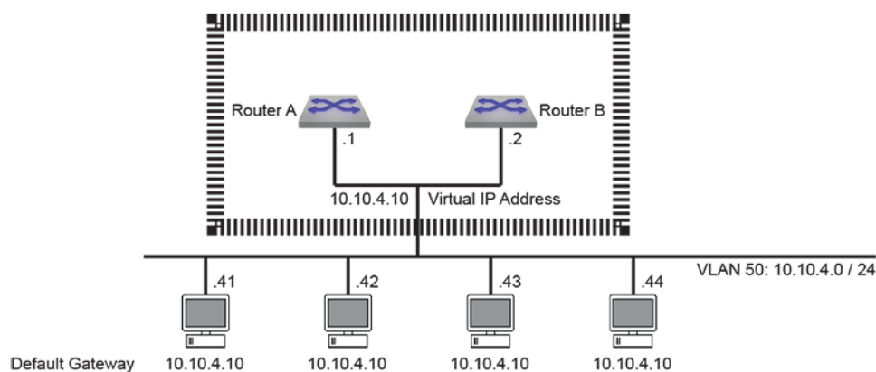
Figure 17: VARP Configuration
