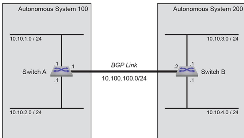
Figure 43: BGP Example 2
