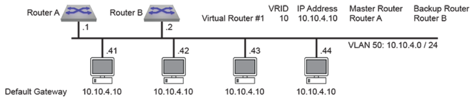
Figure 18: VRRP Example 1 Network Diagram
