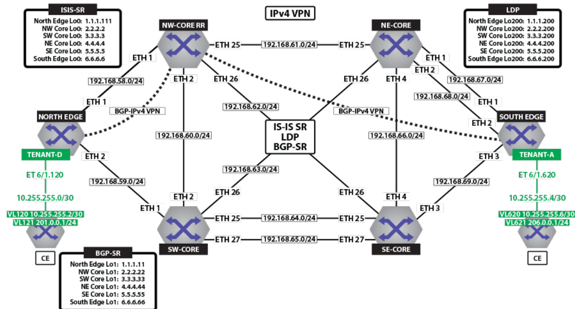
Figure 86: Tenant-D IPv4 VPN
