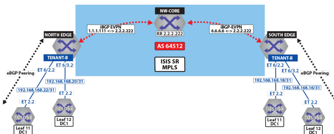
Figure 102: Control Plane Tenant-B over ISIS-SR
