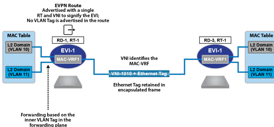
Figure 60: VLAN Bundle Service Interface
