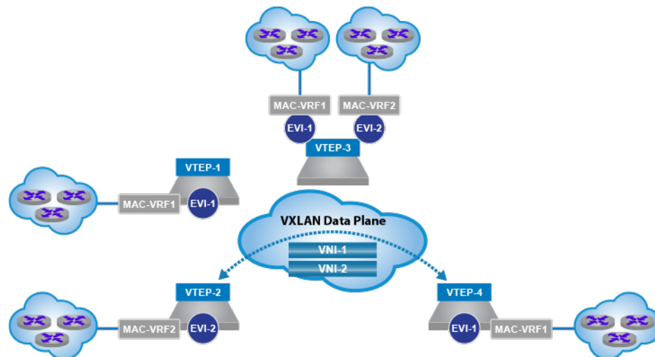
Figure 56: EVPN Terminology for a VXLAN Data Plane
