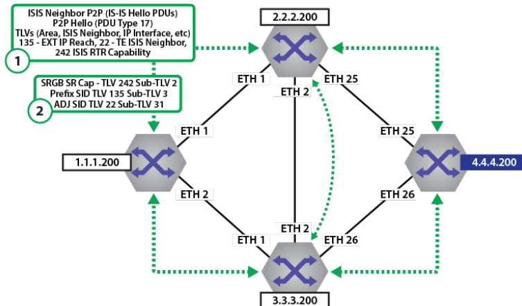
Figure 89: ISIS Neighbor Adj and TLVs
