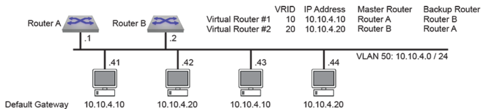
Figure 19: VRRP Example 2 Network Diagram
