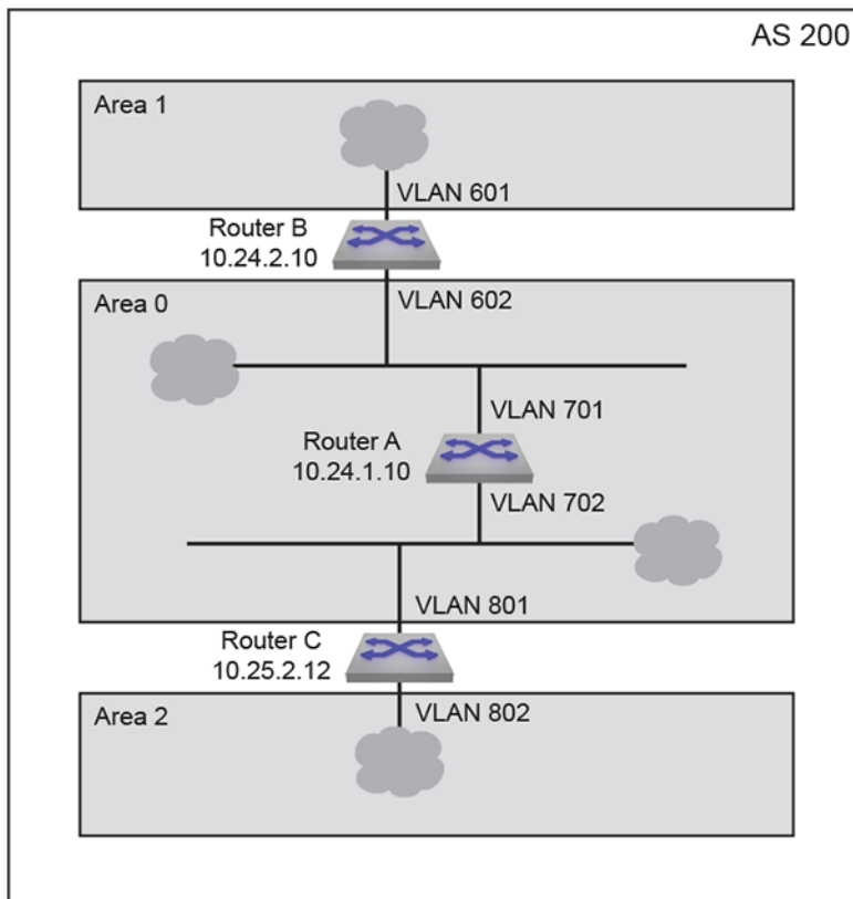
Figure 39: OSPFv3 Example 2
