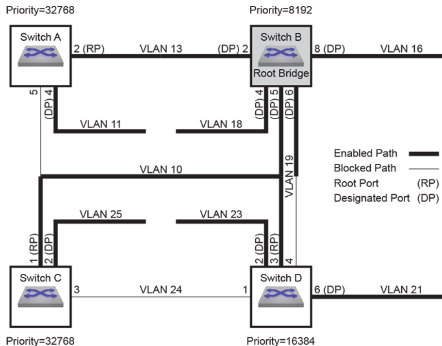
Figure 13: Spanning Tree Network Example
