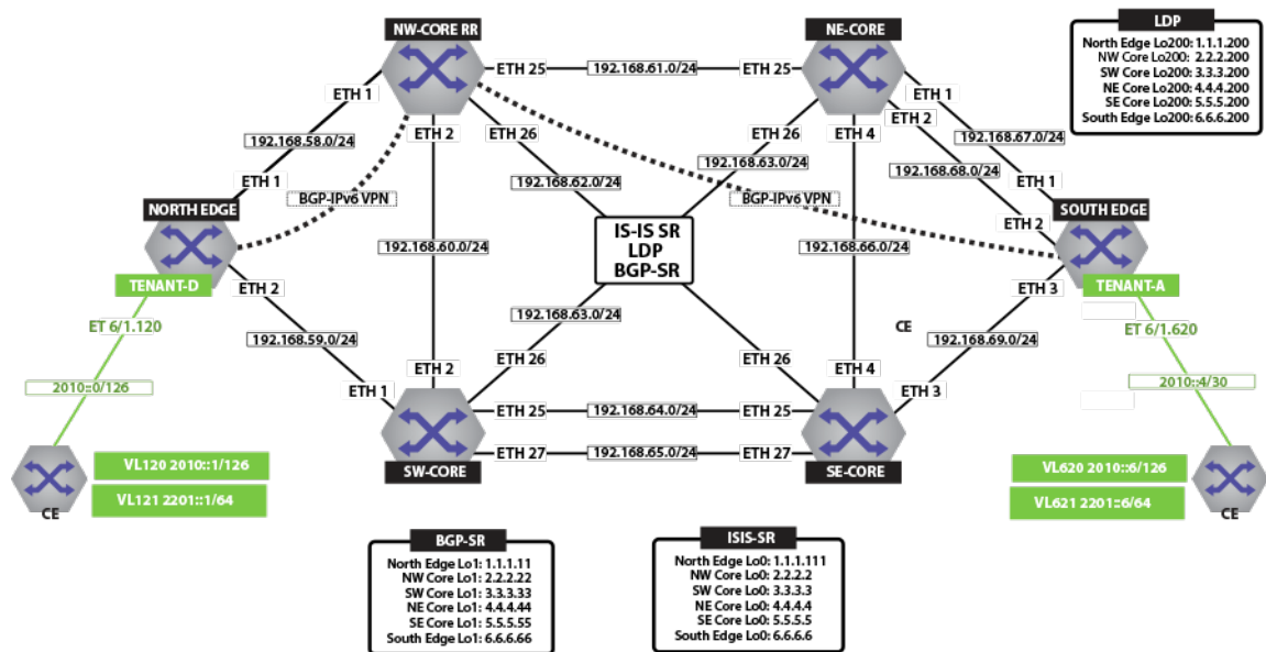
Figure 111: IPv6 VPN Physical Topology
