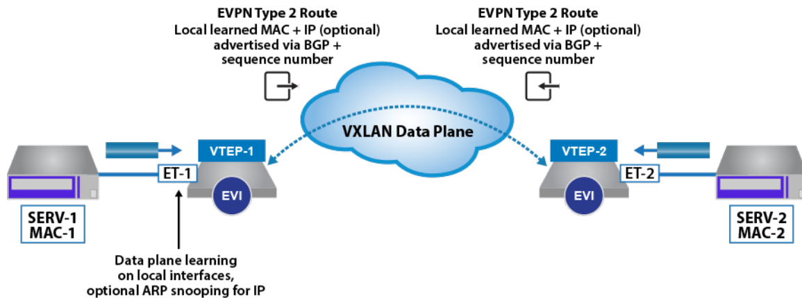
Figure 65: EVPN Type 2 Route Announcement
