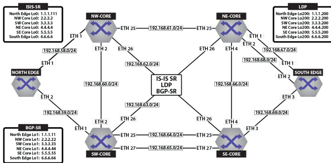
Figure 82: Physical Topology For ISIS-SR, LDP and BGP-SR Transport
