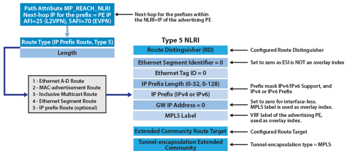
Figure 63: EVPN Route Type-5, for Advertisement of IP-Prefixes over MPLS
