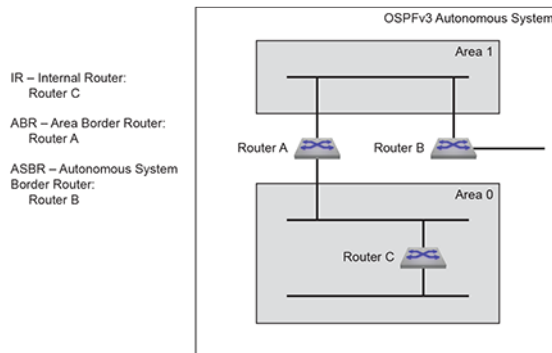
Figure 36: OSPFv3 Router Types
