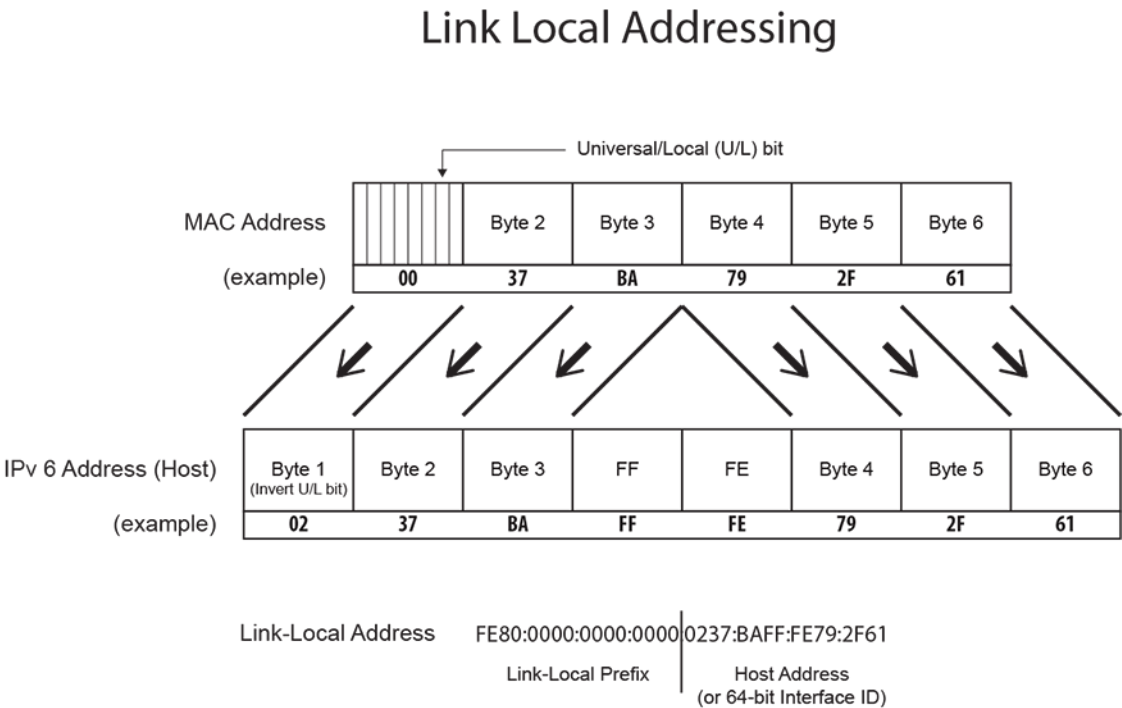
Figure 15: Link Local Address Derivation
