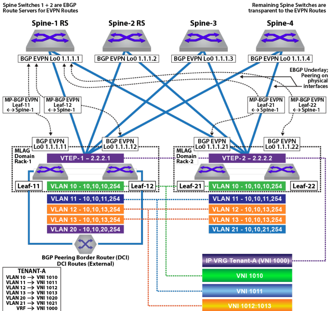
Figure 98: Tenant-A: Symmetric IRB
