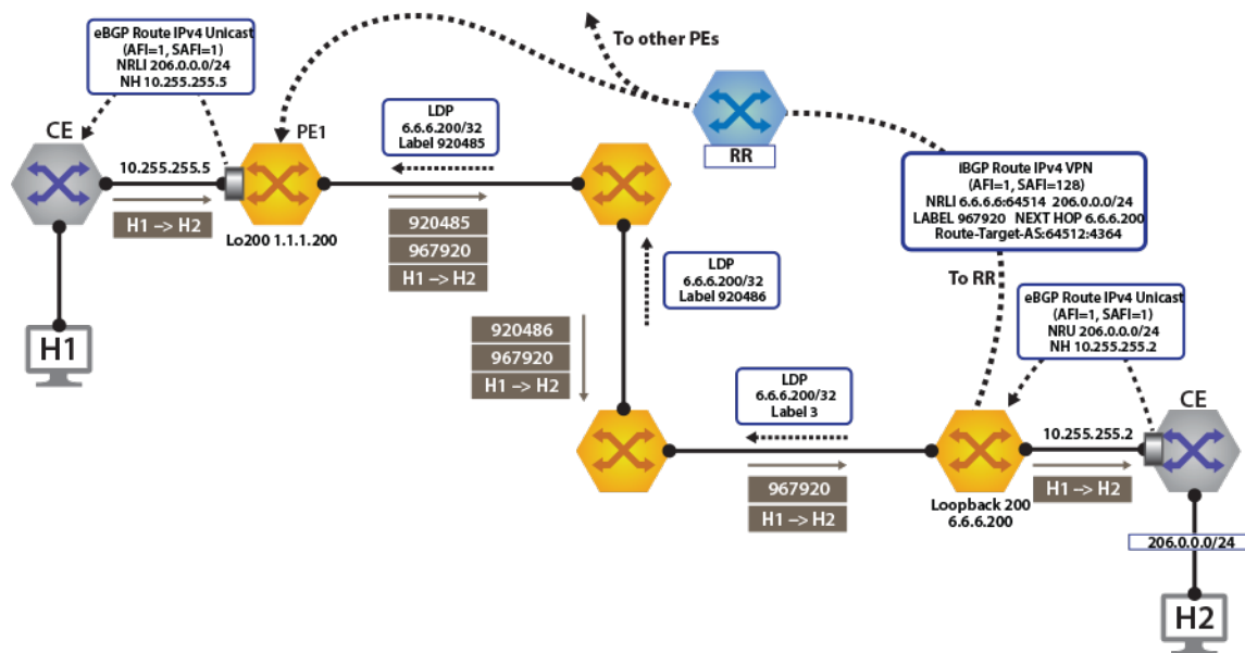
Figure 116: IPv4 VPN Forwarding Over LDP MPLS
