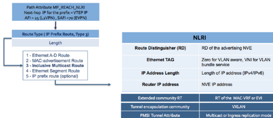
Figure 69: EVPN Type-3 IMET Route Format
