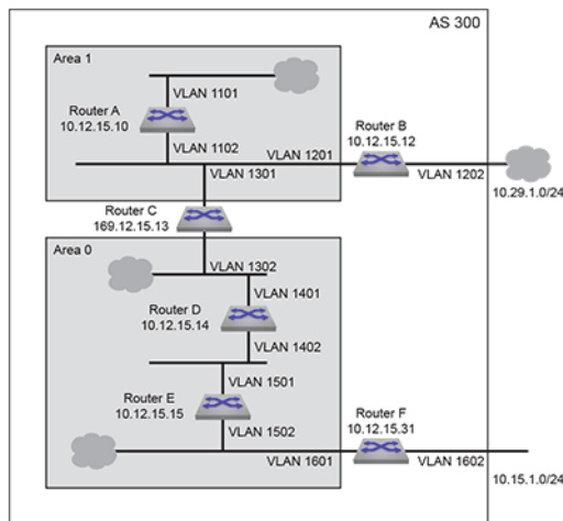
Figure 40: OSPFv3 Example 3
