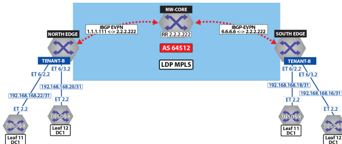
Figure 105: Control Plane Tenant-B over LDP
