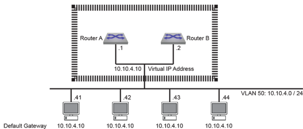
Figure 16: VARP Configuration
