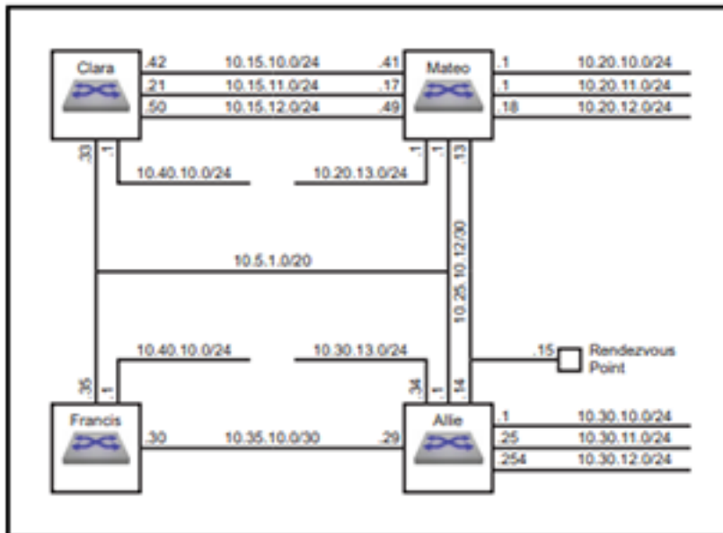
Figure 49: Multicast Example
