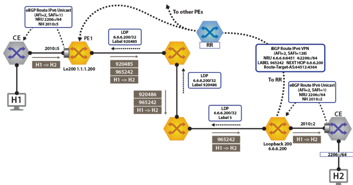
Figure 117: IPv6 VPN Forwarding Over LDP MPLS
