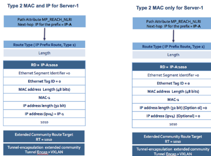
Figure 71: EVPN Comparison of MAC & MAC+IP Type 2 Route in Asymmetric IRB
