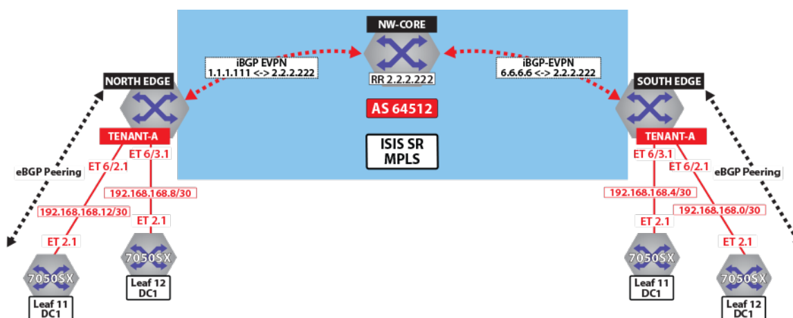
Figure 101: Control Plane Tenant-A Over ISIS-SR
