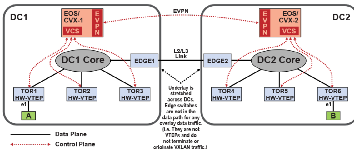
Figure 62: CVX Connected from Multiple DCs
