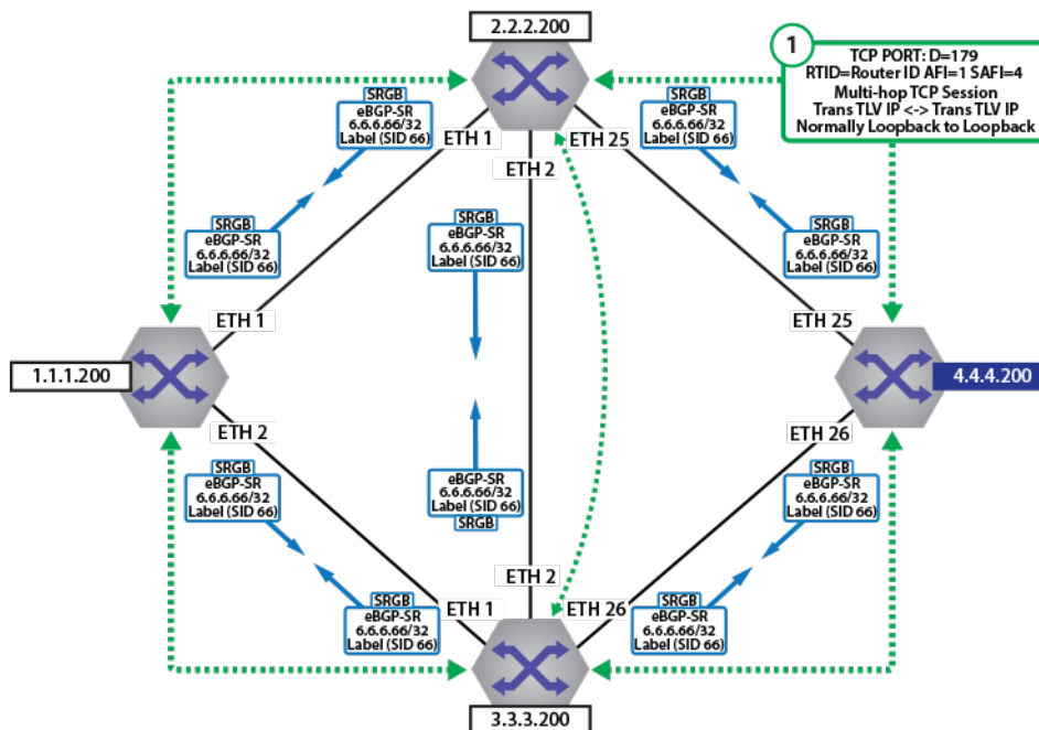
Figure 91: BGP-SR Index and SRGB Distribution
