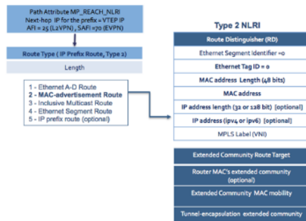
Figure 66: EVPN Type 2 MAC and IP Route Format
