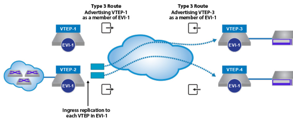
Figure 68: EVPN type-3 IMET Route Behavior for Ingress Replication
