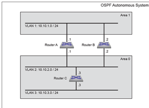
Figure 33: OSPFv2 Example 1
