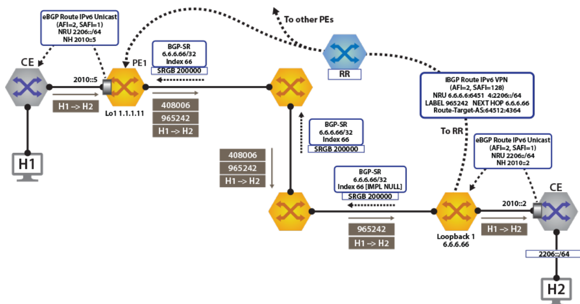
Figure 120: IPv6 VPN Forwarding Over BGP-SR MPLS
