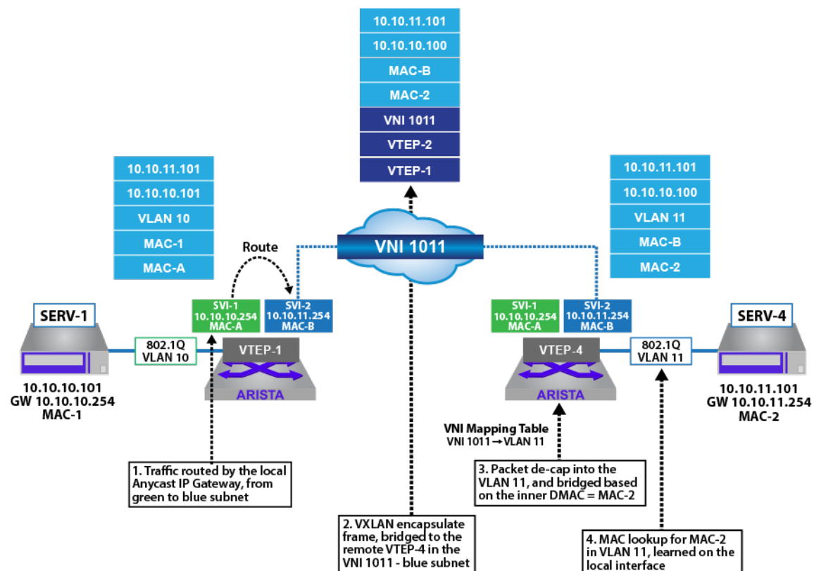
Figure 72: EVPN Asymmetric IRB VxLAN Data-plane Forwarding Detail
