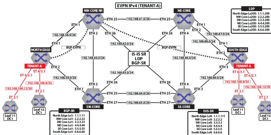
Figure 83: Tenant-A DCI
