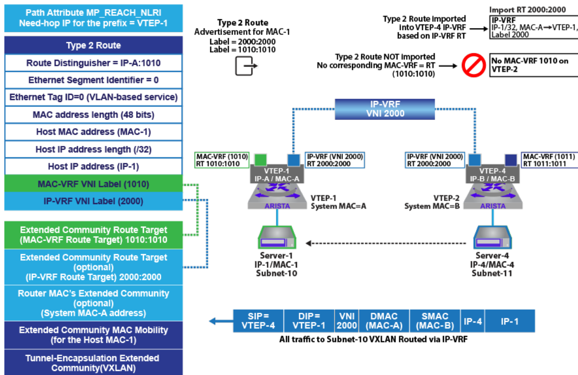
Figure 75: EVPN Type 2 Route in Symmetric IRB - MAC-VRF Only Exists on Sending VTEP
