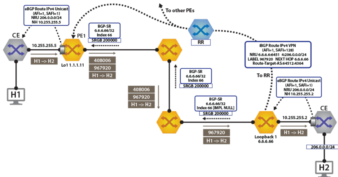
Figure 119: IPv4 VPN Forwarding Over BGP-SR MPLS
