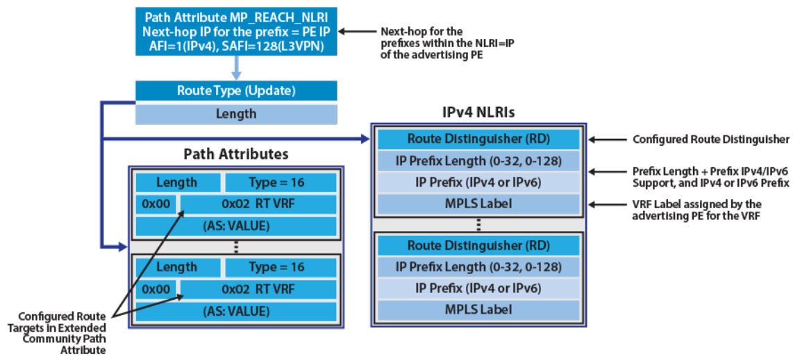
Figure 78: IPv4 and IPv6 VPN Update Route Detail
