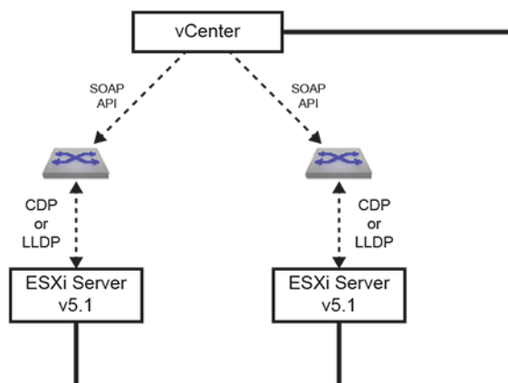
Figure 125: VM Tracer Topology – Monitoring VLAN Based Configurations
