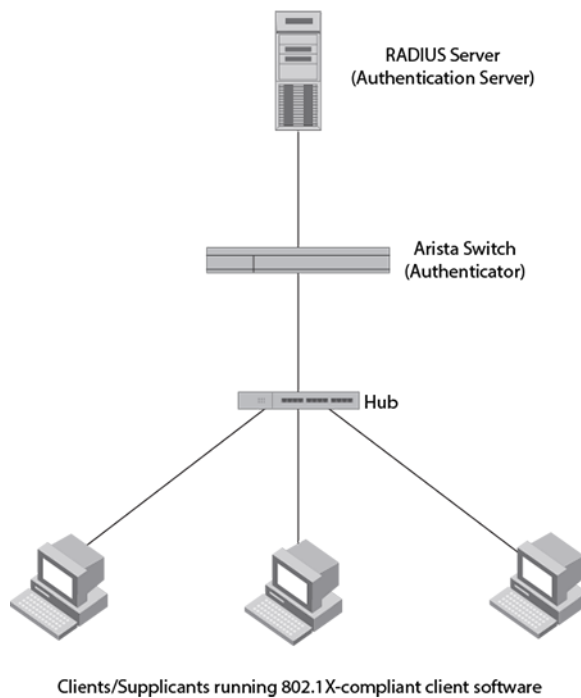
Figure 7: Multiple clients connected to a 802.1X-enabled port
