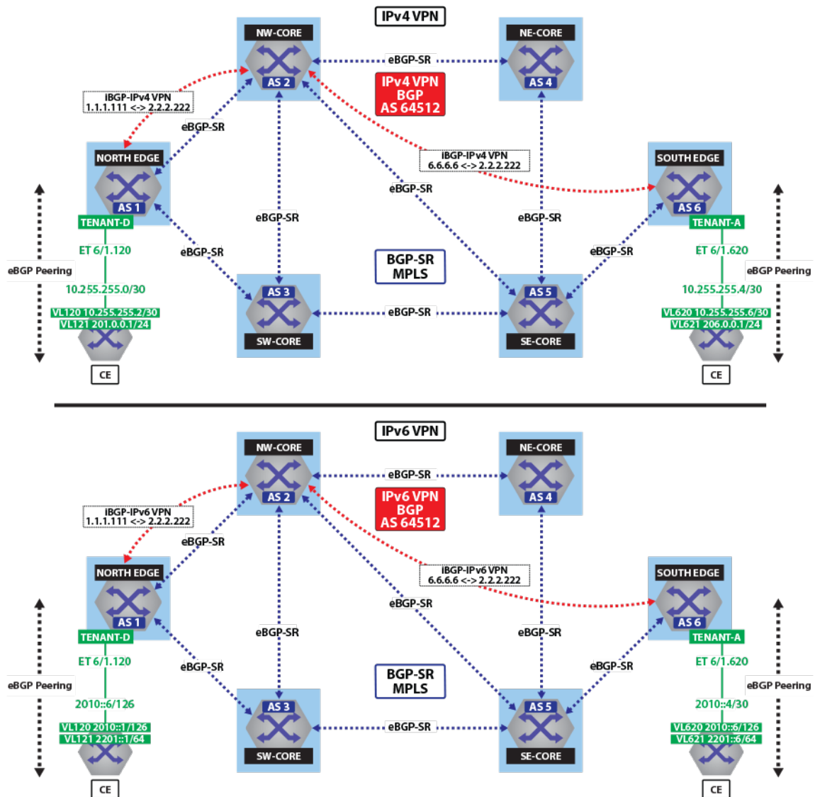
Figure 118: IPv4 VPN and IPv6 VPN Over BGP-SR MPLS
