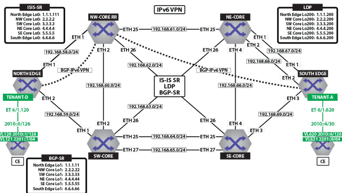
Figure 87: Tenant-D IPv6 VPN
