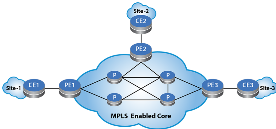
Figure 122: MPOLS Enabled Core Schematic
