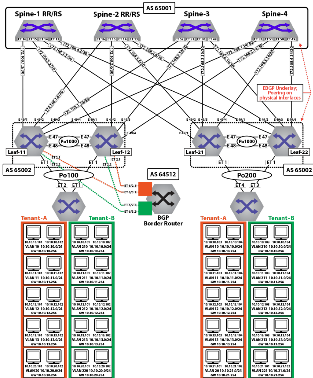
Figure 100: Physical Underlay Topology
