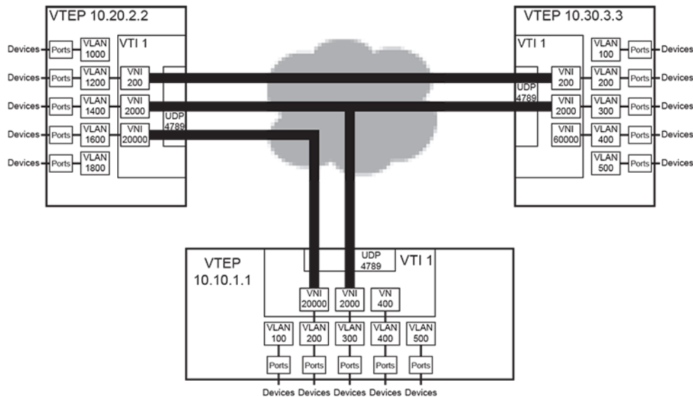
Figure 51: XLAN Implementation
