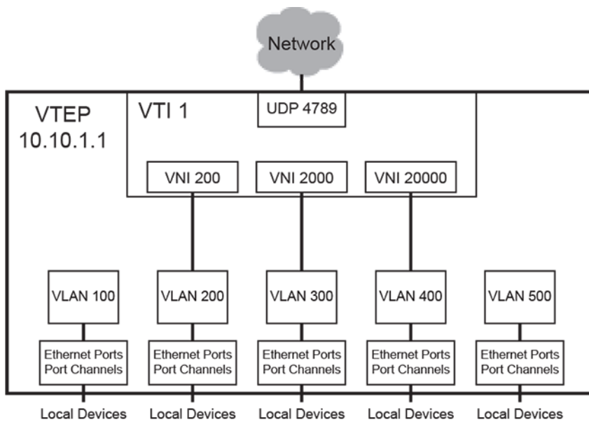
Figure 50: VXLAN Architecture
