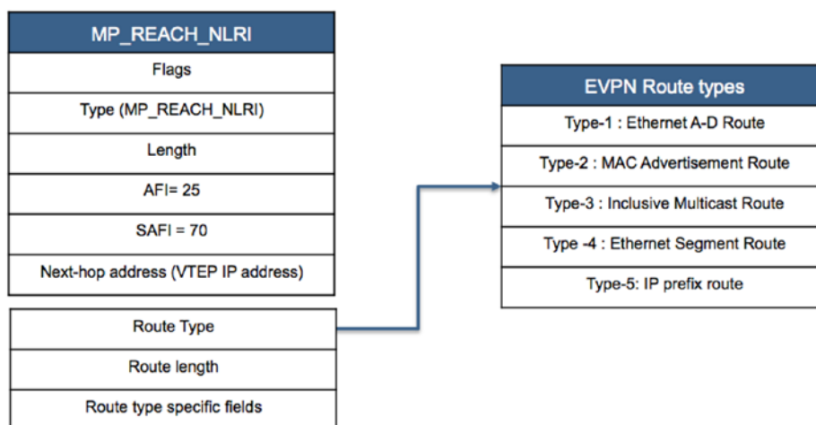
Figure 57: EVPN NLRI Route Format
