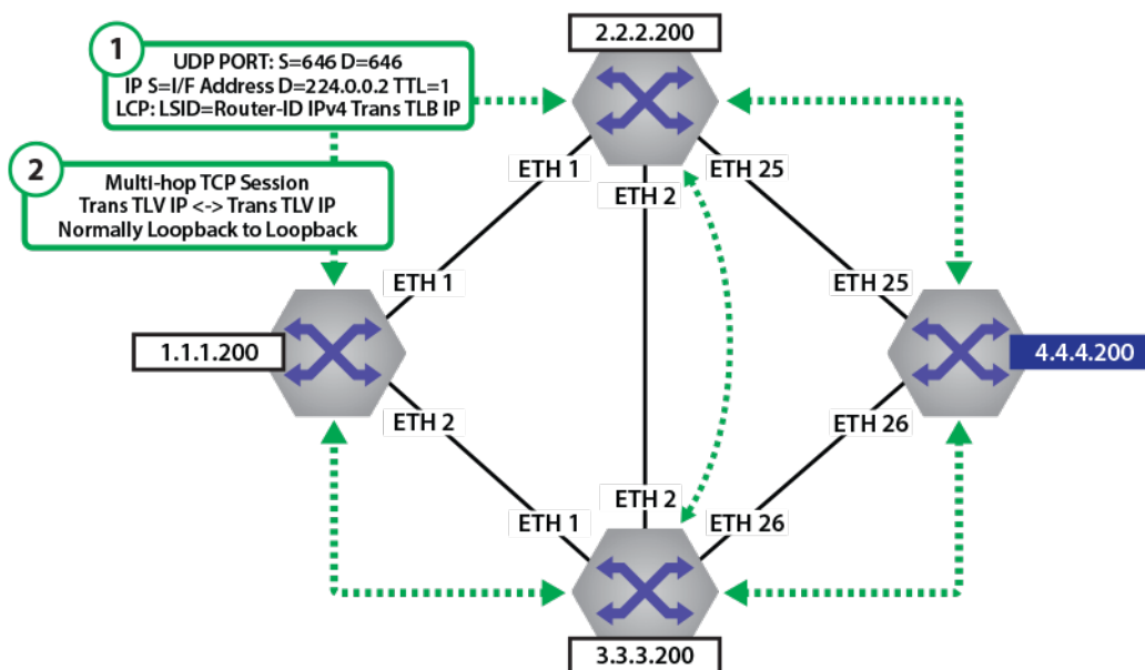
Figure 88: LDP Peering Establishment
