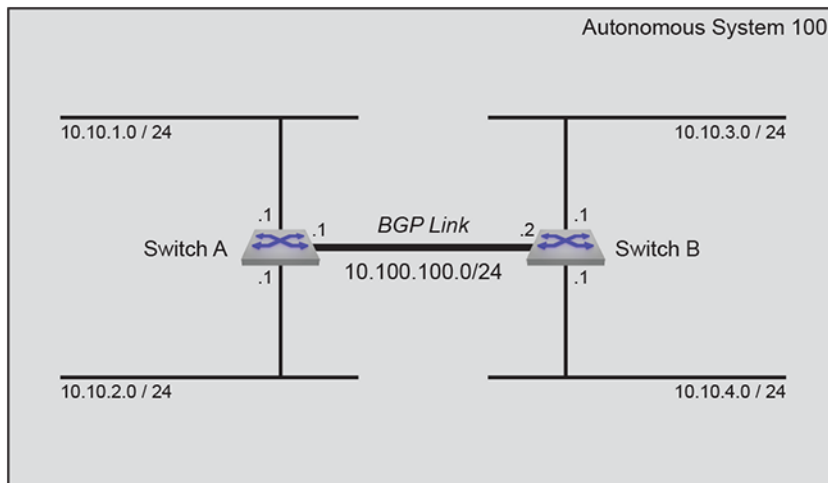
Figure 42: BGP Example 1
