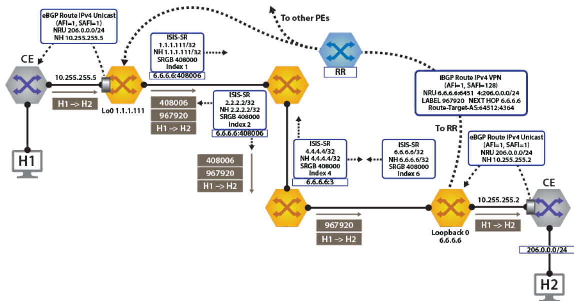
Figure 113: IPv4 VPN Forwarding Over ISIS-SR MPLS
