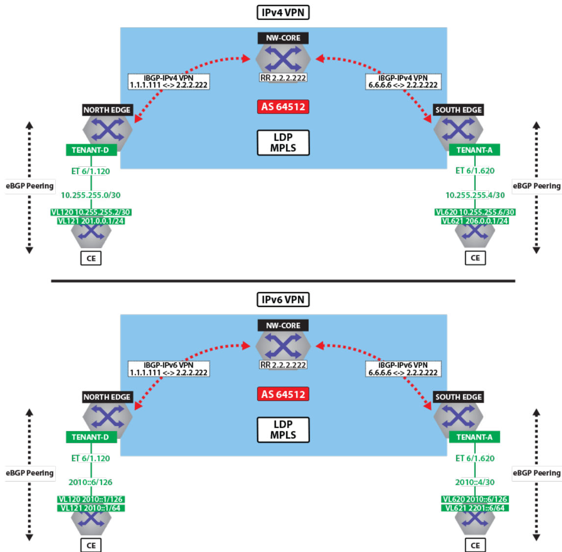
Figure 115: IPv4 VPN and IPv6 VPN Over LDP MPLS
