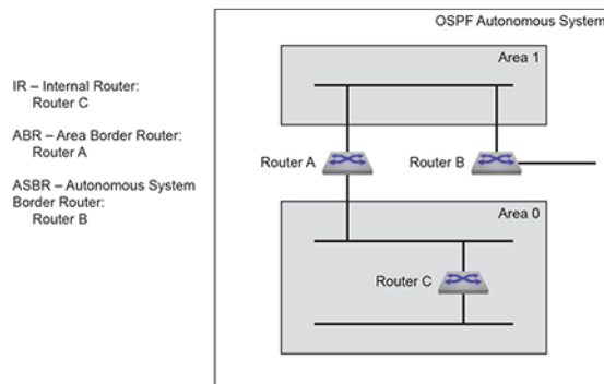
Figure 31: OSPFv2 Router Types
