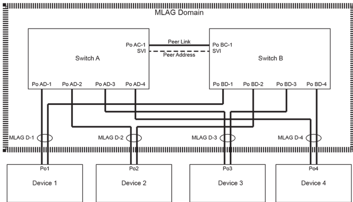
Figure 8: MLAG Domain Topology
