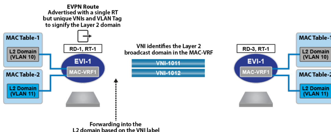
Figure 61: VLAN Aware Bundle Service
