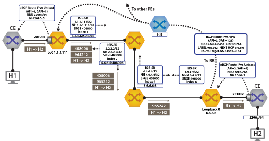
Figure 114: IPv6 VPN Forwarding Over ISIS-SR MPLS
