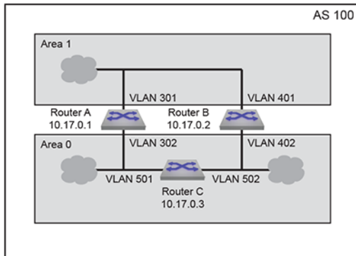
Figure 38: OSPFv3 Example 1
