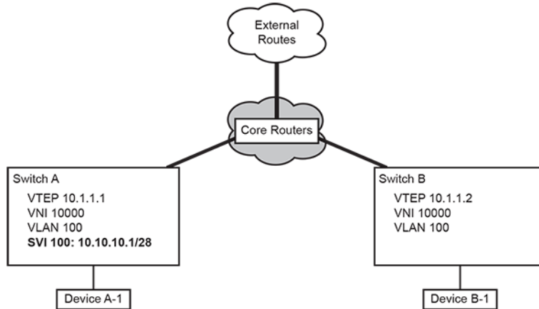
Figure 52: Implementing VXLAN Routing
