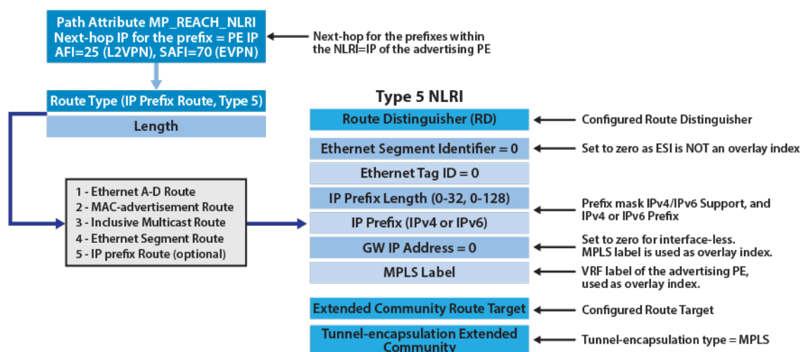
Figure 92: EVPN Route Type-5, for Advertisement of IP Prefixes
