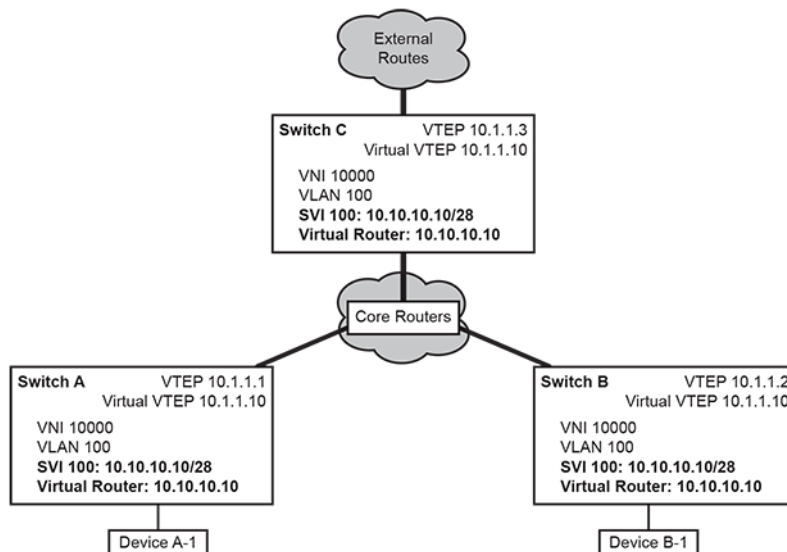
Figure 53: Direct VXLAN Routing
