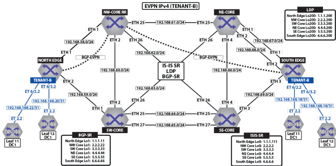
Figure 84: Tenant-B DCI
