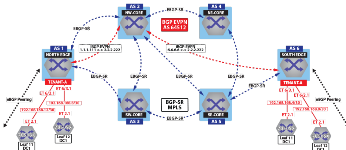
Figure 107: Control Plane Tenant-a Over BGP-SR
