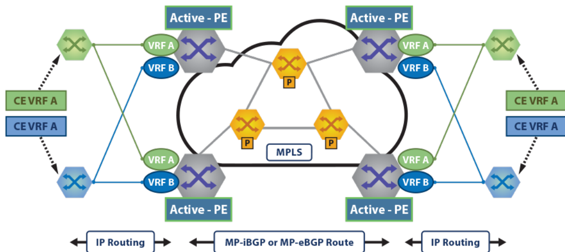
Figure 81: MPLS Layer 3 VPN Topology
