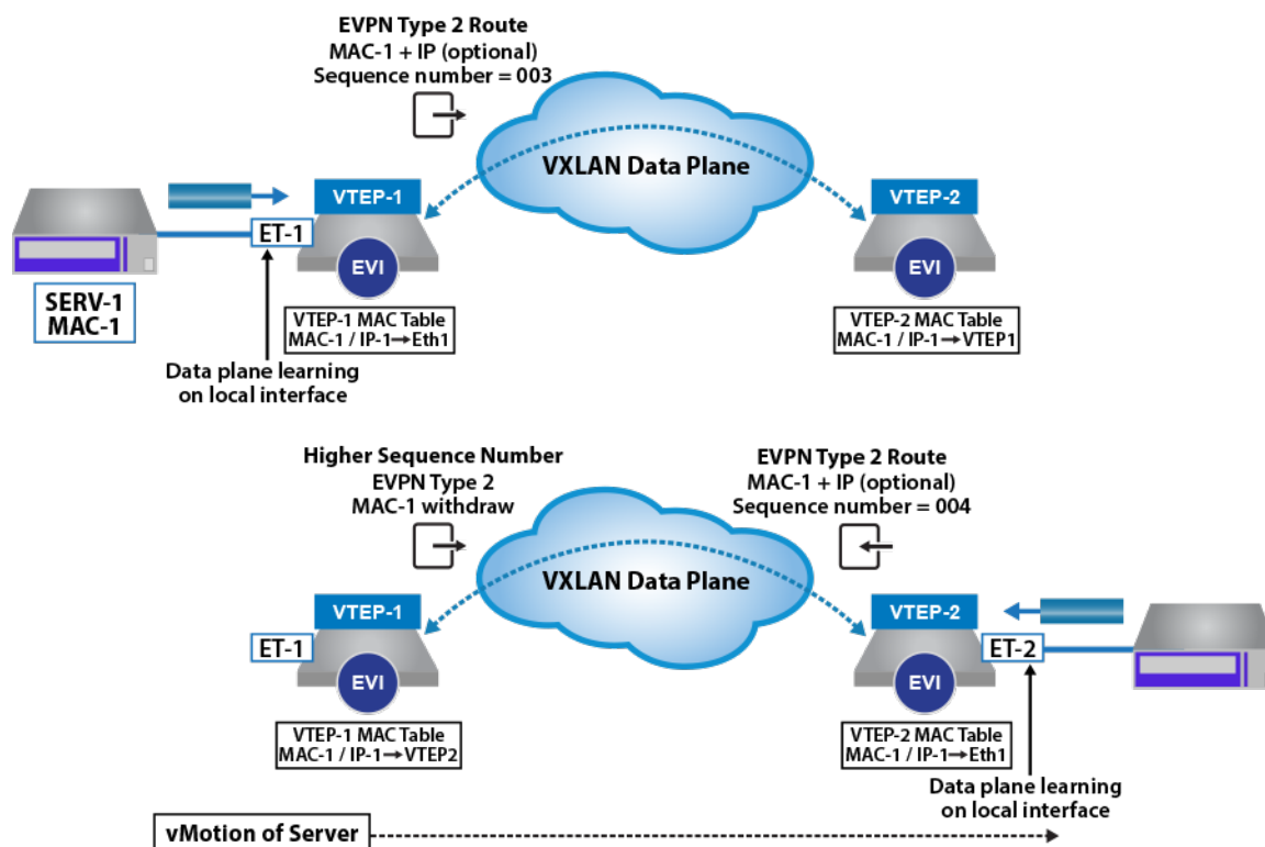
Figure 67: EVPN type-2 MAC Mobility Behavior
