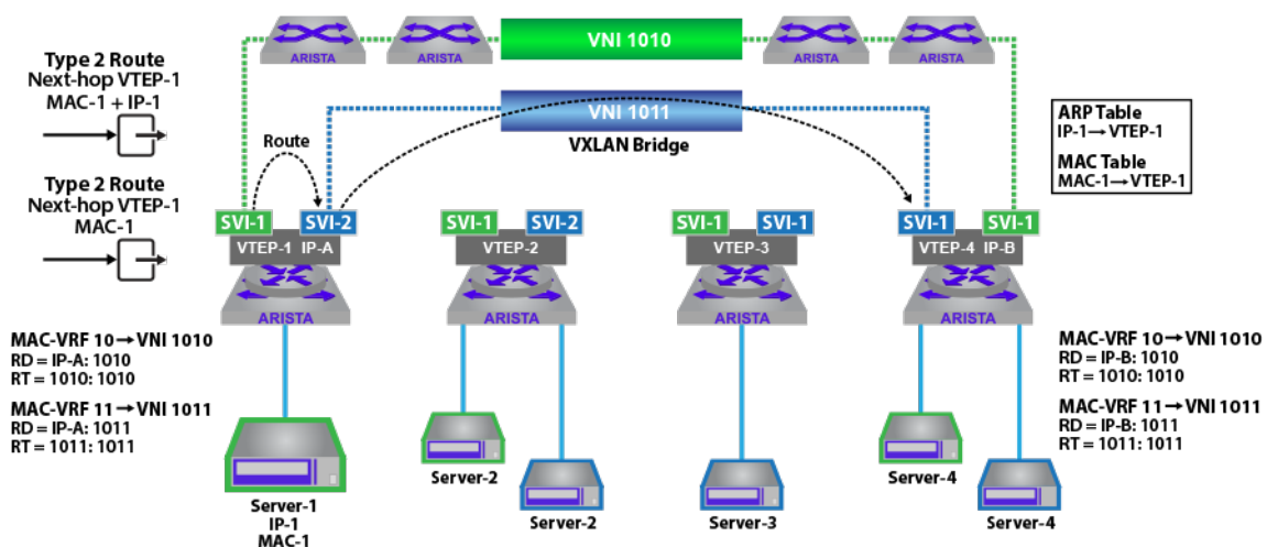
Figure 73: EVPN Symmetric IRB
