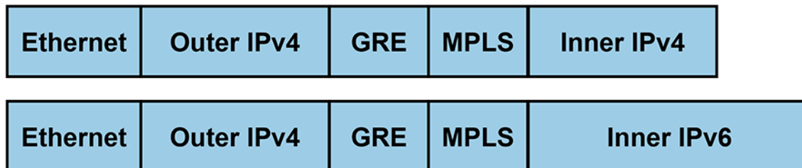
Figure 121: Header Format of Packets
