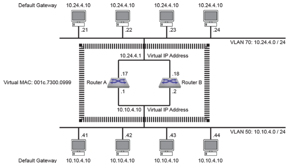
Figure 21: VARP Example Network Diagram
