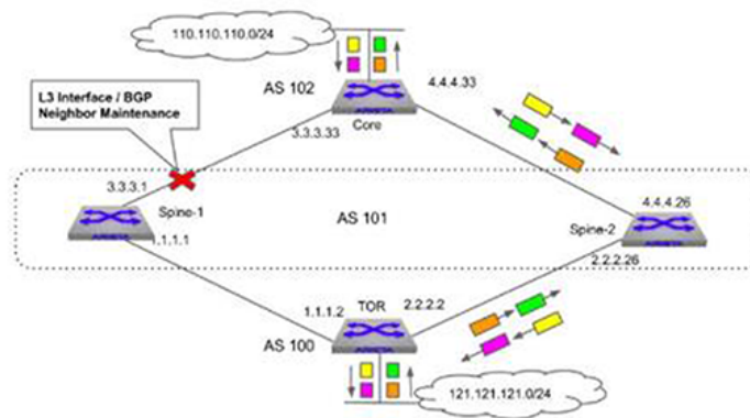
Figure 45: Traffic flow pattern between TOR and Core After unit on Spine-1 is put into Maintenance
