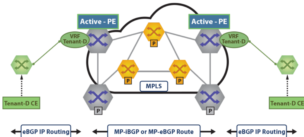
Figure 85: IPv4 & IPv6 VPN Sample Topology
