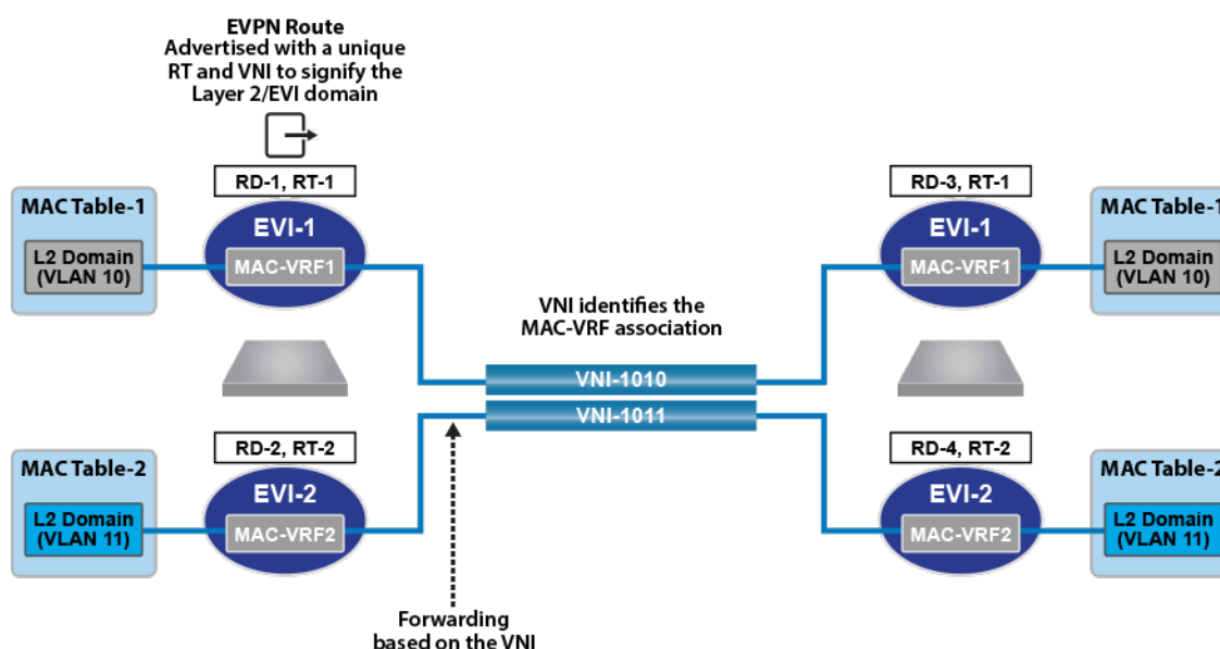
Figure 59: VLAN Based Service Interface
