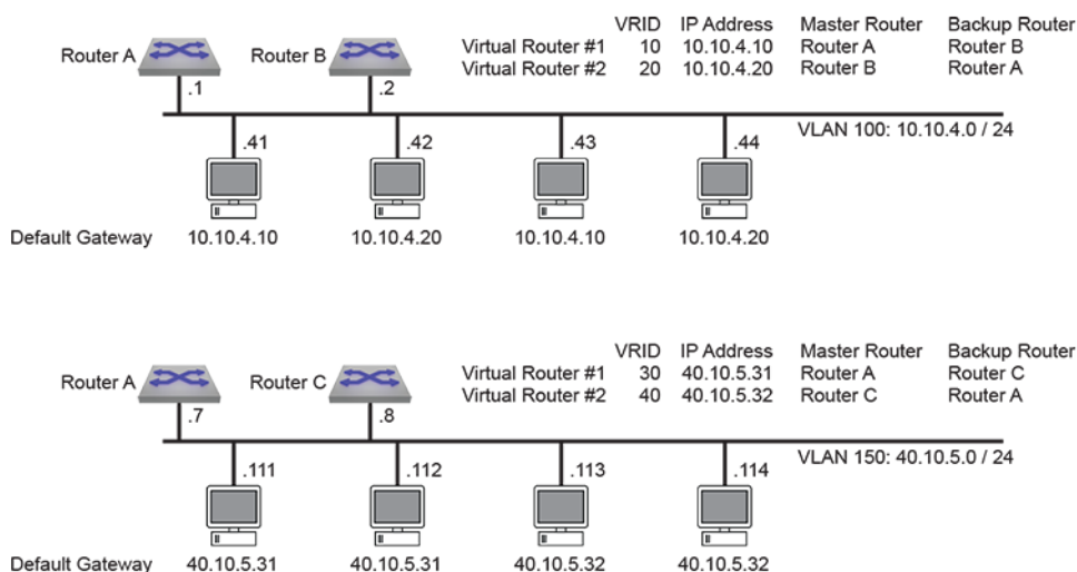
Figure 20: VRRP Example 3 Network Diagram
