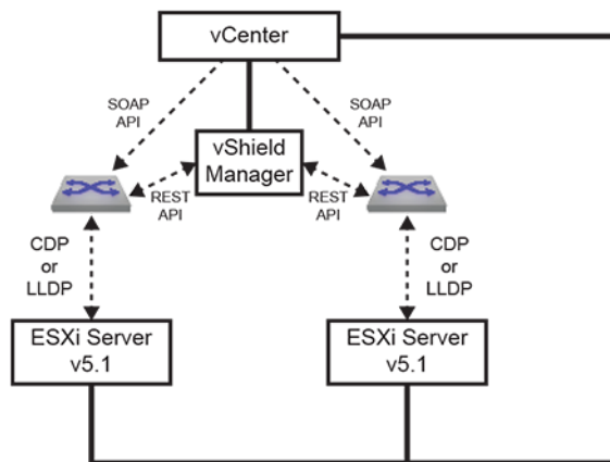
Figure 126: VM Tracer Topology – Monitoring VXLAN Based Configurations
