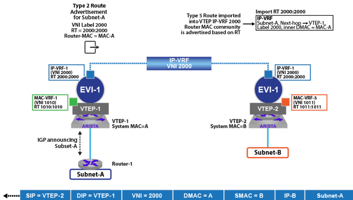
Figure 93: EVPN Route Type-5, Interface-less Update
