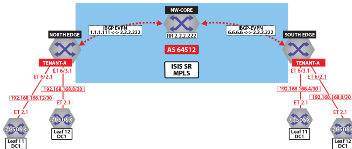
Figure 104: Control Plane Tenant-A Over LDP
