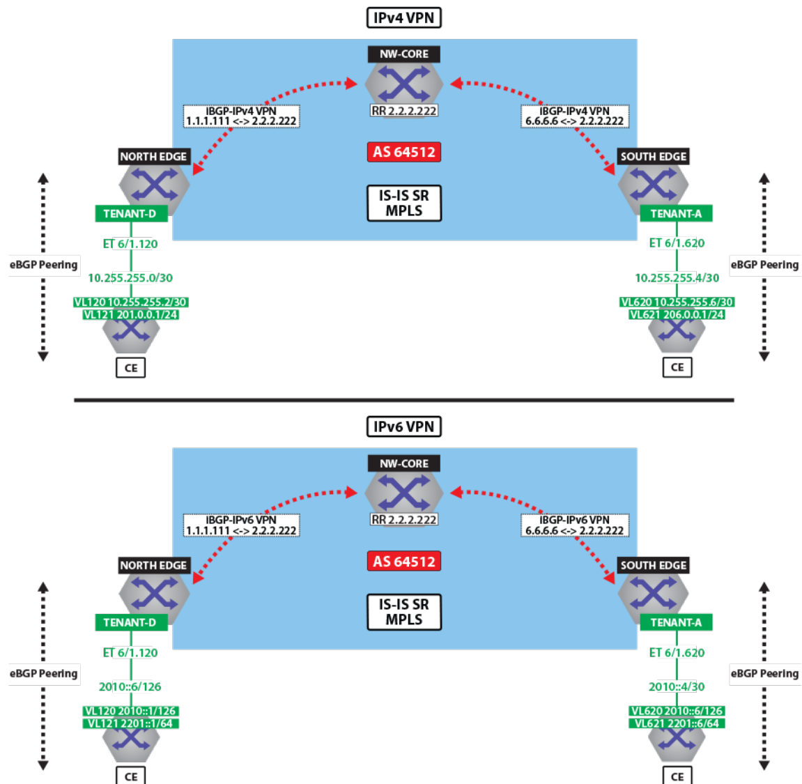
Figure 112: IPv4 VPN and IPv6 VPN Over ISIS-SR MPLS
