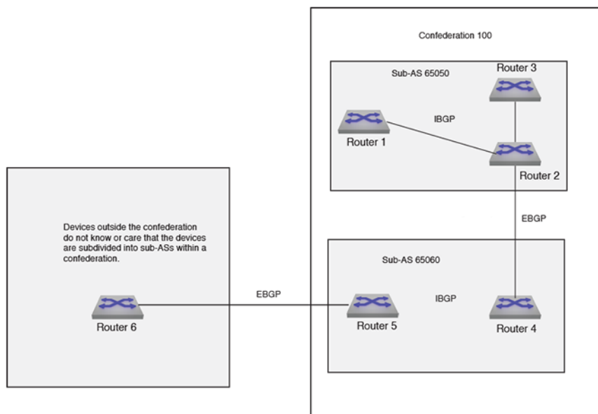
Figure 41: BGP Confederation Example
