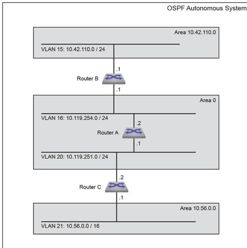
Figure 34: OSPFv2 Example 2
