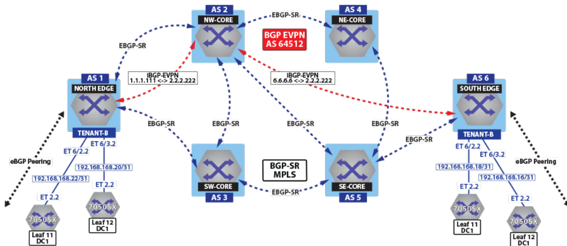
Figure 108: Control Plane Tenant-b Over BGP-SR
