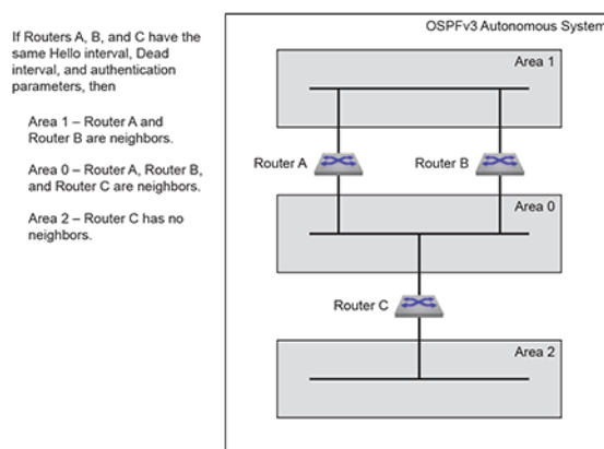
Figure 37: OSPFv3 Neighbors
