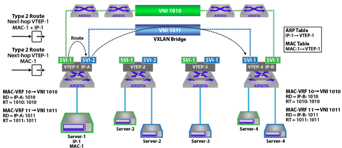
Figure 70: EVPN Asymmetric IRB
