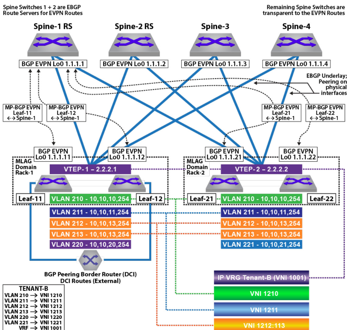
Figure 99: Tenant-B: Asymmetric IRB
