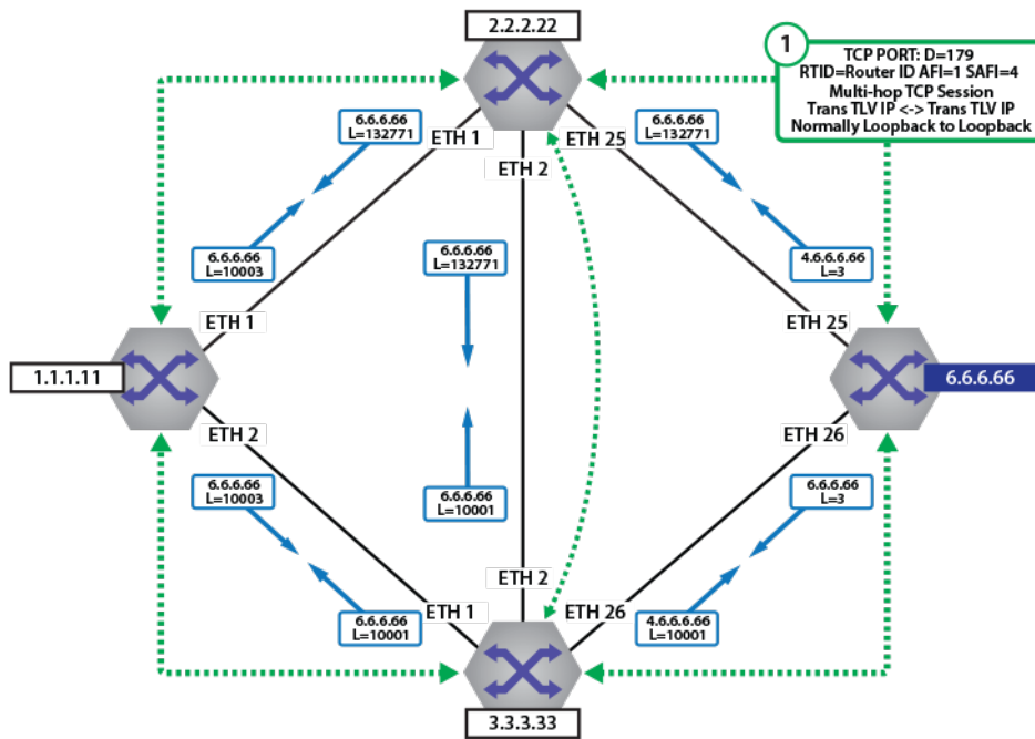
Figure 90: BGP-LU Label Distribution
