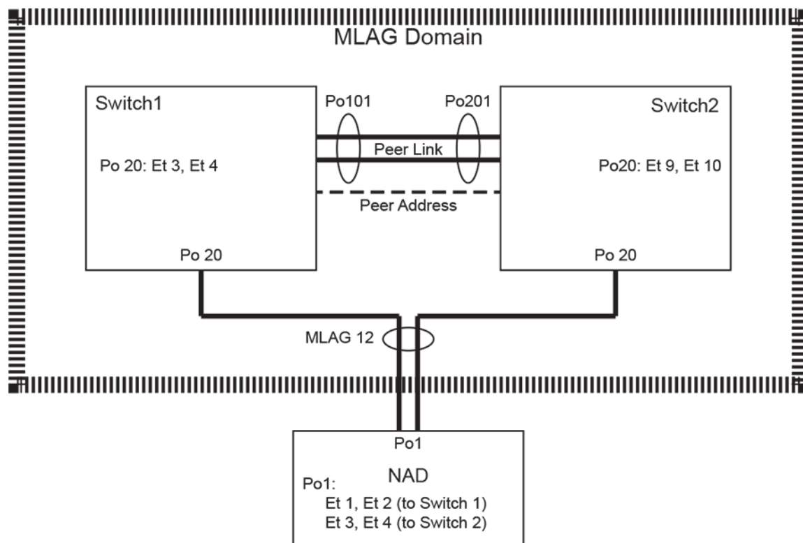
Figure 9: MLAG Interface Configuration
