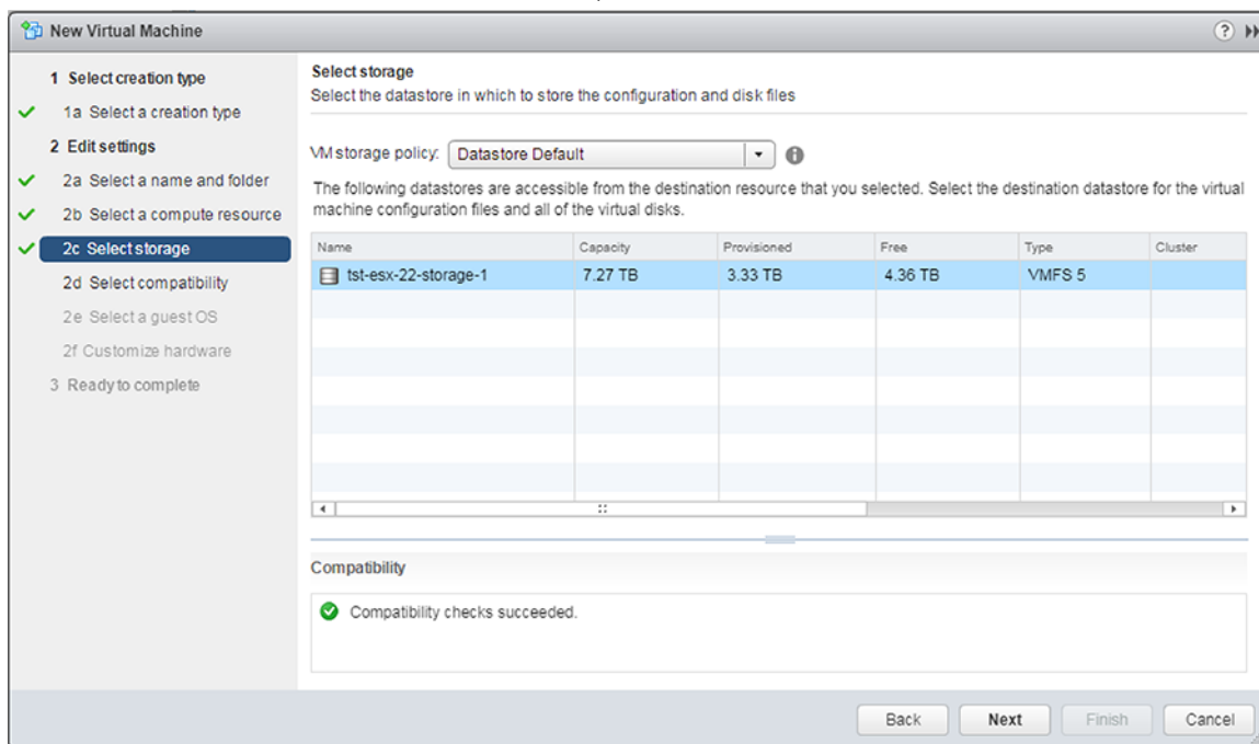
Figure 27: New Virtual Machine dialog (selecting the datastore)
