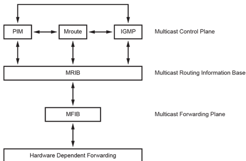
Figure 46: Multicast Architecture
